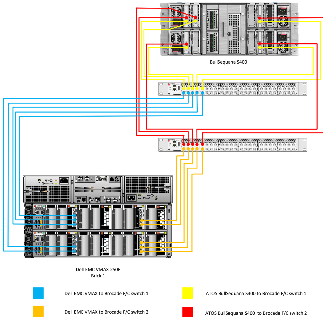
Figure 6: Single server configuration cabling diagram
