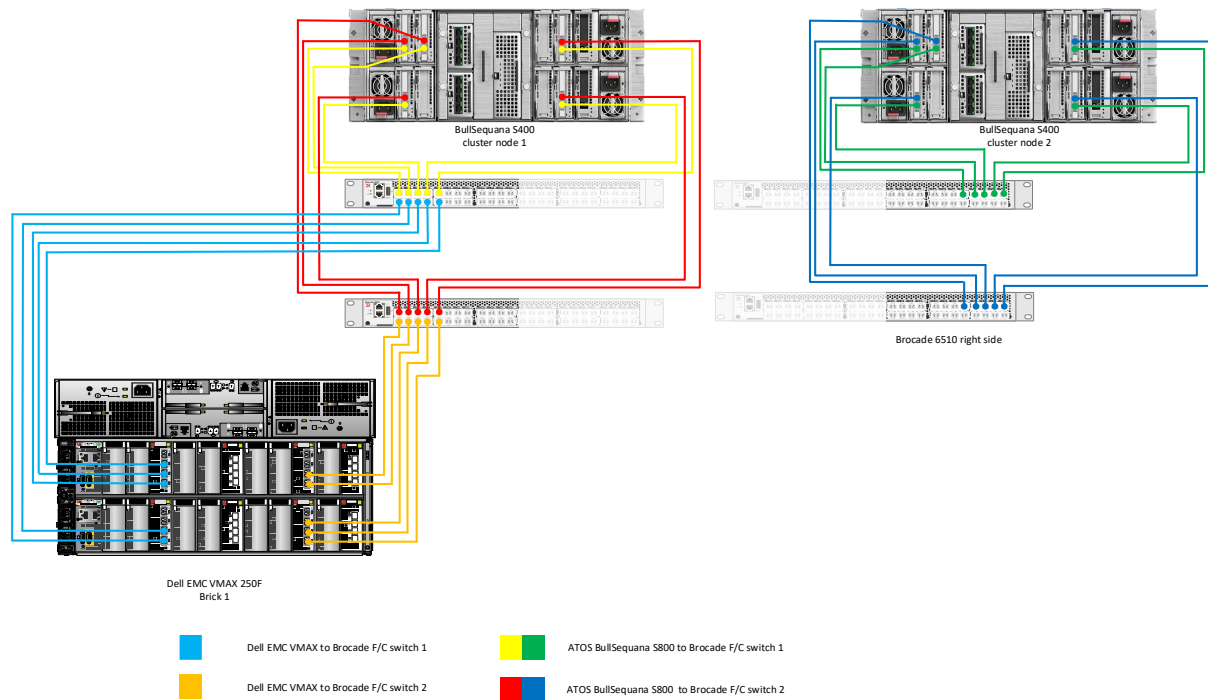
Figure 7: high available server configuration cabling diagram
