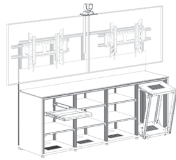
D2/347BM2/ 4-Bay, Standard Profile Cabinet, Dual Display
