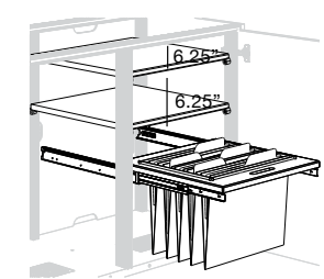
FI/C30/FSK/B File Storage 30B Kit
