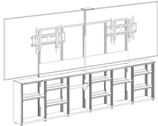
D1/367AM2/ 6-Bay, Low-Profile Wall Cabinet Dual Display*
