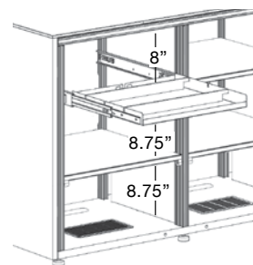
FI/C30/SLK/D Shelving 30D Kit
