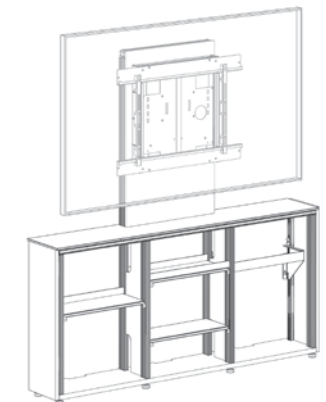
D1/337AL/ 3-Bay, Low-Profile Wall Cabinet EZ-Touch Lift Display
