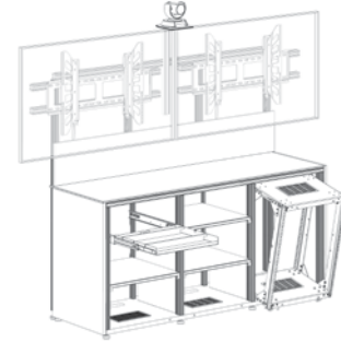
D2/337BM2/ 3-Bay, Standard Profile Cabinet, Dual Display
