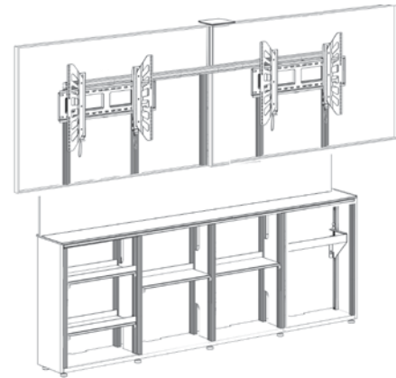
D1/347AM2/ 4-Bay, Low-Profile Wall Cabinet Dual Display
