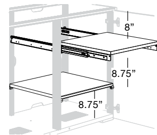
FI/C30/SLK/B Shelving 30B Kit
