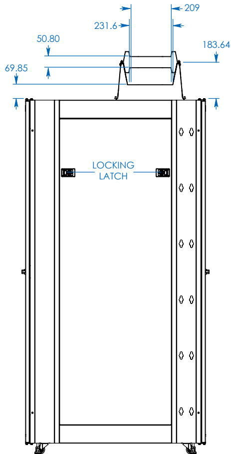
SIDE VIEW
