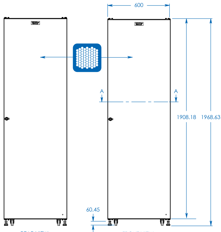
REAR VIEW
