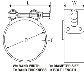
W= BAND WIDTH D= DIAMETER SIZE T= BAND THICKNESS L= BOLT LENGTH
