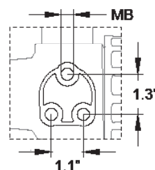
Mounting Dimensions 1 1/2" Ball Valves
