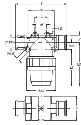
DIMENSIONS 1/2" & 3/4"
