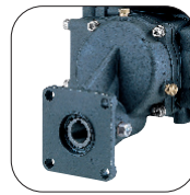
GR-GCI3/4 Version With AR1912 Control Unit and AR1613 Gearbox with 3/4" Hollow Shaft.
