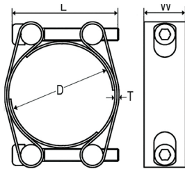
W= BAND WIDTH D= DIAMETER SIZE T= BAND THICKNESS L= BOLT LENGTH
