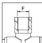
Double swivel female nozzle body - BSP 3/8" fly nut
