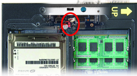
Location of Jumper J9
