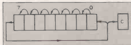
Figure 3b. operation will move the byte one bit to the right or left, and put the bit which falls-off into the carry.
