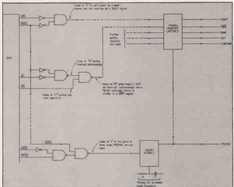
Figure 4. Combinational logic, generation of the SYNC pulse and the transparent latch.
