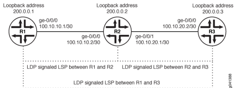
Figure 2: Typical LDP-Signaled LSP
