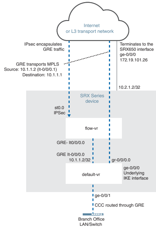
Figure 11: Branch Office Circuit Cross Connect Termination
