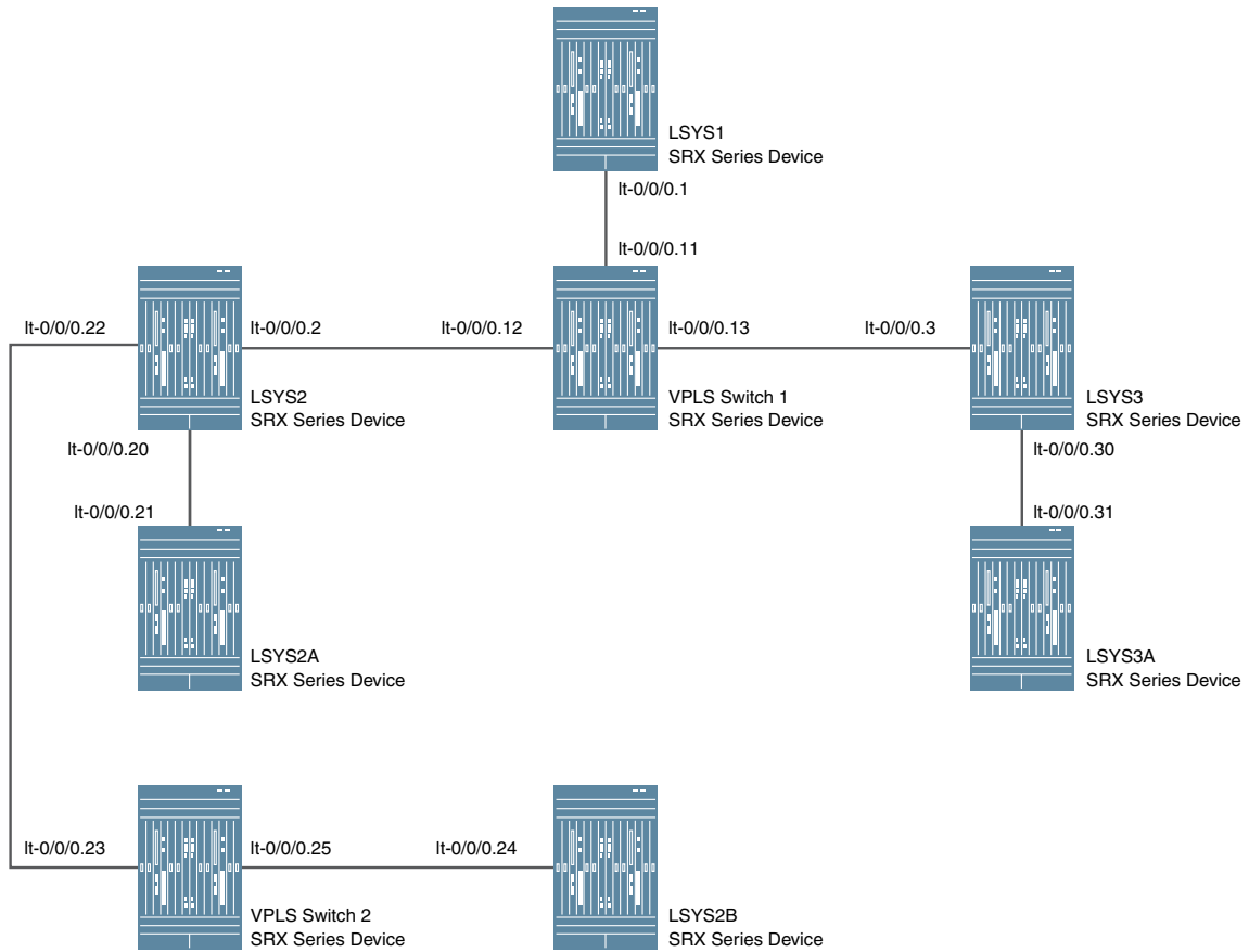
Figure 4: Configuring the interconnect logical systems with VPLS switches
