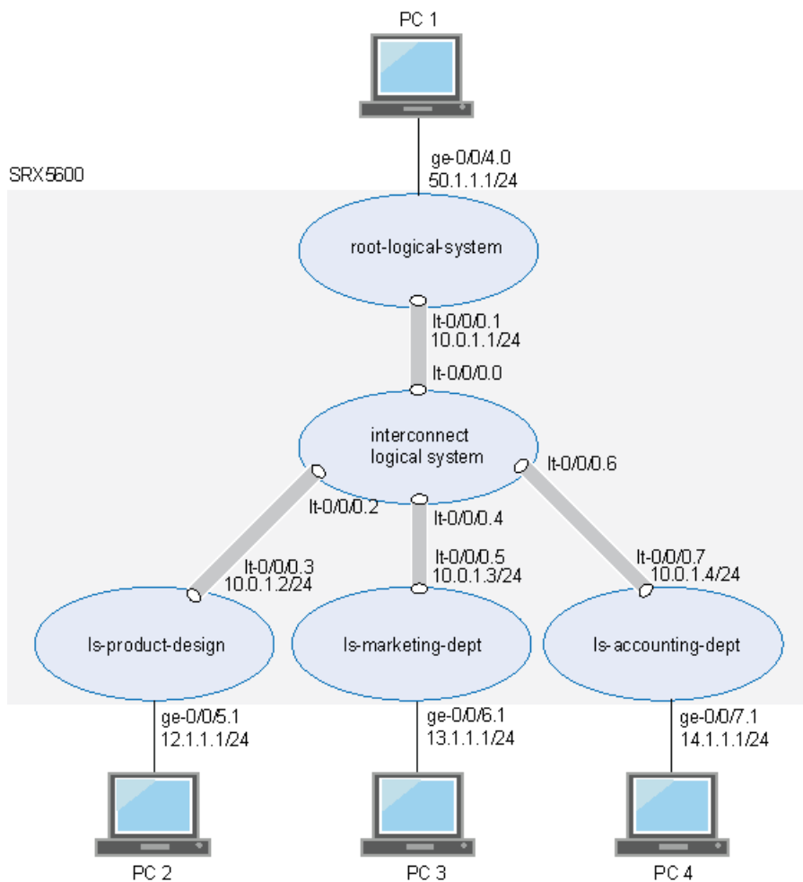
Figure 5: SRX Series Device Configured for Logical Systems
