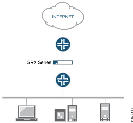
Figure 7: SRX Series Device In-Path Deployment with Secure Wire
