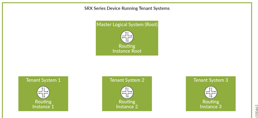
Figure 12: Tenant Systems
