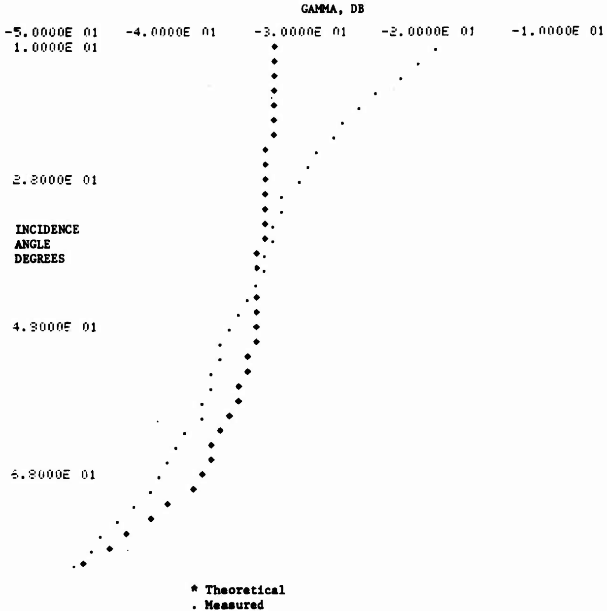
Figure C-7-- BEST MATCH FOR BACKSCATTER FROM CONCRETE AT X-BAND, HORIZONTAL POLARIZATION
