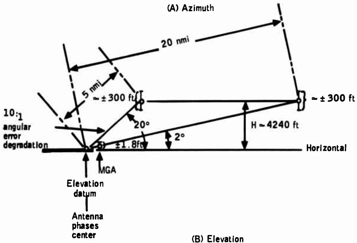
Figure A-2 -- Allowable Degradation Characteristics for Type 3 Subsystem
