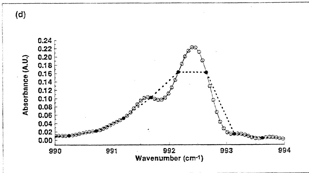
Figure 3. Effect of eight times zero filling on absorbance bands at (a) 908.04\text{ cm}^{-1} , (b) 930.70\text{ cm}^{-1} , (c) 966.74\text{ cm}^{-1} , (d) 992.41\text{ cm}^{-1} , and (e) 1026.80\text{ cm}^{-1} (Continued)
