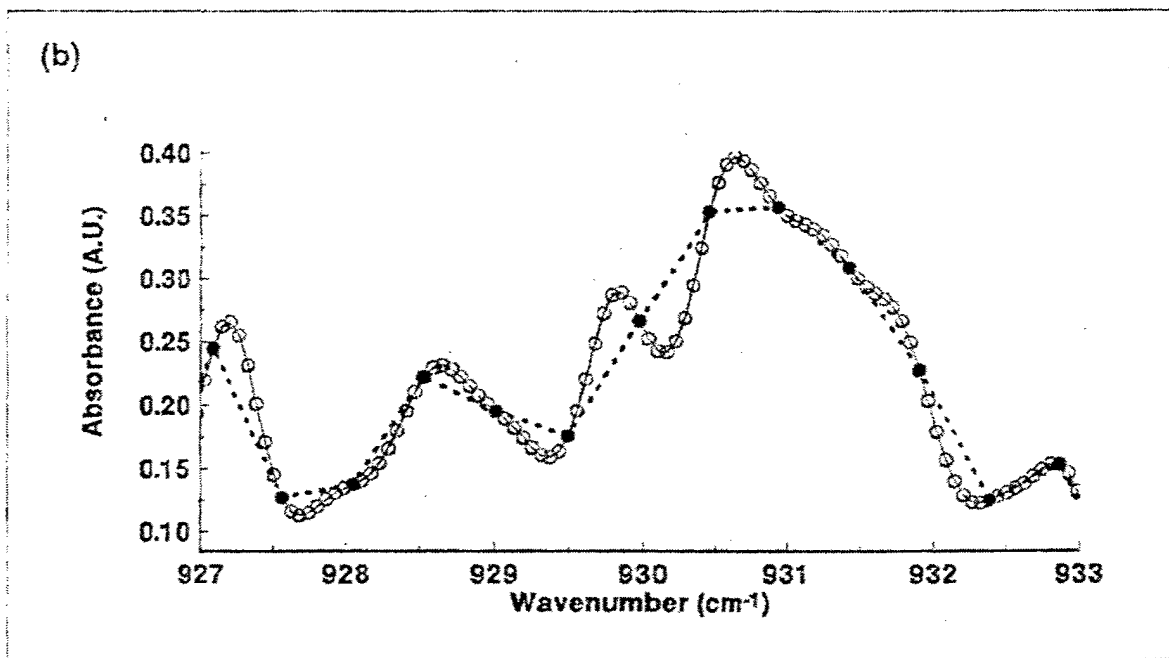
Figure 3. Effect of eight times zero filling on absorbance bands at (a) 908.04\text{ cm}^{-1} , (b) 930.70\text{ cm}^{-1} , (c) 966.74\text{ cm}^{-1} , (d) 992.41\text{ cm}^{-1} , and (e) 1026.80\text{ cm}^{-1}
