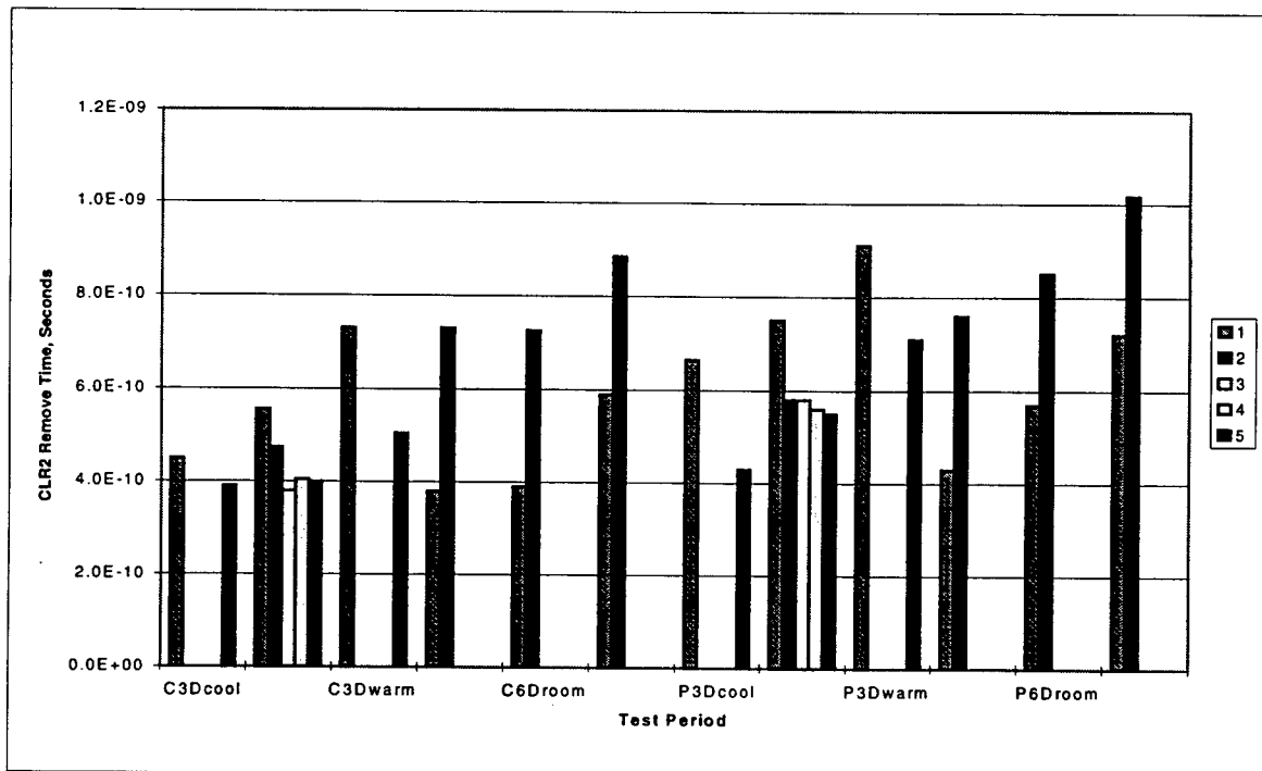
Figure 3.2.5-10: Average CLR2 Removal Time with V_{CC}=5.5V , Lots 3D and 6D (Exposed)
