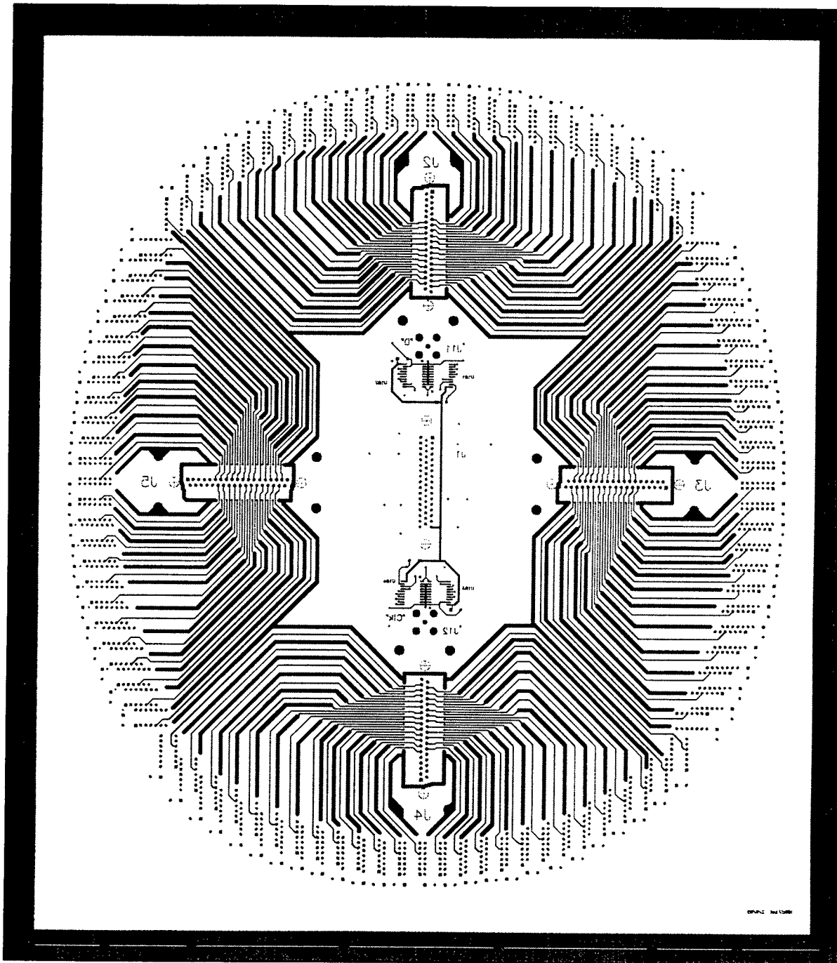
Figure 11.1-4: Bottom Circuit Layer of Digital Test Fixture.
