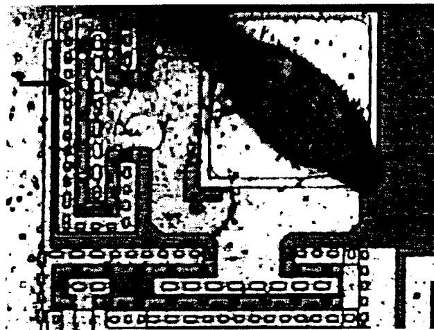
Figure 3.5-3: Photograph of Digital Part #2053 Showing Physical Damage Near Pin 3
