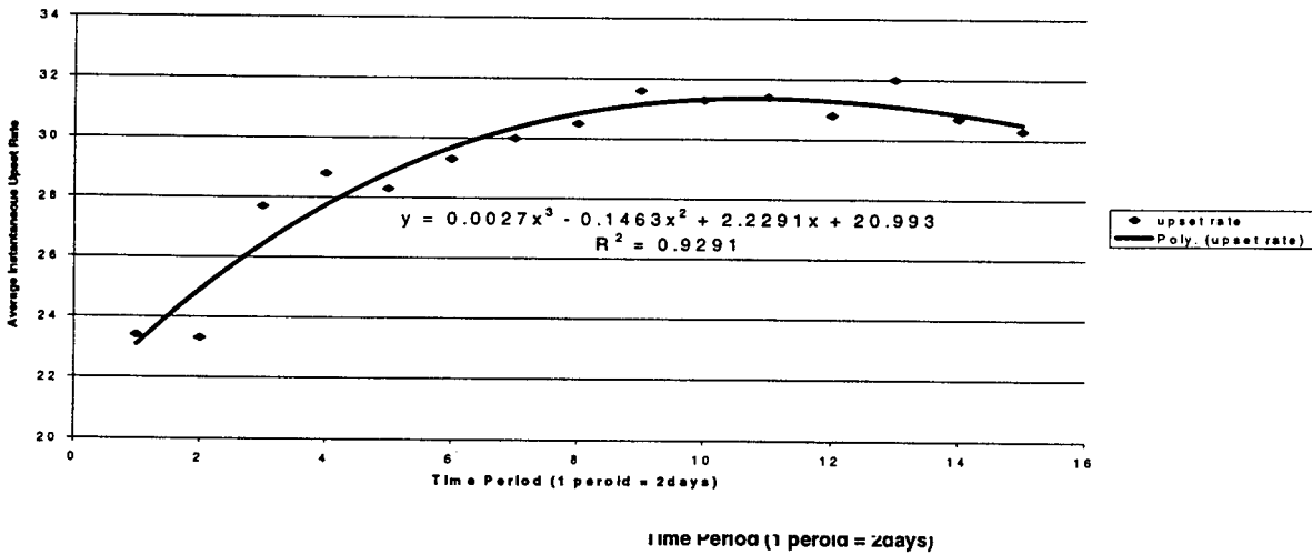
Figure 3.4.3-4: One Dimensional Polynomial Regression Analysis, Test #4
