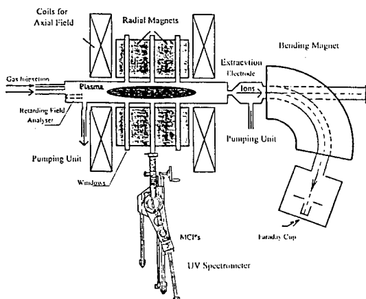
Fig 1. Quadrumafios source and V.U.V. spectrometer.
