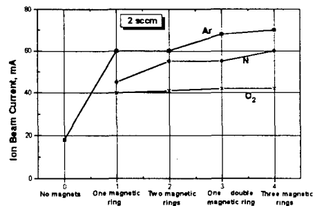
Fig.1. The extracted ion currents of different gases, obtained at fixed HF power input to the ion sources with different magnetic systems.
