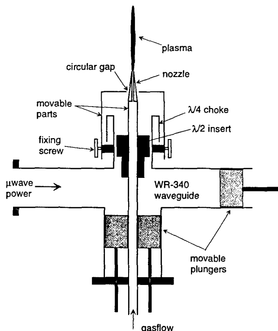
Figure 1: The TIA consists of a coaxial waveguide perpendicular to a standard rectangular waveguide. Due to its specific design the matching is very insensitive for changes in plasma parameters like applied power and gas flow [1].
