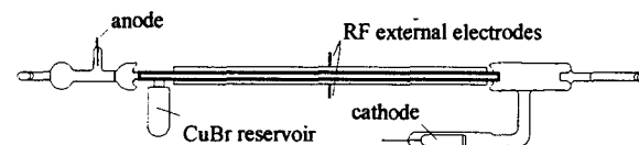
Fig.2 The scheme of the He-CuBr discharge tube.
