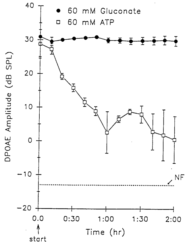
Fig. 3. Magnitude (mean ± S.E.) of the cubic DPOAE recorded in response to 70 dB SPL primaries ( L_1=L_2 ; f_1=6.25 kHz, f_2=7.5 kHz, 2f_1-f_2=5 kHz) during the perfusion of the perilymph compartment of the cochlea with gluconate (60 mM; n=3) and ATP (60 mM; n=3) in acute animals. Start indicates the start of the perfusions (0 h). NF is the representative average noise floor.
