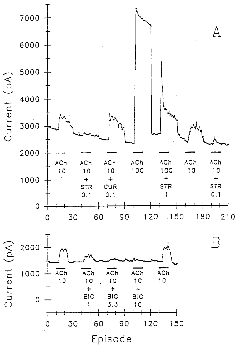
Figure 2-10. Effect of the nontraditional cholinergic antagonists, strychnine (STR) and bicuculline (BIC) on the response to ACh. A: strychnine (0.1 \mu\text{M} ) blocked ACh. The large response (4.7 nA) to ACh (100 \mu\text{M} ) is suppressed in great extent by strychnine at 1 \mu\text{M} . Bicuculline (3.3 and 10 \mu\text{M} ) blocked ACh. Numbers near the drug abbreviations are drug concentrations in \mu\text{M} . Shown are data obtained as voltage clamp current responses at zero mV utilizing the same step protocol as illustrated and described in Figure 2-2. See Figure 2-2 for further description. (From Erostequi et al., 1994, with permission.)
