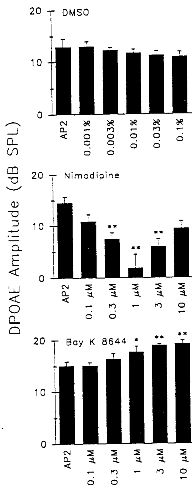
Fig. 4. Effect of increasing concentrations of DMSO, nimodipine in DMSO and Bay K 8644 in DMSO on the first f_2 - f_1 DPOAE amplitude value recorded (point A) following each perfusion. Points that are significantly different from their respective AP2 or DMSO alone concentrations are designated: * P < 0.05 ; ** P < 0.01 . Data are represented as means \pm SE ( n = 5 animals per drug treatment).
