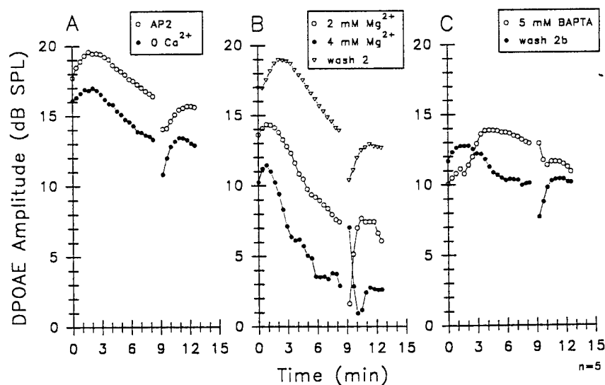
Fig. 2. Effect of altering perilymph Ca^{2+} or Mg^{2+} on perstimulatory changes in f_2 - f_1 amplitude. Response amplitude (means: n = 5 ) recorded following successive perfusions in the same animals of: normal artificial perilymph (AP2), artificial perilymph with no added Ca^{2+} ( 0 Ca^{2+} ), 0 Ca^{2+} artificial perilymph with 2 mM Mg^{2+} (2 mM Mg^{2+} ) or with 4 mM Mg^{2+} (4 mM Mg^{2+} ), a wash perfusion with normal artificial perilymph (wash 2), 0 Ca^{2+} artificial perilymph with 5 mM BAPTA (5 mM BAPTA) and a final wash with normal artificial perilymph (wash 2b). Only every 5th data point is plotted for clearer identification of symbol type. Pooled standard errors were: AP2 = 1.20; 0 Ca^{2+} = 0.75; 2 mM Mg^{2+} = 1.19; 4 mM Mg^{2+} = 2.55; wash 2 = 0.72; 5 mM BAPTA = 1.62 and wash 2b = 1.42 dB. See legend to Fig. 1 for additional information.
