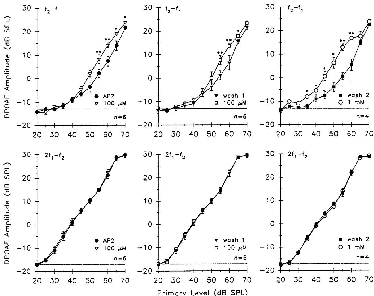
Fig. 9. Effect of suramin on the amplitude growth functions for quadratic ( f_2-f_1 ) and cubic ( 2f_1-f_2 ) DPOEs. Shown are the values obtained following the second control perfusion (AP2), suramin ( 100 \mu\text{M} ), a wash out (wash 1), a second suramin ( 100 \mu\text{M} ), a wash out (wash 2) and a third suramin ( 1 \text{ mM} ) and collection of the data shown in Fig. 7. Data are represented as means \pm S.E. Significance was tested with ANOVA and subsequent Student-Newman-Keuls post hoc multiple range test for all means except wash 2 vs. 1 \text{ mM} suramin means which were compared only to each other by a t -test. Values that are significantly different from their respective AP2 concentrations (or in the case of 1 \text{ mM} suramin, its respective wash 2) are designated: * P < 0.05 ; ** P < 0.01 . The dashed line in each panel represents the average value of the noise floor.
