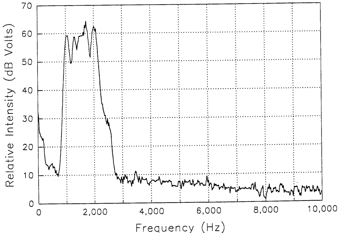
Fig. 1. The frequency spectrum of the 65 dB SPL (A-scale) noise used for continuous exposure. The sound level was monitored with a sound level meter and a 1/2 in. microphone (Brüel & Kjær type 2230 meter and type 4155 microphone) and viewed with a dynamic signal analyzer (Hewlett-Packard 3561A) set at a bandwidth of 95.485 Hz.
