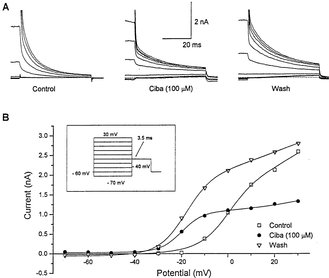
Fig. 5. Tail activation curves of cibacon induced inhibition of voltage gated current in Deiters cells. A: Superimposed tail current traces recorded from a Deiters' cell before (control), during (Ciba) and after (wash) application of cibacon (100 \mu M). Current elicitation was the same as in Fig. 4. B: Tail activation curves constructed from current records in A. Tail current amplitude was measured 3.5 ms after the termination of the pulses as indicated in inset. The tail activation curves were best fitted to a double Boltzmann function. The parameters for the fits: V_{h1} = -3.7 \pm 3.2 mV, K_1 = 5.4 \pm 0.3 mV, V_{h2} = 35.4 \pm 2.7 mV, and K_2 = 17.9 \pm 1.2 mV for the control ( n=3 ); V_{h1} = -20.7 \pm 1.2 mV, K_1 = 5.1 \pm 0.3 mV, V_{h2} = 34.3 \pm 2.2 mV, and K_2 = 20.8 \pm 2.8 mV for the cibacon ( n=3 ); V_{h1} = -15.2 \pm 1.8 mV, K_1 = 6.2 \pm 0.2 mV, V_{h2} = 27.0 \pm 4.0 mV, and K_2 = 17.4 \pm 1.1 mV for the wash ( n=3 ).
