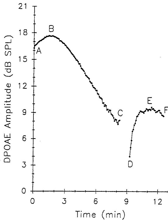
Fig. 6. A typical example of the effect of equilevel ( L_1=L_2=60 dB SPL) primary stimulation on quadratic ( f_2-f_1=1.25 kHz) DPOAE amplitude ( f_1=6.25 kHz, f_2=7.5 kHz). Each data point represents a 10-spectrum average and required 5 s to complete. The break in response amplitude trace (C–D) represents 1 min during which the primaries were turned off. Points A–F were used to calculate magnitudes of component amplitude changes for statistical analyses. This particular trace was obtained following a second control artificial perilymph perfusion (AP2) and is also shown in Fig 7. For reading ease, symbols occur only at every third data point; connecting lines follow all data points.
