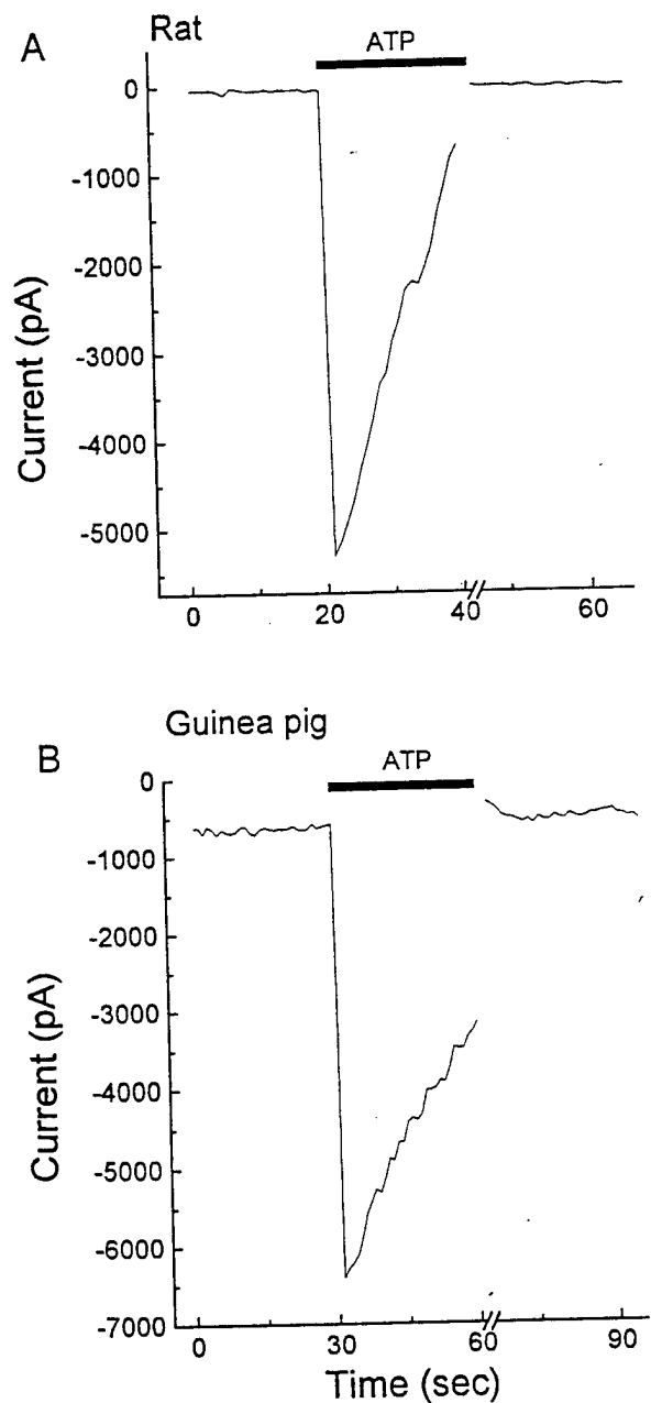
Fig. 5. Examples of an ATP-induced inward current response obtained from a rat Deiters' cell (A) and a guinea pig Deiters' cell (B) at -70 mV. Current-voltage ( I-V ) relationships were recorded in the absence and presence of 10 \mu\text{M} ATP. The voltage command was ramped from -150 mV to +60 mV ( 0.5 mV/ms) and the ramp was presented at the rate of one every second. Membrane potential was held at -60 mV. Traces were constructed from the current evoked by the ramp utilizing the current value obtained at -70 mV.
