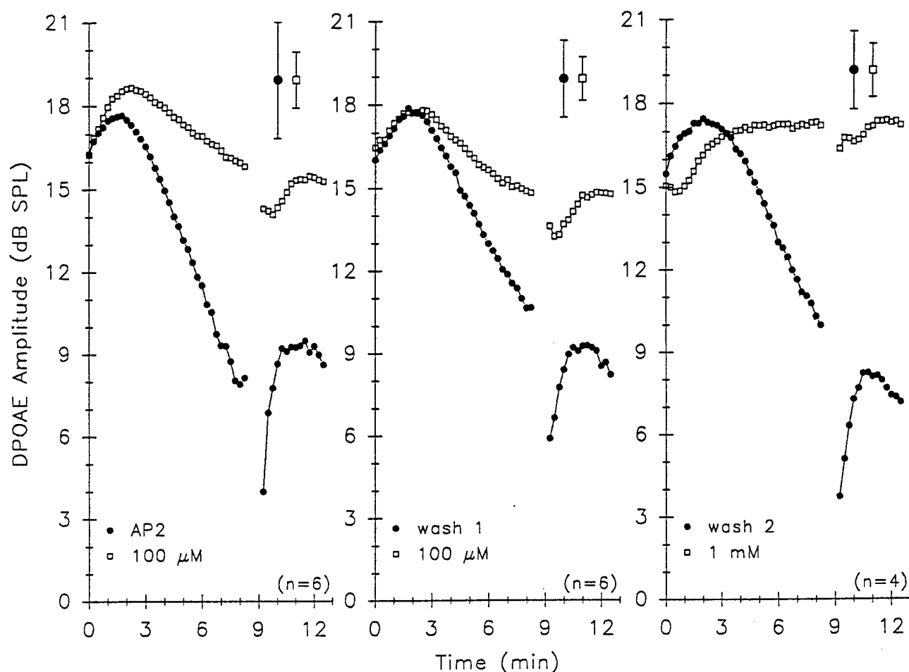
Fig. 7. Effect of suramin on f_2-f_1 DPOAE amplitude alterations during continuous primary stimulation ( f_1=6.25 kHz, f_2=7.5 kHz, L1=L2=60 dB SPL). Response amplitude as recorded following the second control perfusion (AP2), suramin ( 100 \mu\text{M} ), a following wash (wash 1), a second suramin ( 100 \mu\text{M} ), a second wash (wash 2), and a third suramin ( 1 \text{ mM} ). Pooled errors are shown in the upper right hand corner of each frame. See legend for Fig. 6 for additional information.
