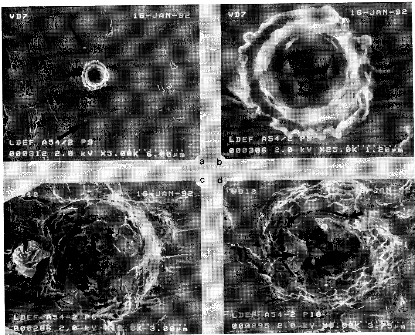
Figure 2. FESEM images of very small LDEF impact craters. (a) Image of a small crater in Al with a prominent raised rim ( \approx 3 microns in diameter); arrows point to melt ejecta which is mostly Al. (b) Enlarged view of the crater in a showing the vermicular morphology of the rim and a melt ball in the crater bottom. (c) Shallow crater with little residual impactor and no raised rim. Arrows point to contamination grains. Note the peculiar polygonal structure of the Al. (d) Another polygonally textured crater with impactor melt residue. Short arrow points to the separation of residue from Al; long arrow points to a contaminant.
