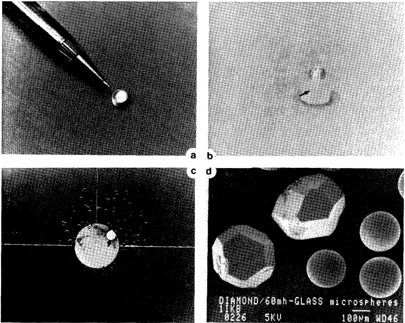
Figure 1. (a) Particle carrier for cluster launches. (b) Carrier with lid set in a plastic sabot. (c) Witness plate showing alignment test pattern of craters produced by boron nitride projectiles. Hole in the center (2.5 cm in dia; covered with mylar film) is the escape hole for the carrier which made the hole in the mylar covering (NE quadrant). Smaller holes in the film are from passage of projectiles. (d) Example of diamond projectiles.
