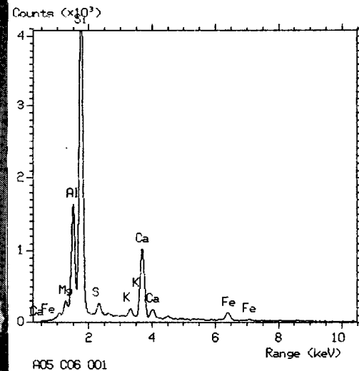
Figure 6. In some cases the projectile collides with the exposed surface at large oblique angles or the projectile contains large voids of porosity, in these cases the impact crater may be asymmetrical. Impact feature number 001, on clamp six, from tray A05 contains grains which appear to be relatively unaffected by collision. Energy dispersive X-ray analysis reveals a typical micrometeoritic spectra.
