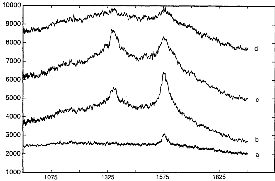
Figure 11. Typical Raman spectra of prelaunched graphite and impactor residues. (a) Precursor graphite. (b) Spectrum from crater centers. (c) Spectrum from crater walls to near the centers. (d) Spectrum from raised rim and outside ejecta.
