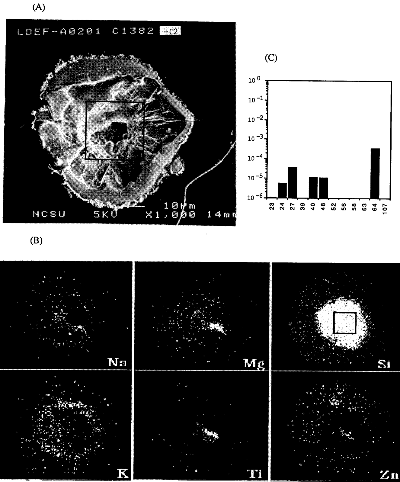
Figure 1. Example of a manmade debris impact (1382-C2) on an IDE sensor mounted on LDEF tray C-3 (Trailing or West side). (A) SEM micrograph. (B) Secondary positive ion images of impact area. Imaged area is 150 \mu\text{m} in diameter. Intensities are uncorrected for relative ion yields. Note exposed area of Si and \text{SiO}_2 defined by the \text{Si}^+ map. (C) Bar graph plot of corrected ion intensity data for boxed area.
