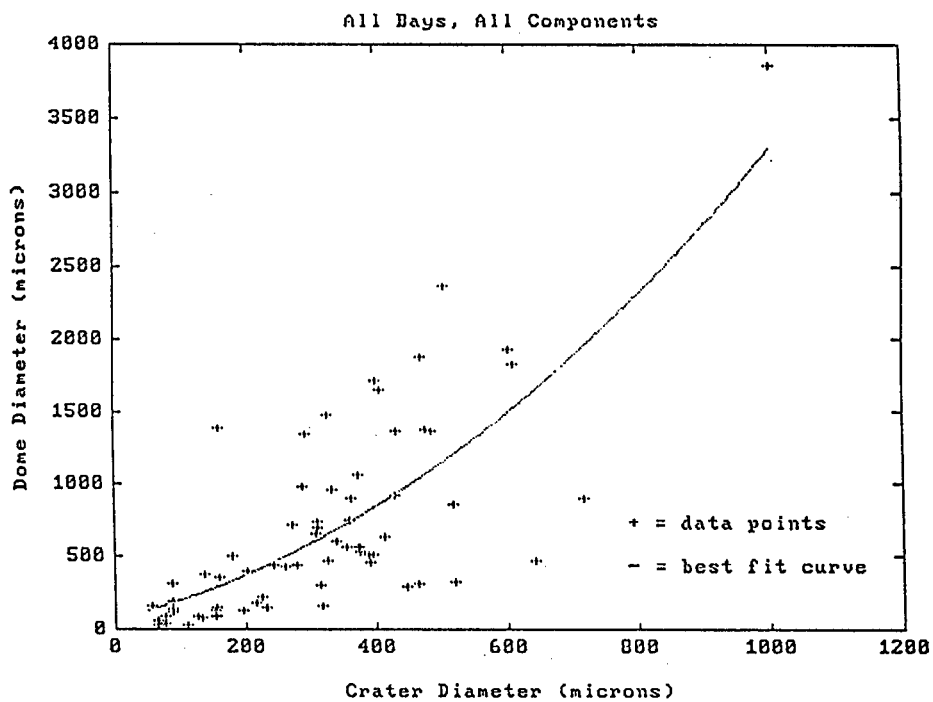
Figure 11b: Comparison plot of crater diameter versus dome diameter for all four components measured in this study.
