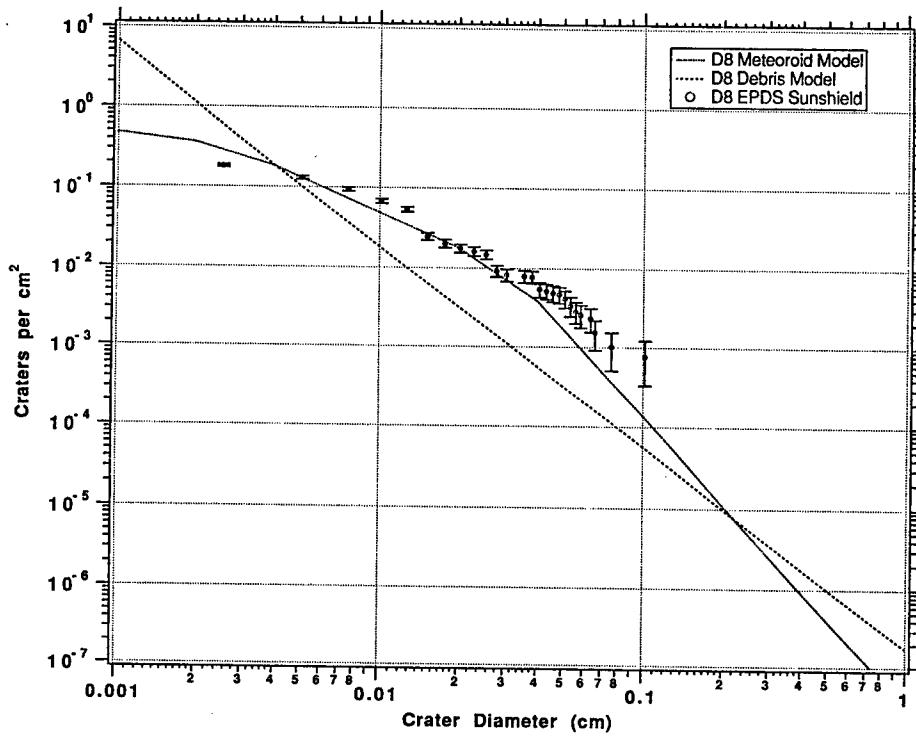
Figure VII-3. D8 EPDS sunshield data compared to meteoroid/debris models.
