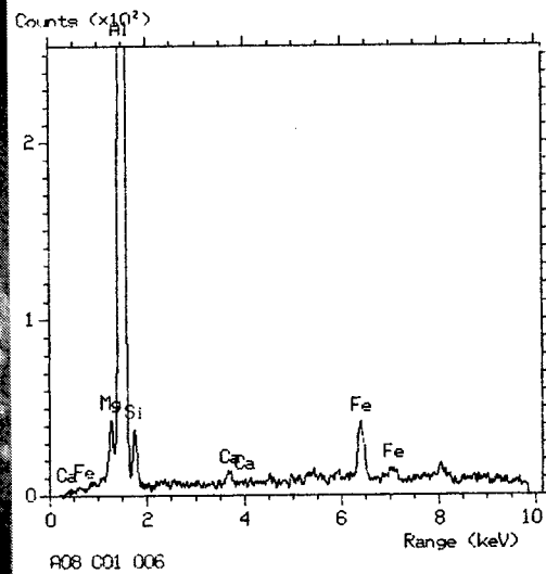
Figure 5. Closer to the leading edge of LDEF, clamp number one of tray A08 has an unusually deep morphology as seen in this oblique view. The walls and bottom to the impact feature are completely coated with micrometeoritic residues. The X-ray spectra retains large amounts of the clamp target material. The anodized layer of the aluminum clamp is very evident when shown as radial cracking around the parameter of the crater.
