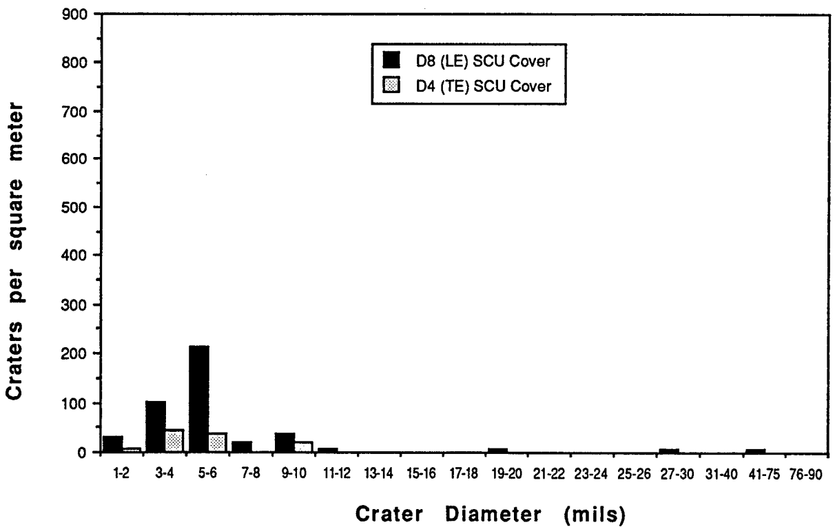
Figure V-12 Linear histograms for painted surfaces.
