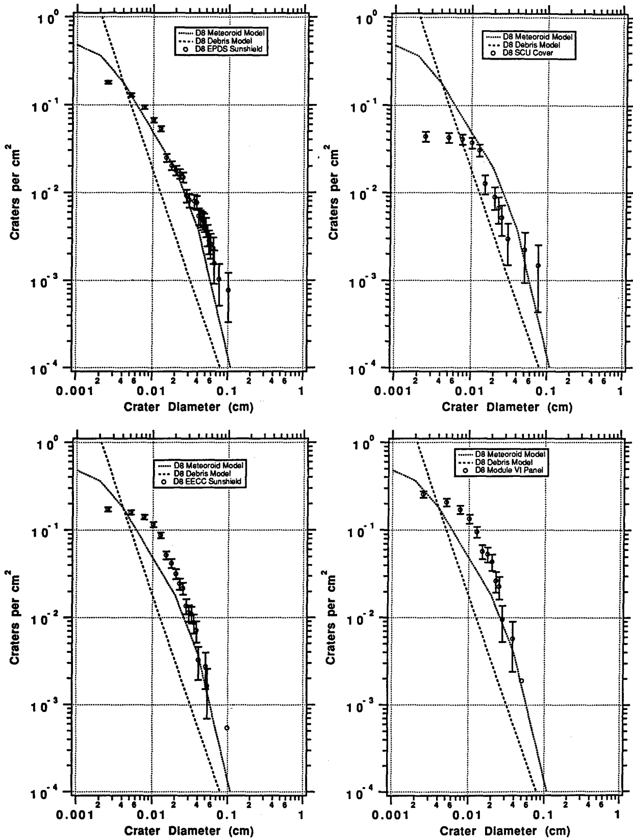
Figure VII-5. Graphs for each D8 surface compared to models.
