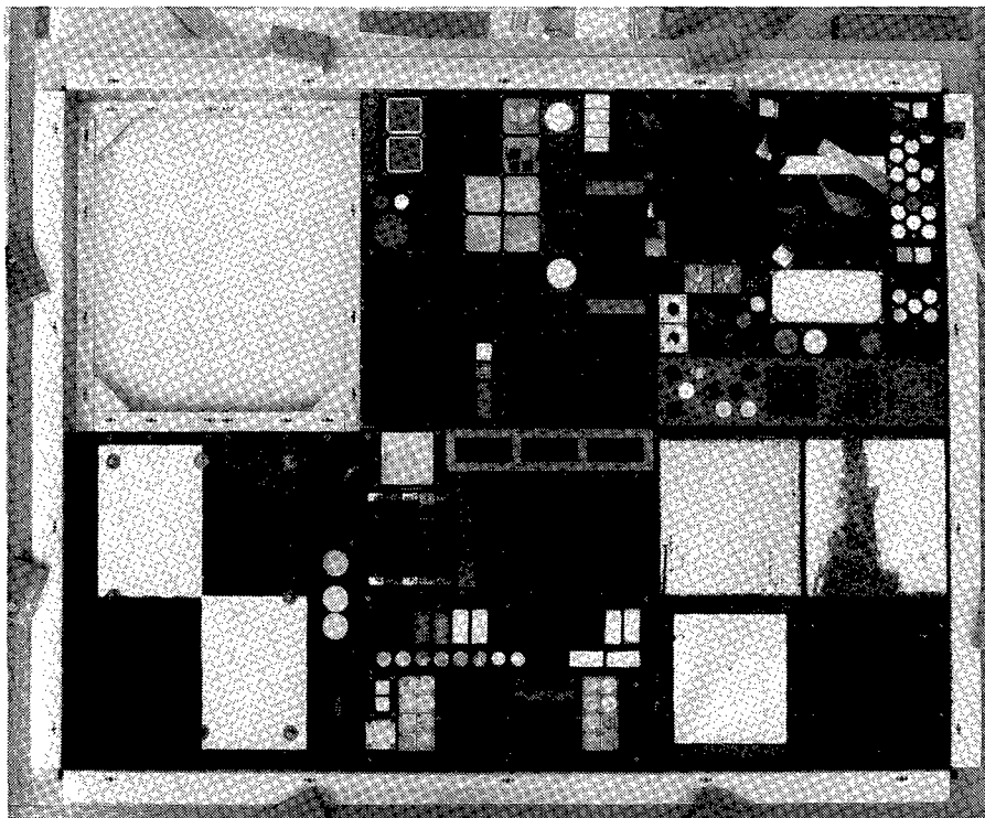
Figure III-5. D9 tray postflight, prior to sample deintegration, in tray holding fixture.
