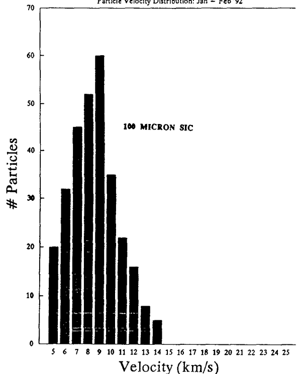
Figure 7. Velocity distribution postulated for meteoroids and the velocity distribution from the hypervelocity facility using nominal 100 micron silicon carbide particles.
