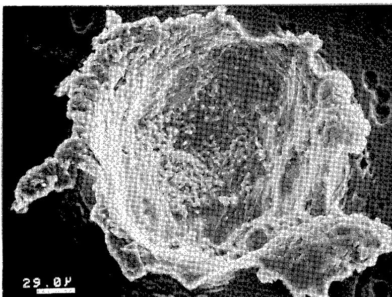
Figure 6. In some cases the projectile collides with the exposed surface at large oblique angles or the projectile contains large voids of porosity, in these cases the impact crater may be asymmetrical. Impact feature number 001, on clamp six, from tray A05 contains grains which appear to be relatively unaffected by collision. Energy dispersive X-ray analysis reveals a typical micrometeoritic spectra.
