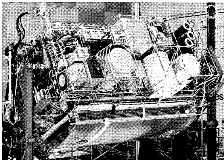
Fig. 4. Total integrated EURECA under testing.
