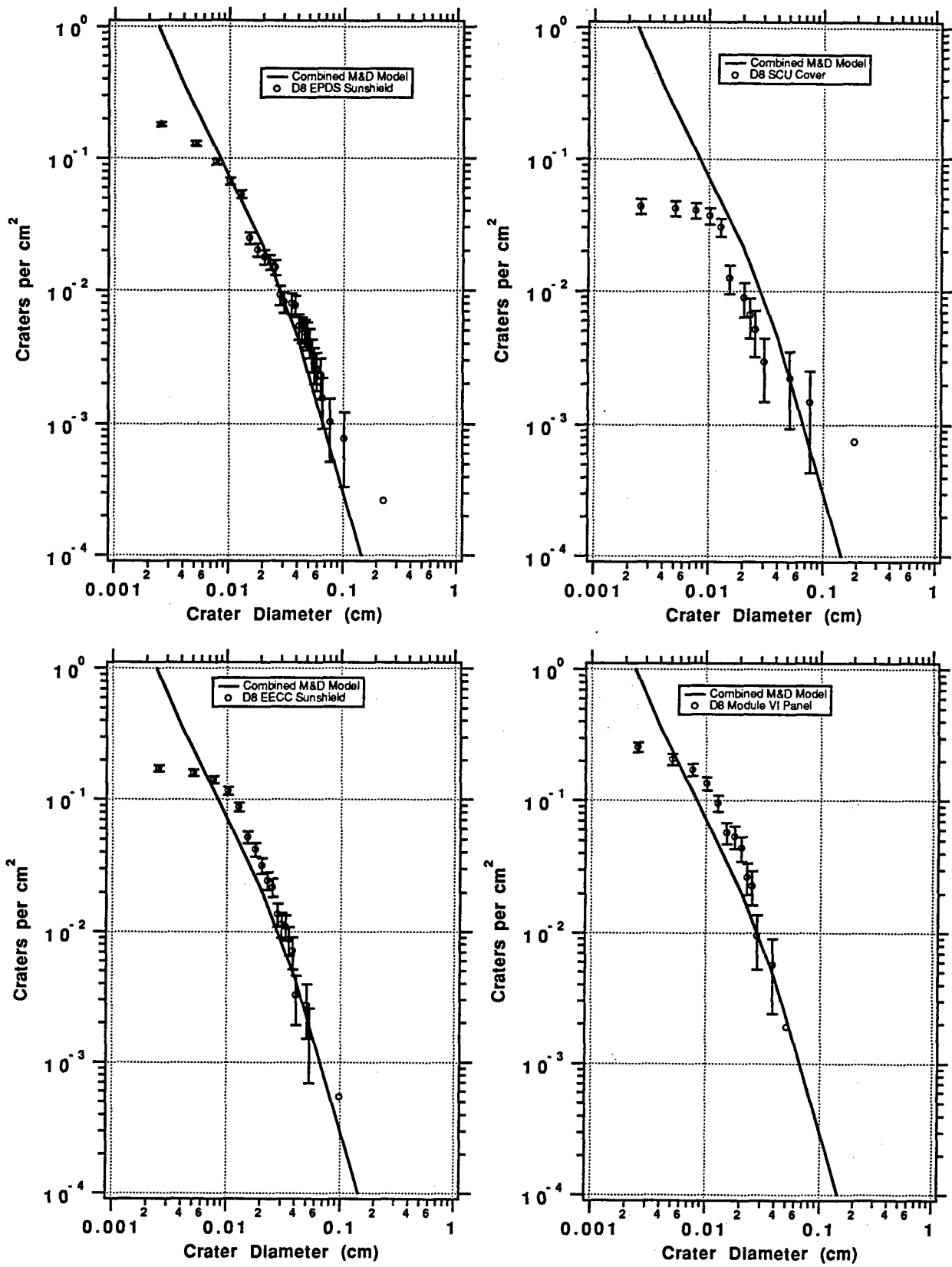
Figure VII-6. Graphs of each D8 surface compared to models' sums.
