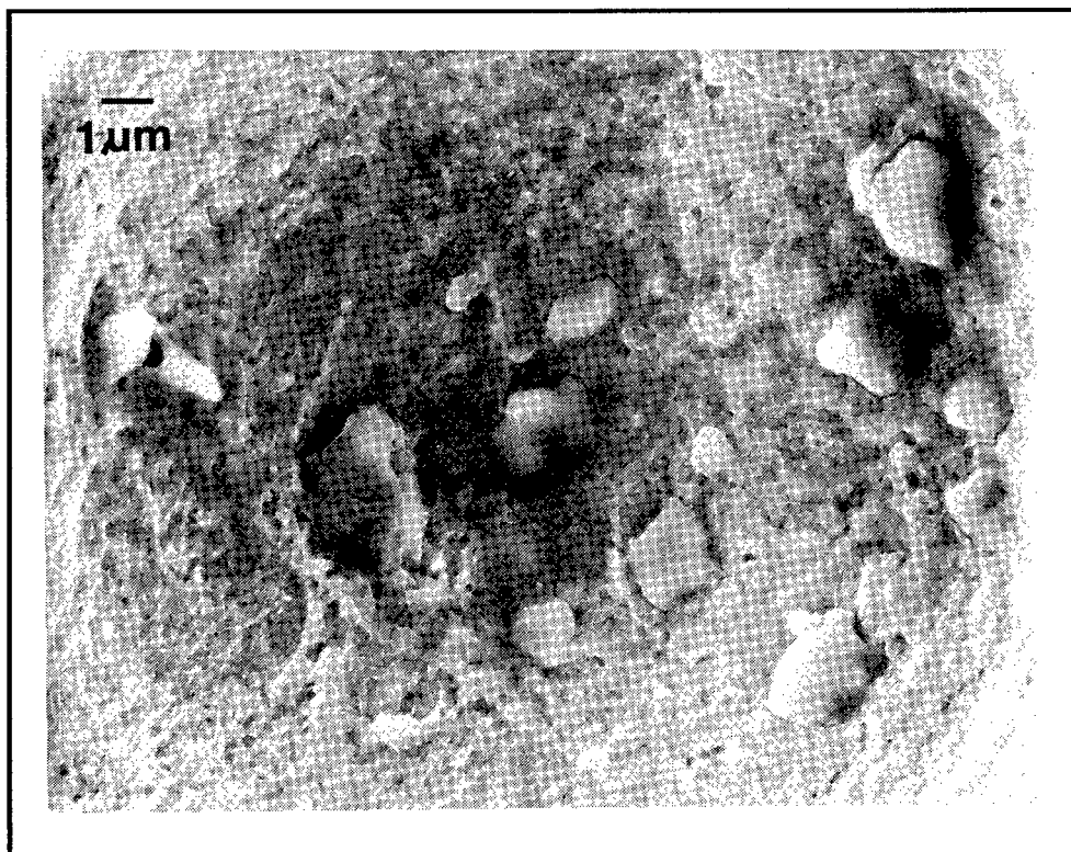
Figure 4 Glass and micron-sized unmelted FeS grains lining the base of a crater in pure Au.
