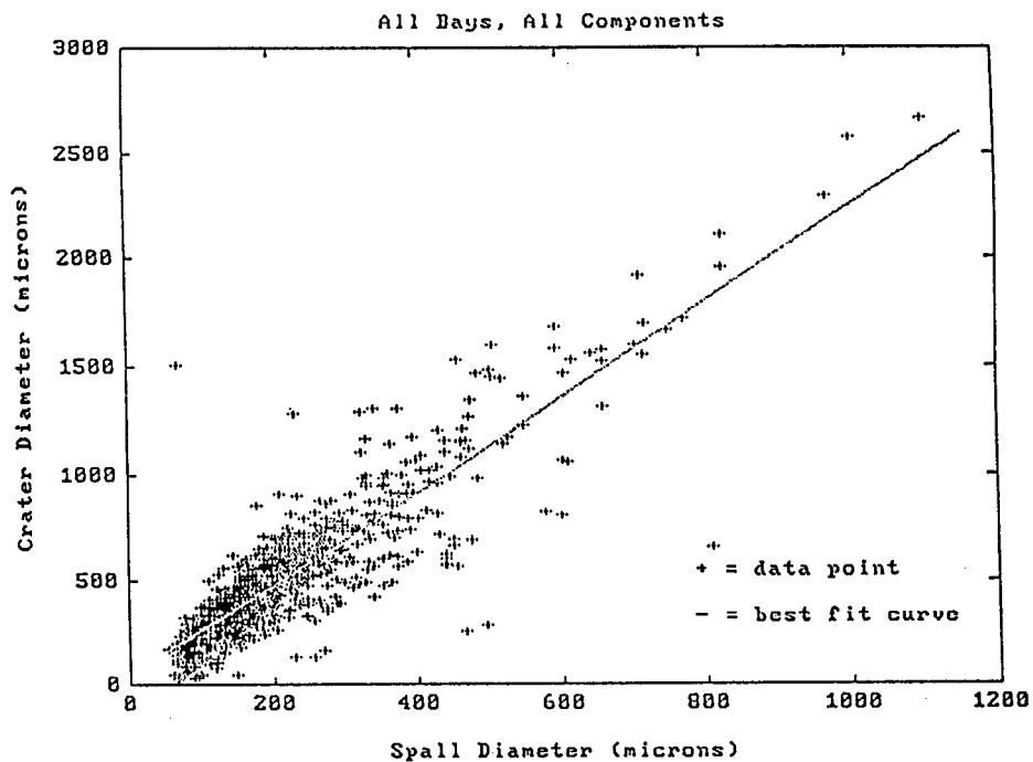
Figure 11a: Comparison plot of crater diameter versus spall diameter for all four components measured in this study.
