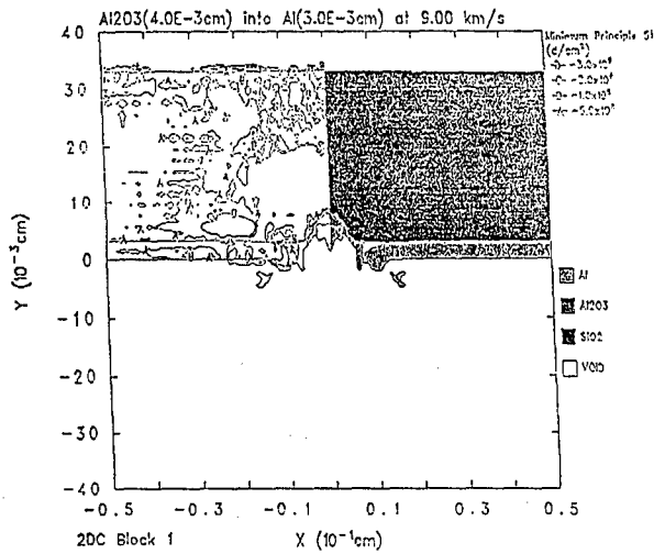
Figure 7: Example results from a CTH run where an alumina projectile impacted a 2-layer target at 9.0 km/s. Time is in sec. Note the factor of 100 vertical exaggeration.
