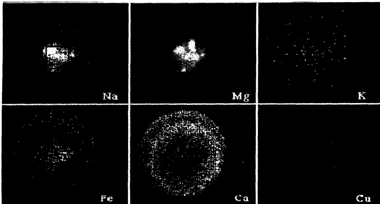
Figure 2. Example of a natural micrometeorite impact (1336-C4) on an IDE sensor mounted on LDEF tray C-3 (Trailing or West side). (A) Optical micrograph. (B) Secondary positive ion images of impact area. Imaged area is 150 \mu\text{m} in diameter. Intensities are uncorrected for relative ion yields. (C) Bar graph plot of corrected ion intensity data for boxed area. Note the low intensity for mass 64 ( \text{Cu}^+ ) in the ion image and the relatively high concentration value displayed in the bar graph. This methodological artifact raises the minimum detectable Cu level to the 100 ppm range. The high \text{Ca}^+ background intensity surrounding the impact has been traced to contamination in the top layer of aluminum on the substrate.
