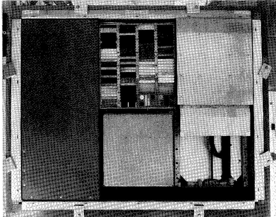
Figure III-8. D4 tray postflight, prior to sample deintegration, in tray holding fixture.
