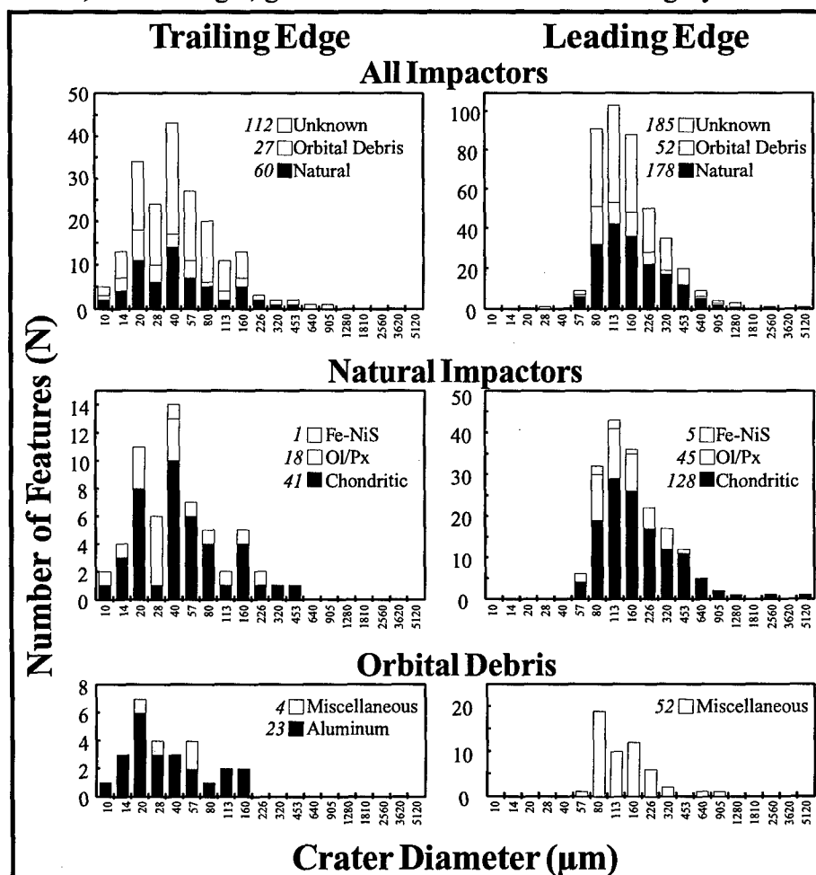
FIGURE 2. Relative frequencies of the different compositional crater classes, as defined by this study, of ~600 impactors that encountered the trailing- and leading-edge CME surfaces.
