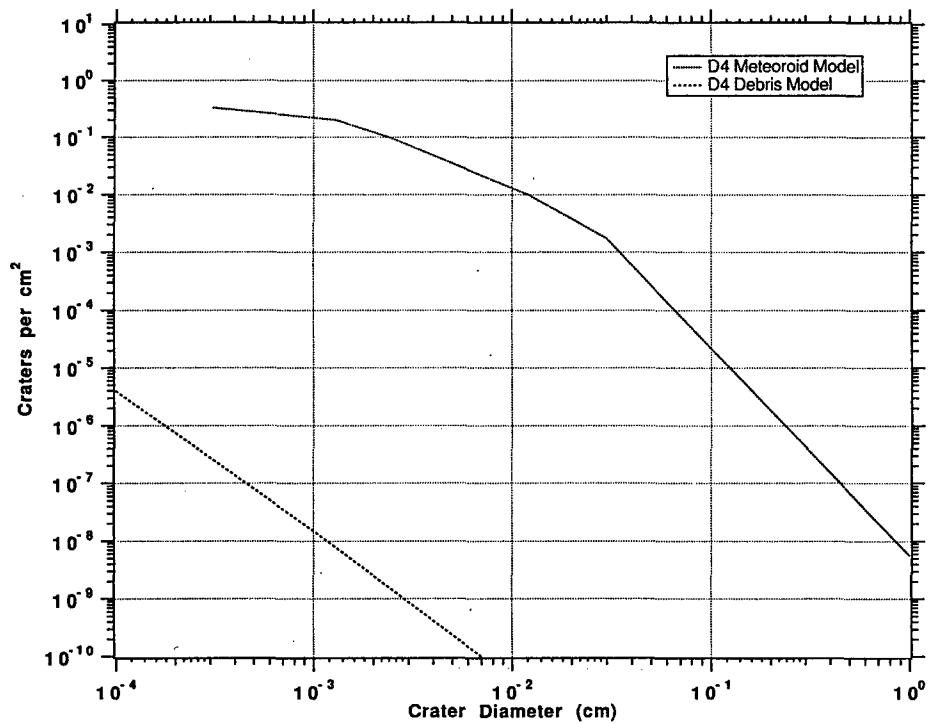
Figure VII-2. Meteoroid and Debris model predictions for LDEF row 4.*
