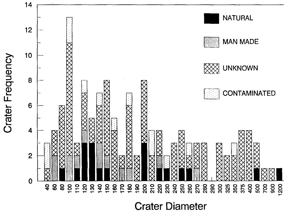
Figure 2. A breakdown of analyzed clamp-impact residues into categories of "natural," "man made," "unknown" and "contaminated."
