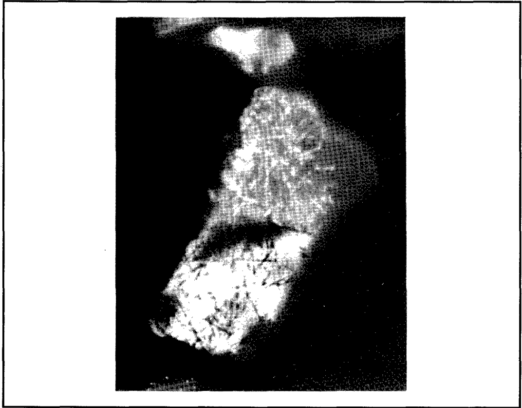
Figure 6 Solar flare tracks in a 0.3 \mu m long anorthite grain extracted from the bottom crater in Figure 5. The tracks are imaged in both darkfield and bright field conditions in the transmission electron microscope. Many of the grains extracted from this crater are track-rich indicating an unshielded exposure to solar cosmic rays for >10,000 years. The preservation of tracks implies only moderate alteration during the cratering event with peak heating not significantly above the track erasure temperature of 600 C.
