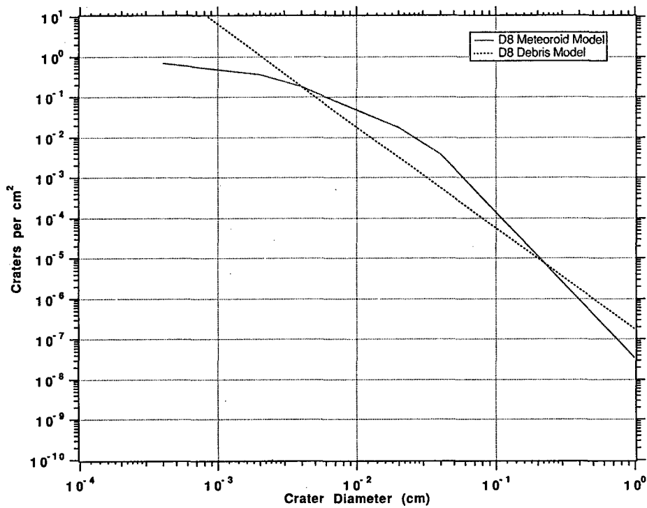
Figure VII-1. Meteoroid and Debris model predictions for LDEF row 8.*
