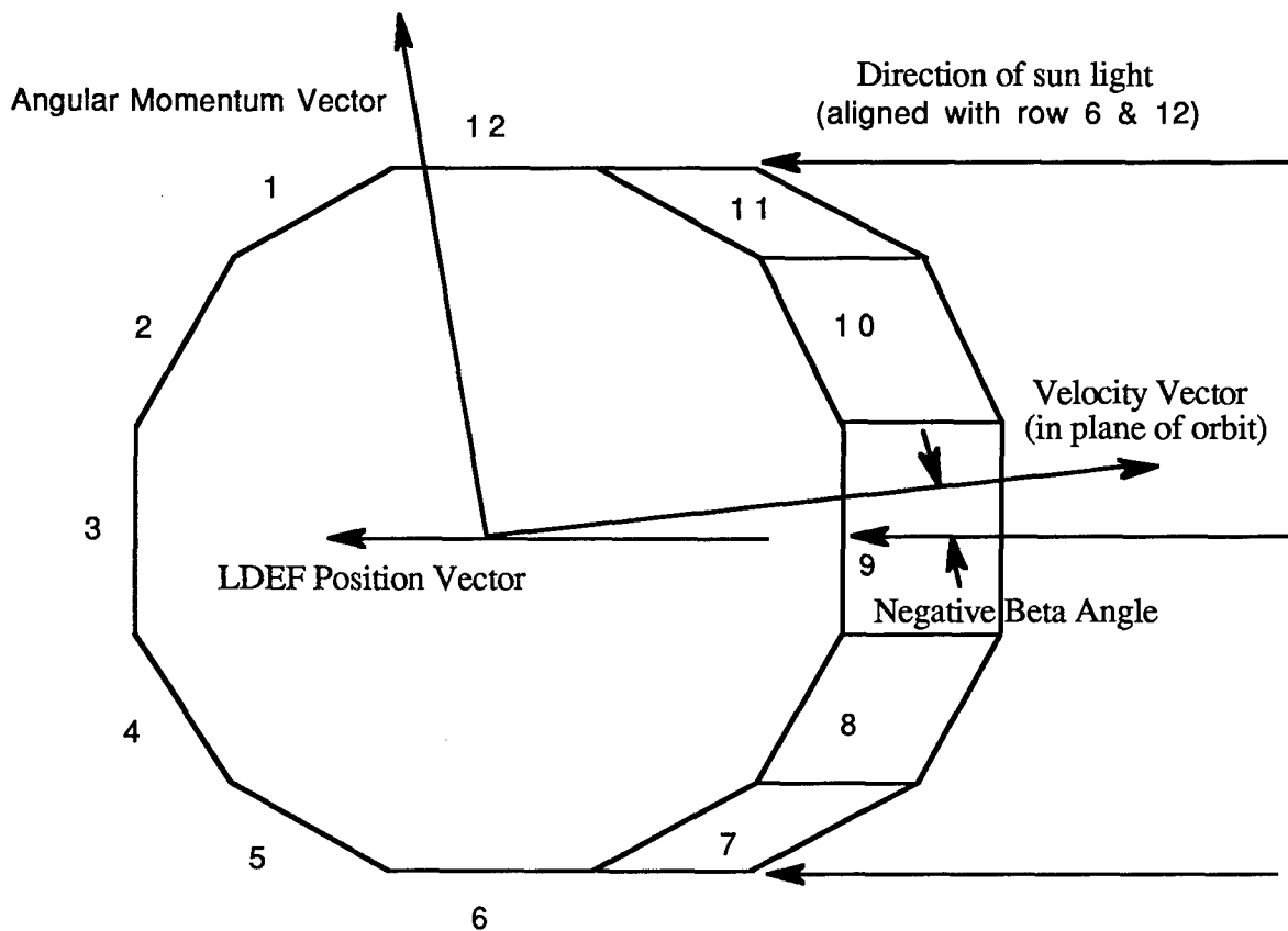
Figure 4. Alignment of yaw and beta angles near sunrise.
