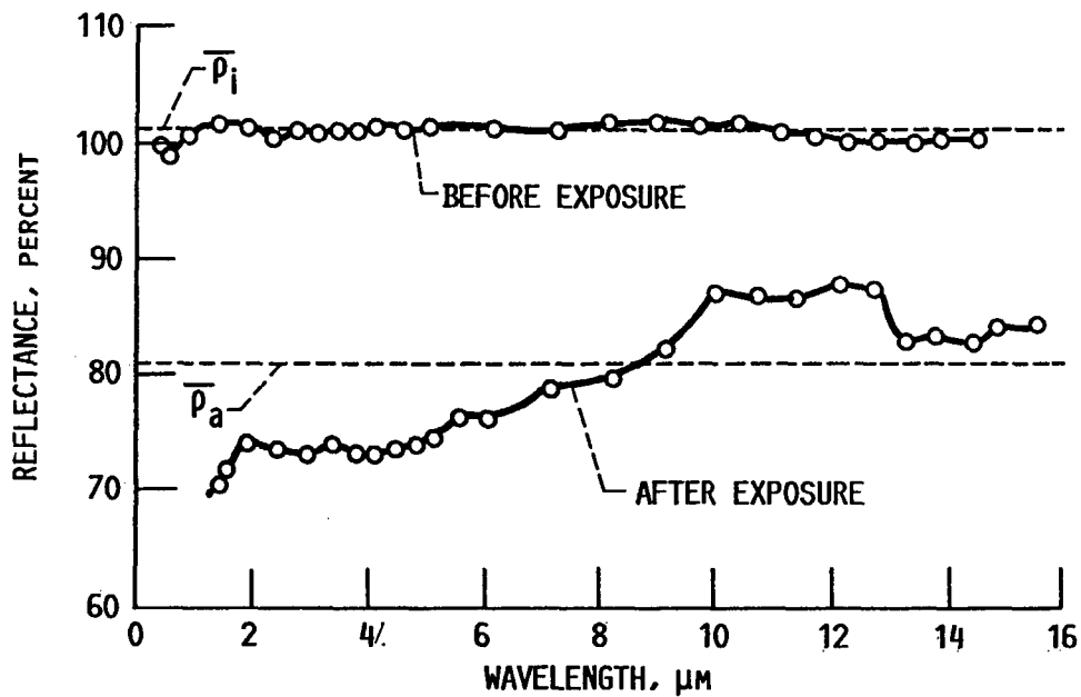
11. Spectral reflectance \rho_{H-A} for 1900Å aluminum on stainless steel substrate exposed to approximately 0.2 \text{ J/cm}^2 of hypervelocity impaction.
