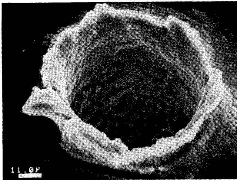
Figure 5. Closer to the leading edge of LDEF, clamp number one of tray A08 has an unusually deep morphology as seen in this oblique view. The walls and bottom to the impact feature are completely coated with micrometeoritic residues. The X-ray spectra retains large amounts of the clamp target material. The anodized layer of the aluminum clamp is very evident when shown as radial cracking around the parameter of the crater.
