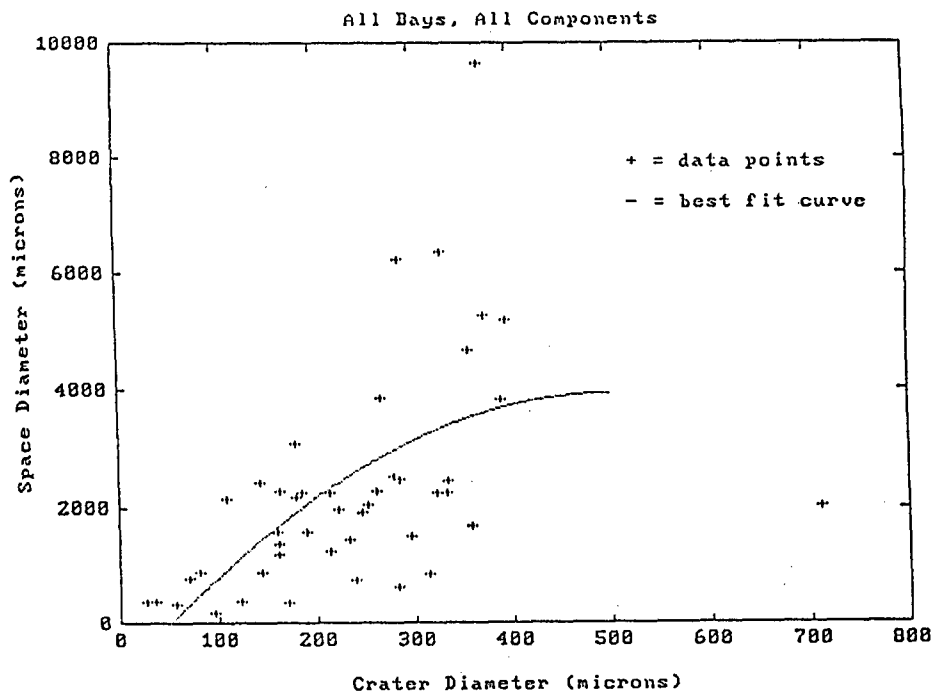
Figure 11c: Comparison plot of crater diameter versus space diameter for all four components measured in this study.
