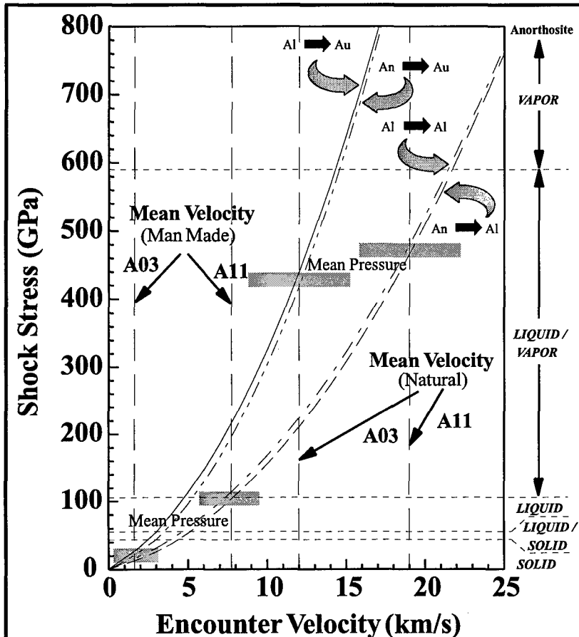
Figure 5. Shock pressures (refs. 28 and 29) of aluminum (Al) and anorthosite (An) projectiles impacting gold and aluminum targets at velocities up to 25 km/s. Also illustrated are the phase transitions of anorthosite upon release from a specific shock stress (ref. 30). Note the dramatically different stress regimes characterizing typical debris and cosmic-dust impacts. Also note that the typical cosmic-dust impact resides substantially into the vaporization regime for both aluminum and gold targets.
