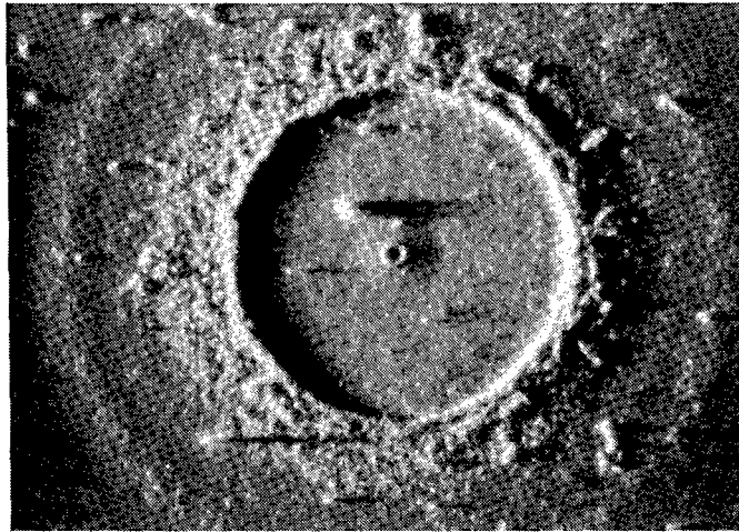
Figure 9: Impact crater from Bay C-12 showing fine powderiness of ring structure and paint surface. Crater diameter is 35 \mu\text{m} , total ring diameter is \sim 1.6 mm; magnified 40x.
