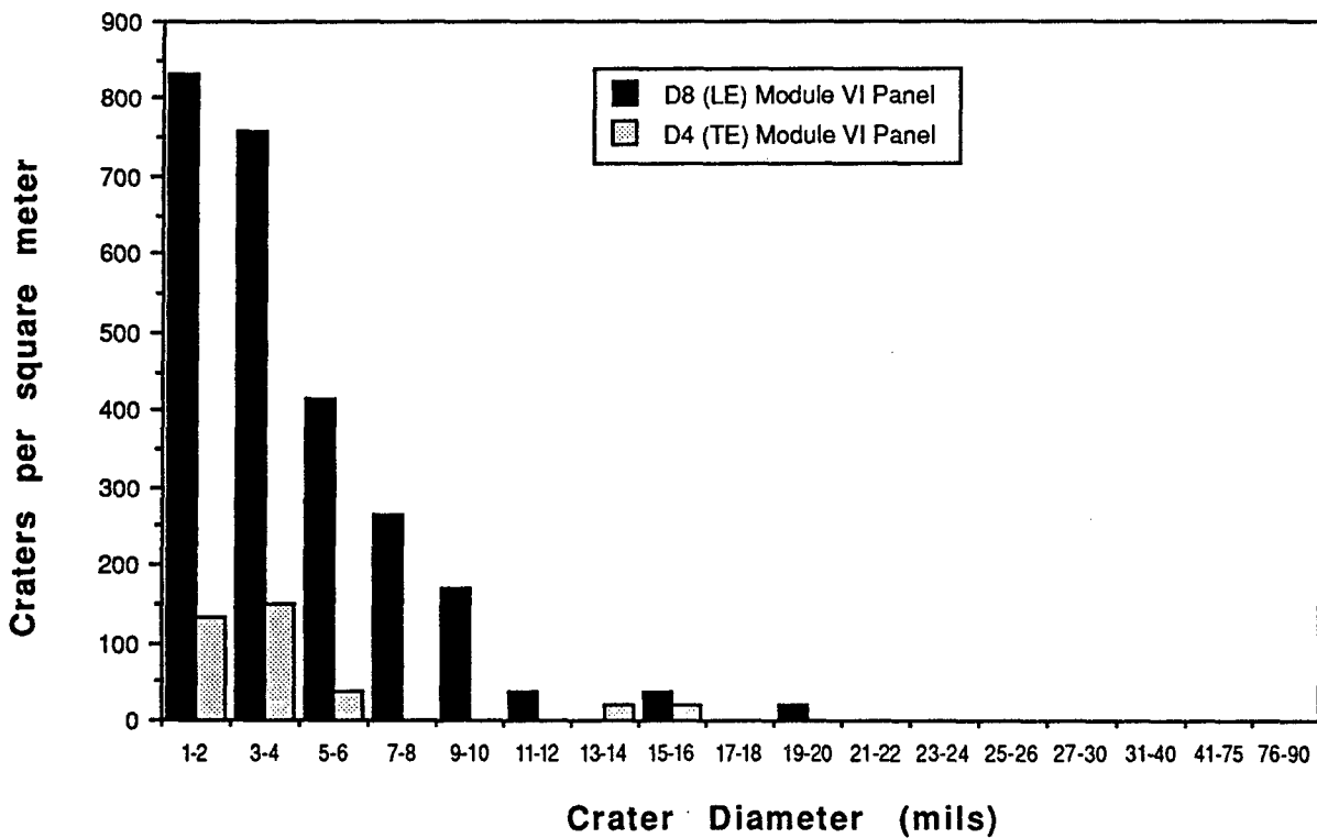
Figure V-13 Linear histograms for anodized surfaces.
