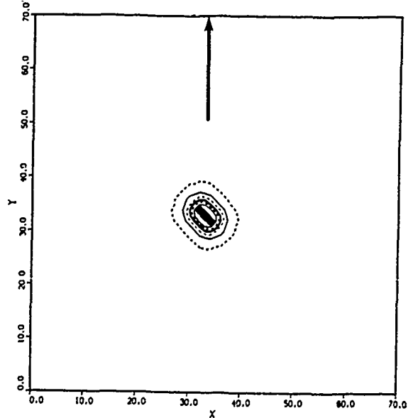
FIGURES 2.2:2-4. Elevation magnitude spectra, \sqrt{P(k_x, k_y)} .
