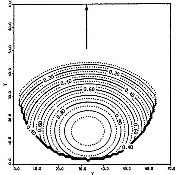
FIGURE 2.5:2. Map of COS(omega) to coordinates (beta,alpha).
