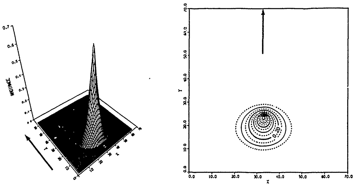
FIGURE 2.5:8. Map of reflected skydome radiance, L_r' , to coordinates ( \beta, \alpha ) for vertical polarization.
