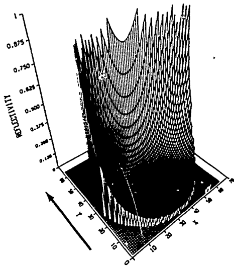
FIGURE 2.5:3. Map of Fresnel reflectivity, R(\omega) , to coordinates (\beta, \alpha) for horizontal polarization.
