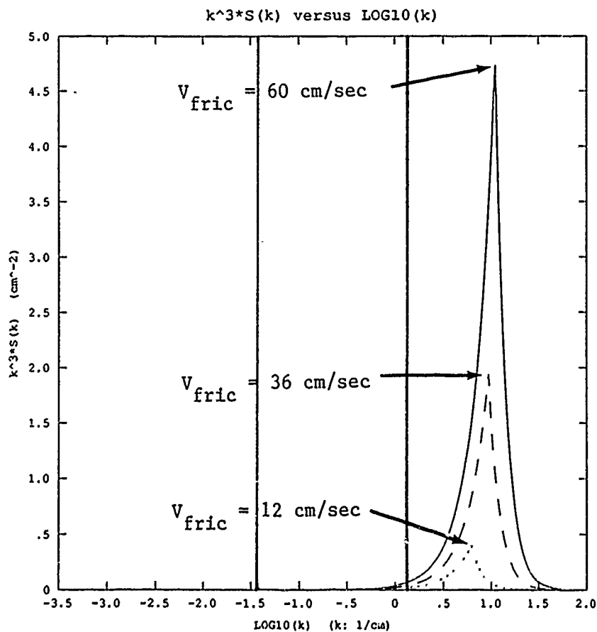
FIGURE 2.5:9. The 1D Pierson-Stacy curvature power spectrum k^3*S(k) versus LOG10(k) .
