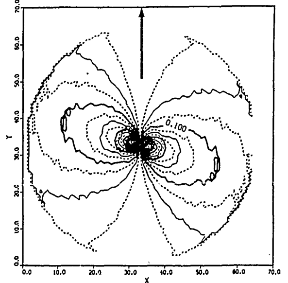
FIGURES 2.2:11-13. Y-components of slope magnitude spectra.
