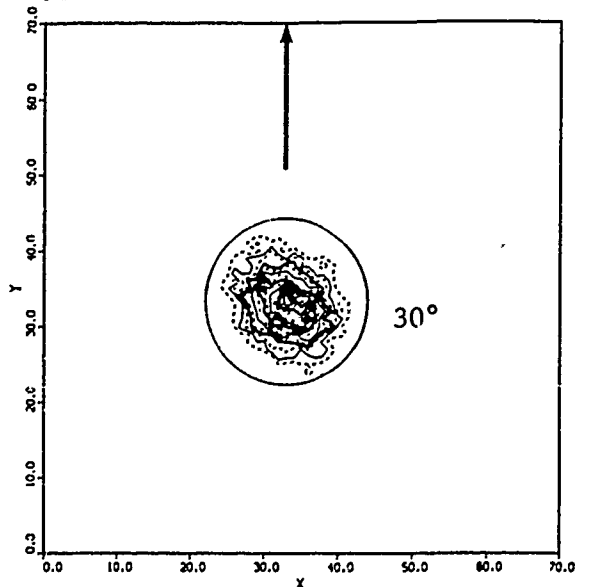
FIGURES 2.2:14-16. Sample slope probability distributions, \Pr(\beta, \alpha) .
