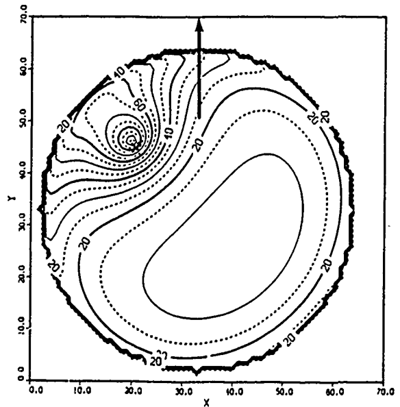
FIGURES 2.3:1-2. Synthetic skydome radiances distributions.
