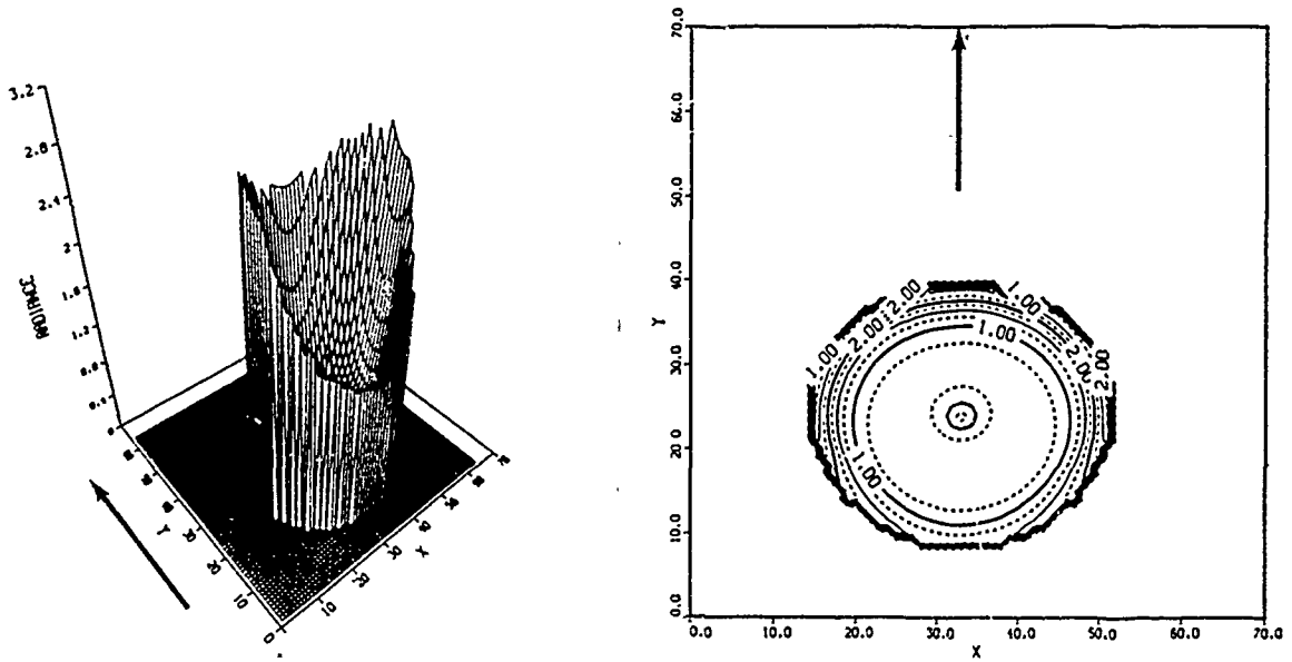
FIGURE 2.5:7. Map of reflected skydome radiance, L_r' , to coordinates ( \beta, \alpha ) for horizontal polarization.
