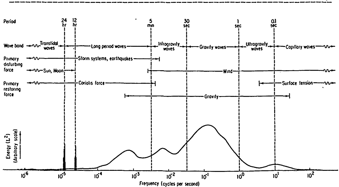
FIGURE 1.1:1. Schematic representation of the energy contained in the surface waves of the oceans - in fact, a guess at the power spectrum. (from Kinsman, 1965)
