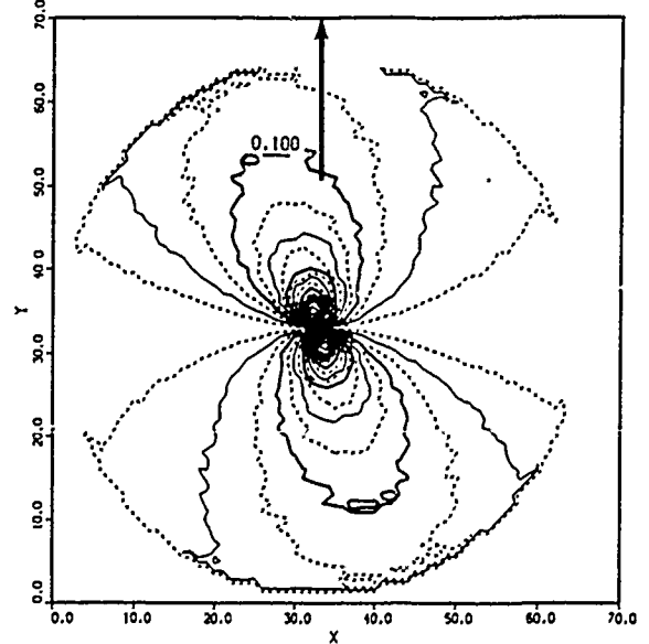
FIGURES 2.2:8-10. X-components of slope magnitude spectra.
