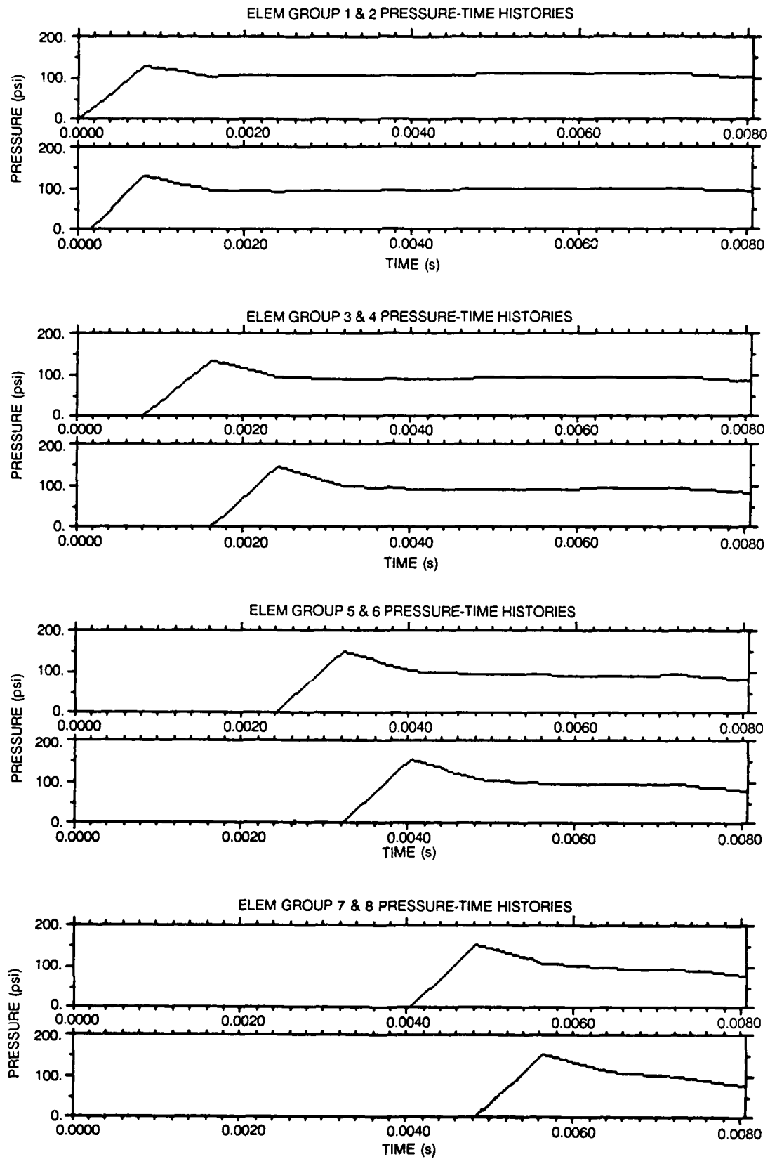
Figure 16. Pressure-time histories (0.000–0.008 s).
