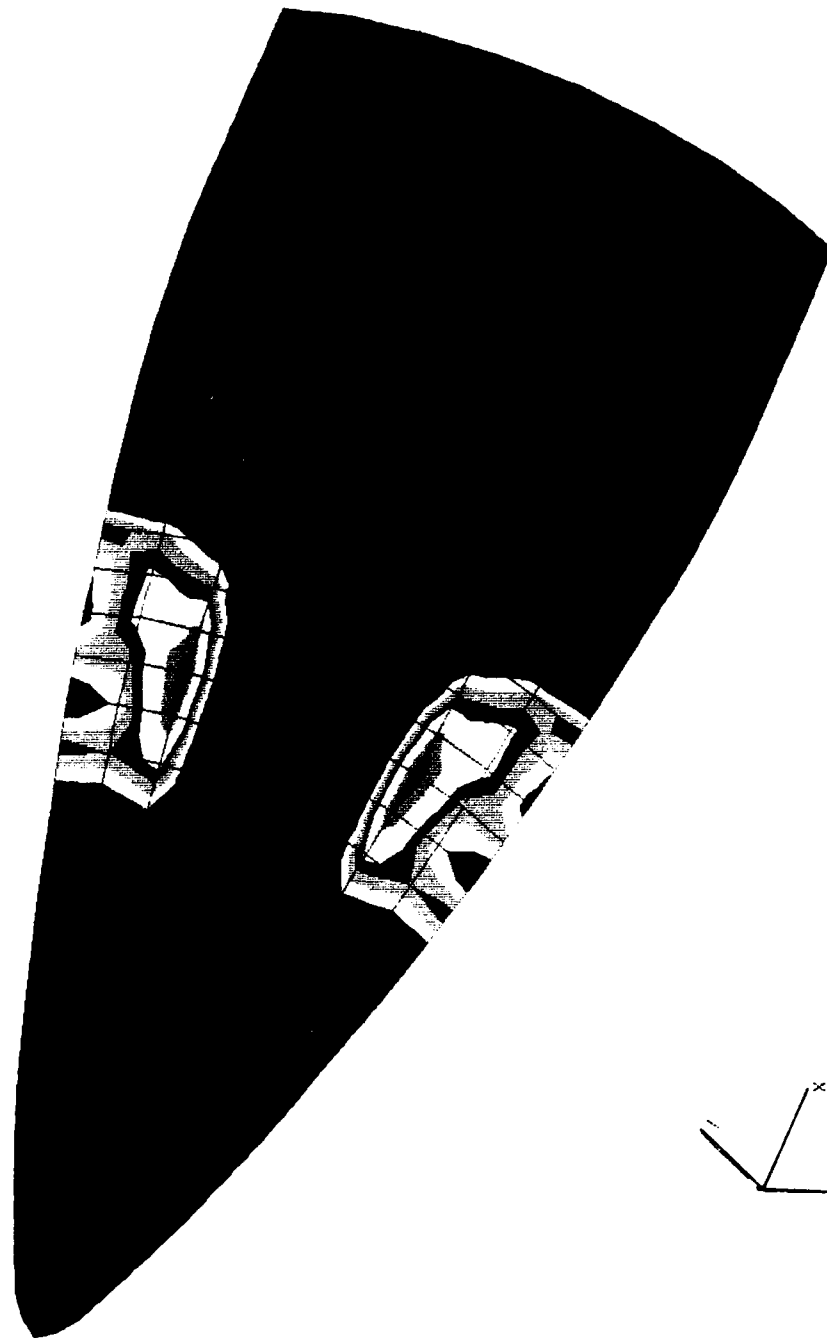
Figure 59. Inside shell surface third principal stresses at t = 1.5624 ms (step 6).
