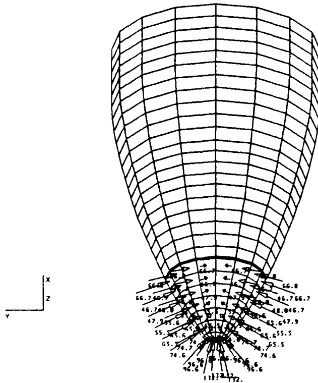
Figure 38. Pressure distribution on vertical water-entry nosecap at t = 2.3226 ms (step 8).
