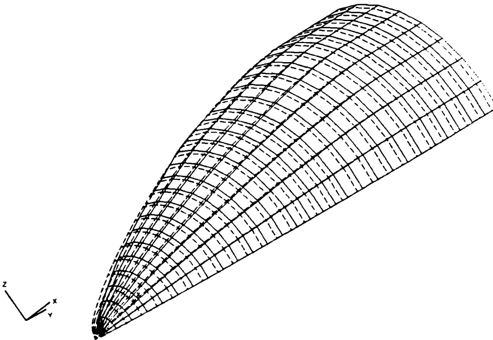
Figure 45. Deformed shape of shell at t = 0.8440 ms (step 4).
