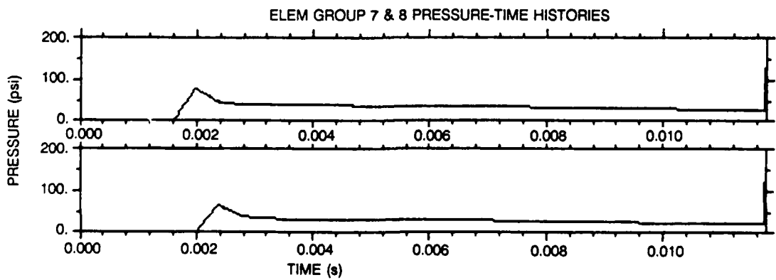
Figure 41. Pressure-time histories (0.000-0.010 s).
