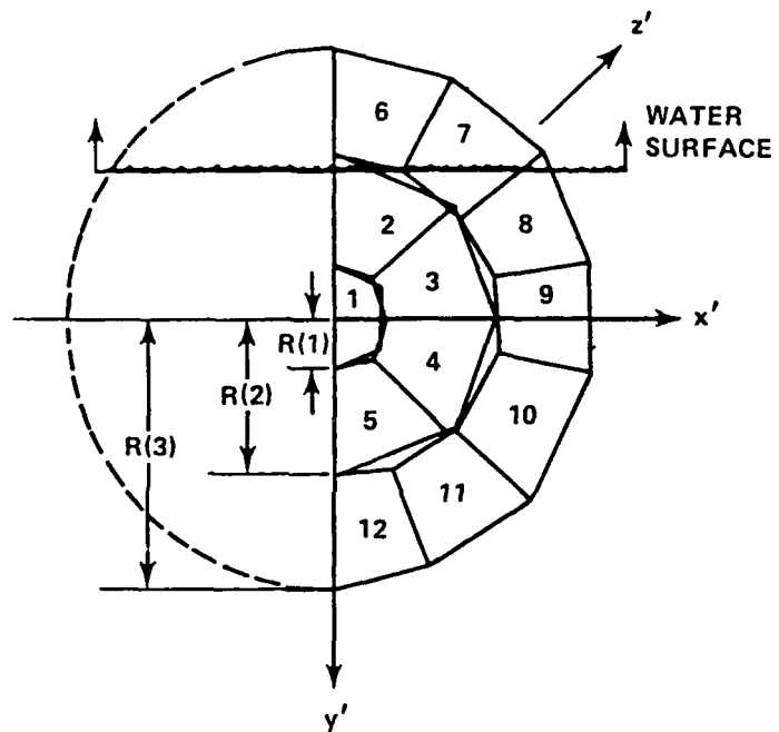
FIG. 6-4 GRID OF A CIRCULAR PLATE
