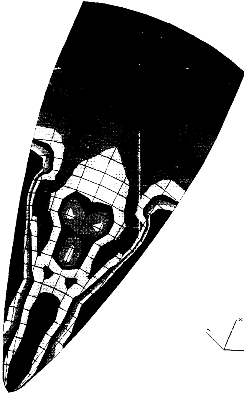
Figure 55. Inside shell surface first principal stresses at t = 3.1128 ms (step 10).
