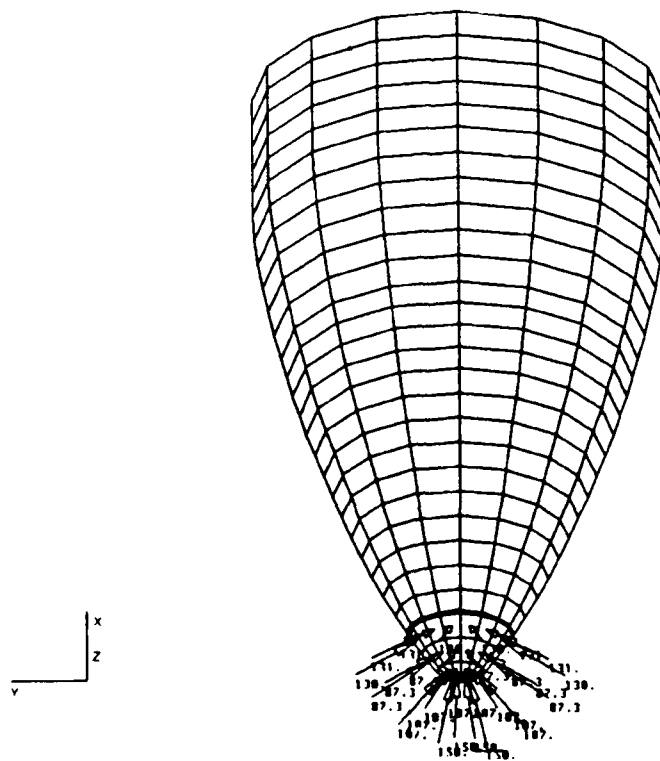
Figure 36. Pressure distribution on vertical water-entry nosecap at t = 0.8440 ms (step 4).
