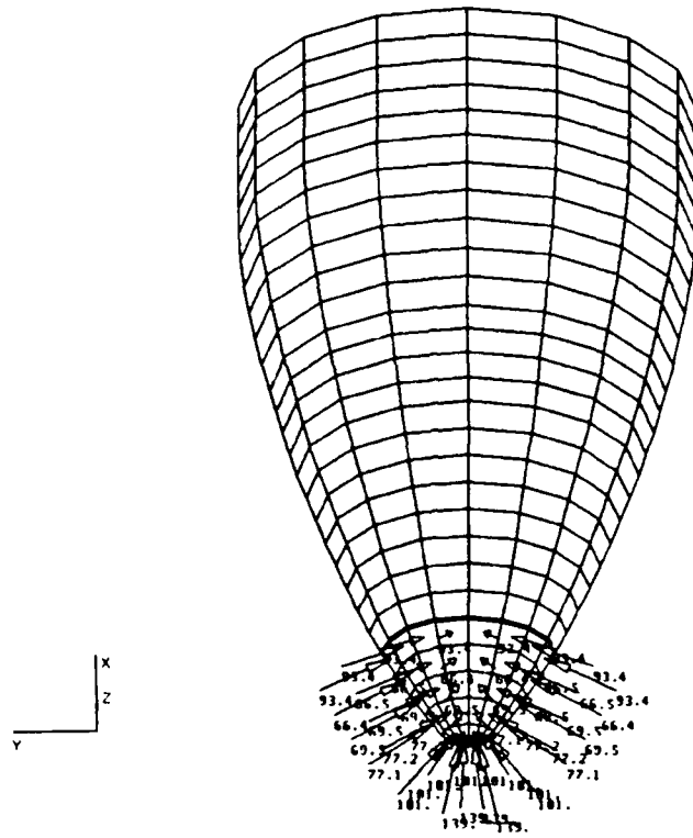
Figure 37. Pressure distribution on vertical water-entry nosecap at t = 1.5624 ms (step 6).
