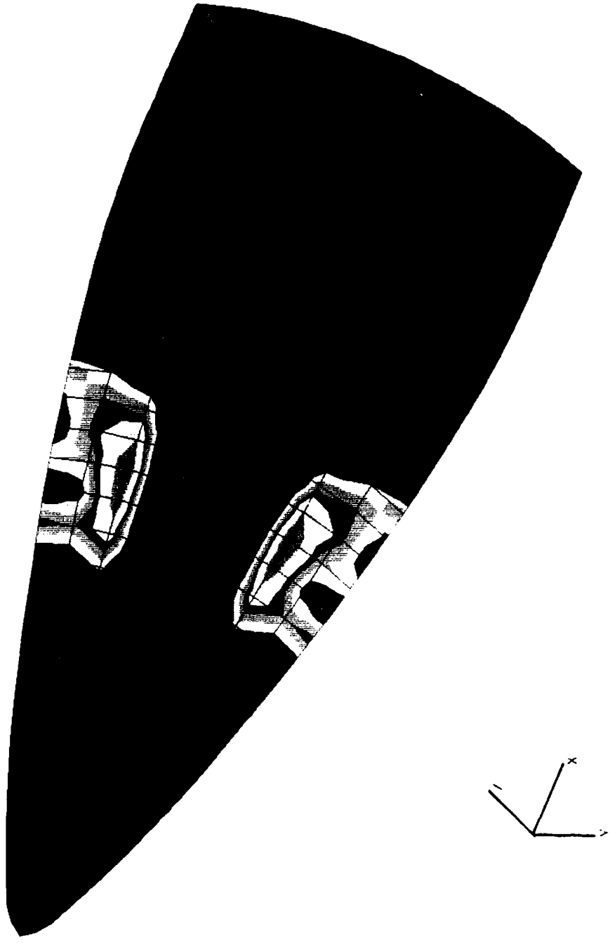
Figure 60. Inside shell surface third principal stresses at t = 3.1128 ms (step 10).
