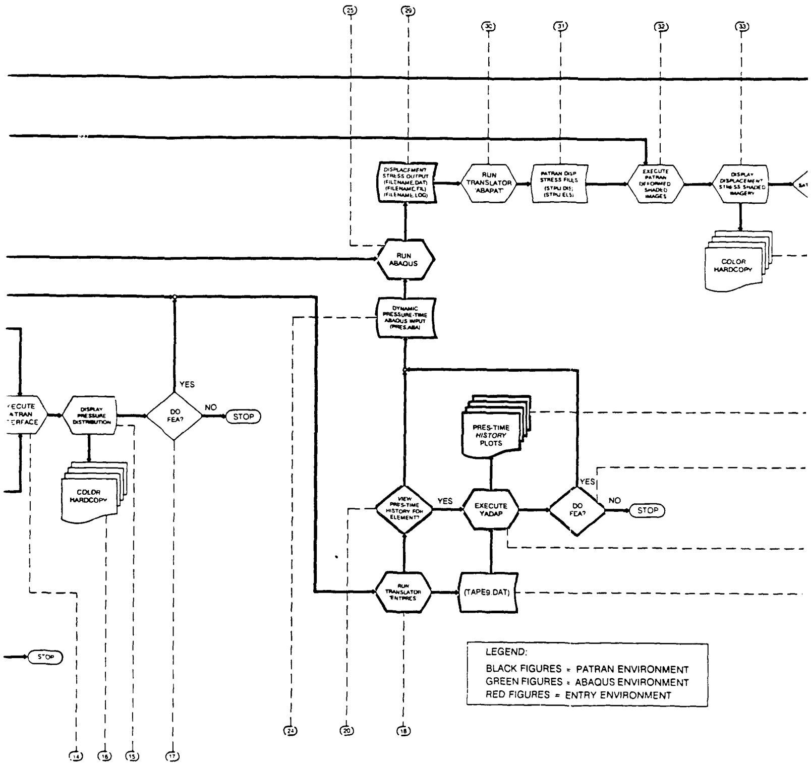
Flow chart of frangible nose cap analysis at water entry.
