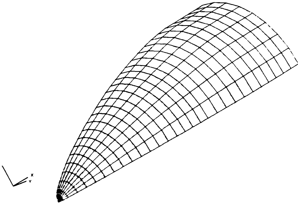
Figure 44. Deformed shape of shell at t = 0.1770 ms (step 2).
