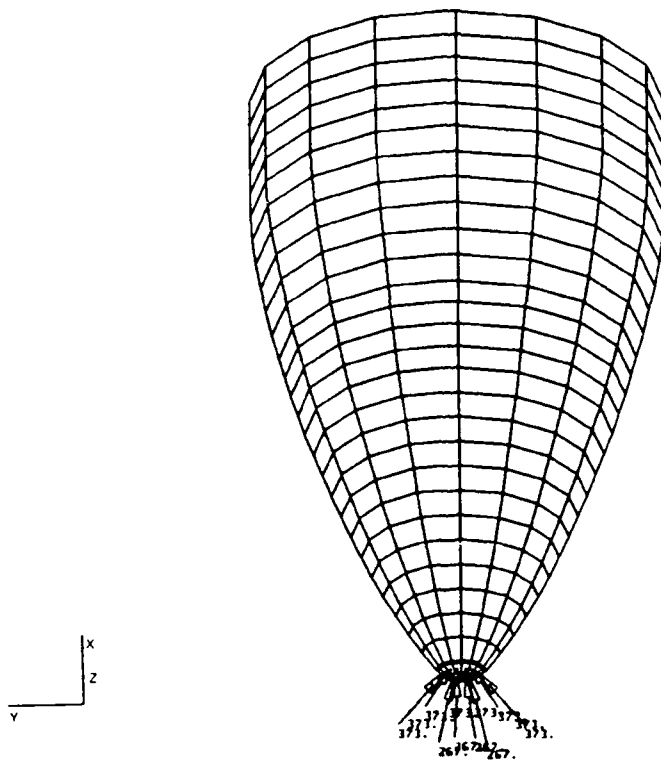
Figure 35. Pressure distribution on vertical water-entry nosecap at t = 0.1770 ms (step 2).
