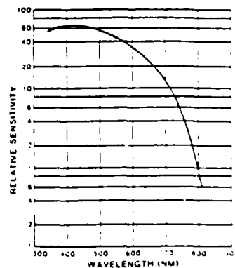
Typical spectral response of S20 photocathode used in standard Optron optical heads extends from ultraviolet to near infrared. Standard photographic filters may be used to eliminate background illumination or enhance target contrast.
