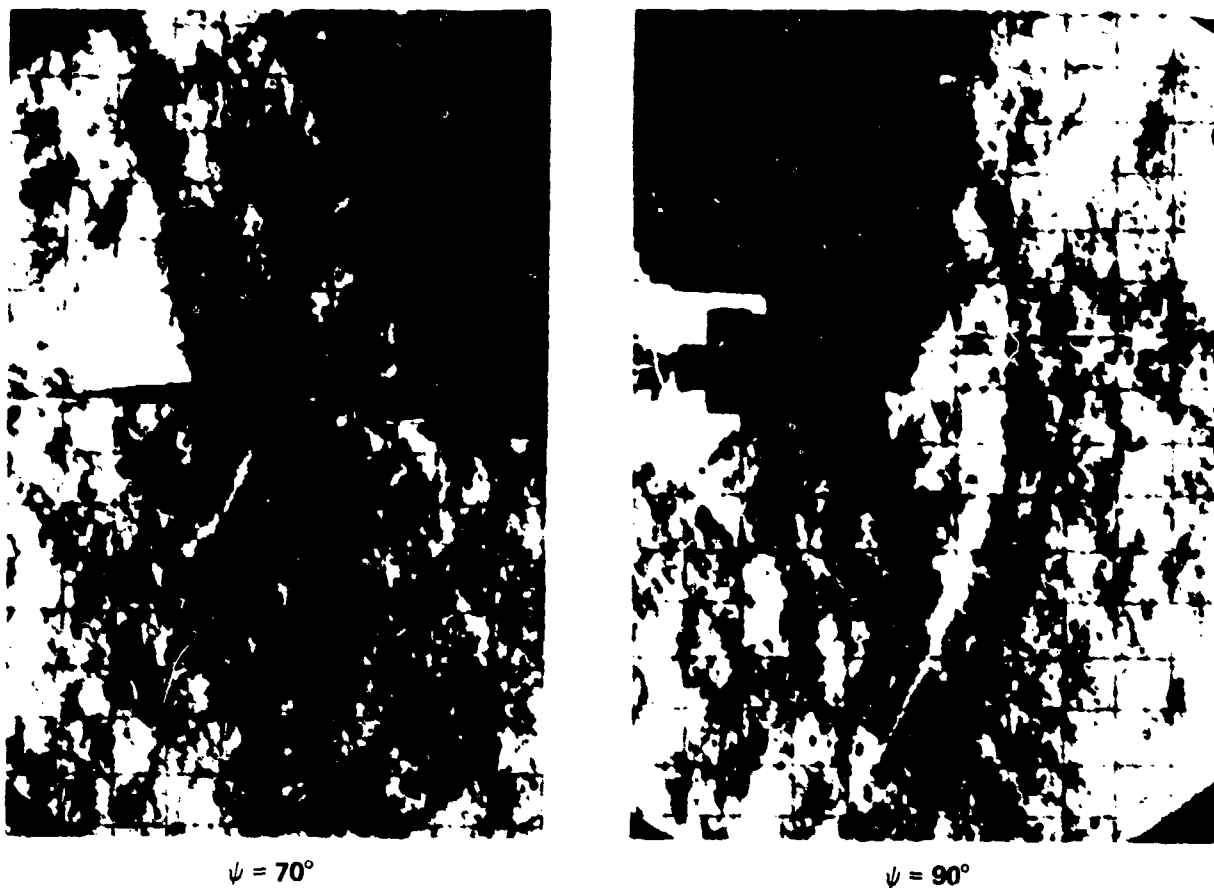
Figure 76.- Shock propagation from blade-vortex interaction.
