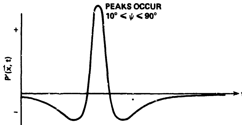
Figure 11.- Acoustic pressure signature of blade-vortex interaction.
