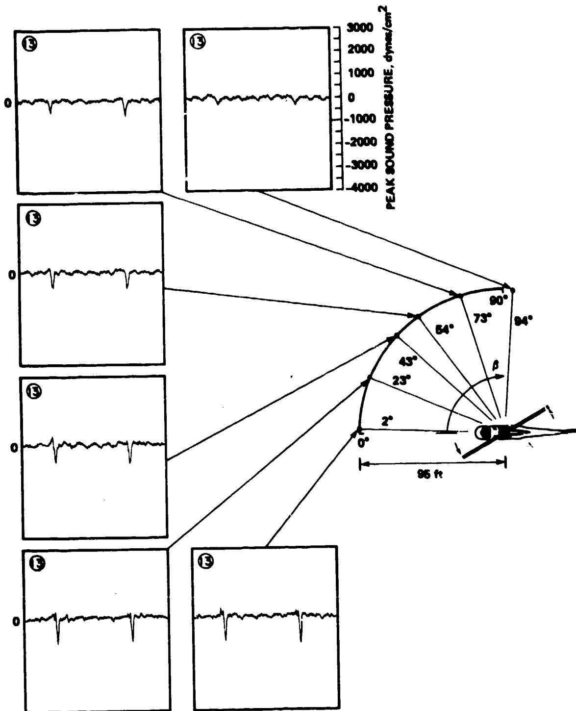
Figure 19.- UH-1H lateral acoustic directivity at 80 knots IAS and 400 f./min rate of descent ( \alpha = 3^\circ ).
