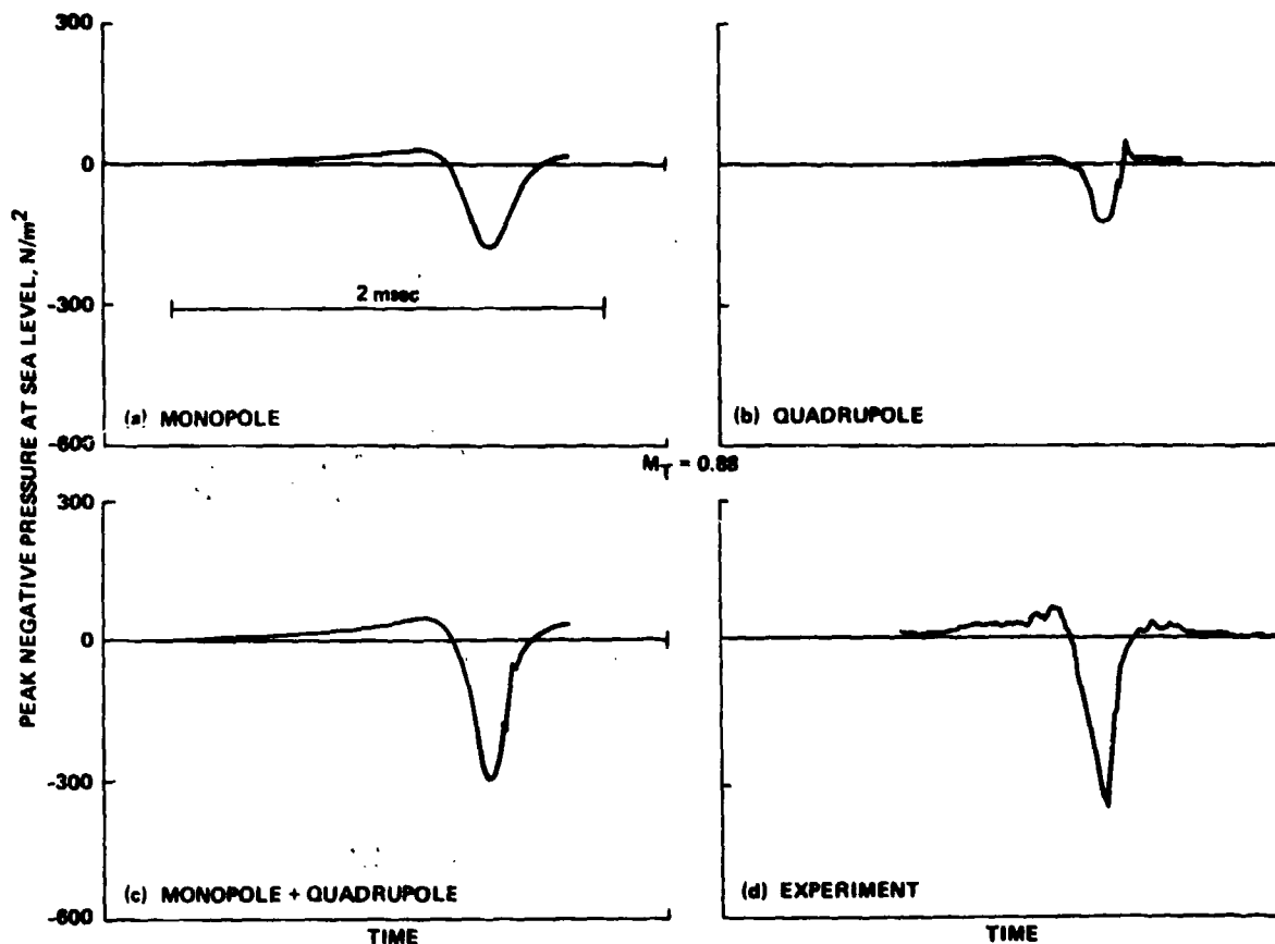
Figure 62.- Theory-experiment comparison, M_T = 0.88 .
