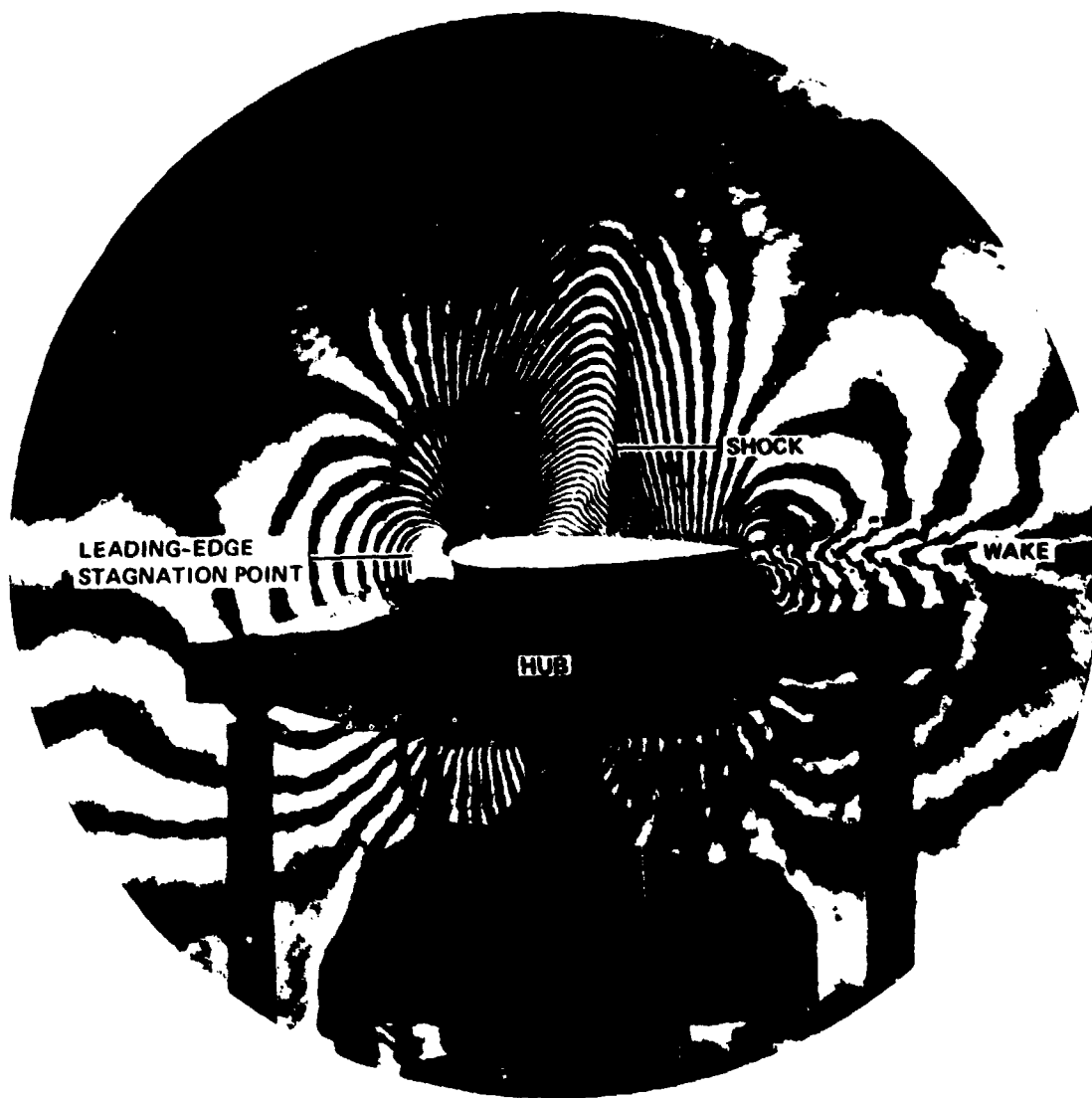
Figure 55.- Interferogram recorded at 180° (chordwise view).
