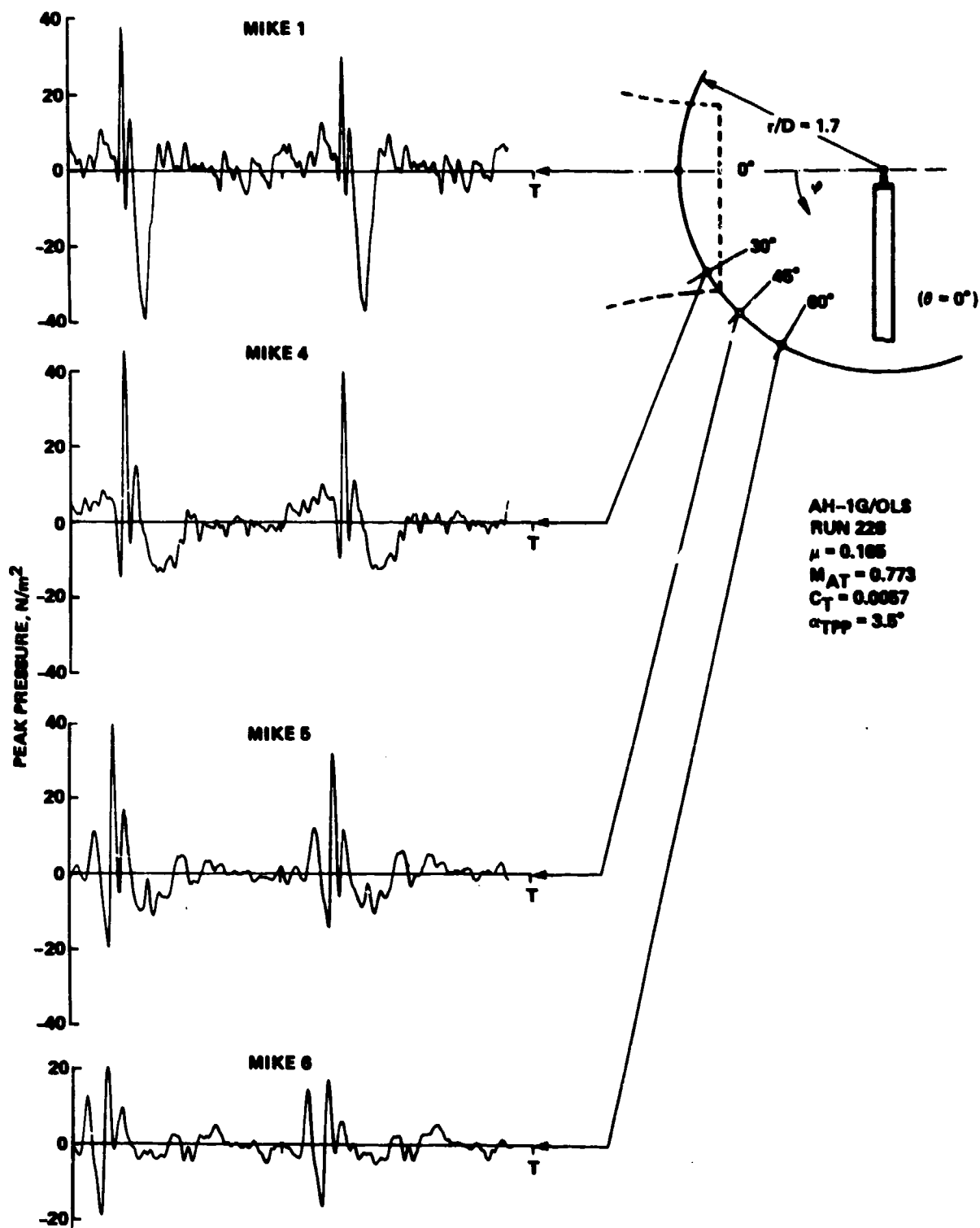
Figure 71.- Longitudinal directivity of blade-vortex interaction noise (averaged data).
