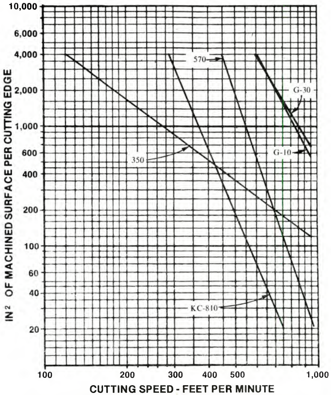
Figure 82: Tool-Life Lines of Listed Cutting Materials on AISI 1340 Steel at 321/340 Brinell Hardness.
