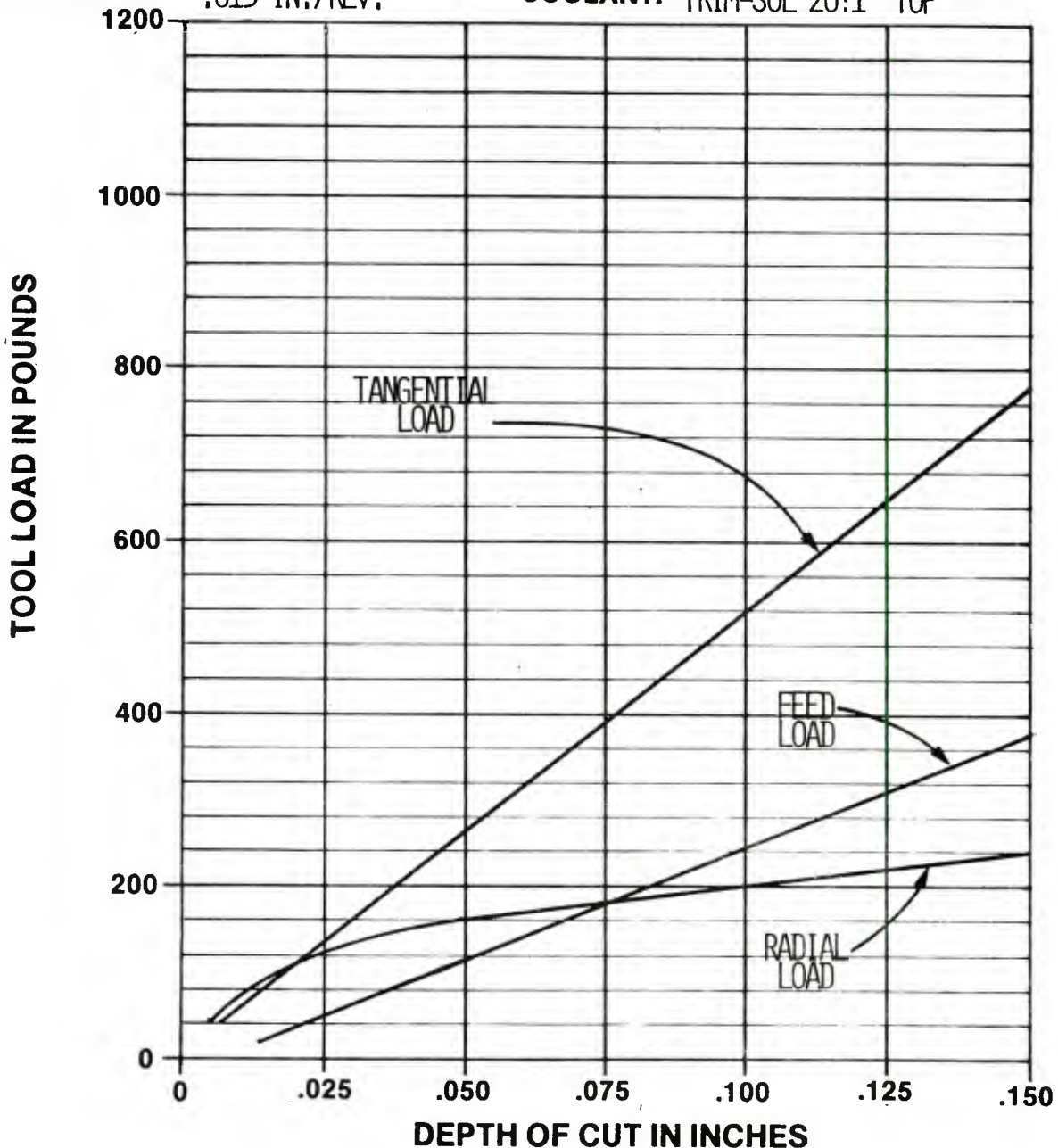
FIGURE 99 : TOOL LOAD CHART
