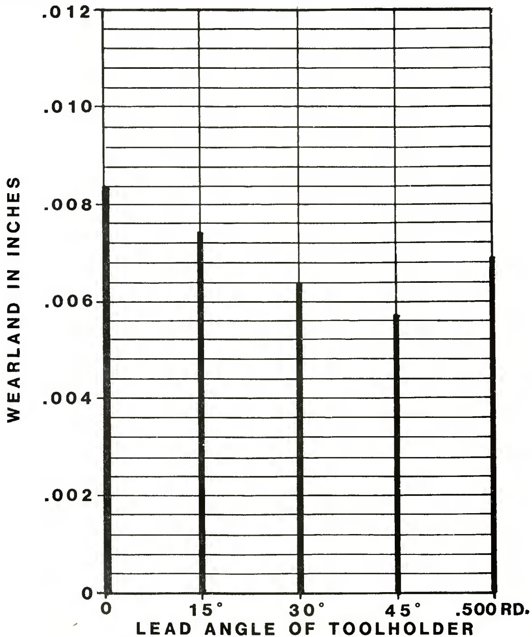
FIGURE 41 WEARLAND FOR LISTED CUTTING MATERIAL
