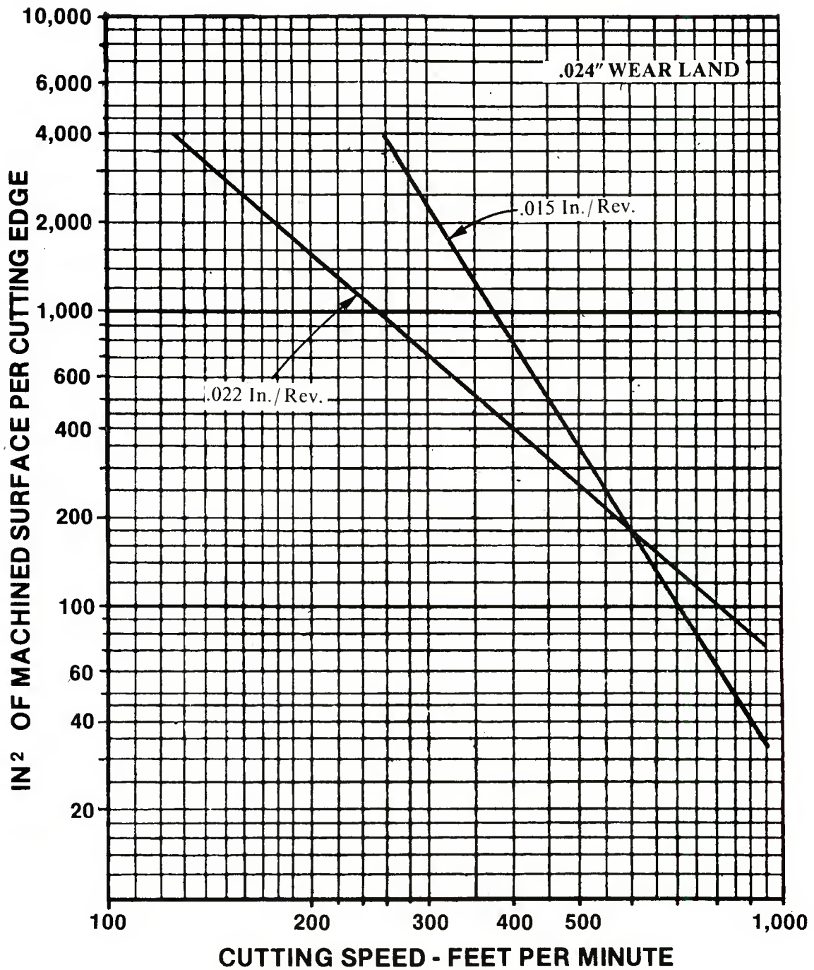
Figure 57: Tool-Life Lines of Carbobloy Grade 350 on HF-1 Steel at 269/277 Brinell Hardness for Listed Feed-Rates.
