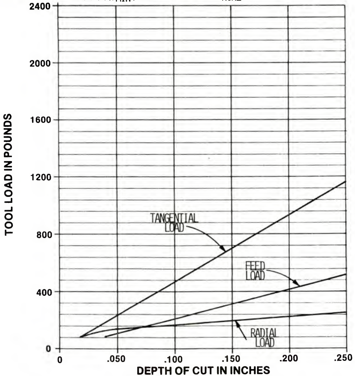
Figure 36: TOOL LOAD CHART
