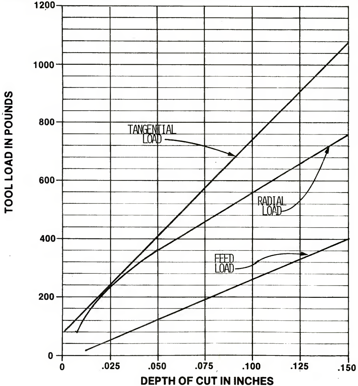
FIGURE 118 : TOOL LOAD CHART
