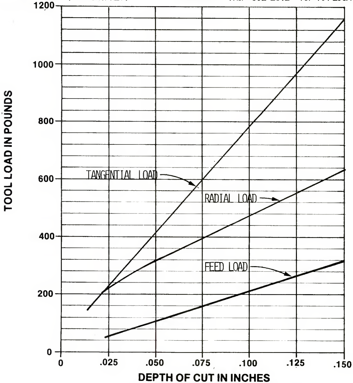
FIGURE 155 : TOOL LOAD CHART
