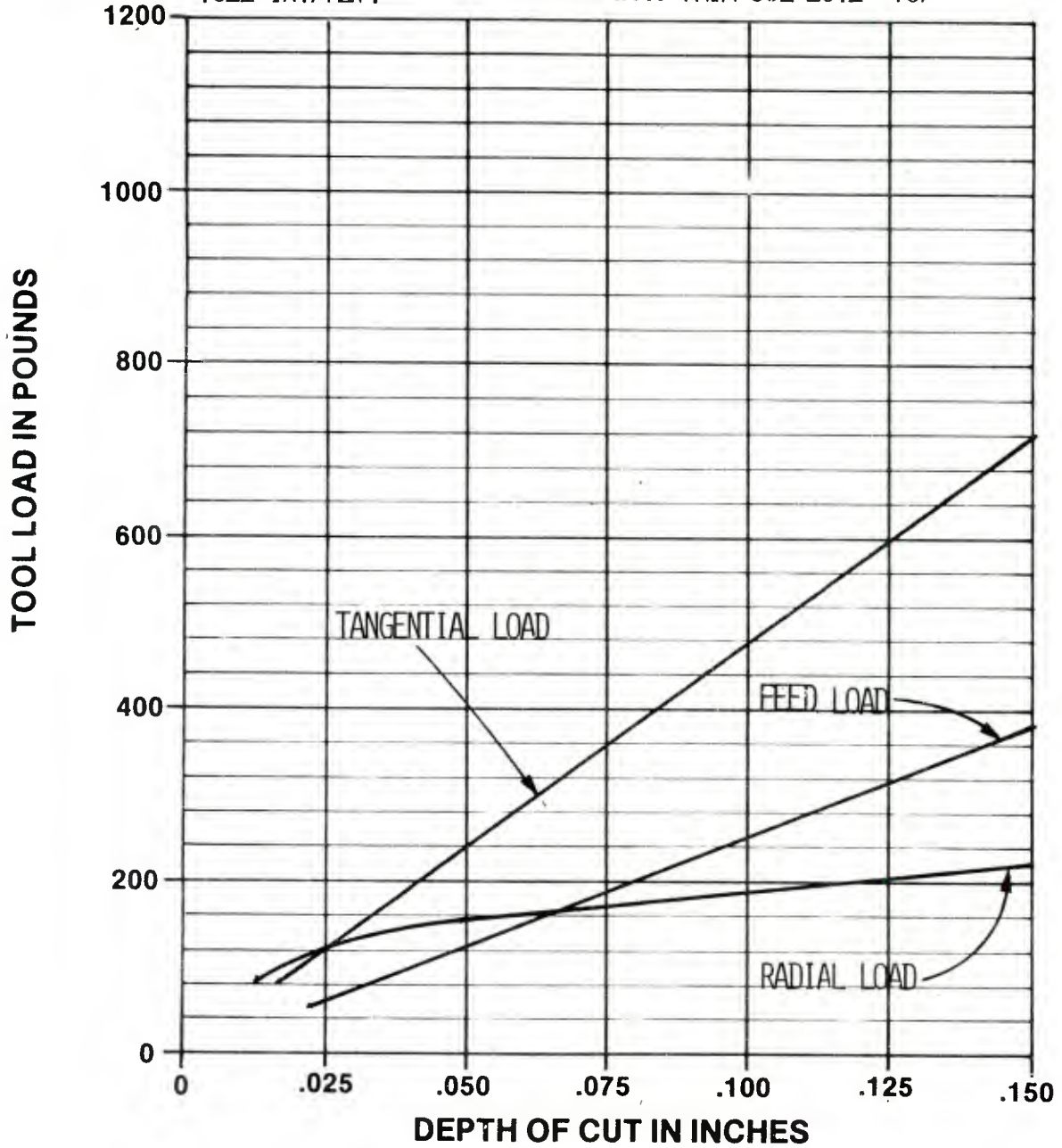
FIGURE 148 : TOOL LOAD CHART
