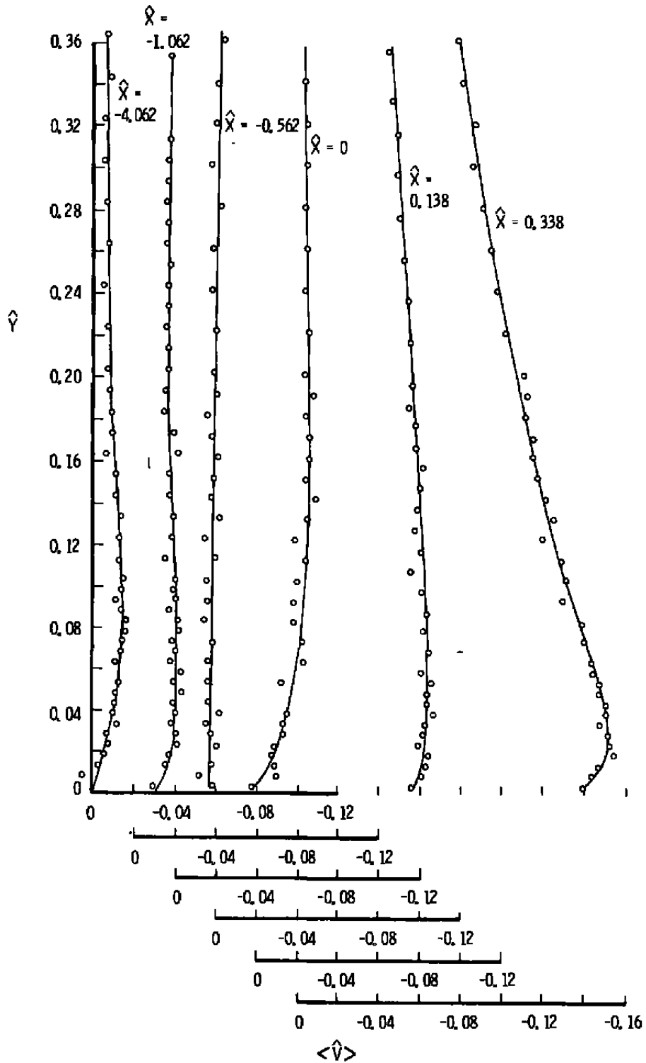
Figure 17. Mean radial velocity component, separated-flow model.
