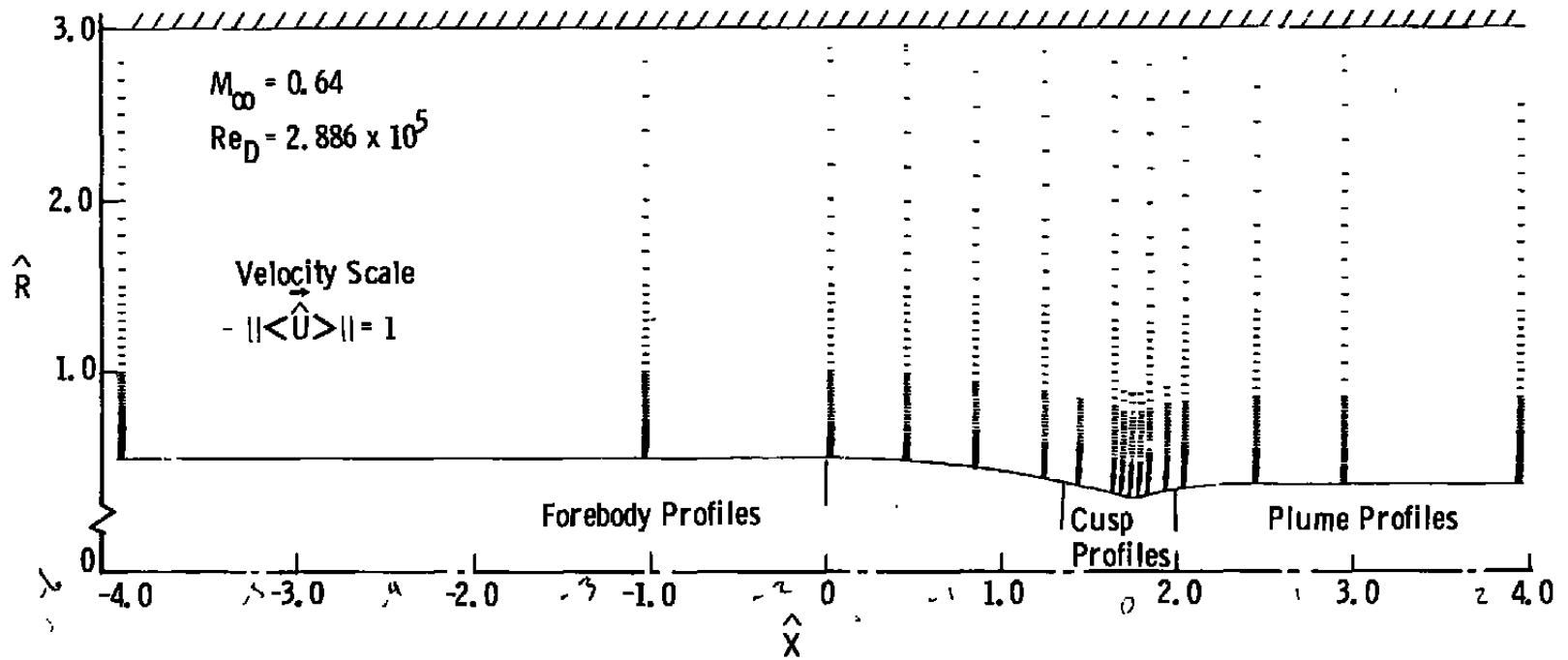
Figure 7. Mean velocity vectors, attached-flow model.
