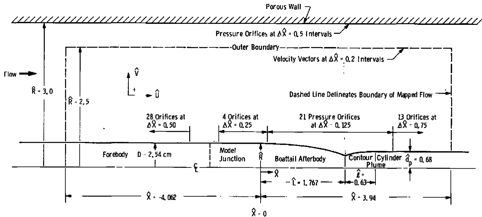
Figure 3. Attached-flow model.
