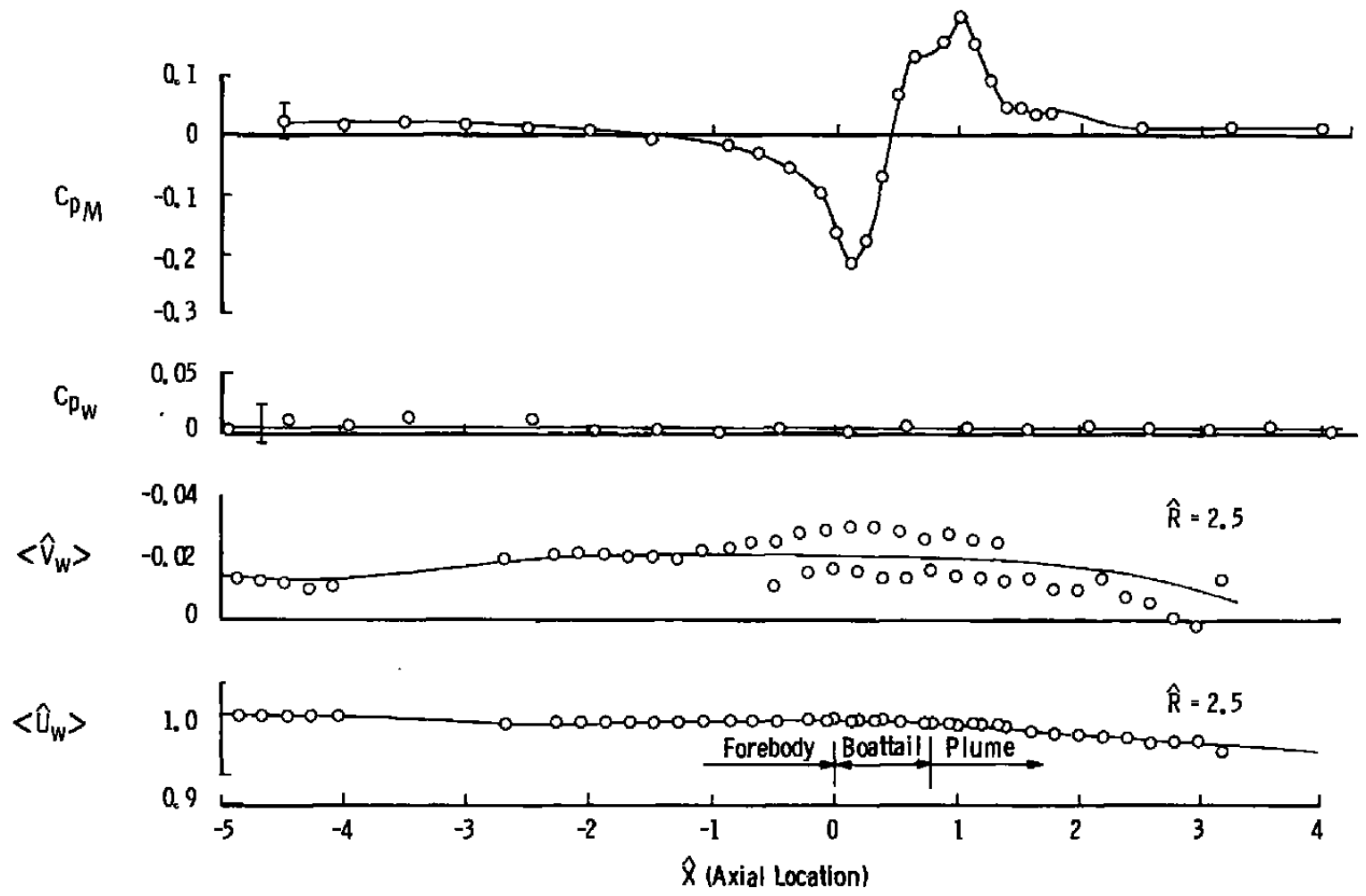
Figure 20. Boundary conditions for separated flow field.
