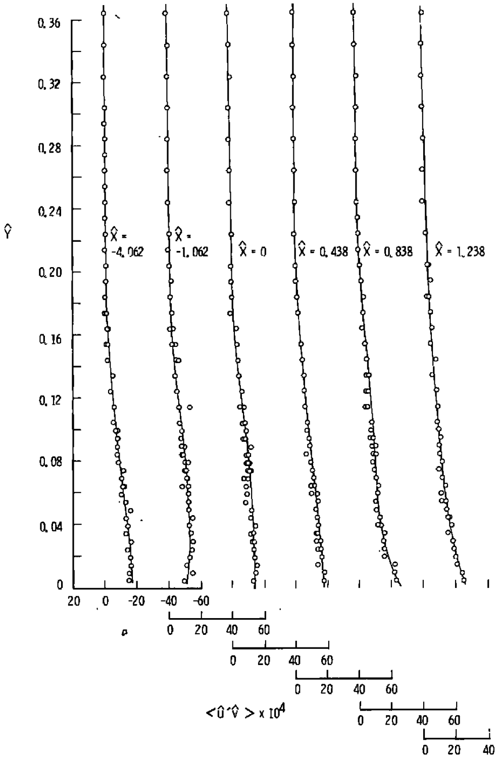
Figure 12. Specific Reynolds shear, attached-flow model.
