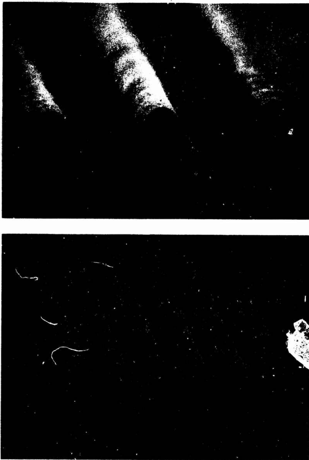
Fig. II.4 Scanning electron microscope photograph of the gold mask on the GaAs substrate used in the fabrication of the (a) dual directional coupler, (b) multichannel directional coupler. The remains of the photoresist can be seen on top of the gold stripes.
