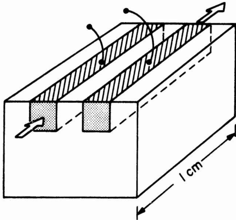
Fig. II.17 Example of a directional coupler modulator.
