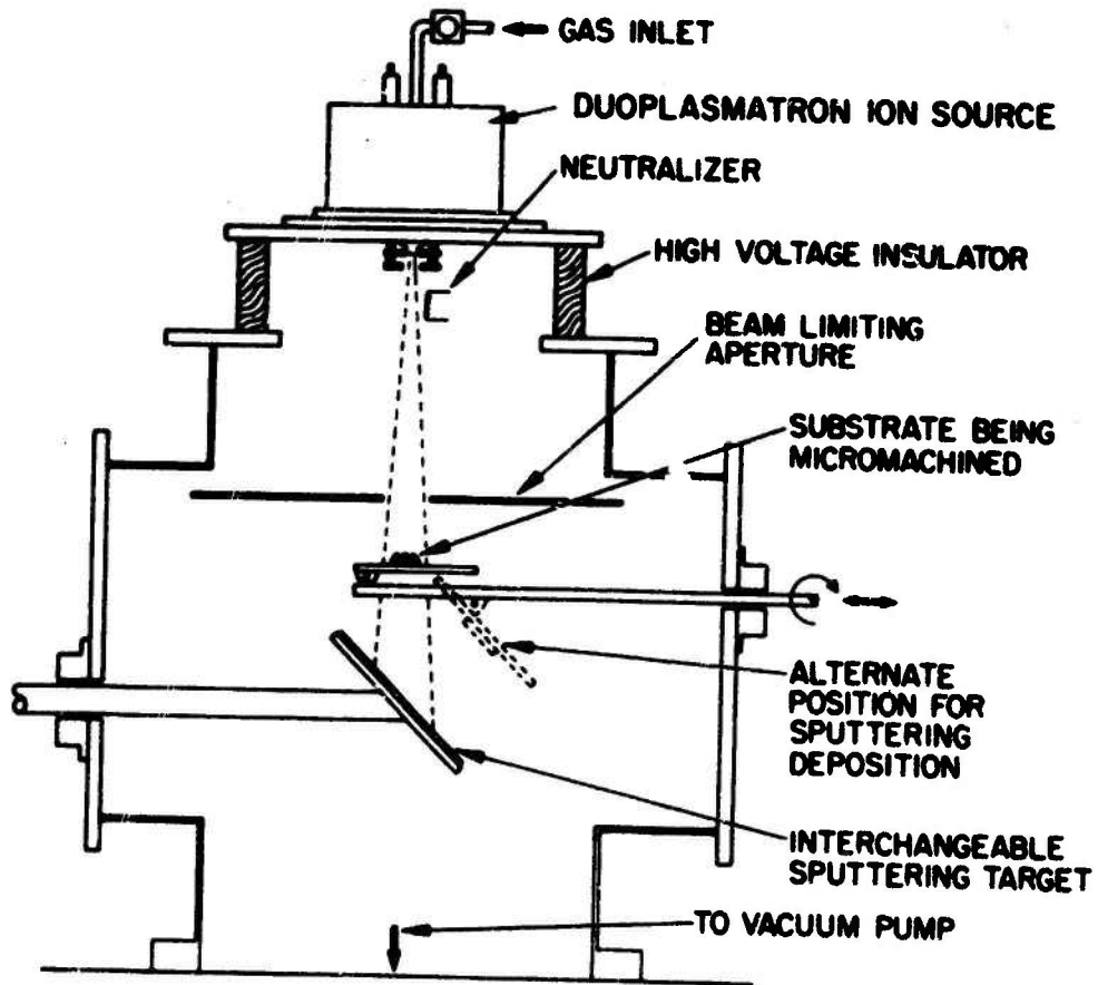
Fig.IV.1 Schematic diagram of the duoplasmatron ion beam sputtering system.
