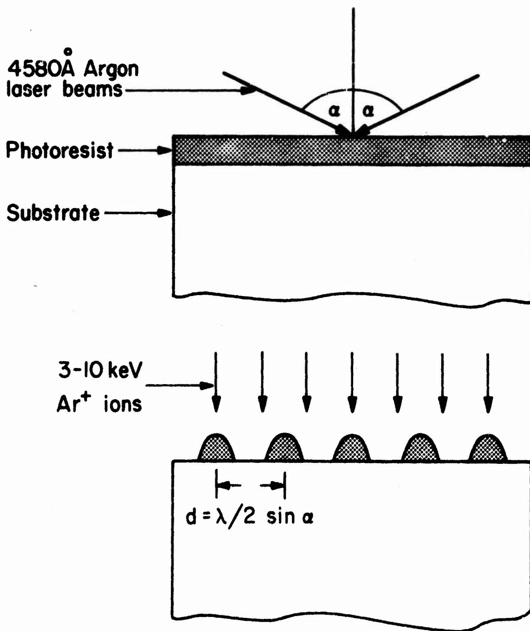
Fig IV.2 (a) Holographic exposure of photoresist. (b) Ion machining of photoresist after development.
