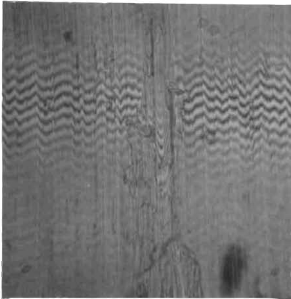
Figure 113. Test Model N_f , Poppet, 0.0065- x 0.0065-Inch Interference Photo Showing Plastic Deformation at Area of Seat Land OD Contact, White Light
