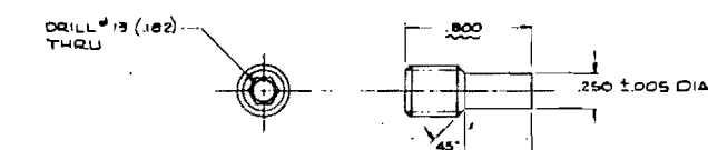
(60) LOCK SCREW
