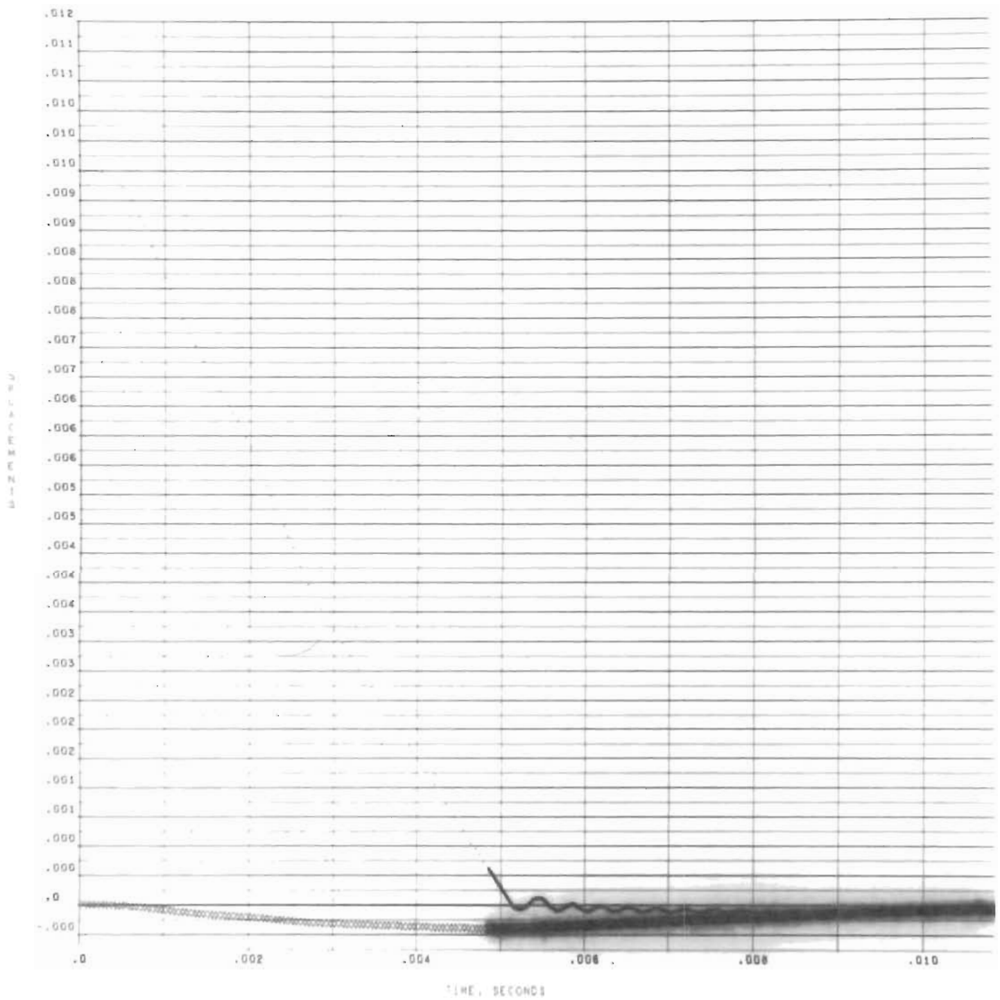
Figure 54. Computed Poppet (·) and Body (x) Displacements, 1.77 in./sec Impact Velocity, PS = 287 psia, D\phi D = 0.0217 in.
