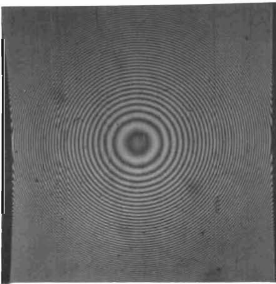
Figure 241. Test Model A S , Seat, 0.033- x 0.033-Inch Interference Photo Showing Fretting Pits
