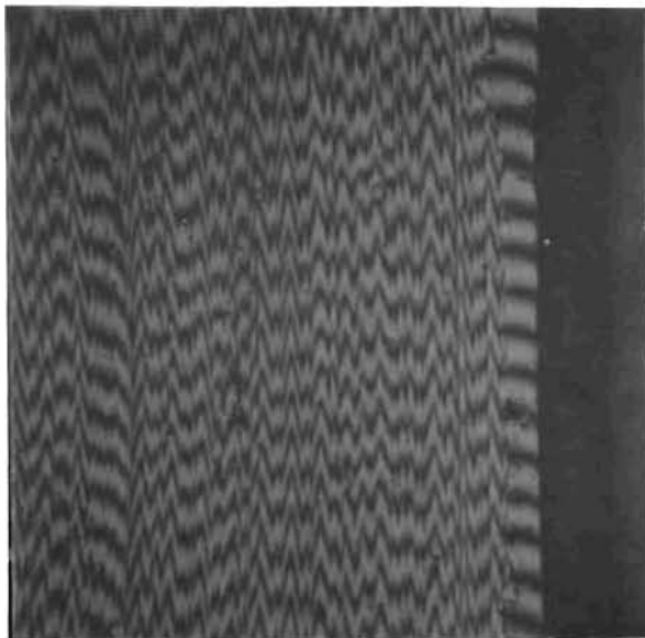
Figure 119. Test Model S_f , Seat, 0.0065- x 0.0065-Inch Interference Photo Showing OD Deformation
