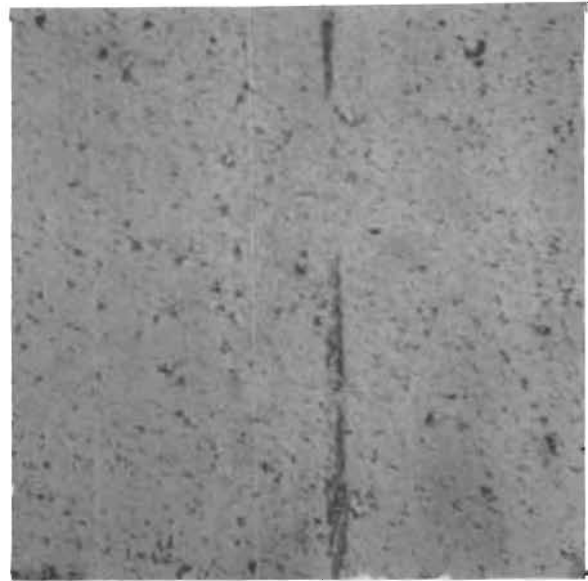
Figure 118. Test Model S_f and R_f , Poppet, 0.0065- x 0.0065-Inch Plain Photo Showing Metal Transfer
