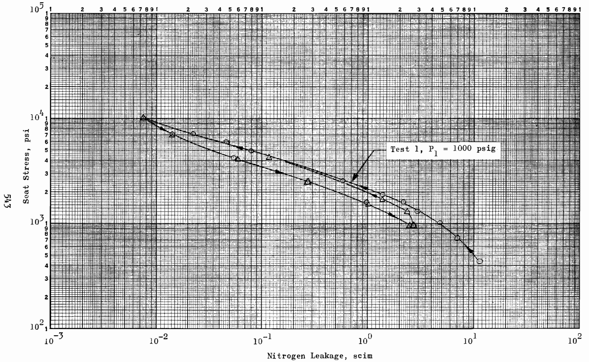
Figure 439. Stress-Leakage Data for Test Model D_s , Test 1
