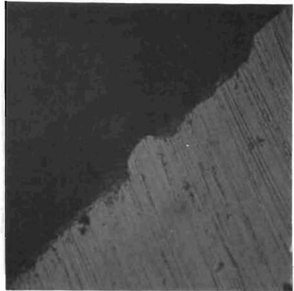
Figure 146. Test Model G_f , Seat, 0.0065- x 0.0065-Inch Plain Photo Showing Corner Fracture Damage (OD)
