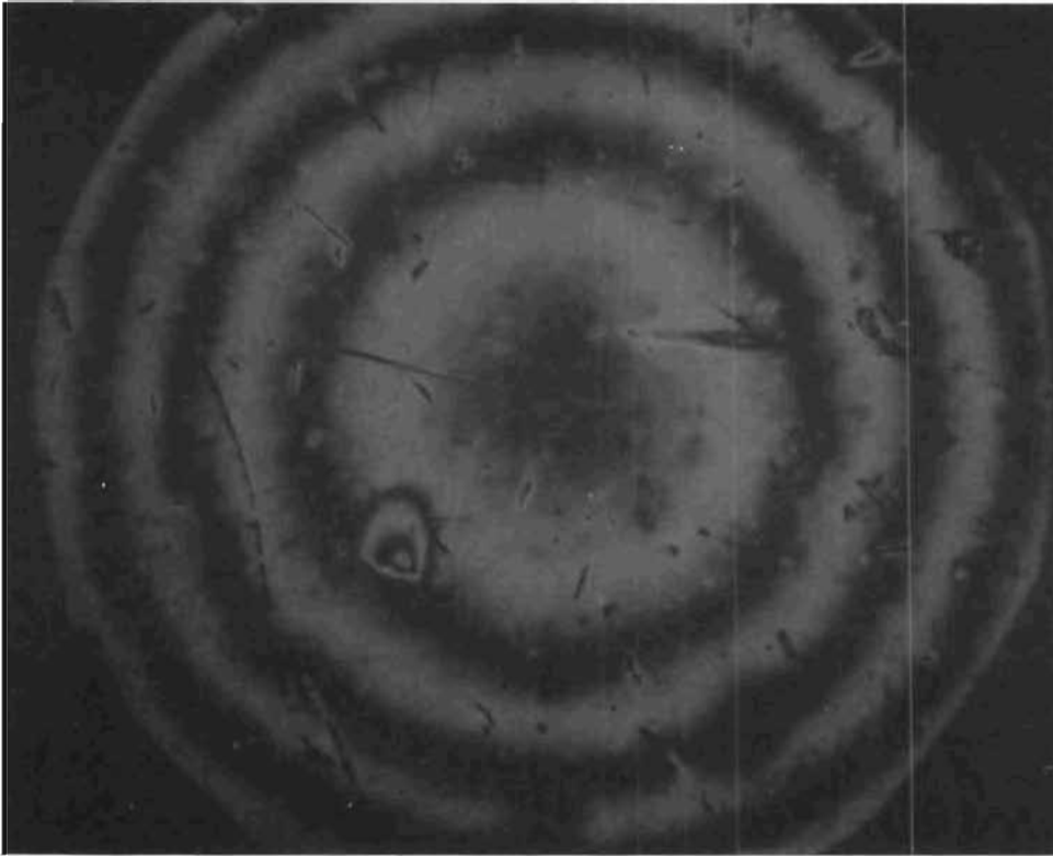
Figure 240. Test Model A S , Poppet, 0.0089- x 0.0110-Inch Interference Photo at \theta = 35 Degrees
