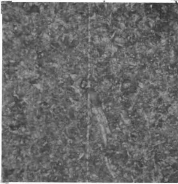
Figure 129. Test Model D, Poppet, 0.0065- x 0.0065-Inch Plain Photo Showing 0.0001-Inch Radius Proficorder Stylus Scratches
