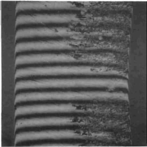
Figure 151. Test Model G f1 , Seat, 0.033- x 0.033-Inch Interference Photo Showing Corrosion Fretting Before Wiping
