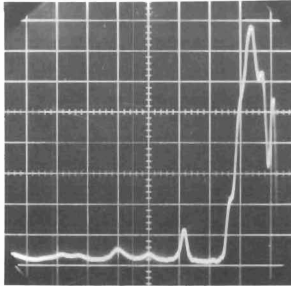
Figure 481. Test Model X_f , Piezo- electric Load Cell, \sim 7.7 in./sec Impact Velocity, PS = 25 psig (150 lb/div.; 0.0001 sec/div.)
