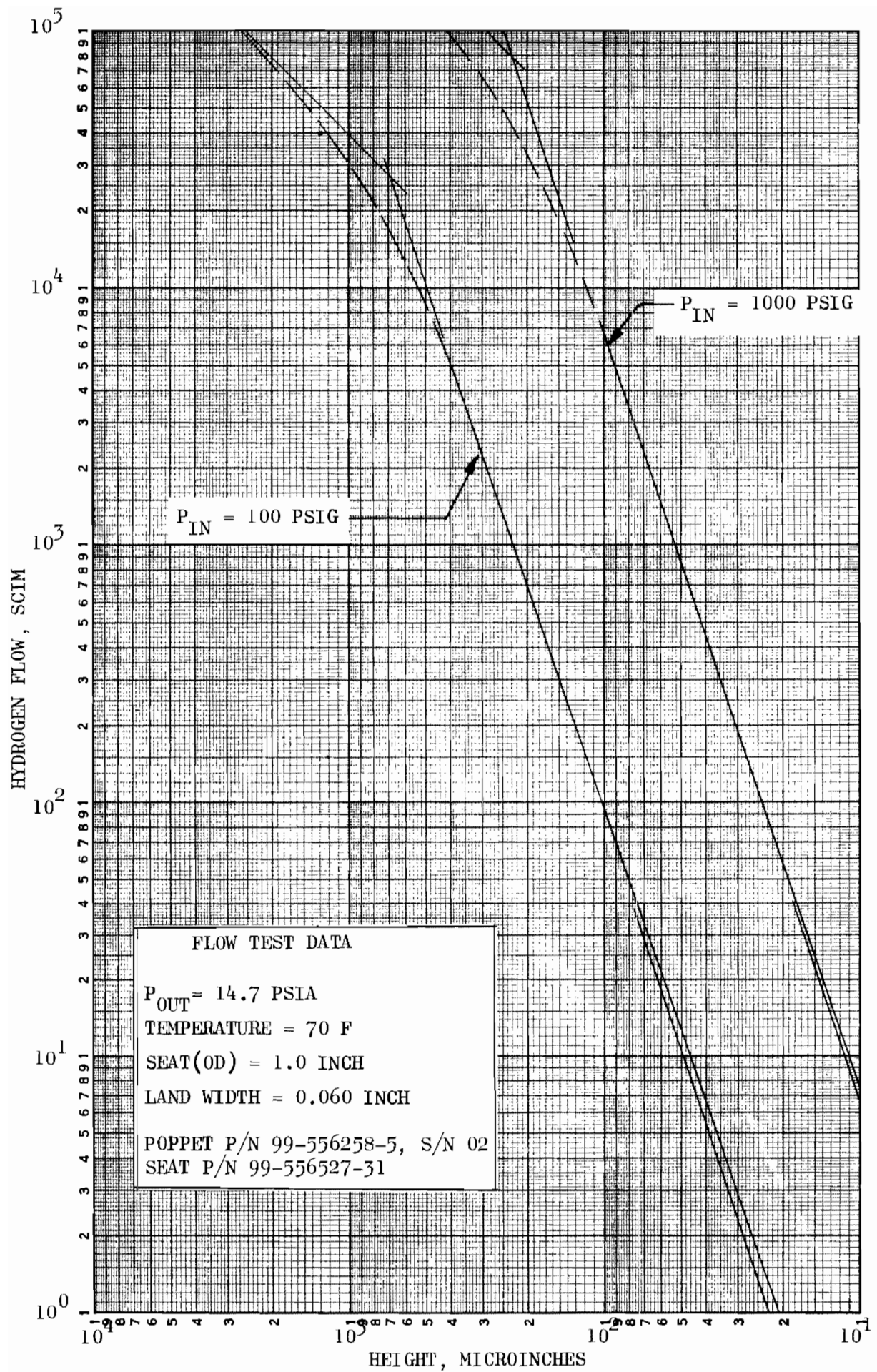
Figure 388. Hydrogen Flow Data, Part 1
