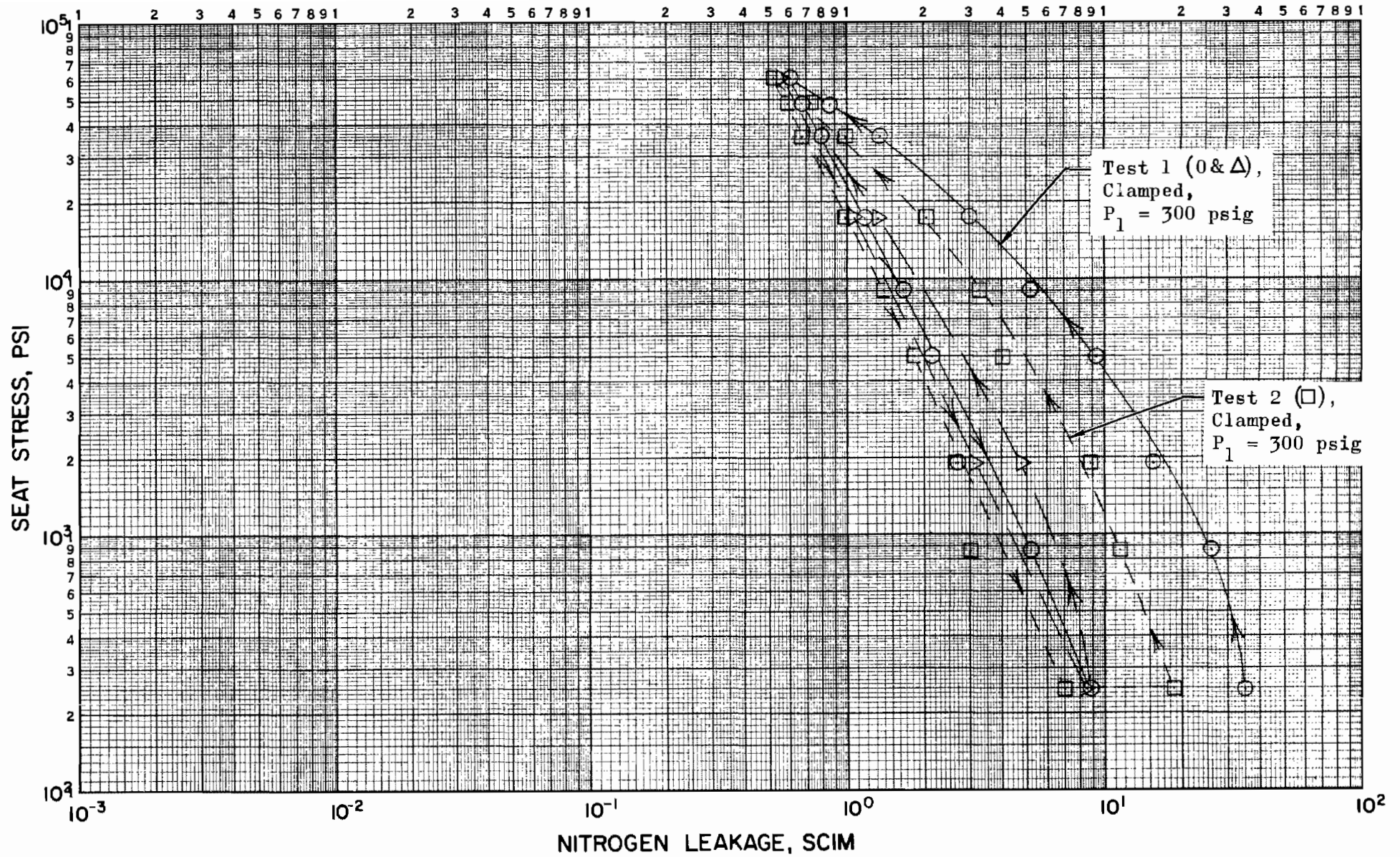
Figure 402. Stress-Leakage Data for Test Model D, Tests 1 and 2
