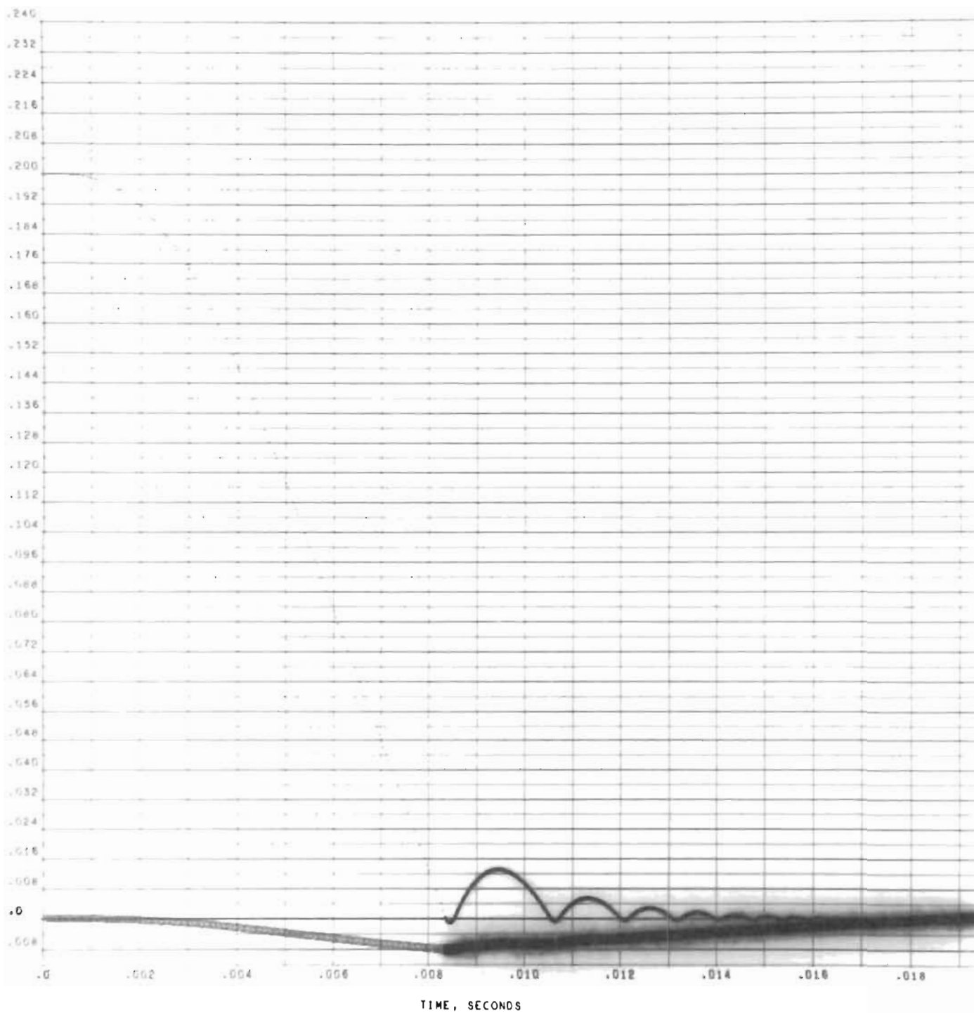
Figure 58. Computed Poppet (·) and Body (x) Displacements, 35.6 in./sec Impact Velocity, PS = 156 psia, DØD = 0.1702 in.
