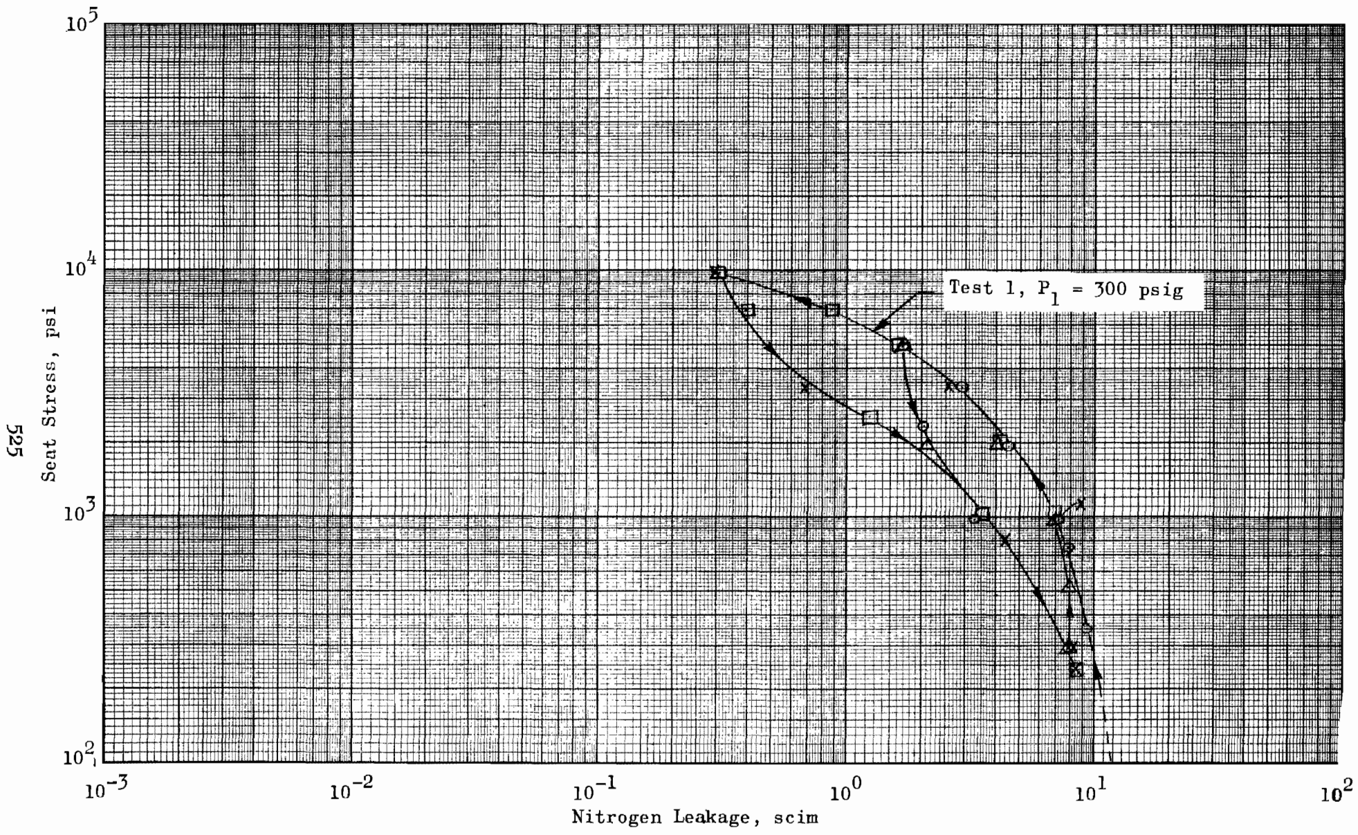
Figure 431. Stress-Leakage Data for Test Model C_c , Test 1
