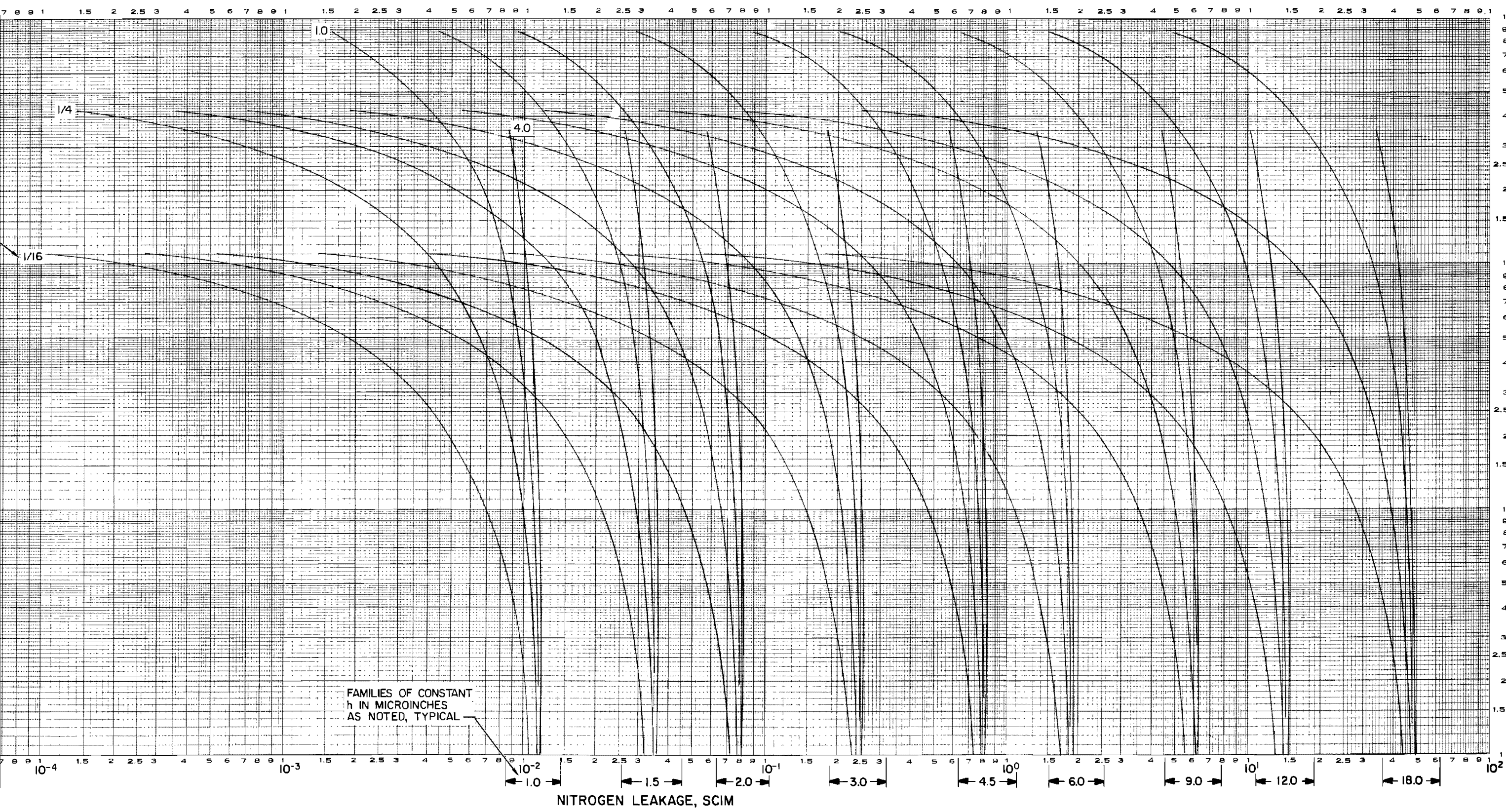
Figure 24. Theoretical Parametric Stress vs Leakage Curves for Tungsten Carbide
