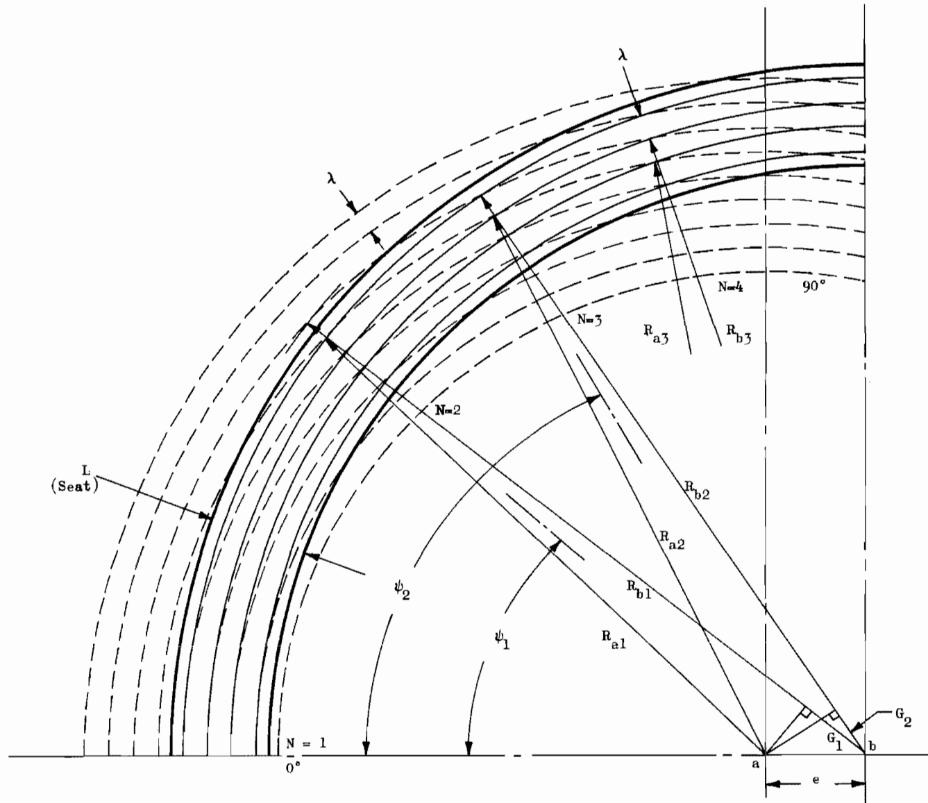
Figure 26. Model of Eccentric Circular Lay Surfaces
