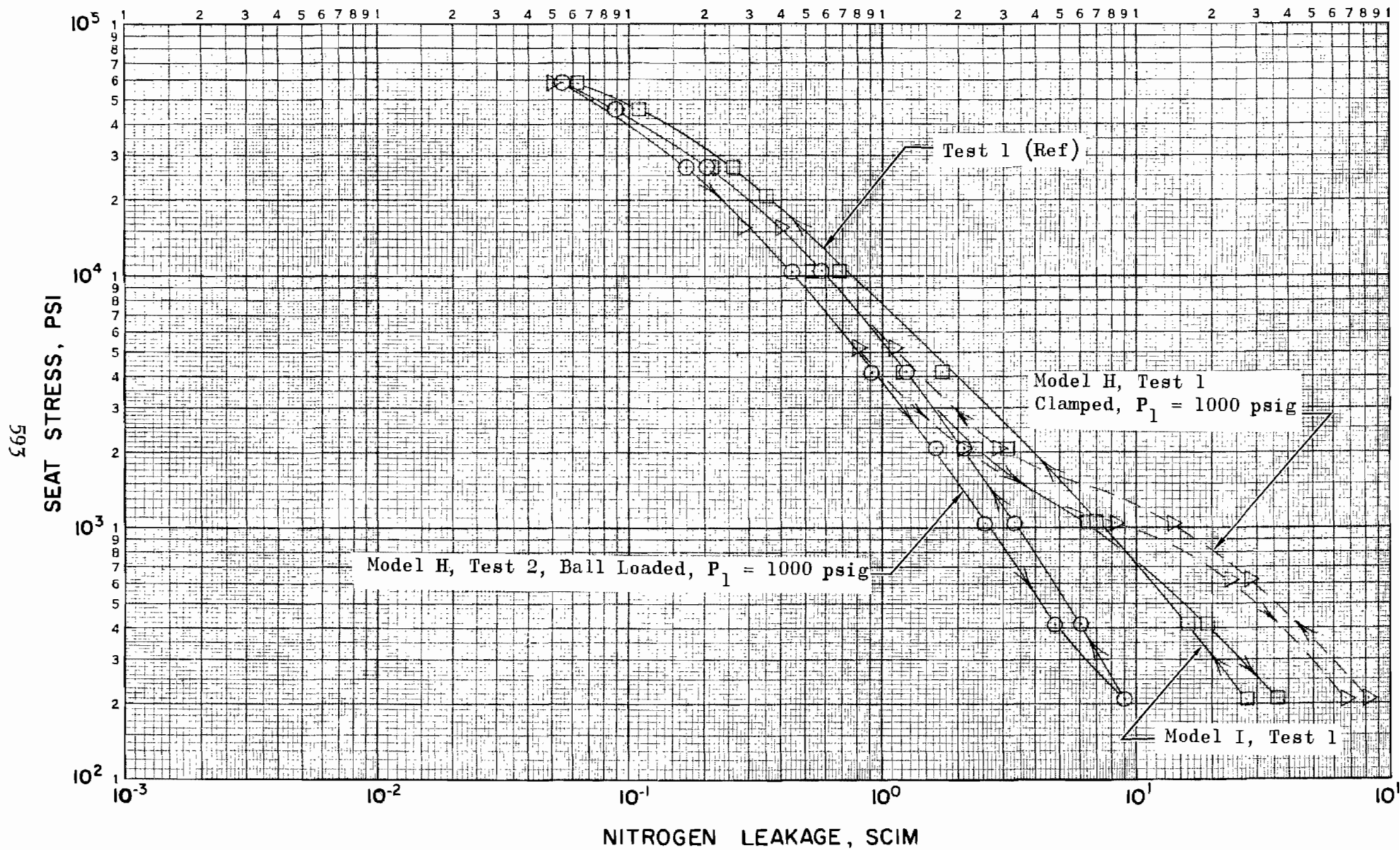
Figure 458. Stress-Leakage Data for Test Models H and I, Tests Noted
