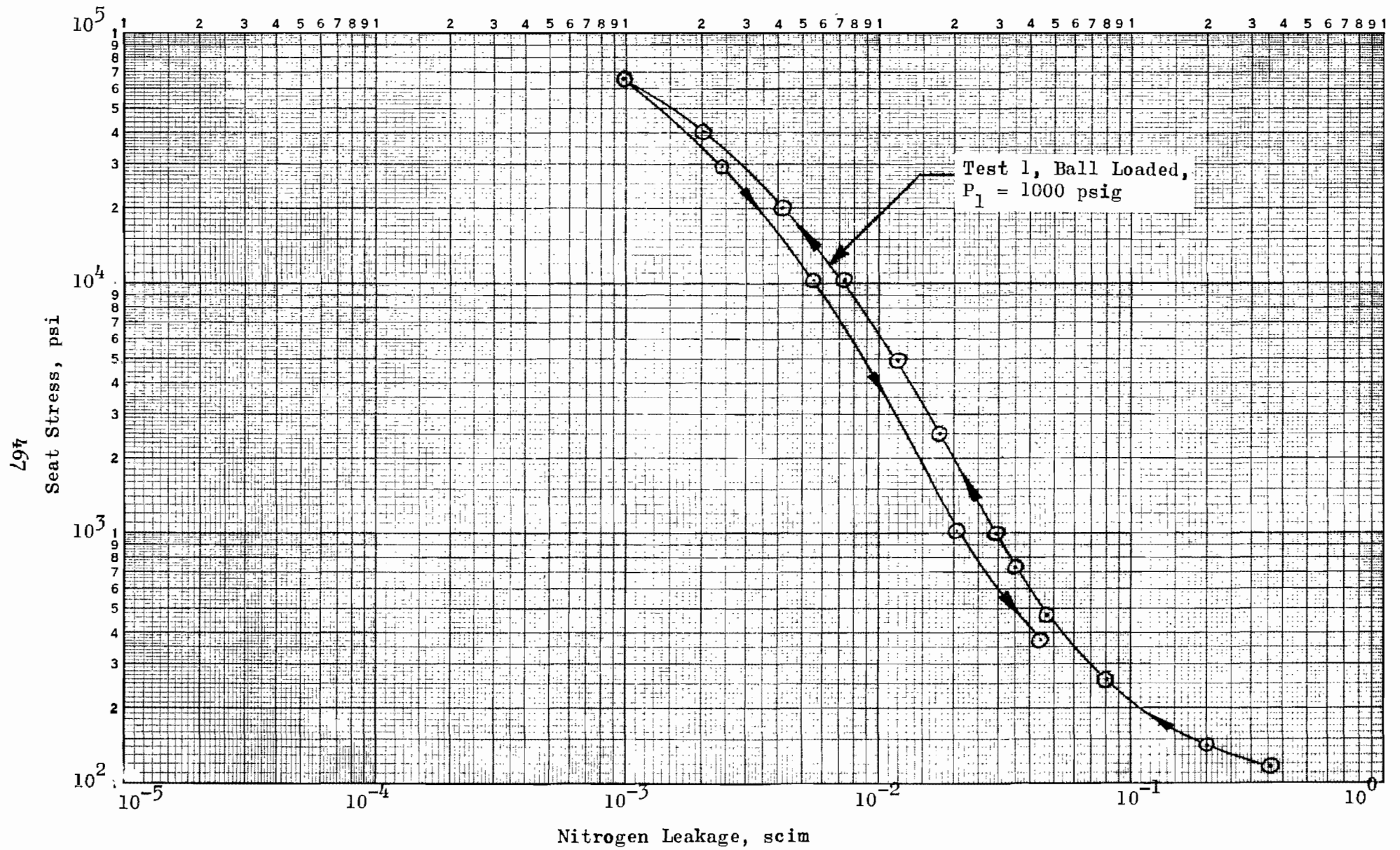
Figure 410. Stress-Leakage Data for Test Model G f1 , Test 1
