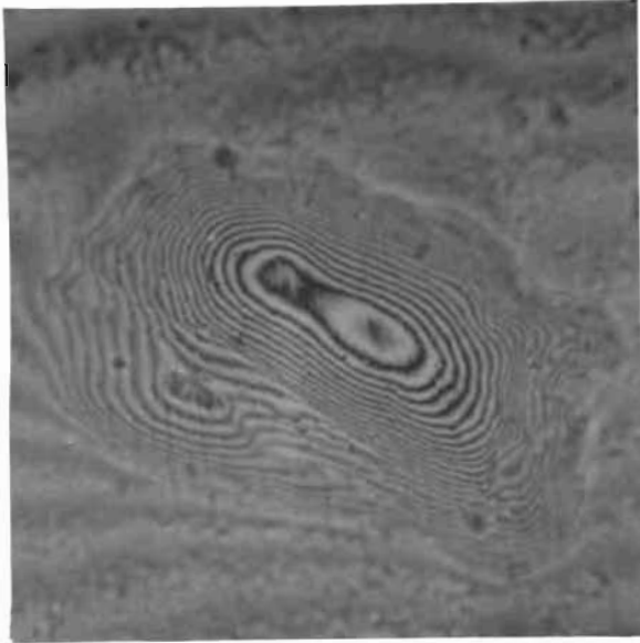
Figure 319. Test Model P f , Seat, 0.0065- x 0.0065-Inch Interference Photo, Same Location as Fig. 318
