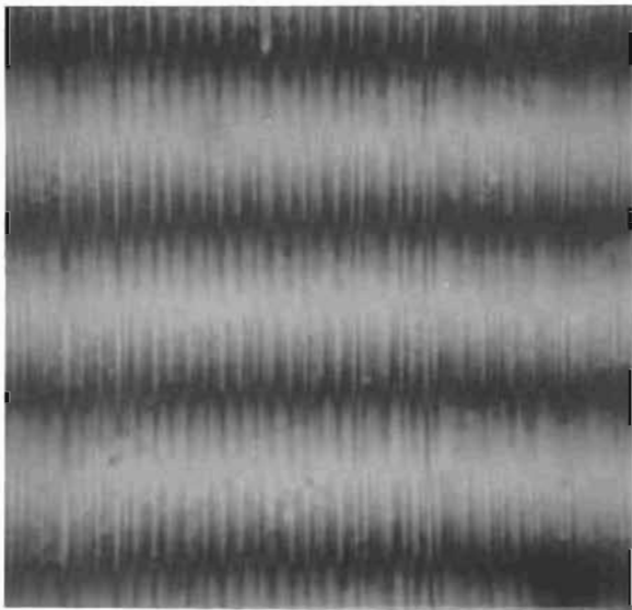
Figure 213. Test Model HH_f , Seat, 0.0065- x 0.0065-Inch Interference Photo
