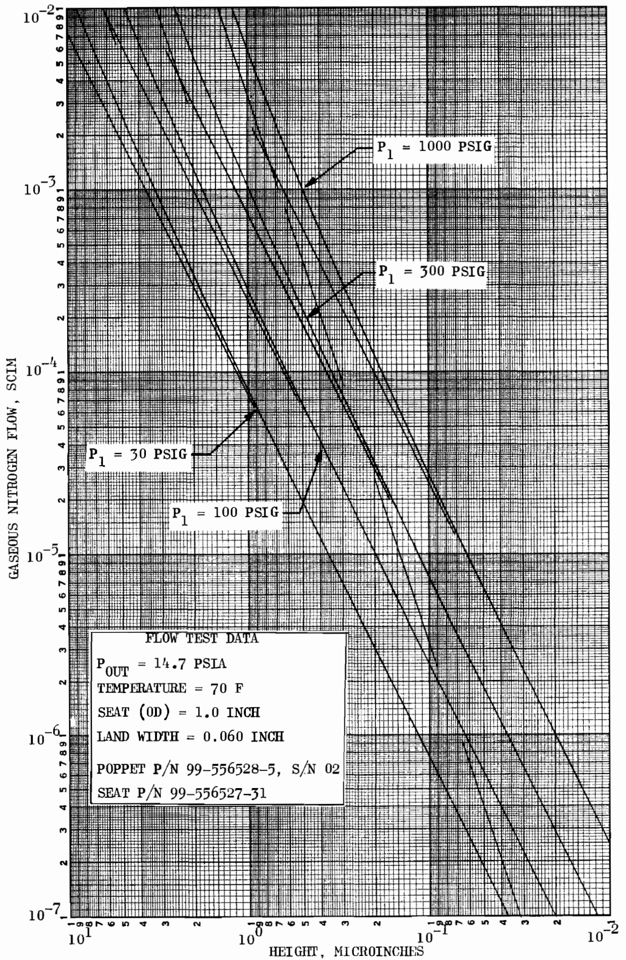
Figure 383. Nitrogen Flow Data, Part 3
