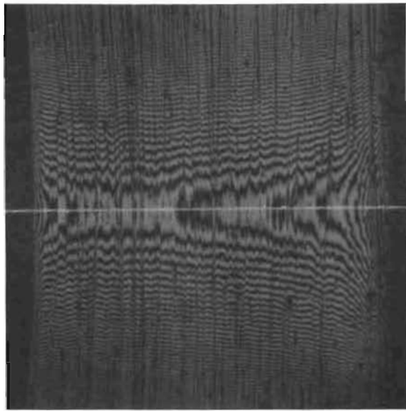
Figure 217. Test Model A c , Seat, 0.033- x 0.033-Inch Interference Photo
