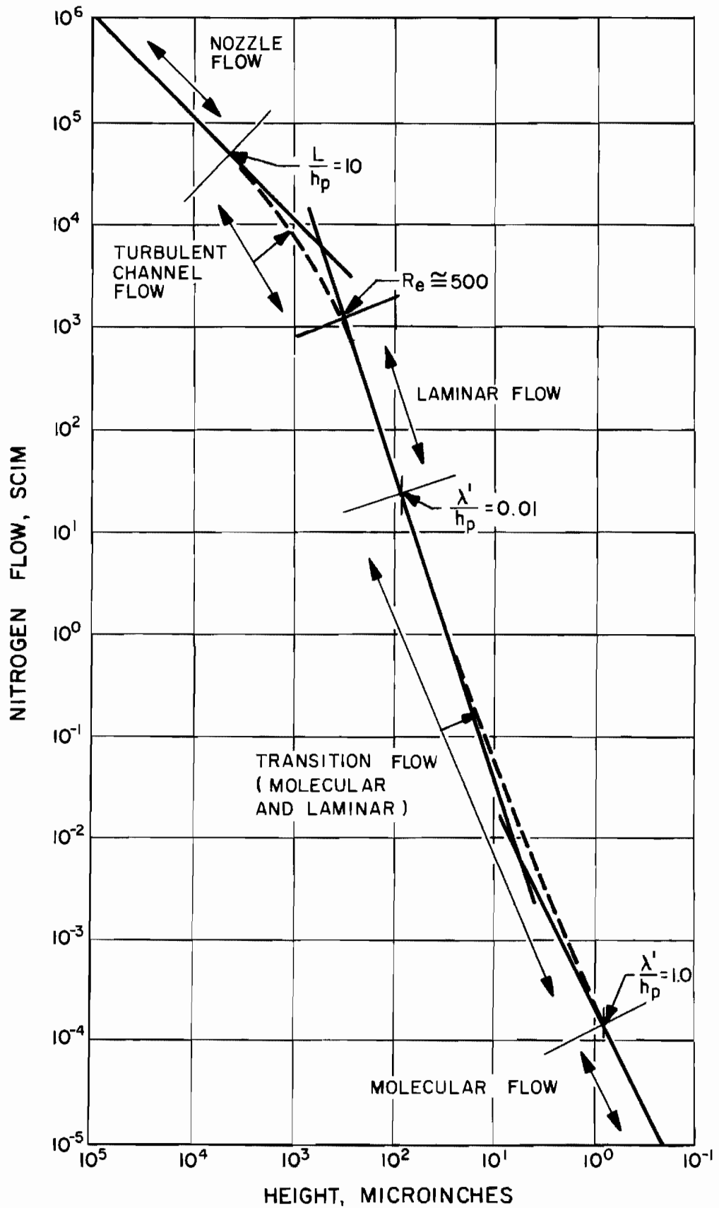
Figure 9. Theoretical Nitrogen Flow Through the Valve Model Shown in Fig. 8.
