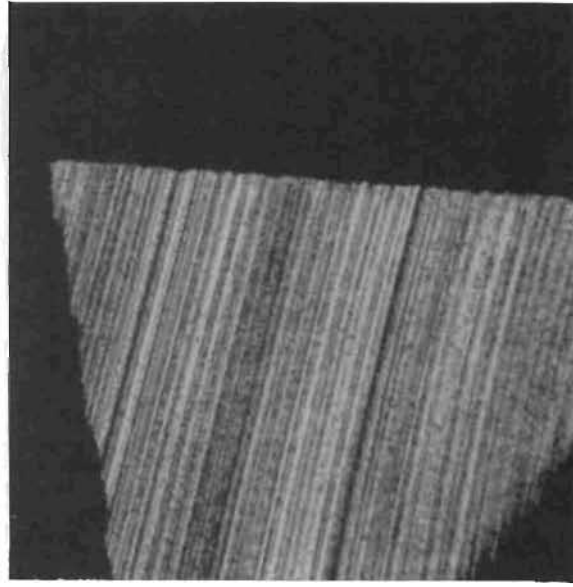
Figure 75. Sample 17-4 PH Cutting Tool No. 1, 0.033- x 0.033-Inch Plain Photo Showing Side Cutting Face As-Ground
