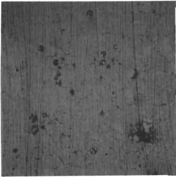
Figure 257. Test Model J_{f1} , Seat, 0.0065- x 0.0065-Inch Plain Photo, Same Location as Fig. 255 After Passivation
