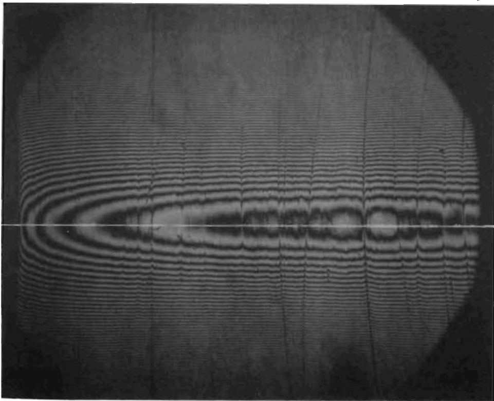
Figure 218. Test Model A c , Poppet, 0.045- x 0.056-Inch Inter- ference Photo, OD at Left
