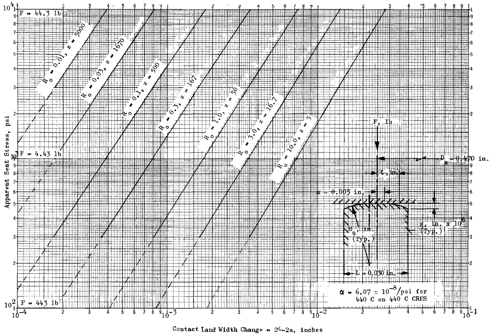
Figure 35. Dubbed Seat Contact Land Width Change vs Apparent Seat Stress
