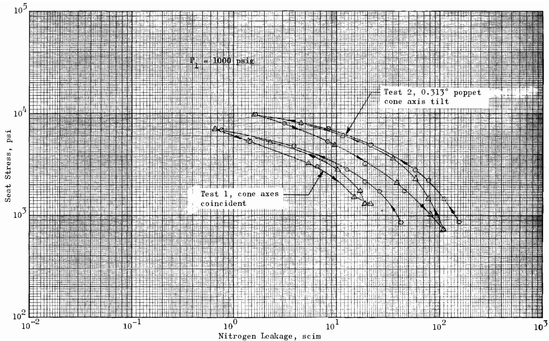
Figure 462. Stress-Leakage Data for Test Model H_c , Tests 1 and 2
