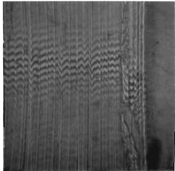
Figure 112. Test Model N_f , Seat, 0.0065- x 0.0065-Inch Interference Photo Showing OD Plastic Deformation, White Light
