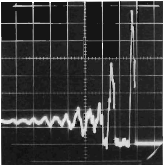
Figure 50. Piezoelectric Load Cell, 8.46 in./sec Impact Velocity, PS = 141 psig (162.5 lb/div; 0.0005 sec/div)
