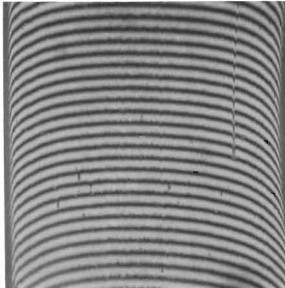
Figure 322. Test Model Z_f , Seat, 0.033- x 0.033-Inch Interference Photo
