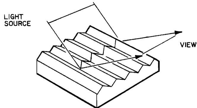
Figure 7. Principle of the Light Section Microscope
