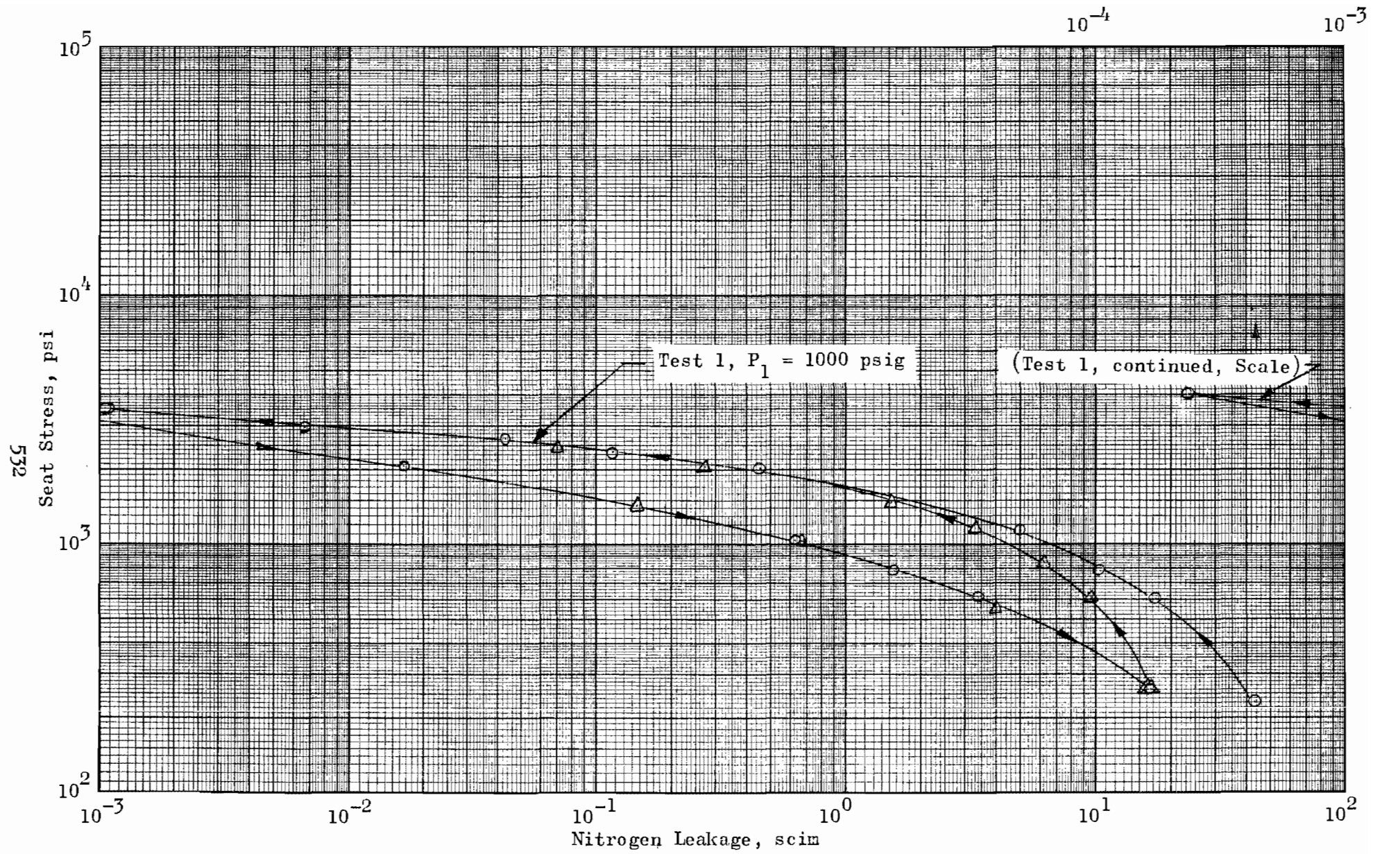
Figure 434. Stress-Leakage Data for Test Model F c , Test 1
