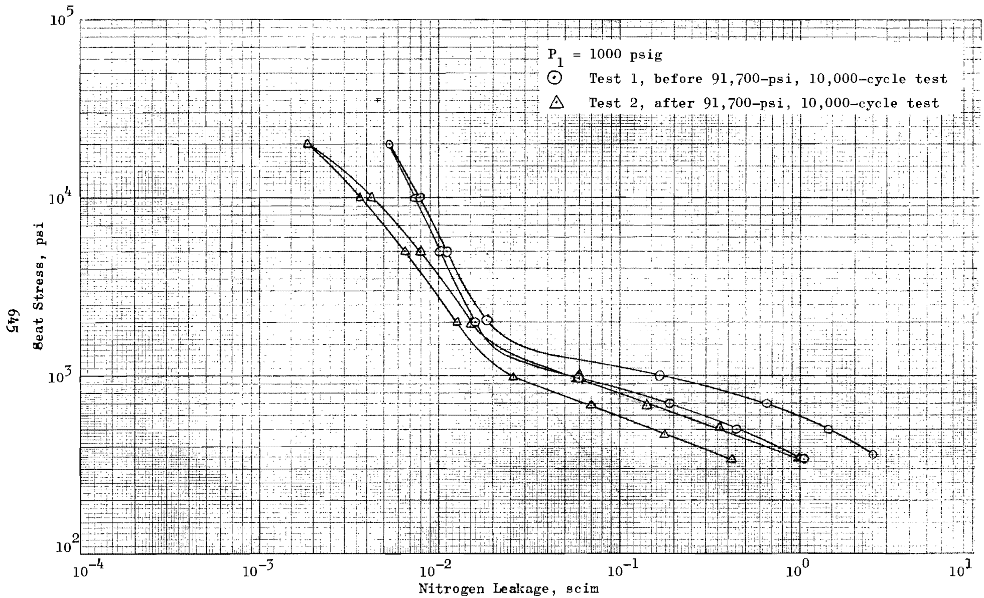
Figure 484. Stress-Leakage Data for Cycle Test Model Y_f , Tests 1 and 2
