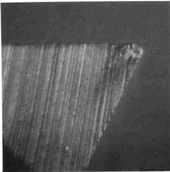
Figure 76. Sample 17-4 PH Cutting Tool No. 1, 0.033- x 0.033-Inch Plain Photo Showing Top Face After Turning Two Samples
