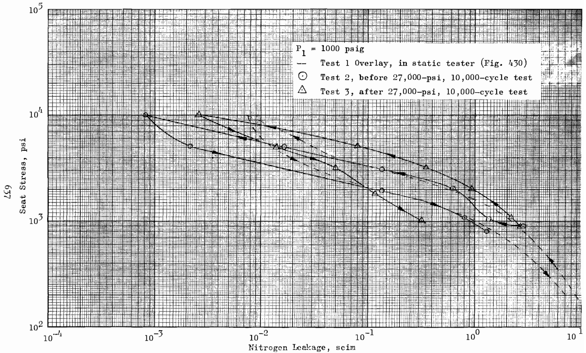
Figure 478. Stress-Leakage Data for Cycle Test Model B c , Tests 2 and 3
