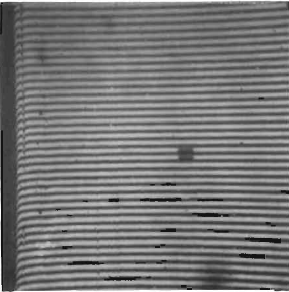
Figure 183. Test Model H f1 , Seat, 0.0065- x 0.0065-Inch Interference Photo Showing Embedded Contaminant From Finishing Process
