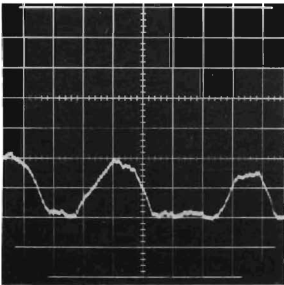
Figure 42. Strain Gage Load Cell No. 2, 1.87 in./sec Impact Velocity, PS=141 psig (50 lb/div; 0.0001 sec/div)
