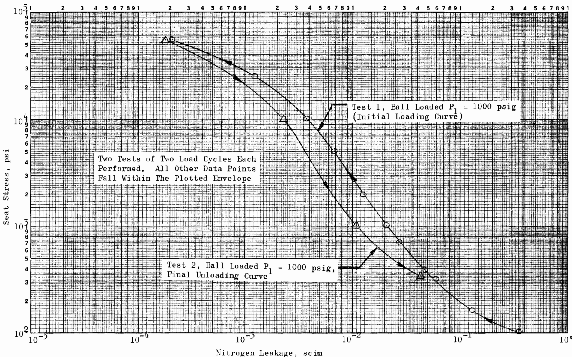
Figure 445. Stress-Leakage Data for Test Model J_f , Tests 1 and 2
