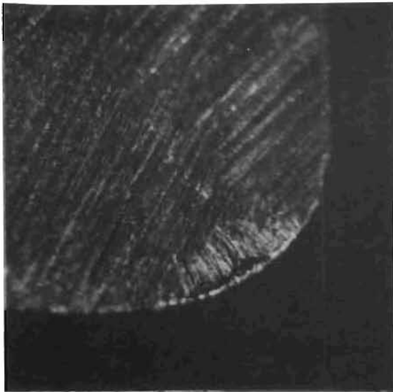
Figure 78. Formed Radius Sample 17.4 PH Cutting Tool, 0.033- x 0.033-Inch Plain Photo Showing Top Face After Sample Turning
