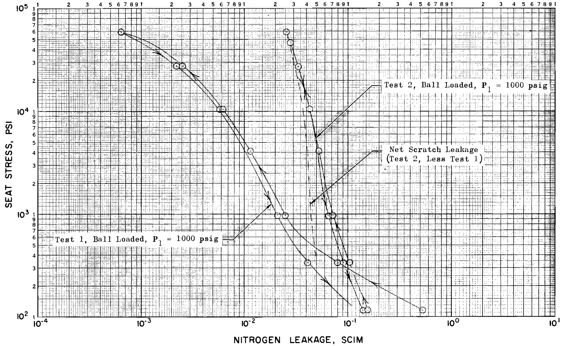
Figure 457. Stress-Leakage Data for Test Model G, Tests 1 and 2
