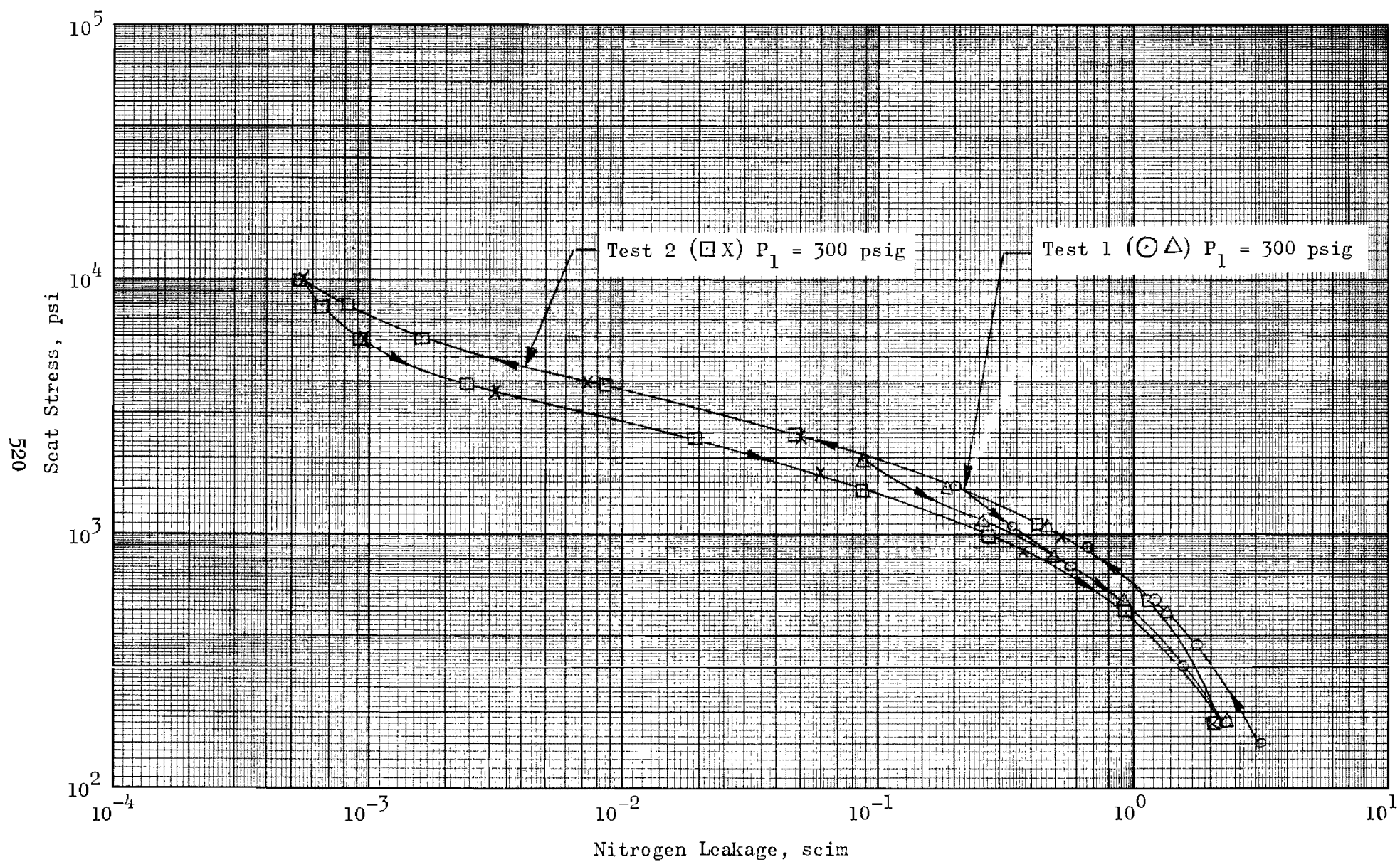
Figure 429. Stress-Leakage Data for Test Model A c , Tests 1 and 2
