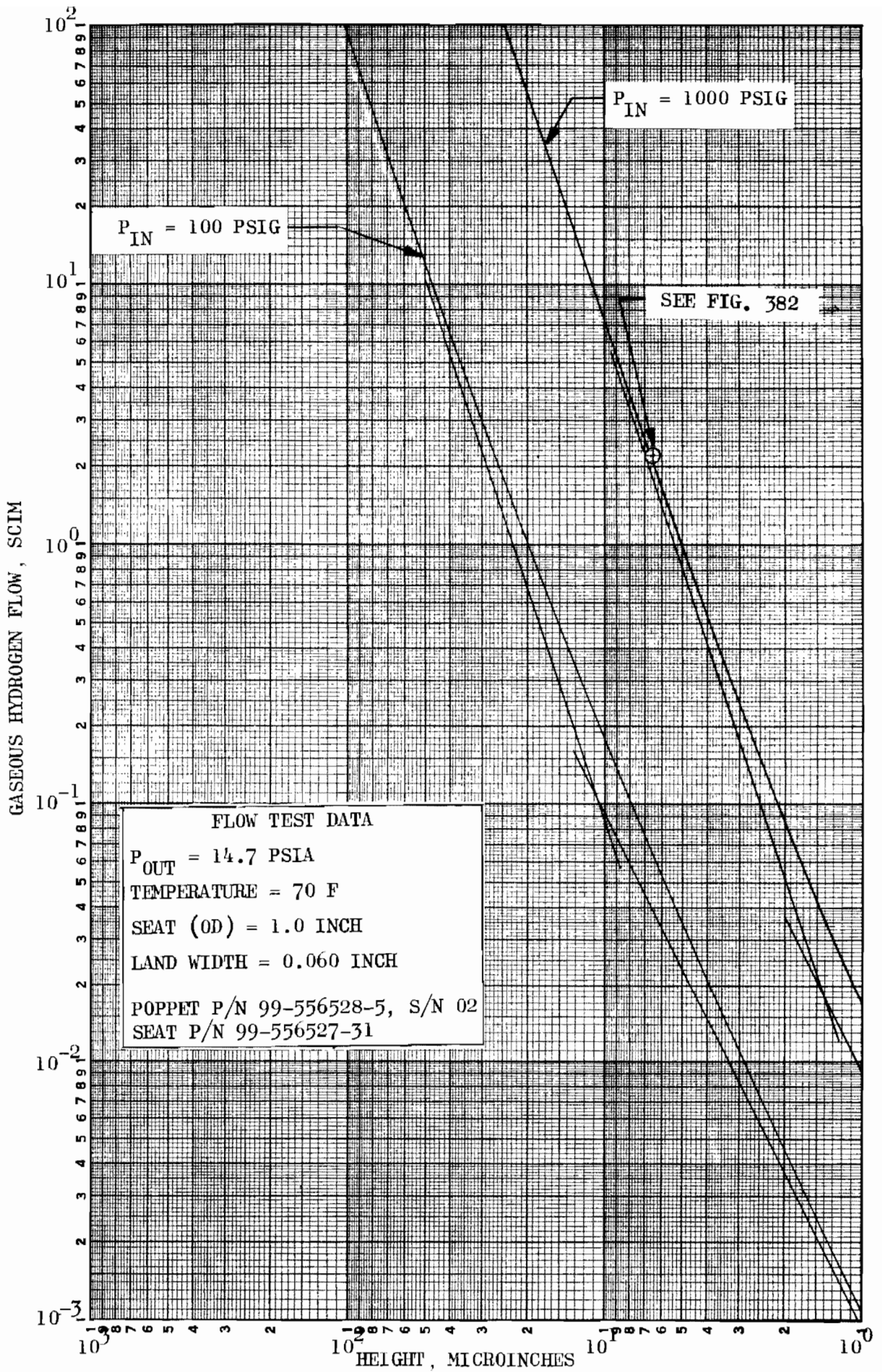
Figure 389. Hydrogen Flow Data, Part 2
