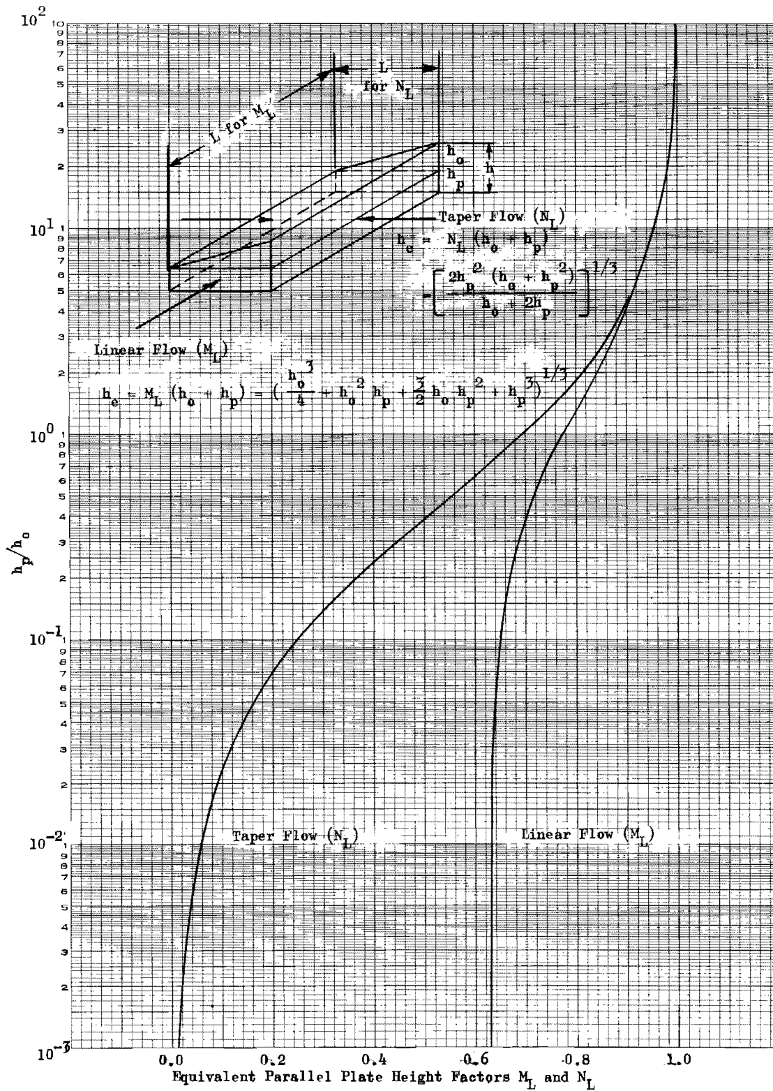
Figure 12. Laminar Flow Factors
