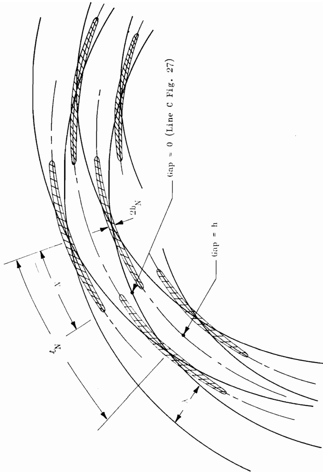
Figure 28. Circular Lay Surface Contact at Closure
