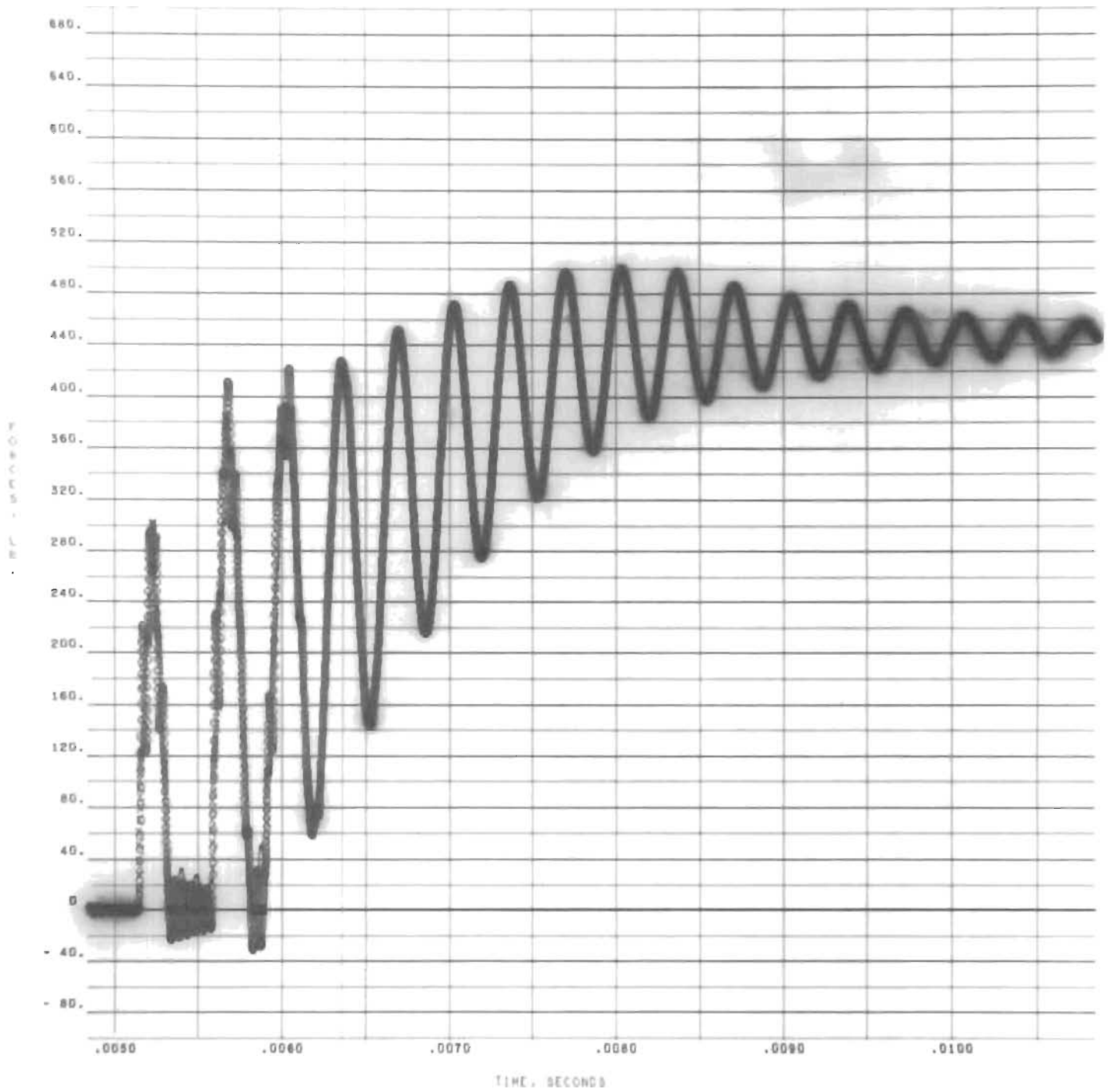
Figure 55. Computed Spring Forces, F1 ( \cdot ), F2 (x), F3 (o), 1.77 in./sec Impact Velocity, PS = 287 psia D\phi D = 0.0217 in.
