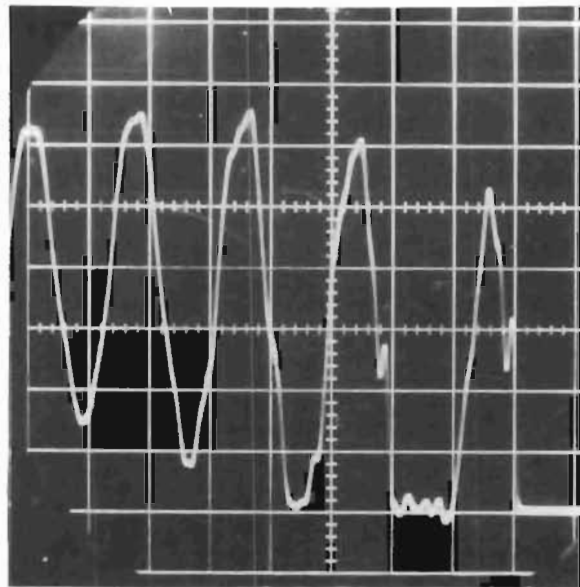
Figure 45. Piezoelectric Load Cell, 1.87 in./sec Impact Velocity, PS = 141 psig (50 lb/div; 0.0002 sec/div)
