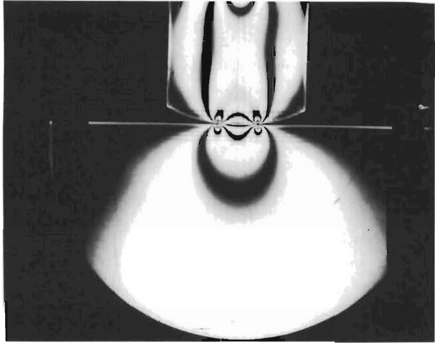
Figure 31. Photoelastic Model Showing Isochromatic Fringes
