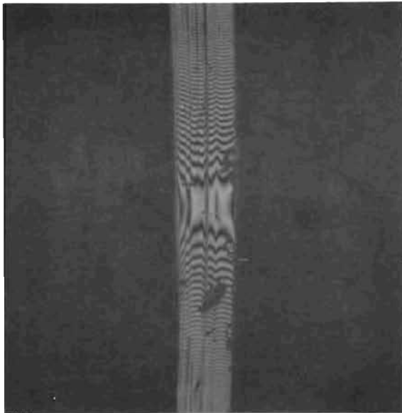
Figure 227. Test Model D_c , Seat, 0.033- x 0.033-Inch Interference Photo, Same Location as Fig. 226 After Rework Lapping
