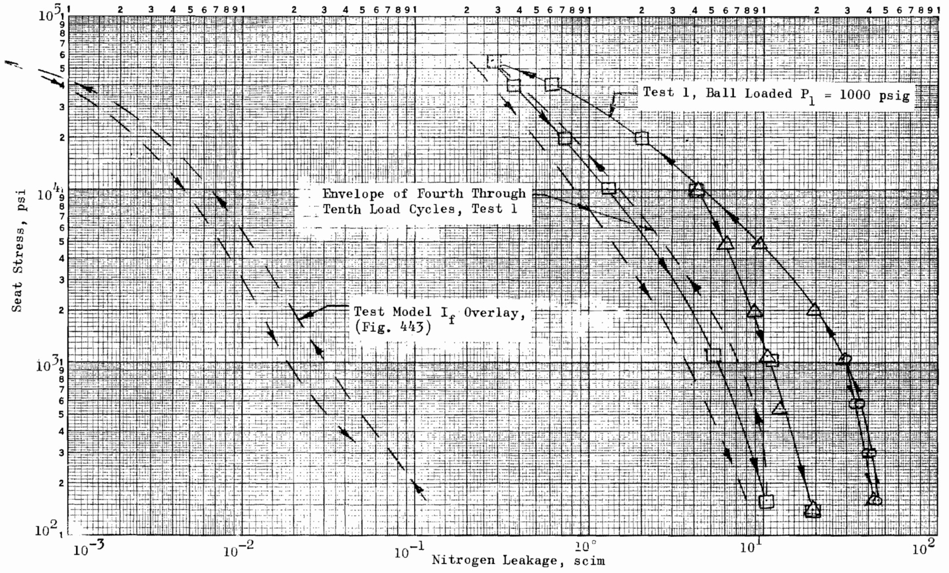
Figure 444. Stress-Leakage Data for Test Model I_{f1} , Test 1
