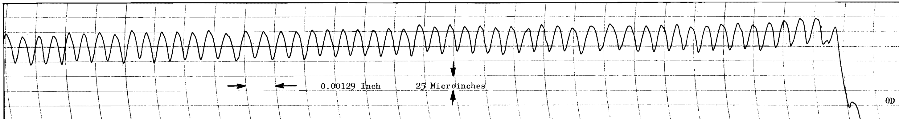
Figure 330. Test Model Q f , Poppet Cross Lay Roughness Profile Record, 0.0001-Inch Radius Stylus
