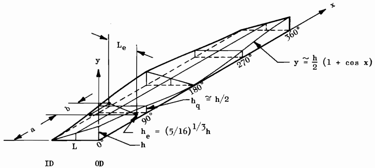
Figure 15. Seat Gap Volume From a Tilted Conical Poppet
