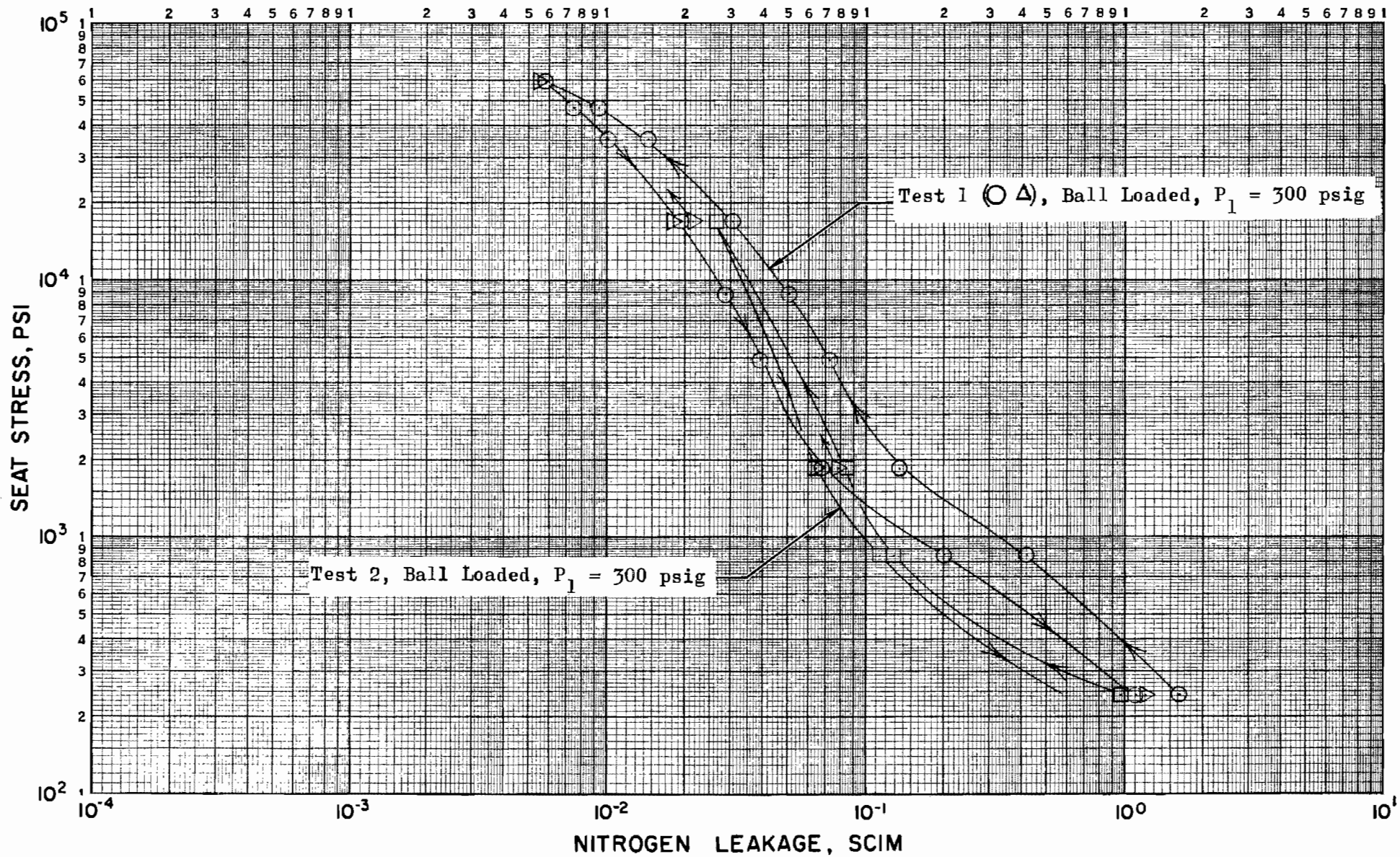
Figure 406. Stress-Leakage Data for Test Model J, Tests 1 and 2
