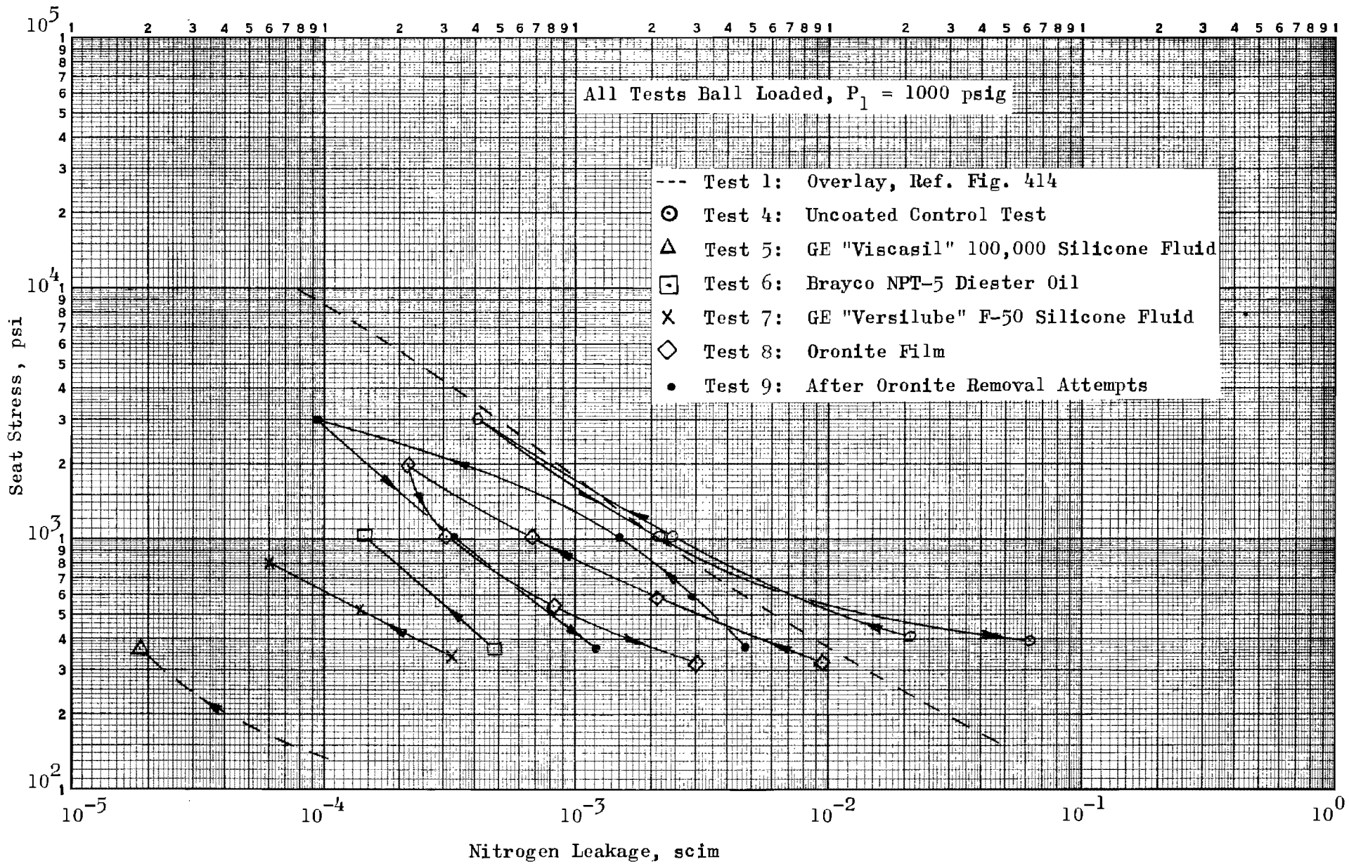
Figure 455. Stress-Leakage Data for Test Model B_{f1} , Tests 4 Through 9
