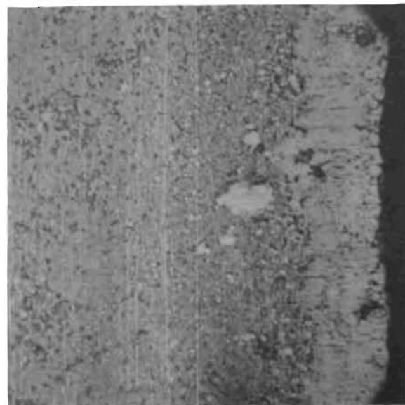
Figure 284. Test Model T_{f1} , Seat, 0.0065- x 0.0065-Inch Plain Photo Showing ID Plastic Flow After Cycling, Same Location as Fig. 282
