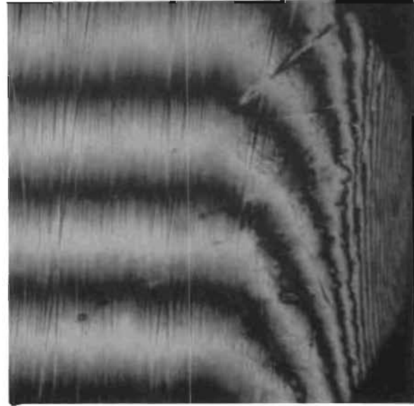
Figure 316. Test Model P f , Poppet, 0.0065- x 0.0065-Inch Interference Photo, Same Location as Fig. 315 at ID
