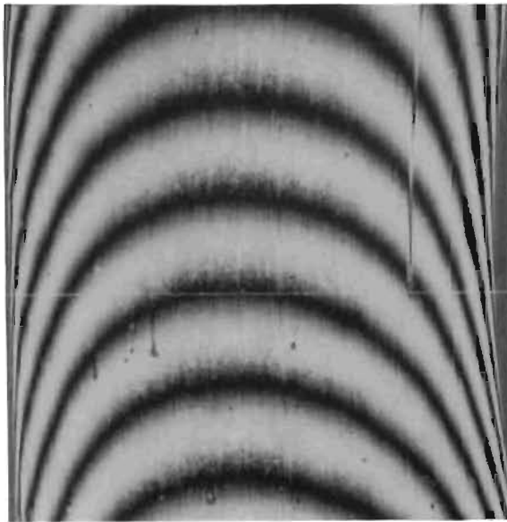
Figure 323. Test Model Z_f , Seat, 0.033- x 0.033-Inch Interference Photo, Same Location as Fig. 322
