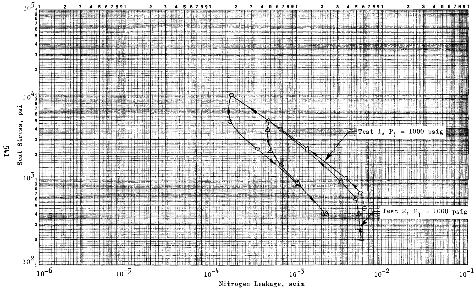
Figure 438. Stress-Leakage Data for Test Model C_s , Tests 1 and 2
