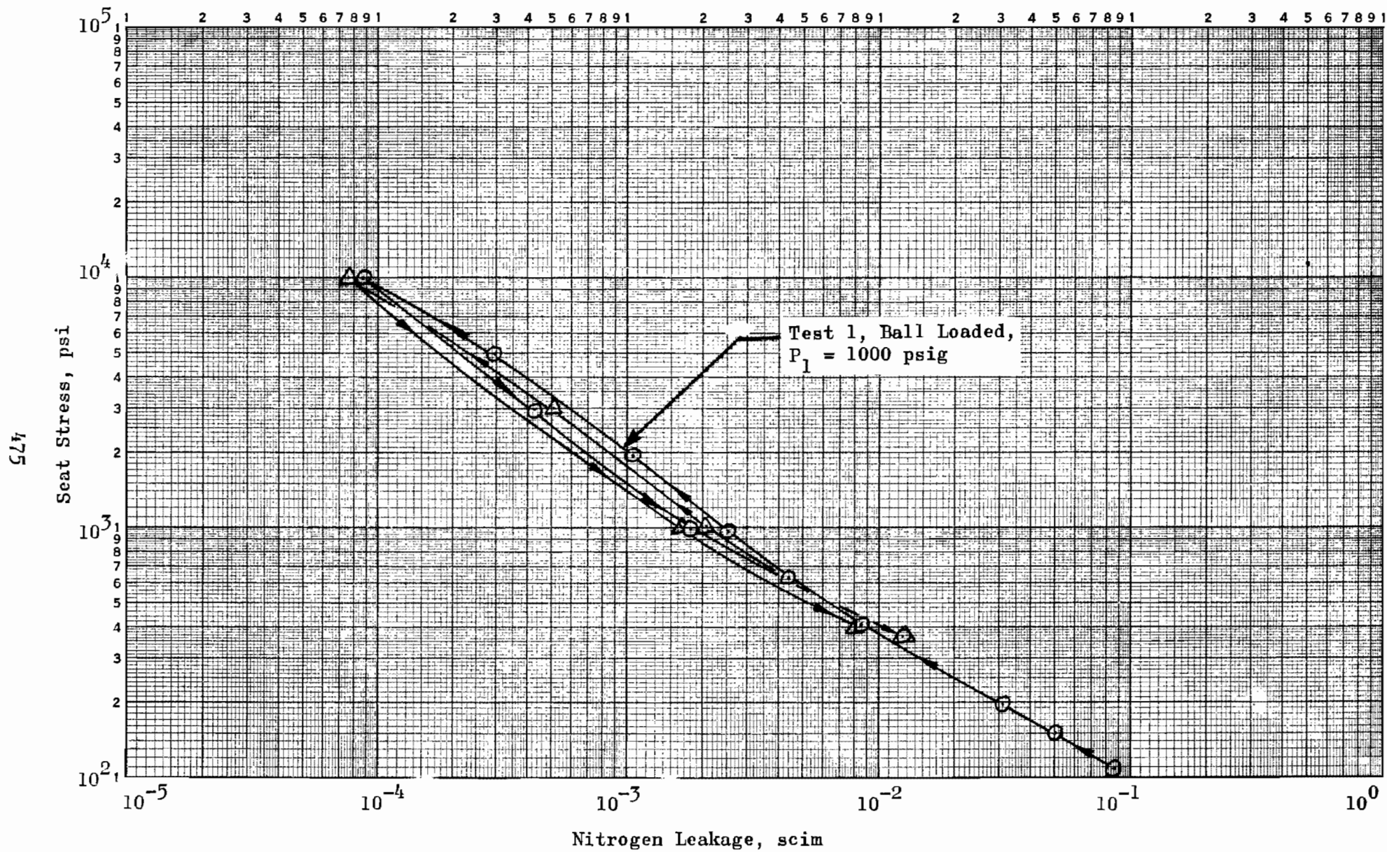
Figure 414. Stress-Leakage Data for Test Model B f1 , Test 1
