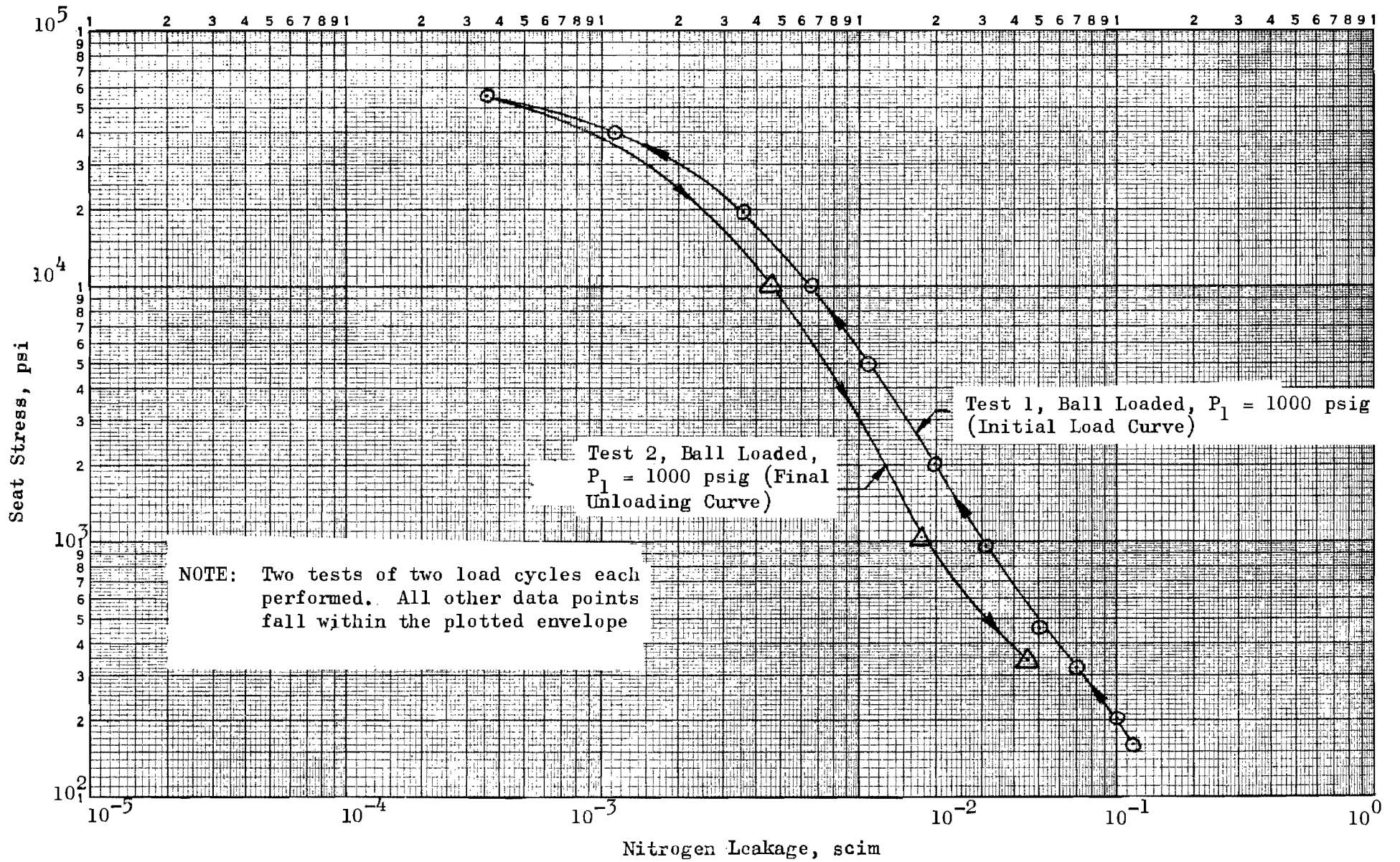
Figure 443. Stress-Leakage Data for Test Model I_f , Tests 1 and 2
