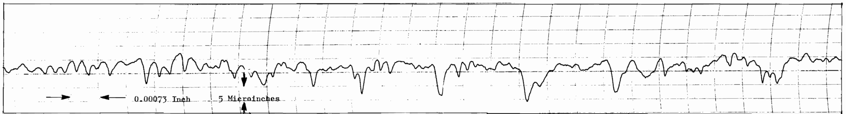
Figure 334. Test Model D_f , Poppet Roughness Profile Record, 0.0001-Inch Radius Stylus
