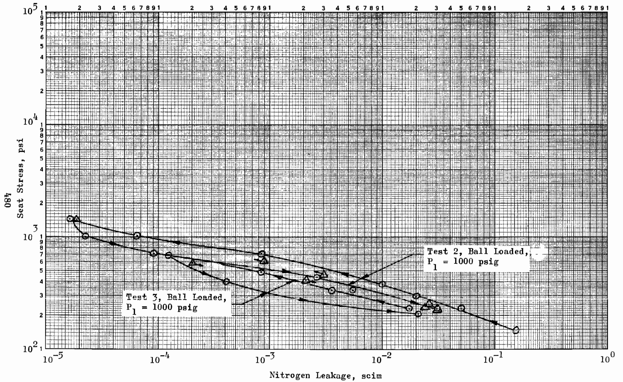
Figure 417. Stress-Leakage Data for Test Model H f1 , Tests 2 and 3
