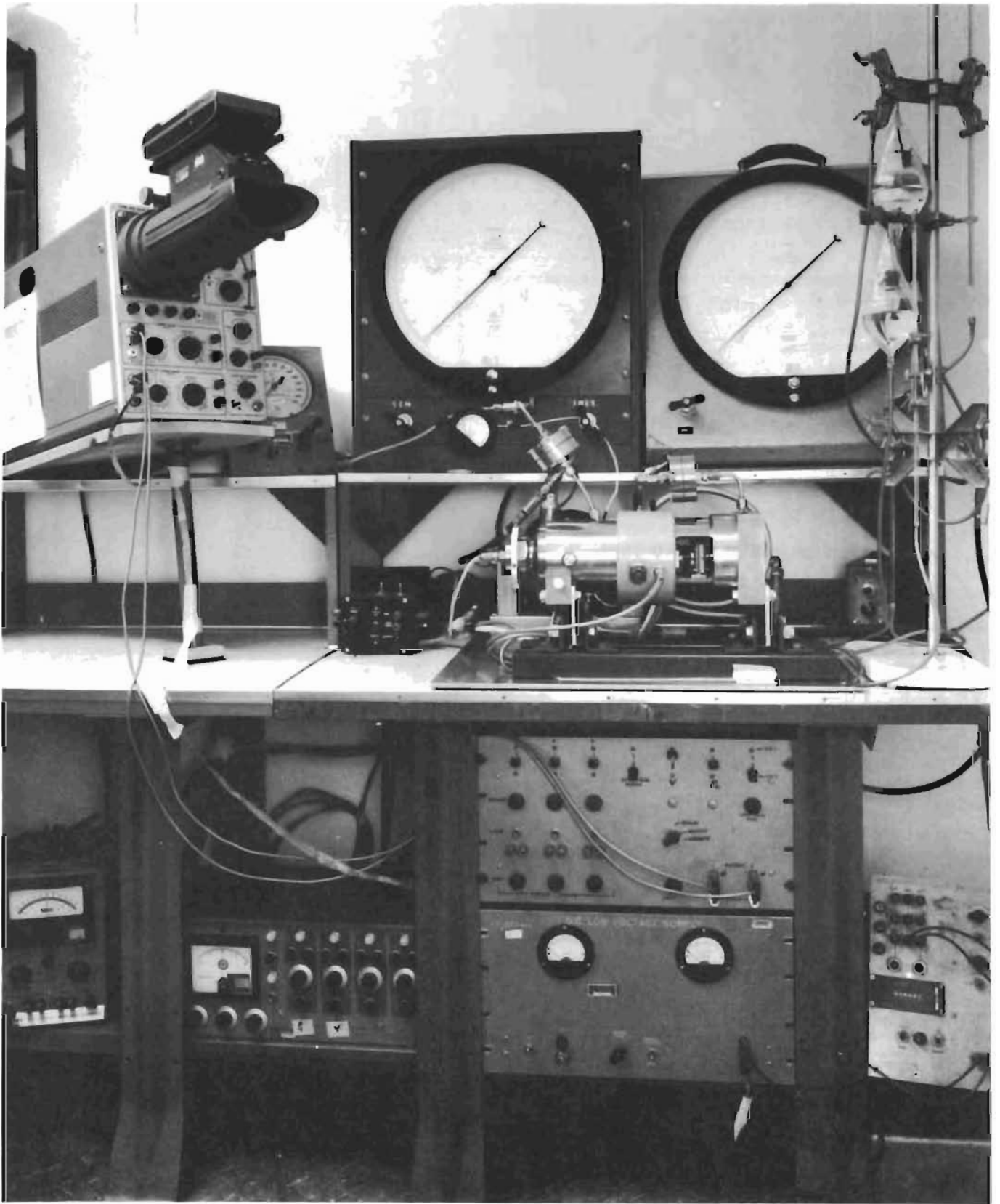
Figure 376. Cycle Test Setup
