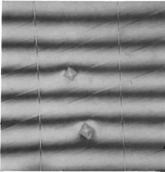
Figure 189. Test Model L_f , Seat, 0.0065- x 0.0065-Inch Interference Photo, Same Location as Fig. 188
