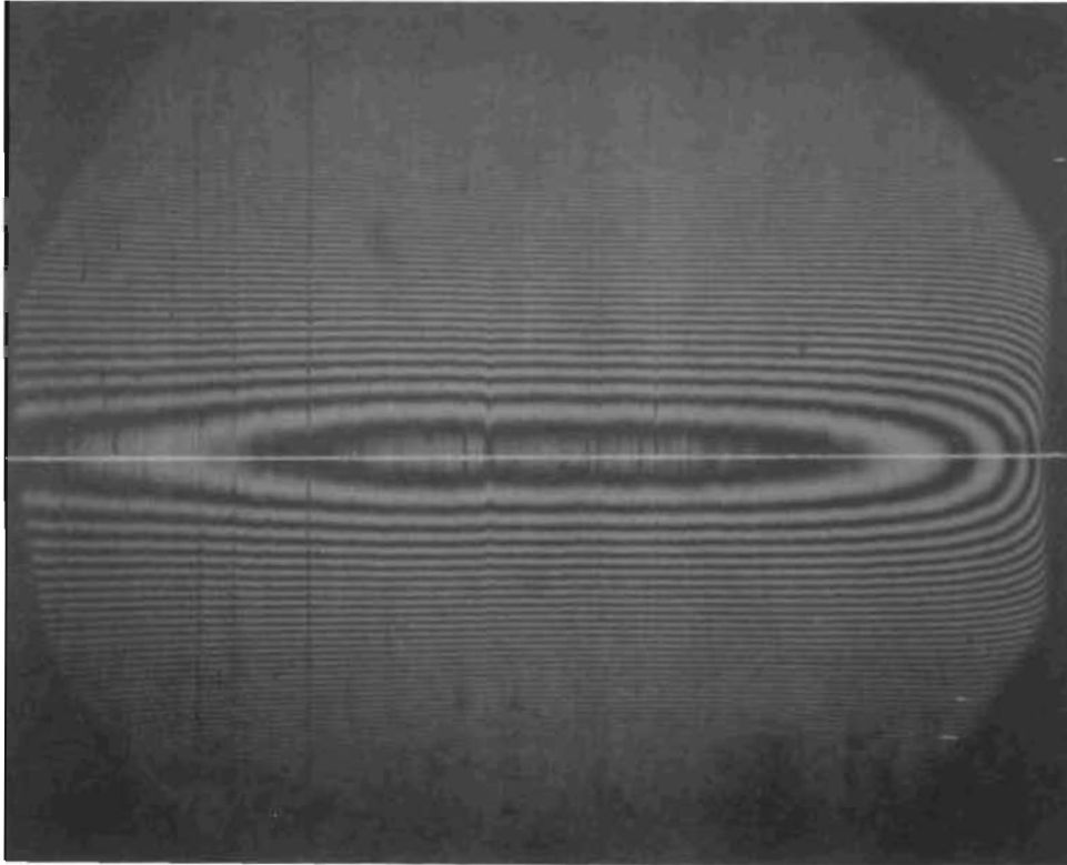
Figure 232. Test Model F_c , Poppet, 0.045- x 0.056-Inch Interference Photo, ID at Right
