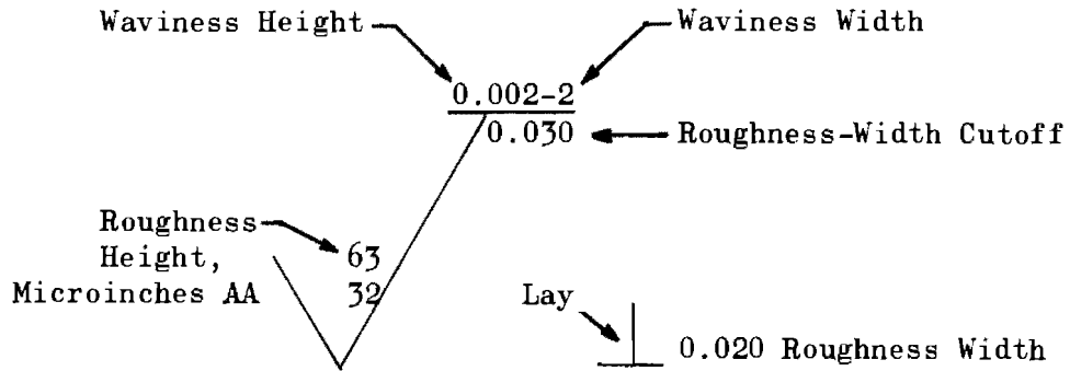
Figure 1. Standard Surface Symbol With Representative Surface Characteristics
