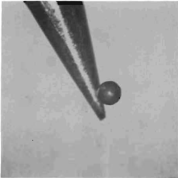
Figure 291. Handling Probe and Lead Particle 3, 0.033- x 0.033-Inch Plain Photo (Ref. Test Model L)
