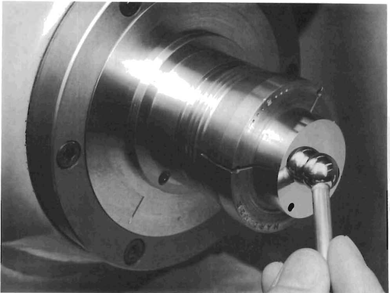
Figure 83. Spherical Seat Lapping
