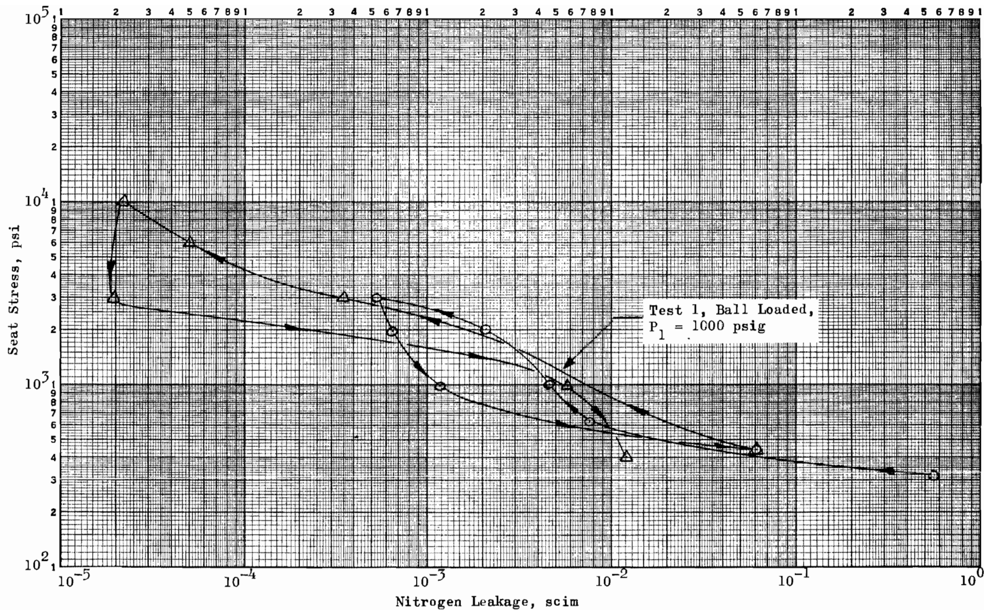
Figure 397. Stress-Leakage Data for Test Model S f , Test 1 (Continued)
