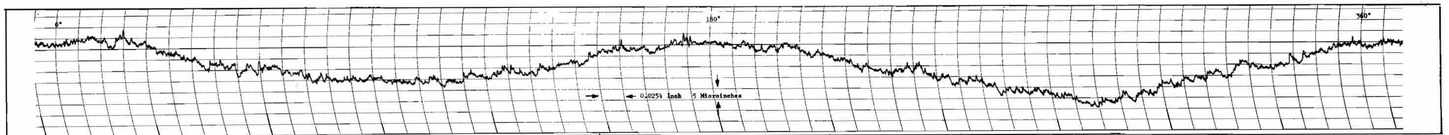
Figure 348. Test Model A c , Seat Circumferential Roundness Profile Record, Midland, 1/16-Inch Ball Stylus
