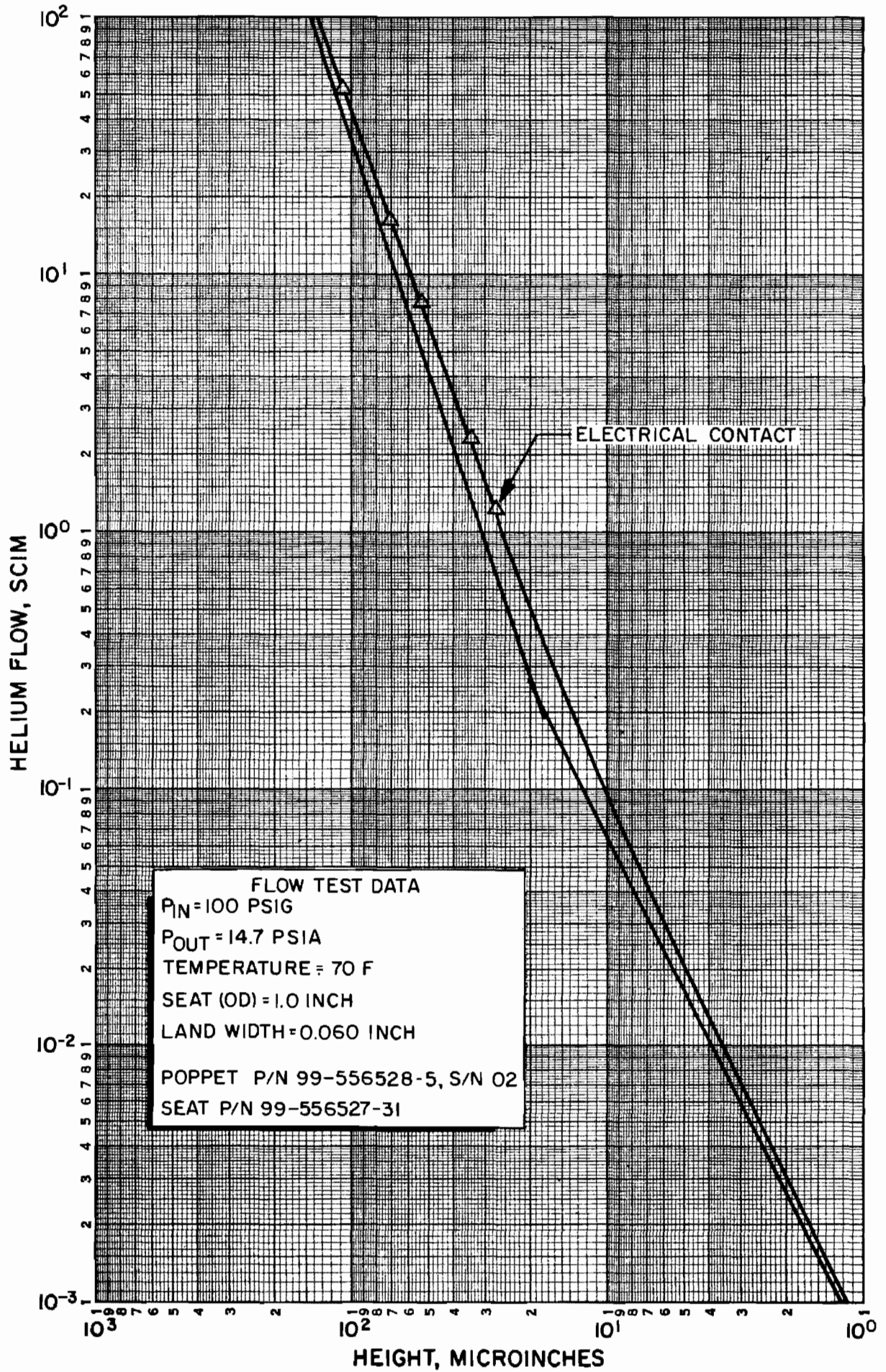
Figure 385. Helium Flow Data, Part 2
