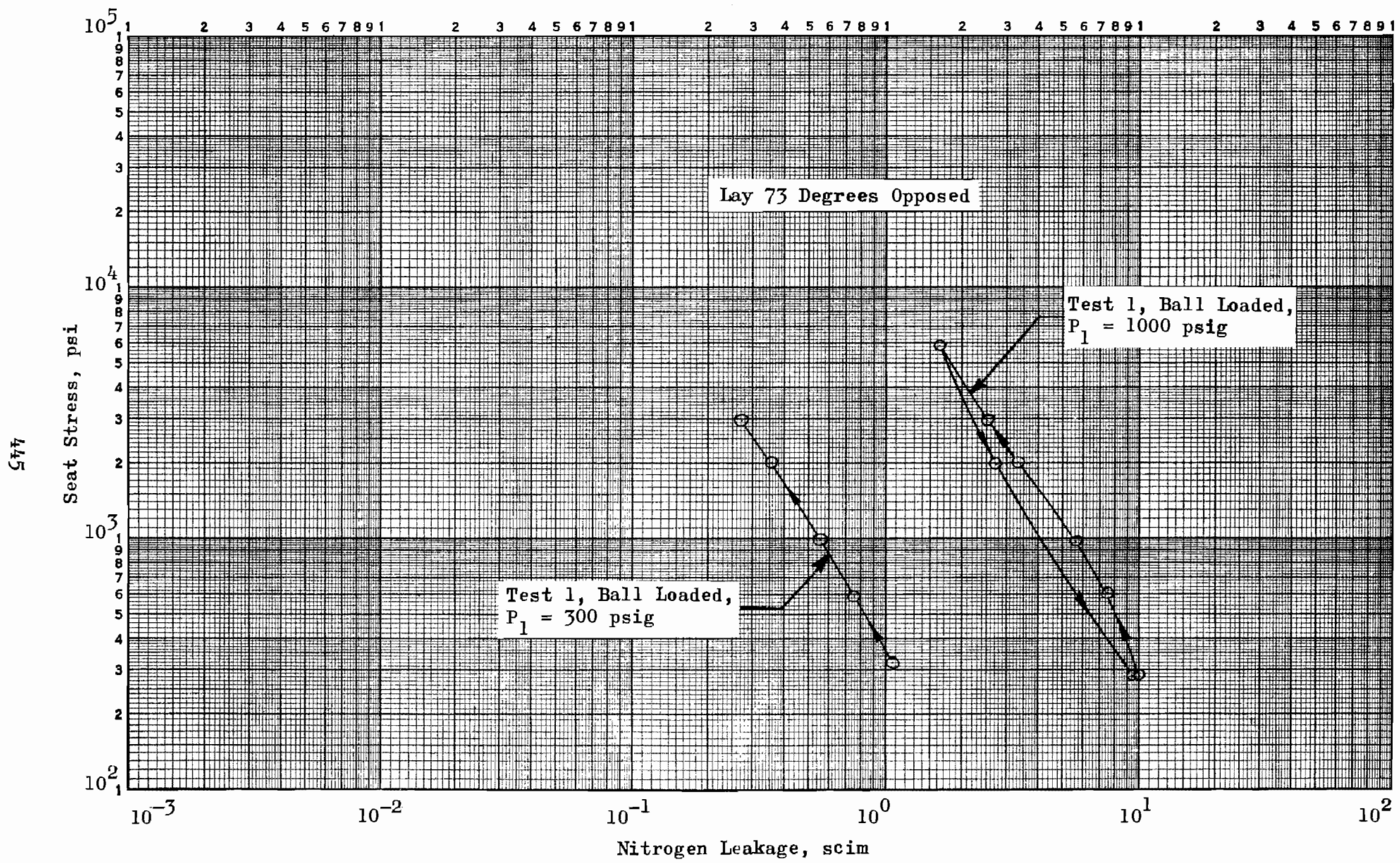
Figure 399. Stress-Leakage Data for Test Model D_f , Test 1
