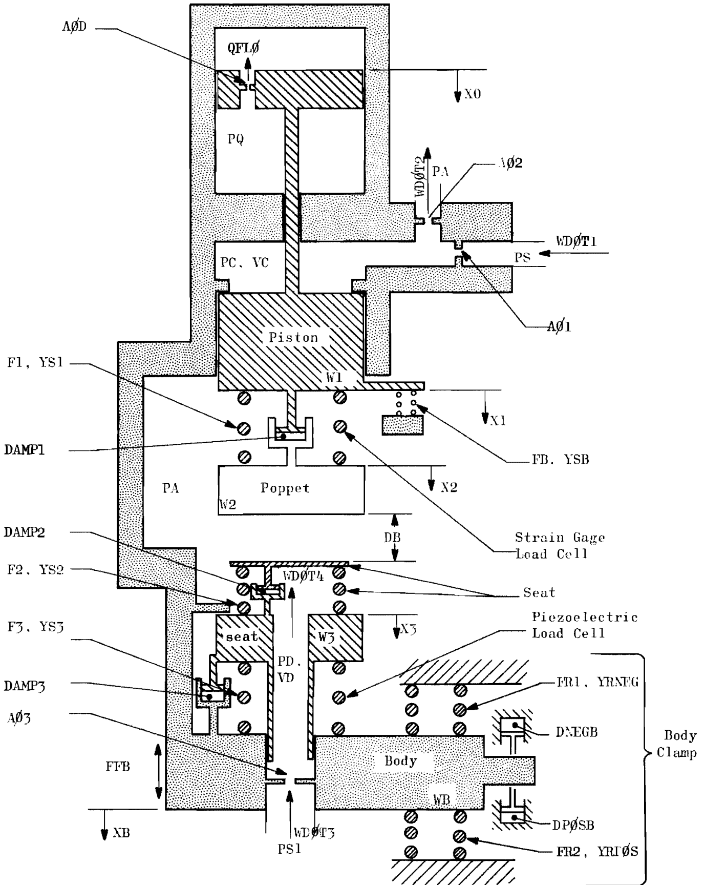
Figure 39.. Cycle Test Fixture Digital Computer Mathematical Model
