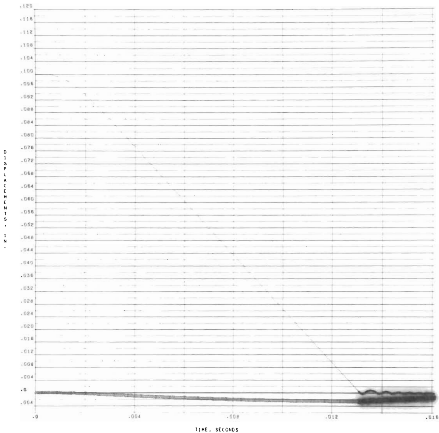
Figure 56. Computed Poppet (·) and Body (x) Displacements, 8.46 in./sec Impact Velocity, PS = 156 psia, D\phi D = 0.0591 in.
