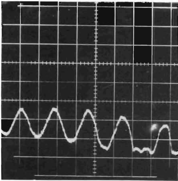
Figure 44. Strain Gage Load Cell No. 1, 1.87 in./sec Impact Velocity, PS = 141 psig (50 lb/div; 0.0002 sec/div)
