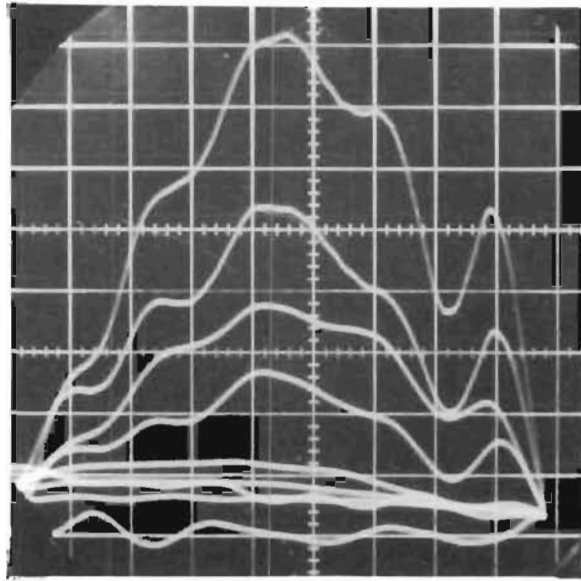
Figure 471. Test Model D f , Piezo- electric Load Cell, 24 in./sec Impact Velocity, PS = 169 psig (500 lb/div.; 0.00002 sec/div.)
