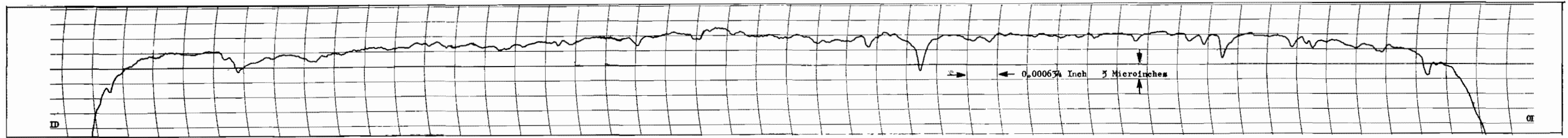
Figure 371. Test Model U_f , Seat Cross Land Roughness Profile Record, 0.0001-Inch Radius Stylus
