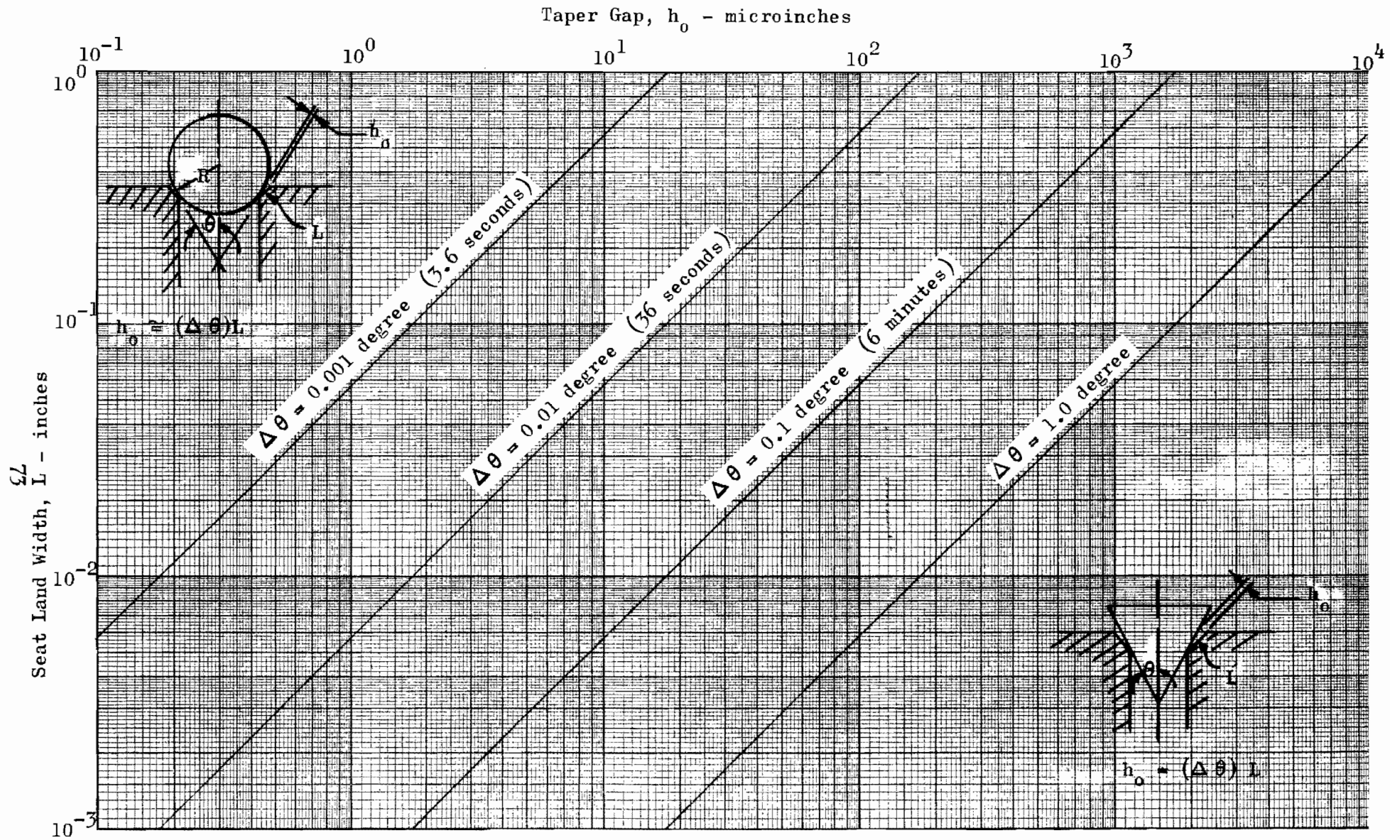
Figure 11. Taper Gap for Flat, Conical, and Spherical Seating
