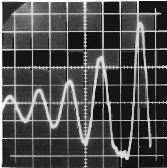
Figure 477. Test Model B c , Piezo- electric Load Cell, 5.6 in./sec Impact Velocity, PS = 150 psig (87.5 lb/div.; 0.0002 sec/div.)
