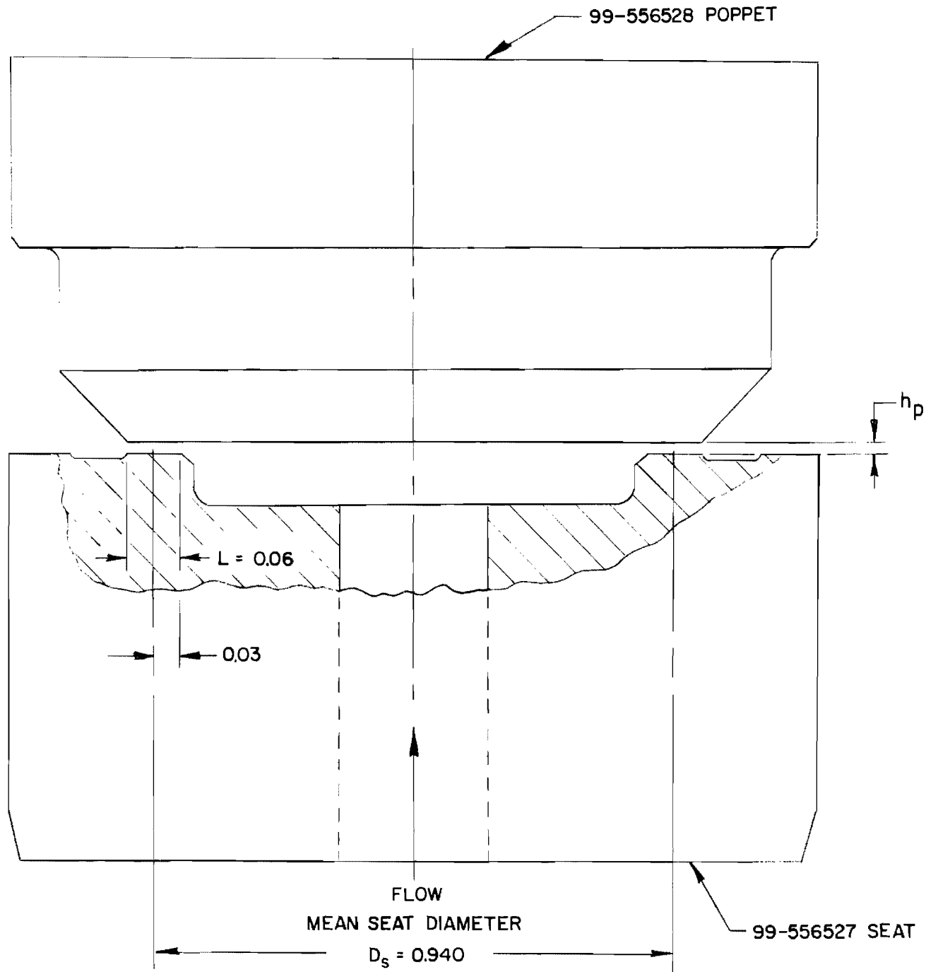
Figure 8. Typical 1.0-Inch Poppet and Seat Model
