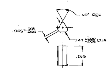
(63) PIN
