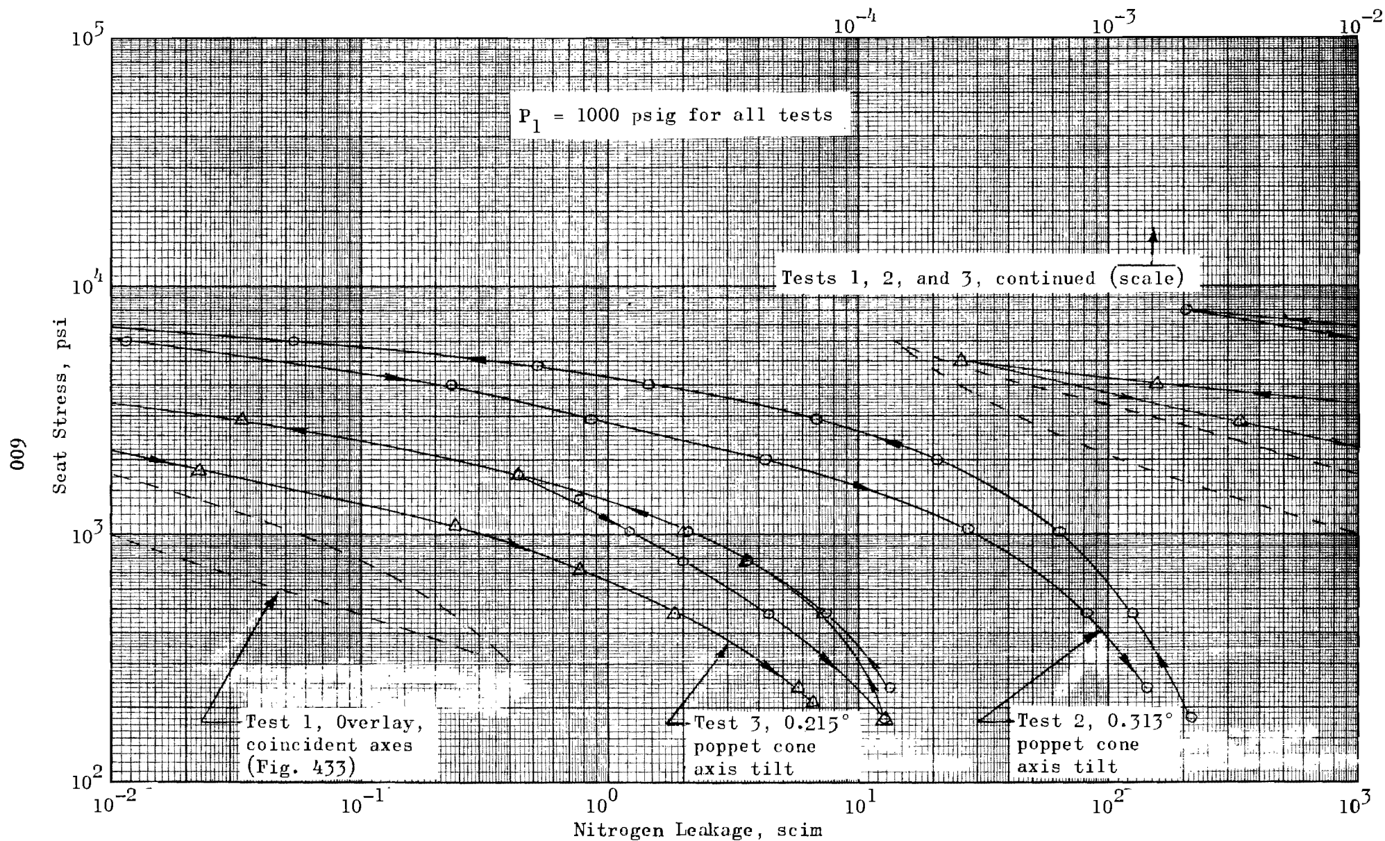
Figure 460. Stress-Leakage Data for Test Model E_c , Tests 2 and 3
