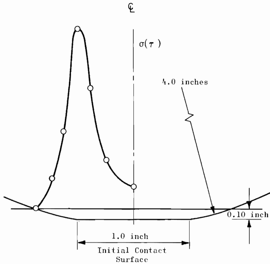
Figure 33. Normal Stress on Gridline 0.10-Inch From Initial Contact Surface
