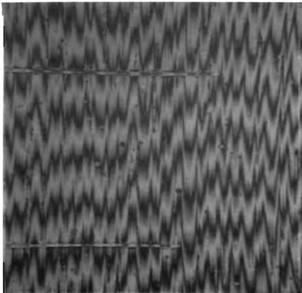
Figure 111. Test Model N_f , Poppet, 0.0065- x 0.0065-Inch Interference Photo (Tracks From 0.0001-Inch Profilometer Stylus)
