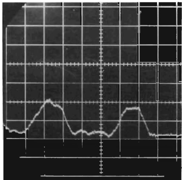
Figure 43. Strain Gage Load Cell No. 3, 1.87 in./sec Impact Velocity, PS=141 psig (50 lb/div; 0.0001 sec/div)
