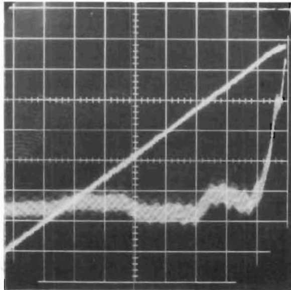
Figure 47. Control Pressure (PC) and Position, 1.87 in./sec Impact Velocity, PS = 141 psig (20 psi/div and 0.0125 in./div; 0.005 sec/div)
