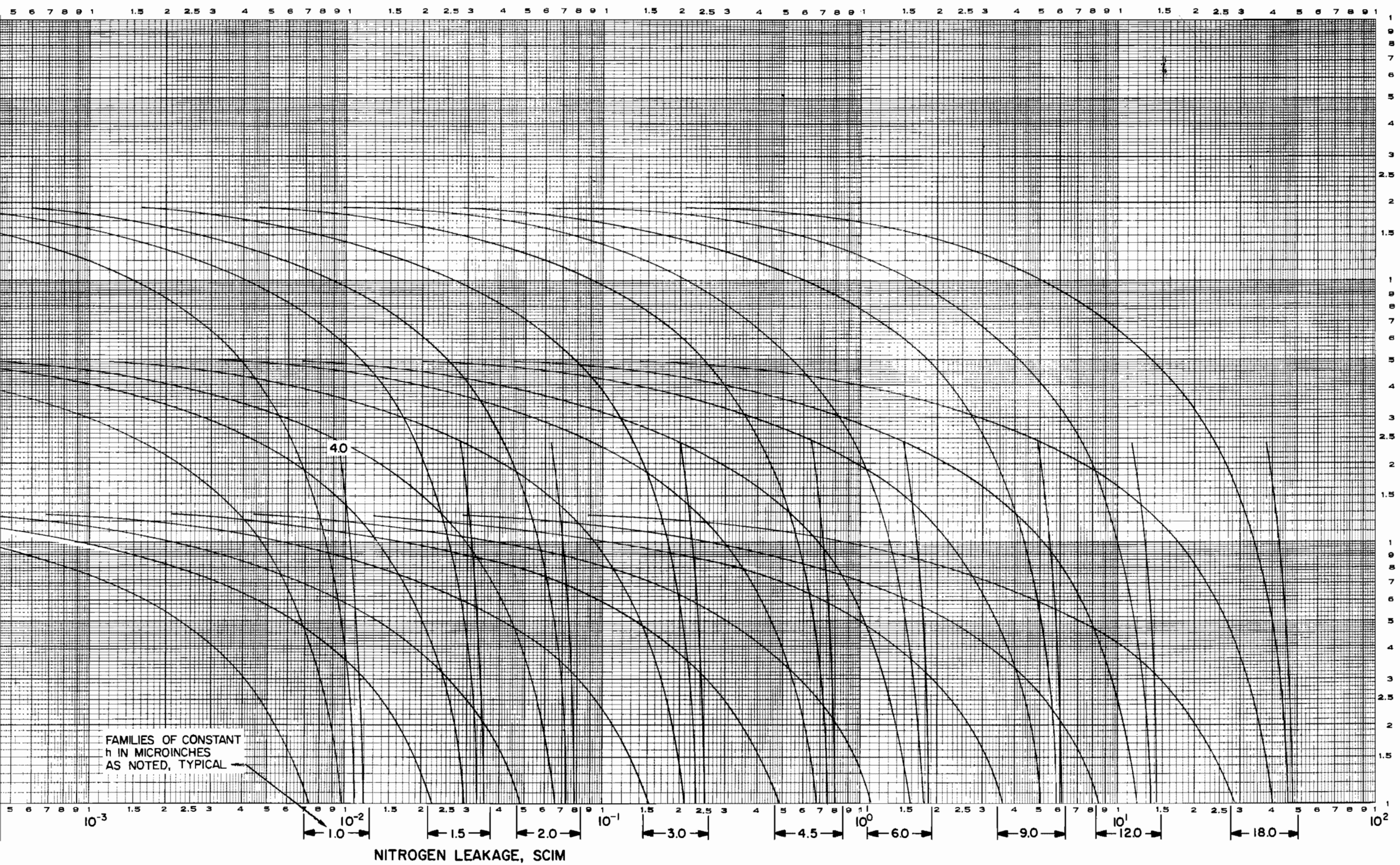
Figure 23. Theoretical Parametric Stress vs Leakage Curves for Aluminum
