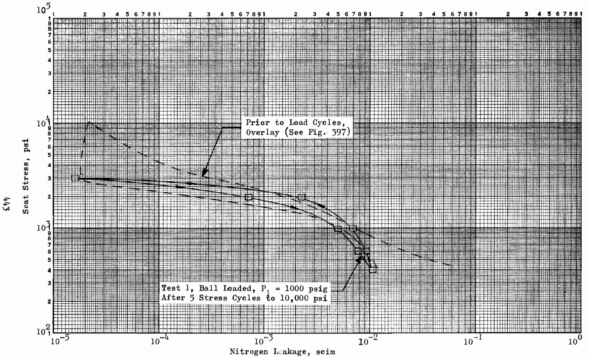
Figure 398. Stress-Leakage Data for Test Model S_f After Load Cycles, Test 1
