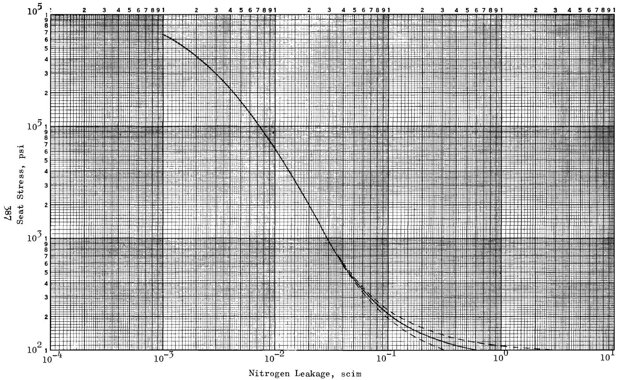
Figure 380. Error Band, Typical Stress-Leakage Curve
