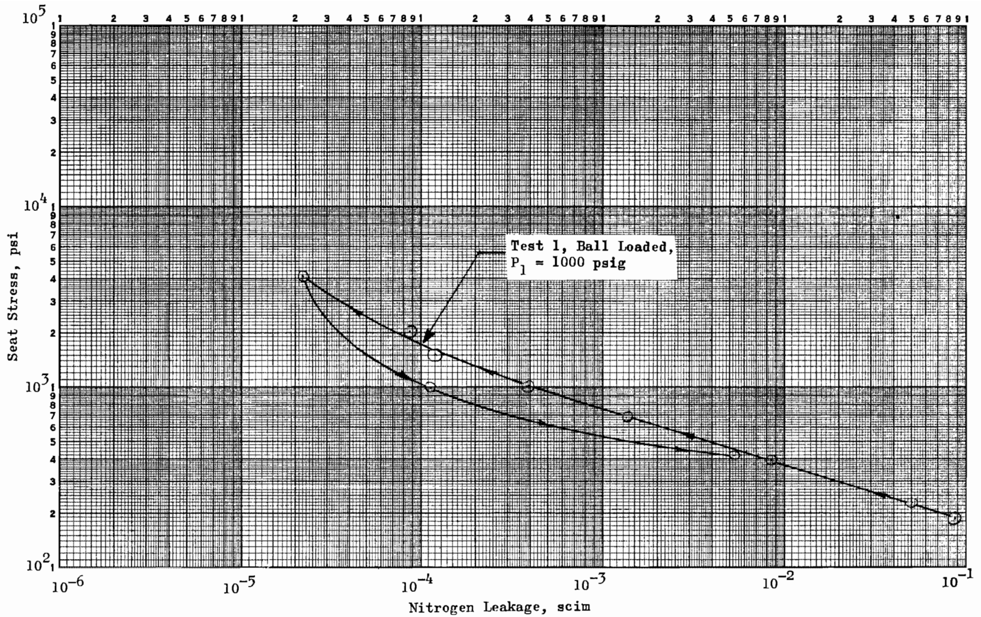
Figure 415. Stress-Leakage Data for Test Model H f , Test 1
