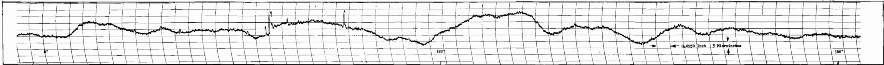
Figure 350. Test Model A c , Poppet Circumferential Roundness Profile Record, Midland, 1/16-Inch Ball Stylus
