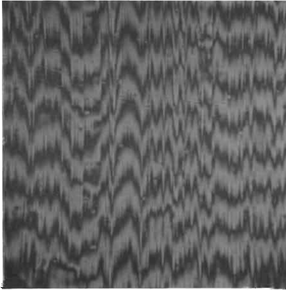
Figure 121. Test Model D f , Seat, 0.0065- x 0.0065-Inch Interference Photo, Tracks From 0.0001-Inch Radius Proficorder Stylus
