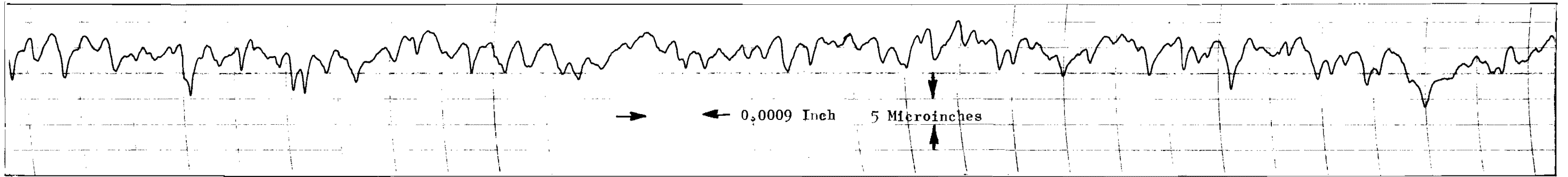
Figure 335. Test Model D f , Seat Roughness Profile Record, 0.0001-Inch Radius Stylus
