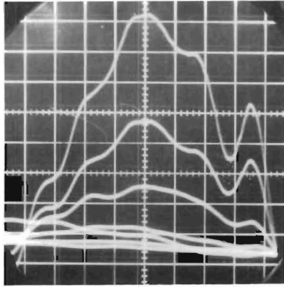
Figure 486. Test Model Y f , Piezo- electric Load Cell, ~ 24 in./sec Impact Velocity, PS = 169 psig (500 lb/div.; 0.00002 sec/div.)
