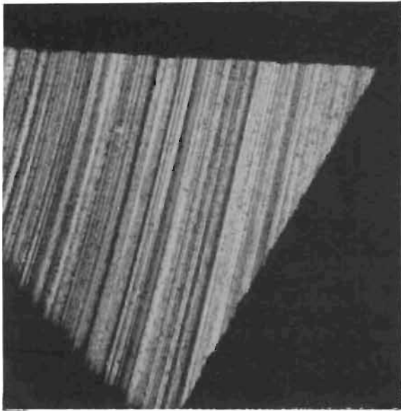
Figure 74. Sample 17-4 PH Cutting Tool No. 1, 0.033- x 0.033-Inch Plain Photo Showing Top Face As-Ground
