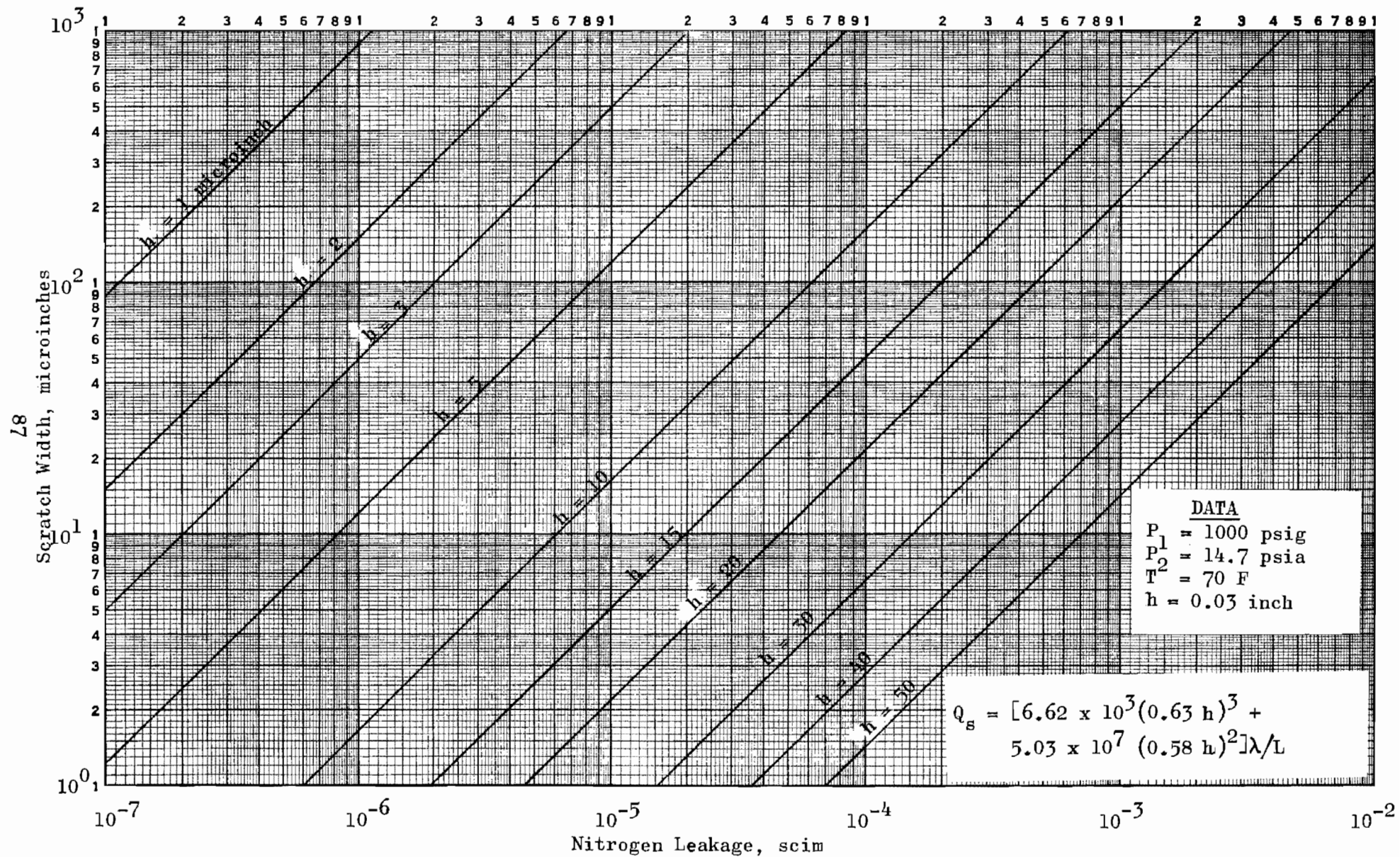
Figure 18. Single Scratch Leakage, Q_s
