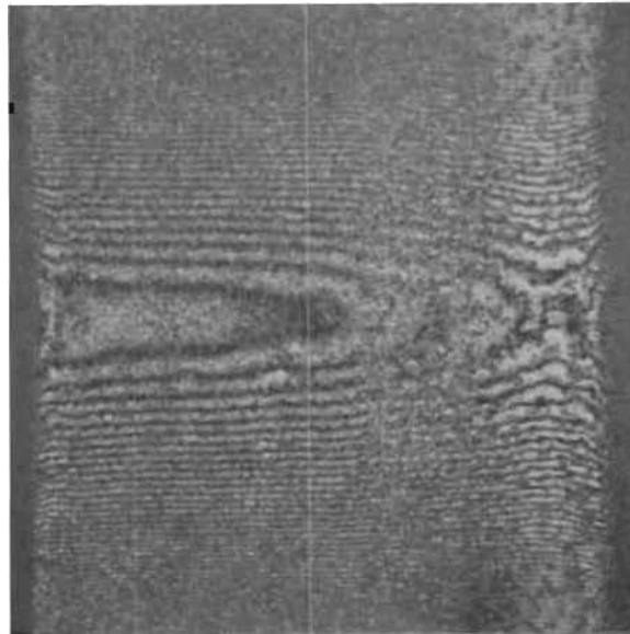
Figure 236. Test Model G_{c1} , Seat, 0.033- x 0.033-Inch Interference Photo Showing Plastic Deformation at ID And OD
