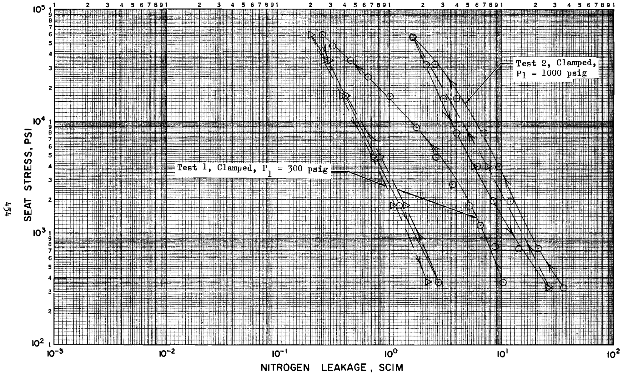
Figure 403. Stress-Leakage Data for Test Model C, Tests 1 and 2
