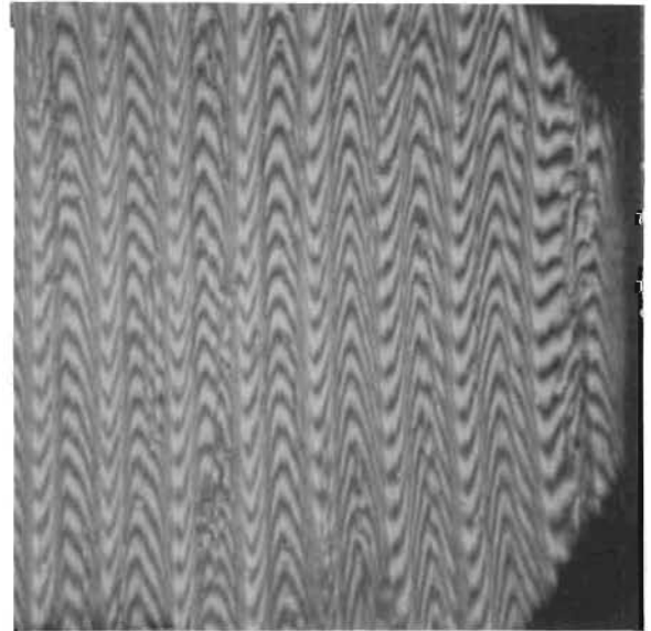
Figure 108. Test Model Q f , Seat, 0.0065- x 0.0065-Inch Interference Photo, OD Plastic Deformation at Right
