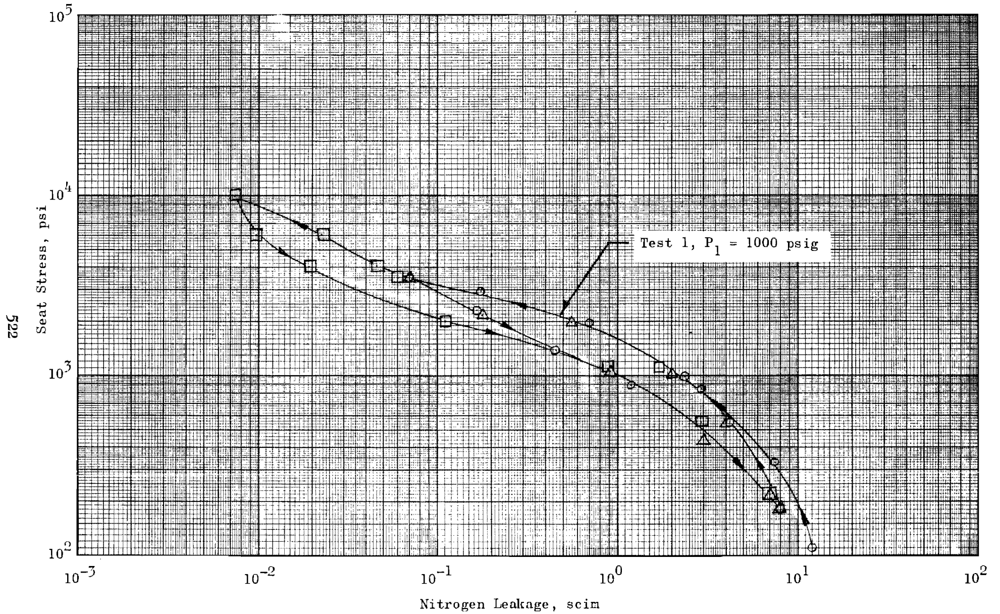
Figure 430. Stress-Leakage Data for Test Model B_c , Test 1
