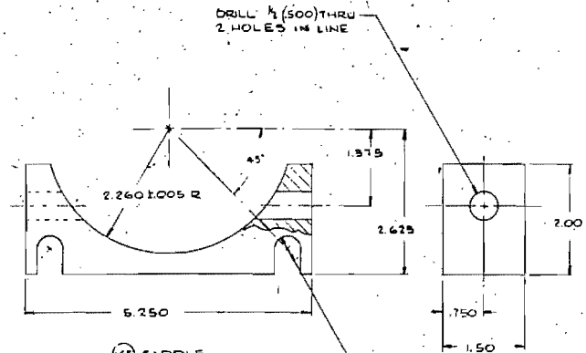
(65) SADDLE
