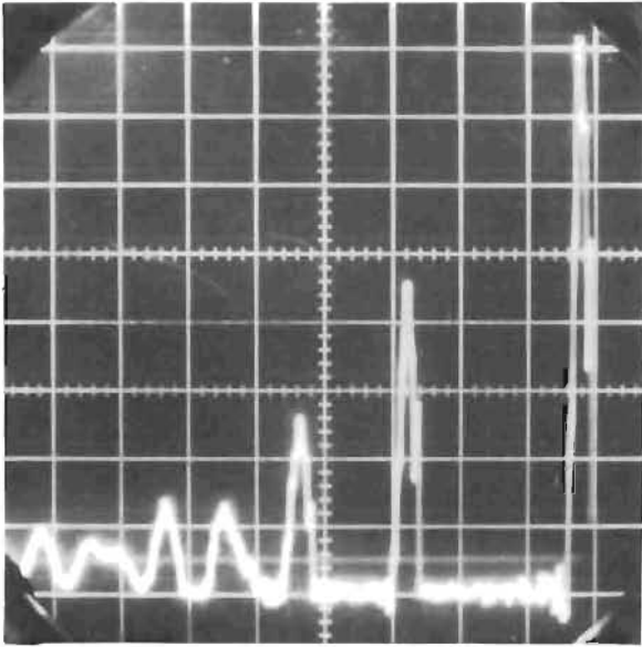
Figure 490. Test Model P f , Piezo- electric Load Cell, ~ 24 in./sec Impact Velocity, PS = 169 psig (500 lb/div.; 0.0005 sec/div.)
