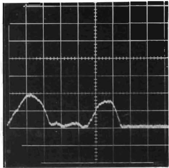
Figure 41. Strain Gage Load Cell No. 1, 1.87 in./sec Impact Velocity, PS=141 psig (50 lb/div; 0.0001 sec/div)
