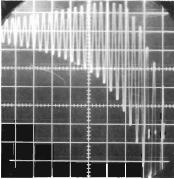
Figure 48. Piezoelectric Load Cell, 1.77 in./sec Impact Velocity, PS = 272 psig (50 lb/div; 0.001 sec/div)
