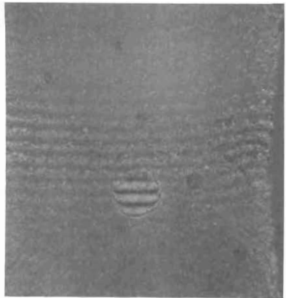
Figure 270. Test Model W_{f1} , Seat, 0.033- x 0.033-Inch Interference Photo Showing Plating Void, White Light (Posttest)
