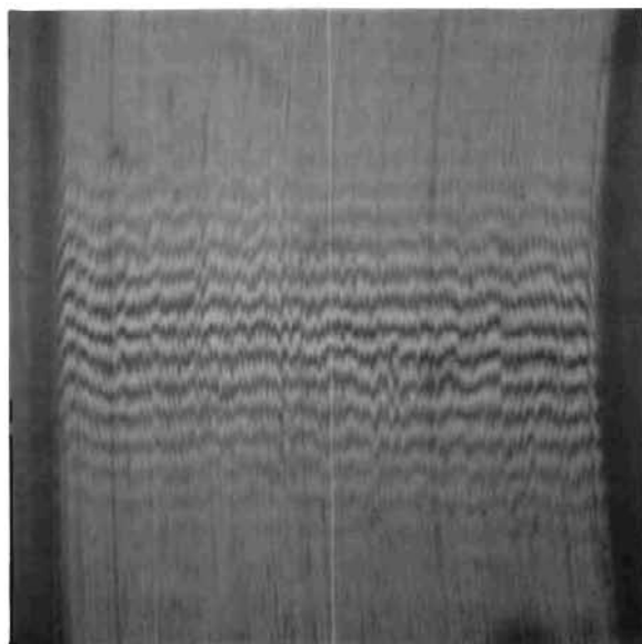
Figure 208. Test Model NN_f , Poppet, 0.033- x 0.033-Inch Interference Photo, White Light
