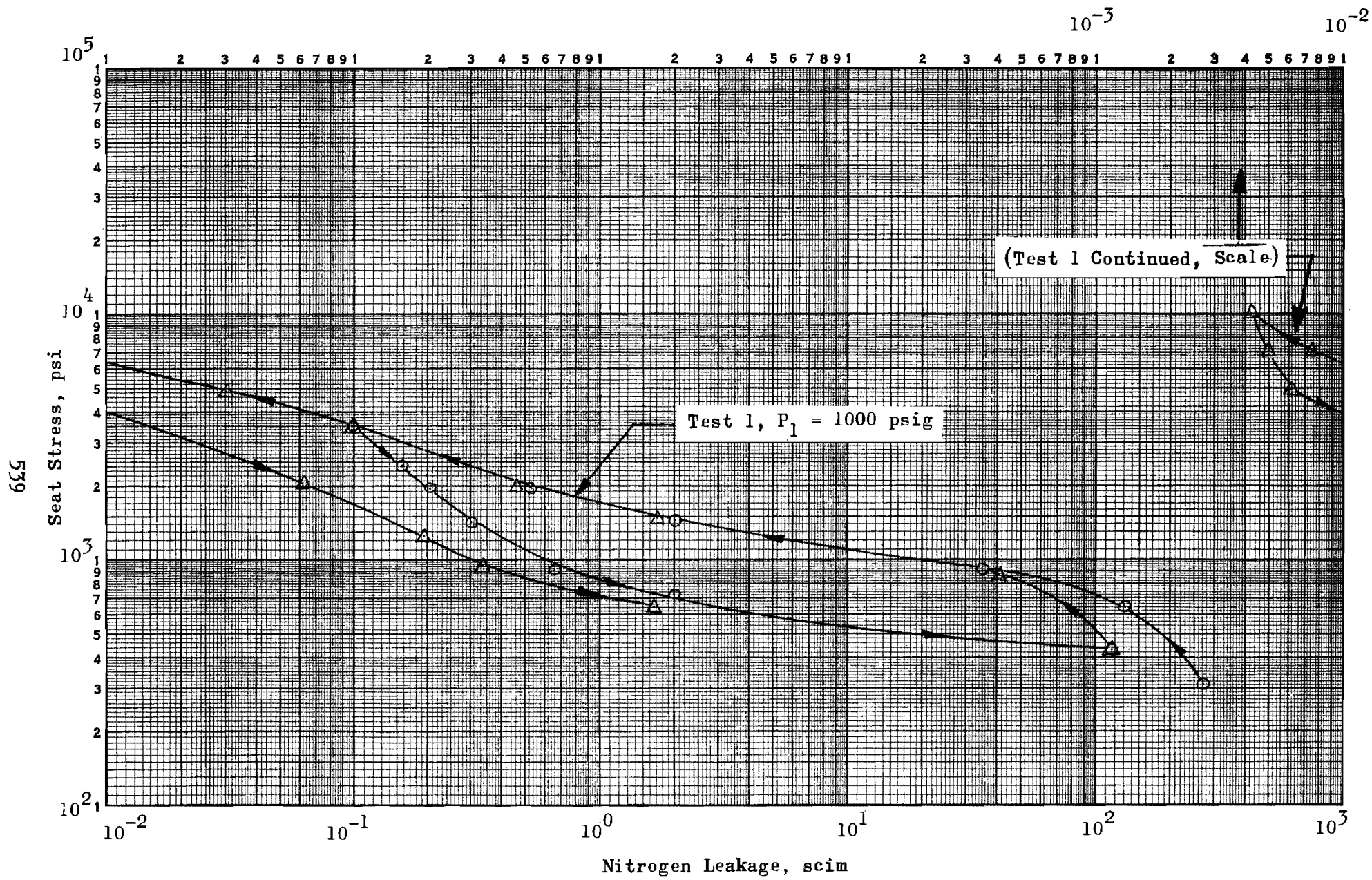
Figure 437. Stress-Leakage Data for Test Model B_s , Test 1
