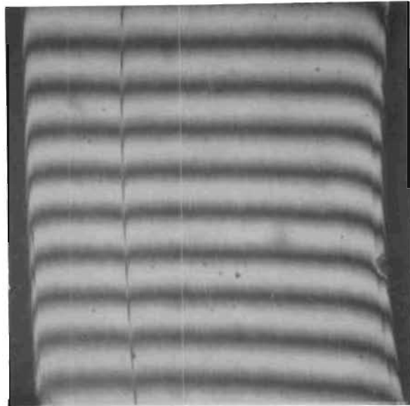
Figure 182. Test Model H f1 , Seat, 0.033- x 0.033-Inch Interference Photo
