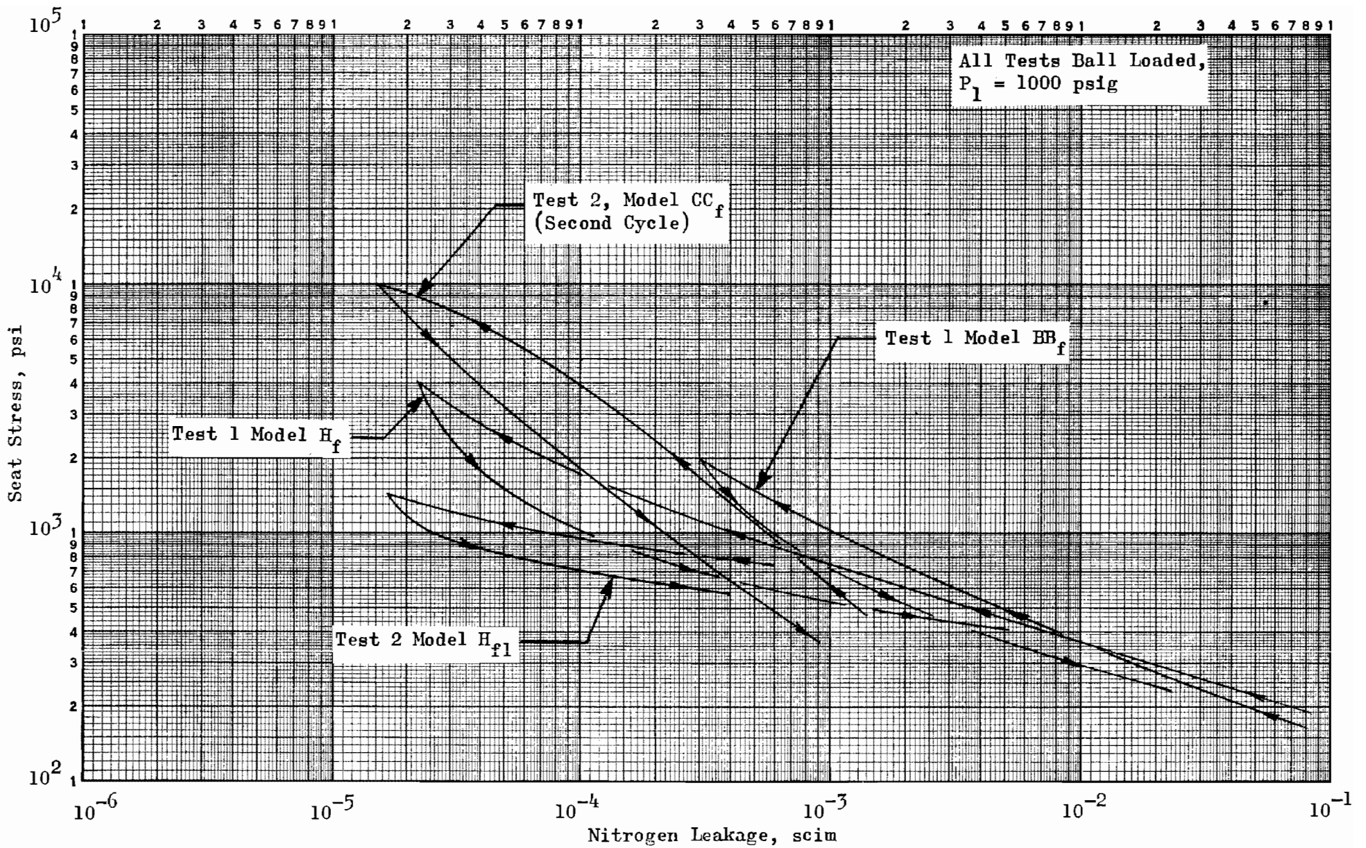
Figure 420. Stress-Leakage Data for Test Models BB_f , CC_f , H_f and H_{f1}
