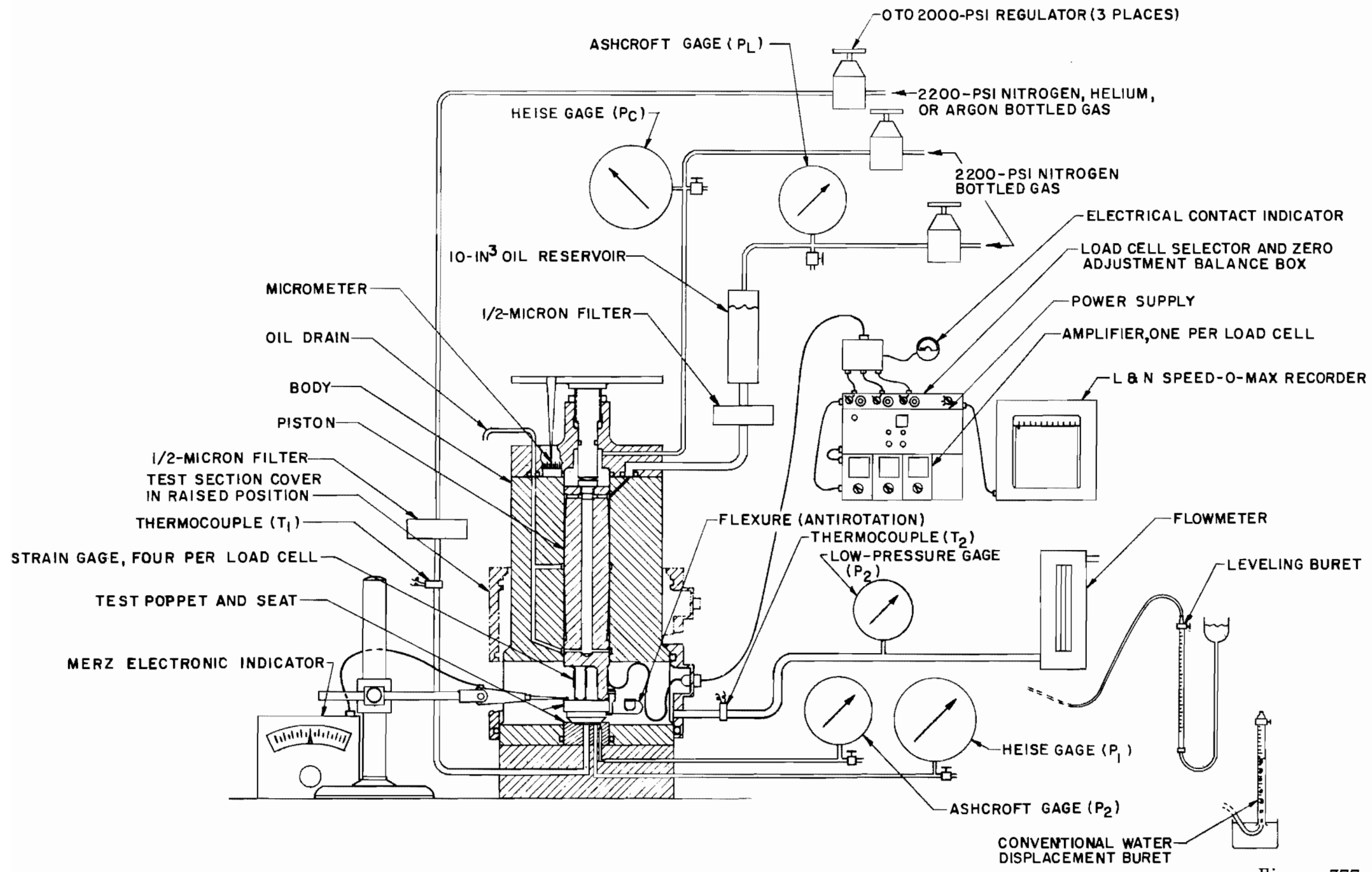
Figure 377. Static Test Setup Schematic (Initial Contract Effort)
