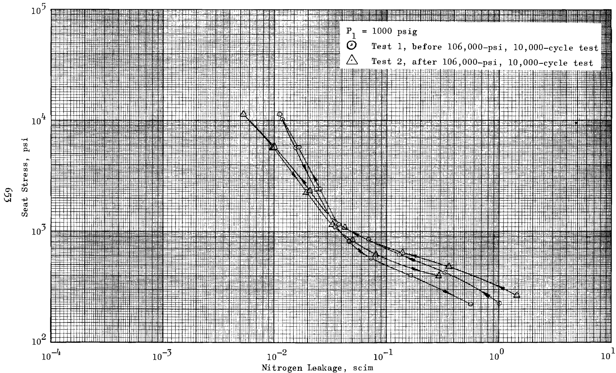
Figure 492. Stress-Leakage Data for Cycle Test Model P_f , Tests 1 and 2
