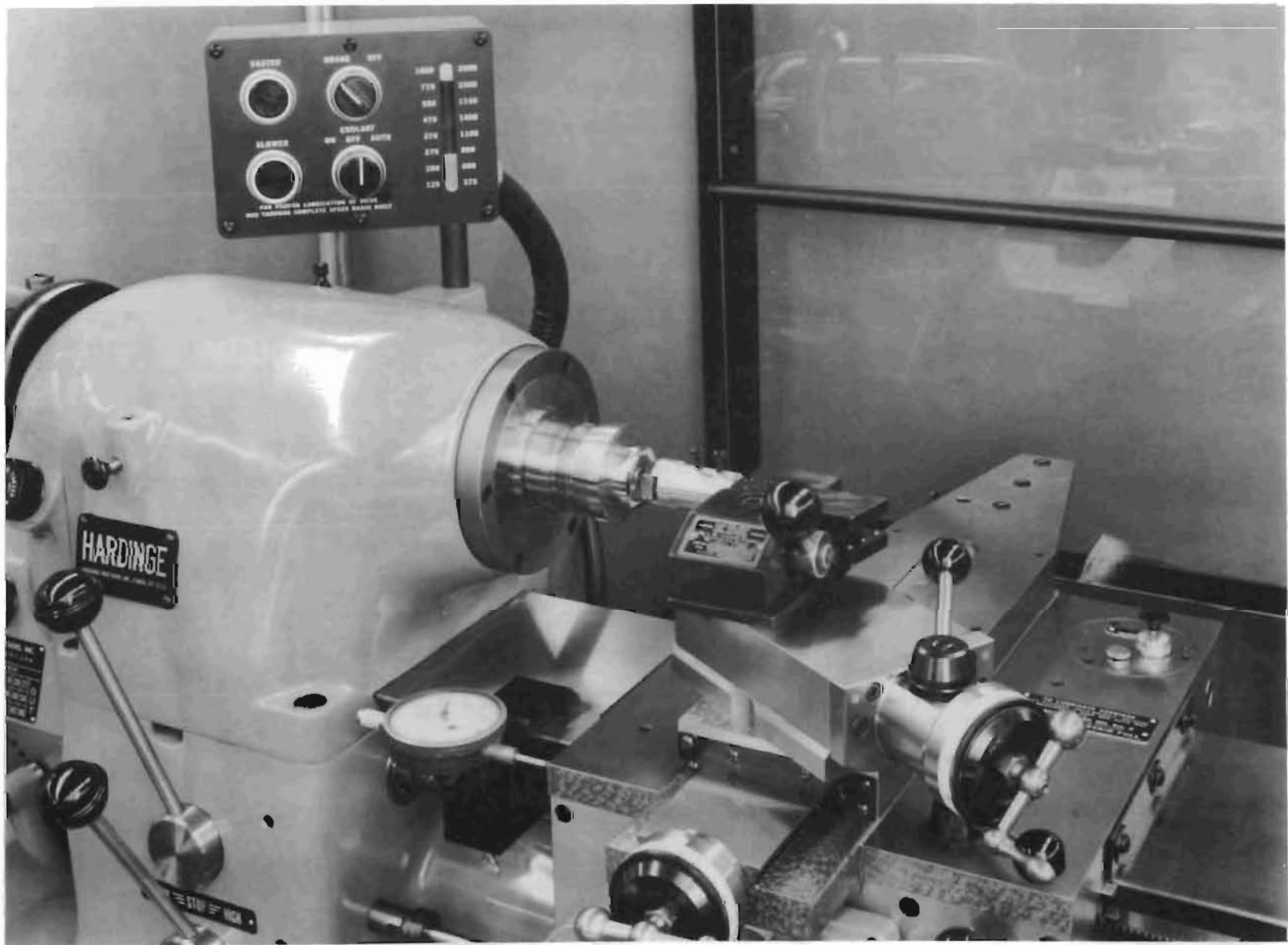
Figure 81. Lathe Setup for Circular Lay Lapping Flat Surfaces
