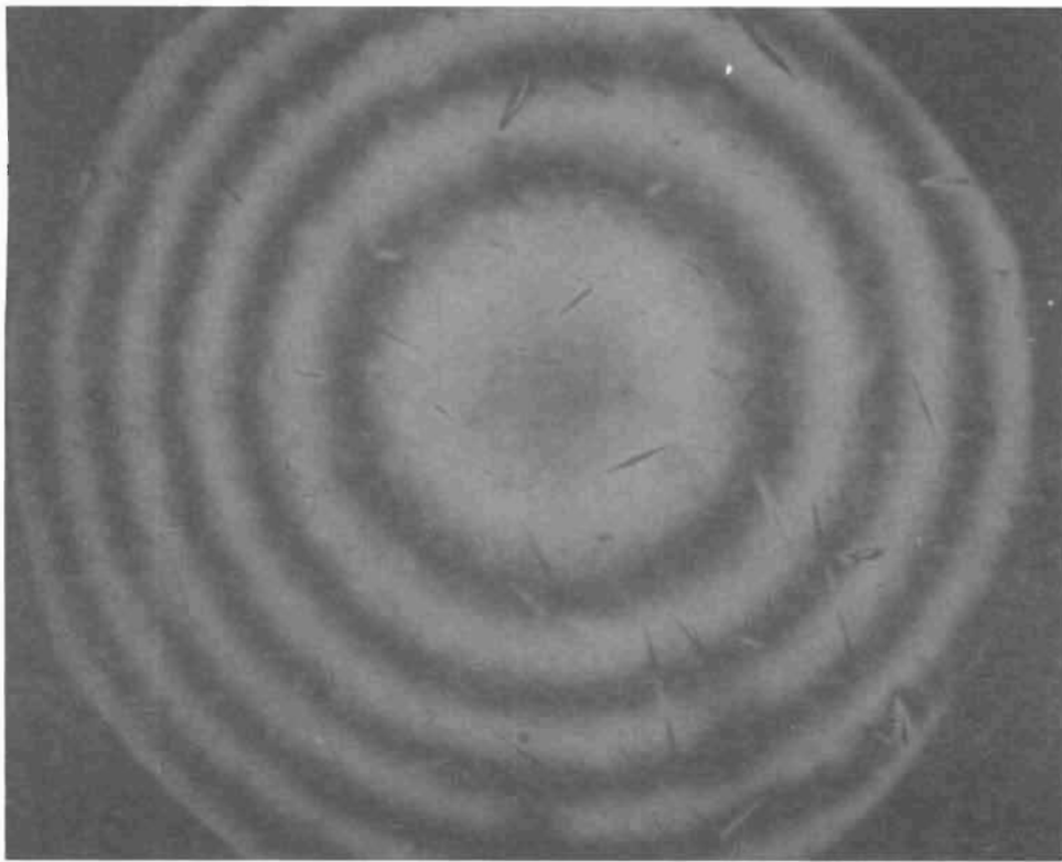
Figure 249. Test Model C s , Poppet, 0.0089- x 0.0110-Inch Interference Photo at \theta = 35 Degrees
