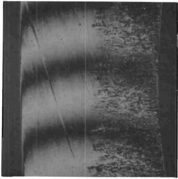
Figure 150. Test Model G f1 , Seat, 0.033- x 0.033-Inch Interference Photo, Same Location as Fig. 147
