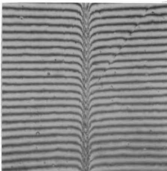
Figure 286. Test Model G, Poppet, 0.0065- x 0.0065-Inch Interference Photo, Narrow Bandwidth Showing Test Scratch
