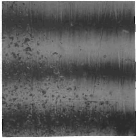
Figure 254. Test Model I_{f1} , Poppet, 0.0065- x 0.0065-Inch Interference Photo Showing Transition From Lapped to Liquid Honed Surface
