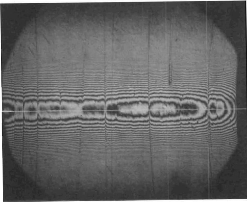
Figure 224. Test Model C c , Poppet, 0.045- x 0.056-Inch Interference Photo at ID
