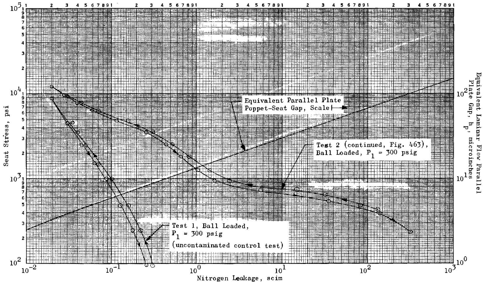
Figure 464. Stress-Leakage Data for Test Model L (Lead Contaminants), Tests 2 (continued) and 1
