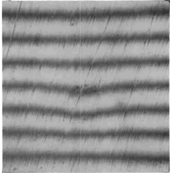
Figure 290. Test Model L, Seat, 0.033- x 0.033-Inch Interference Photo Showing Plastic Deformation at Area of Lead Particle 3
