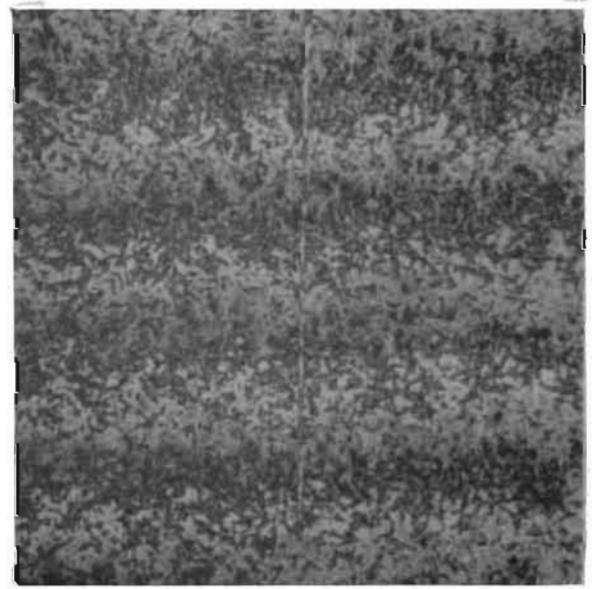
Figure 132. Test Model J, Poppet, 0.0065- x 0.0065-Inch Interference Photo Showing 0.0001-Inch Radius Proficorder Stylus Scratch
