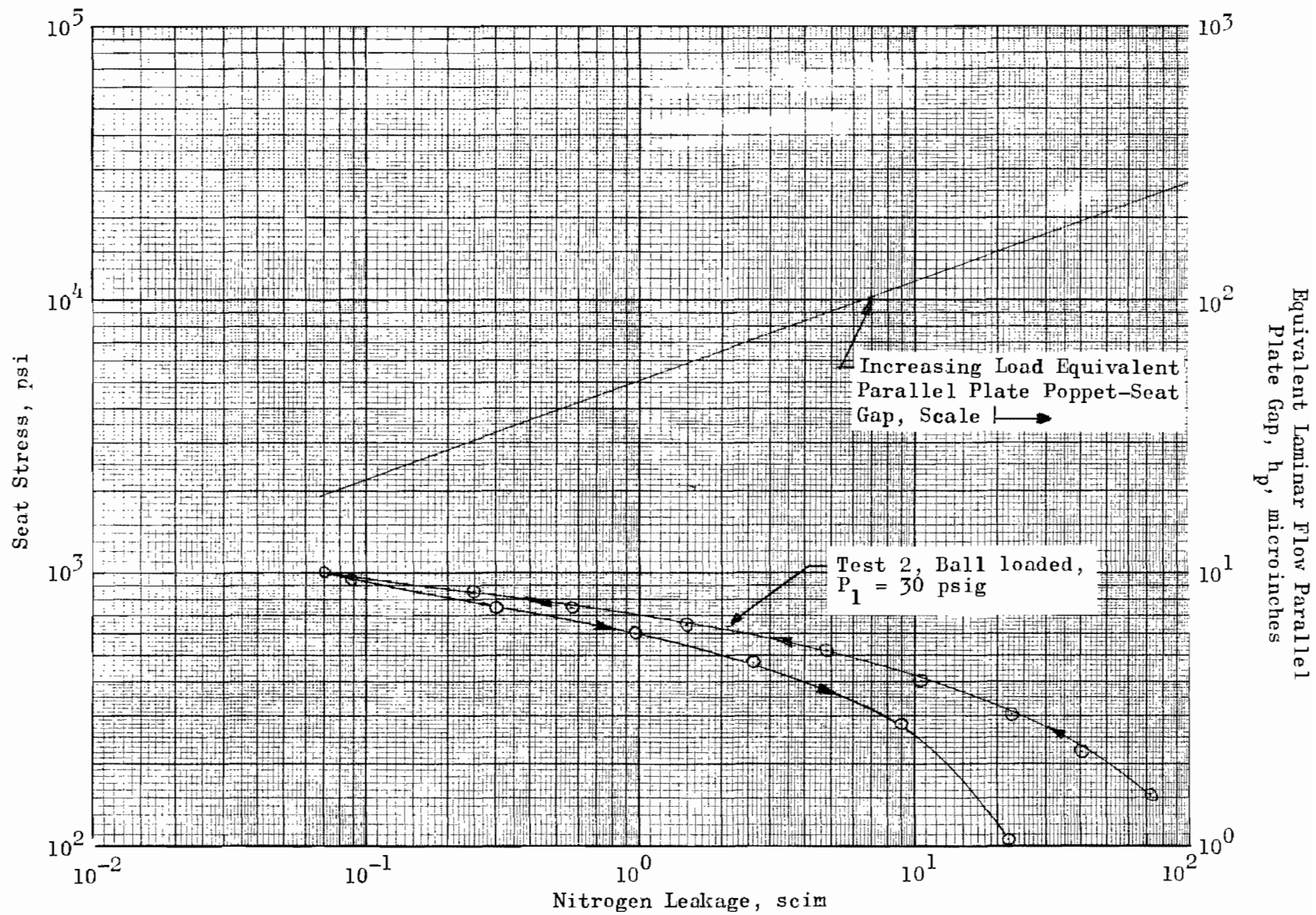
Figure 463. Stress-Leakage Data for Test Model L (Lead Contaminants), Test 2
