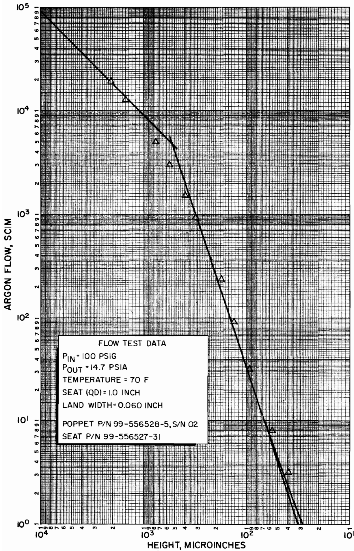
Figure 386. Argon Flow Data, Part 1
