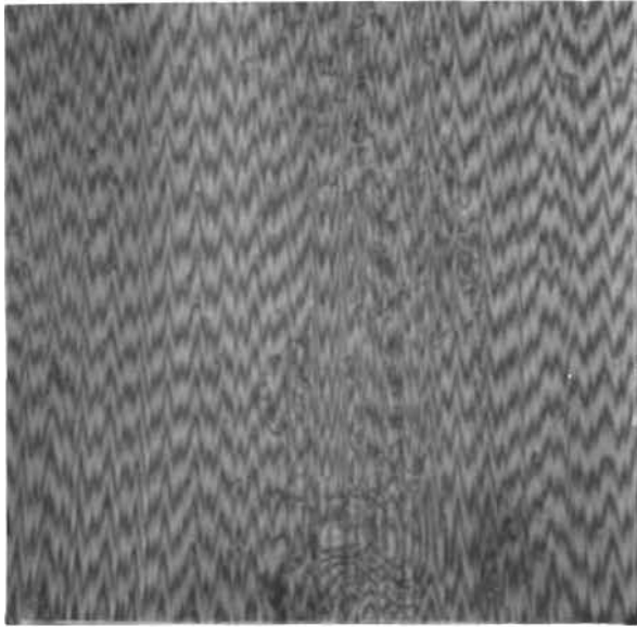
Figure 117. Test Model S_f , Seat, 0.0065- x 0.0065-Inch Interference Photo Showing Plastic Deformation
