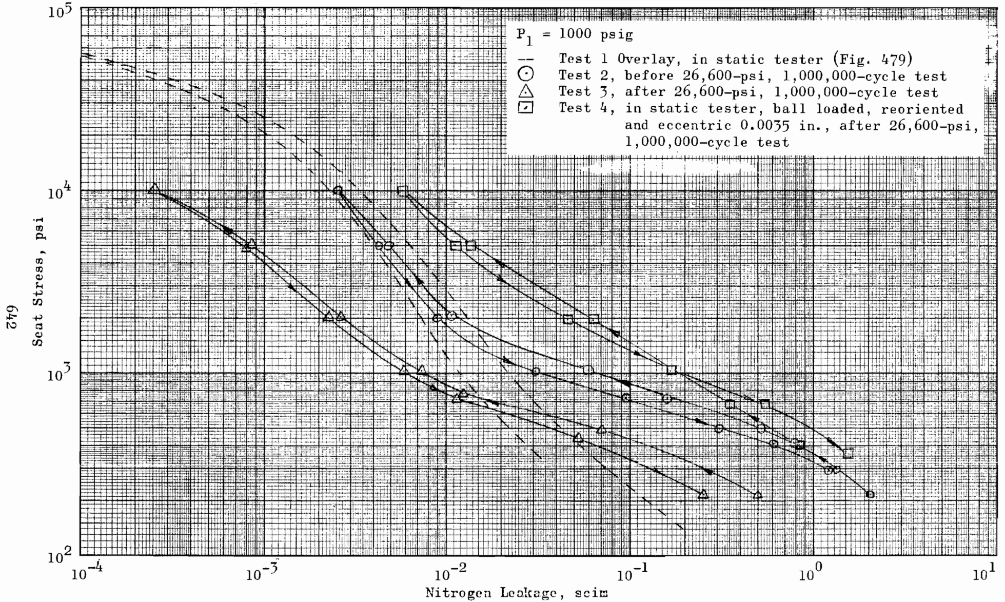
Figure 483. Stress-Leakage Data for Cycle Test Model X_f , Tests 2, 3, and 4
