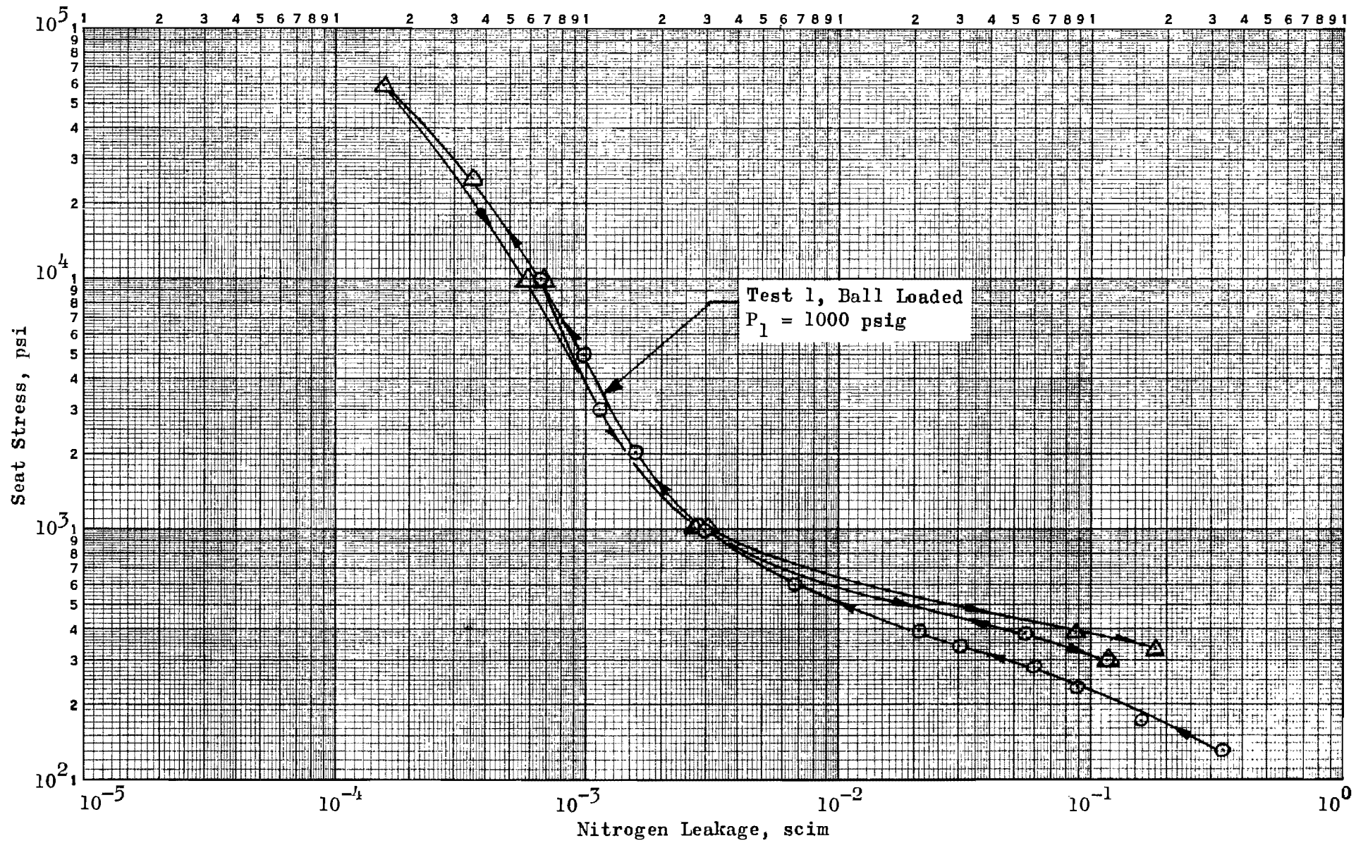
Figure 418. Stress-Leakage Data for Test Model L_f , Test 1
