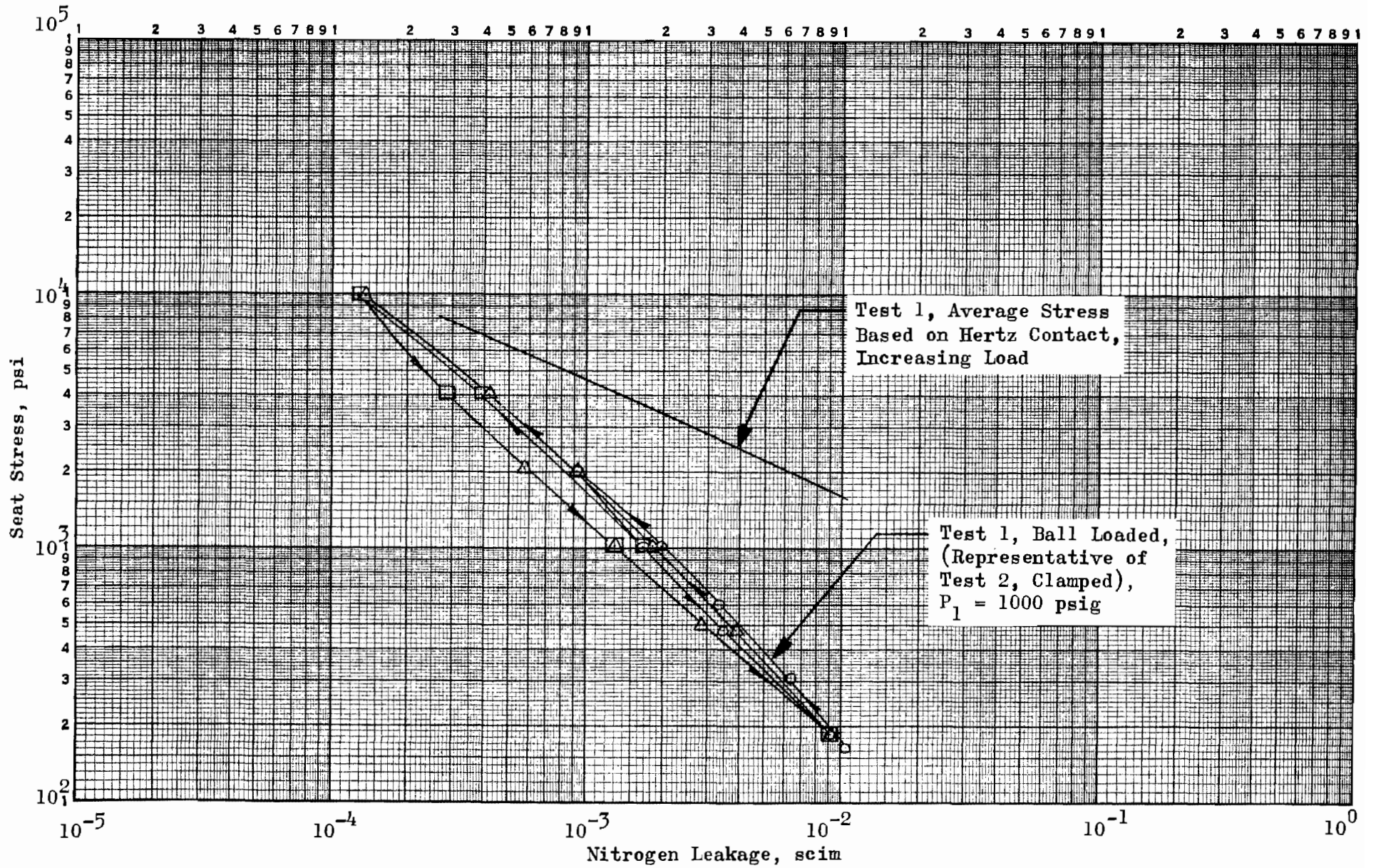
Figure 423. Stress-Leakage Data for Test Model AA f , Test 1
