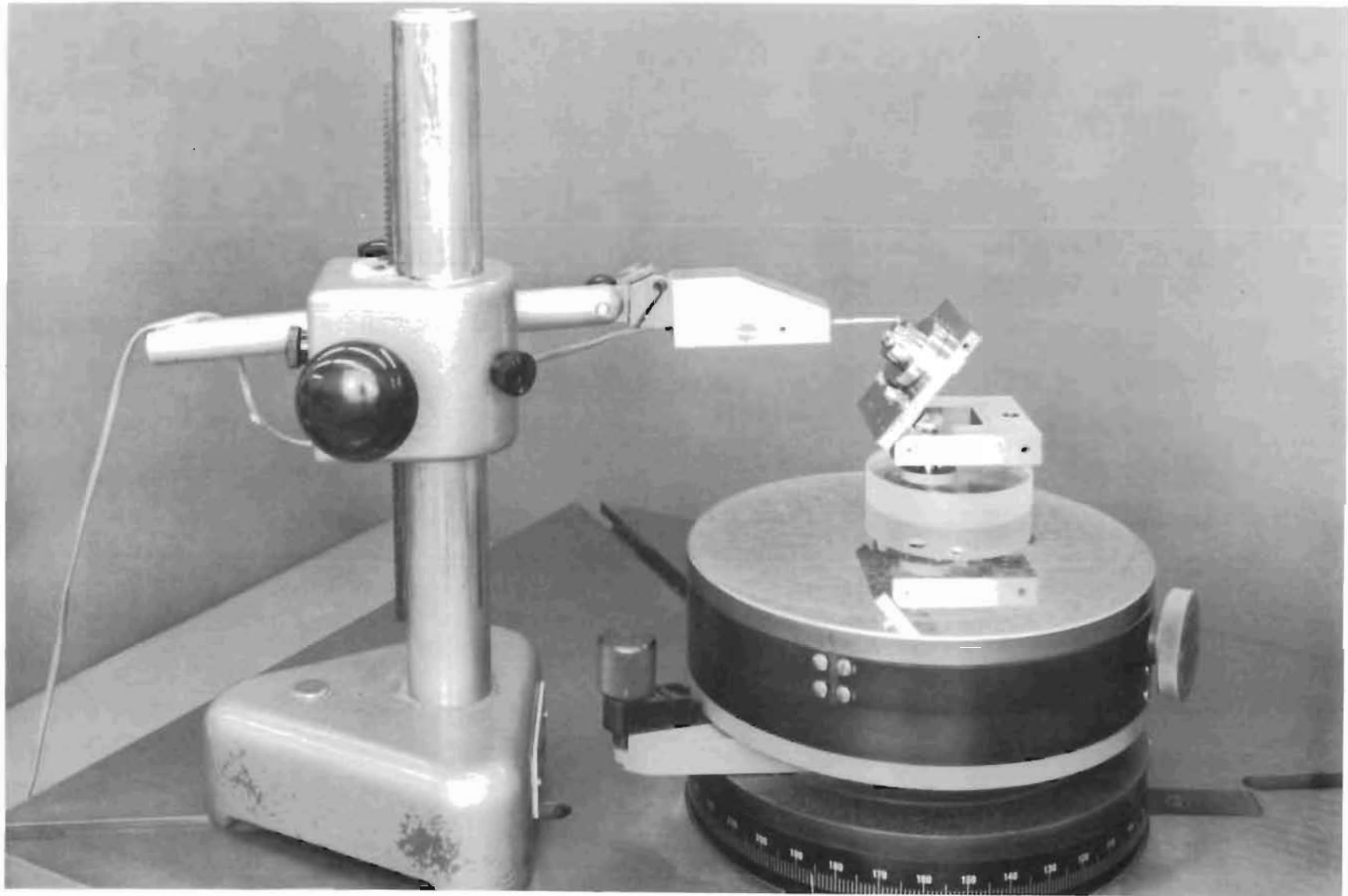
Figure 88. Proficorder Indicating Conical Poppet Seating Land
