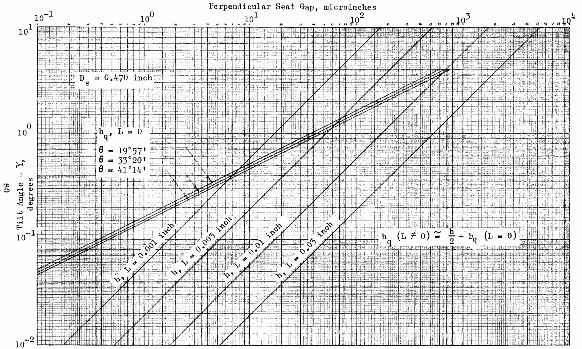
Figure 14. Tilted Conical Poppet-Seat Gap
