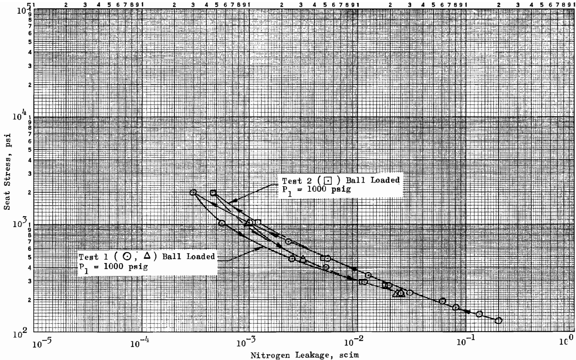
Figure 419. Stress-Leakage Data for Test Model BB_f , Tests 1 and 2
