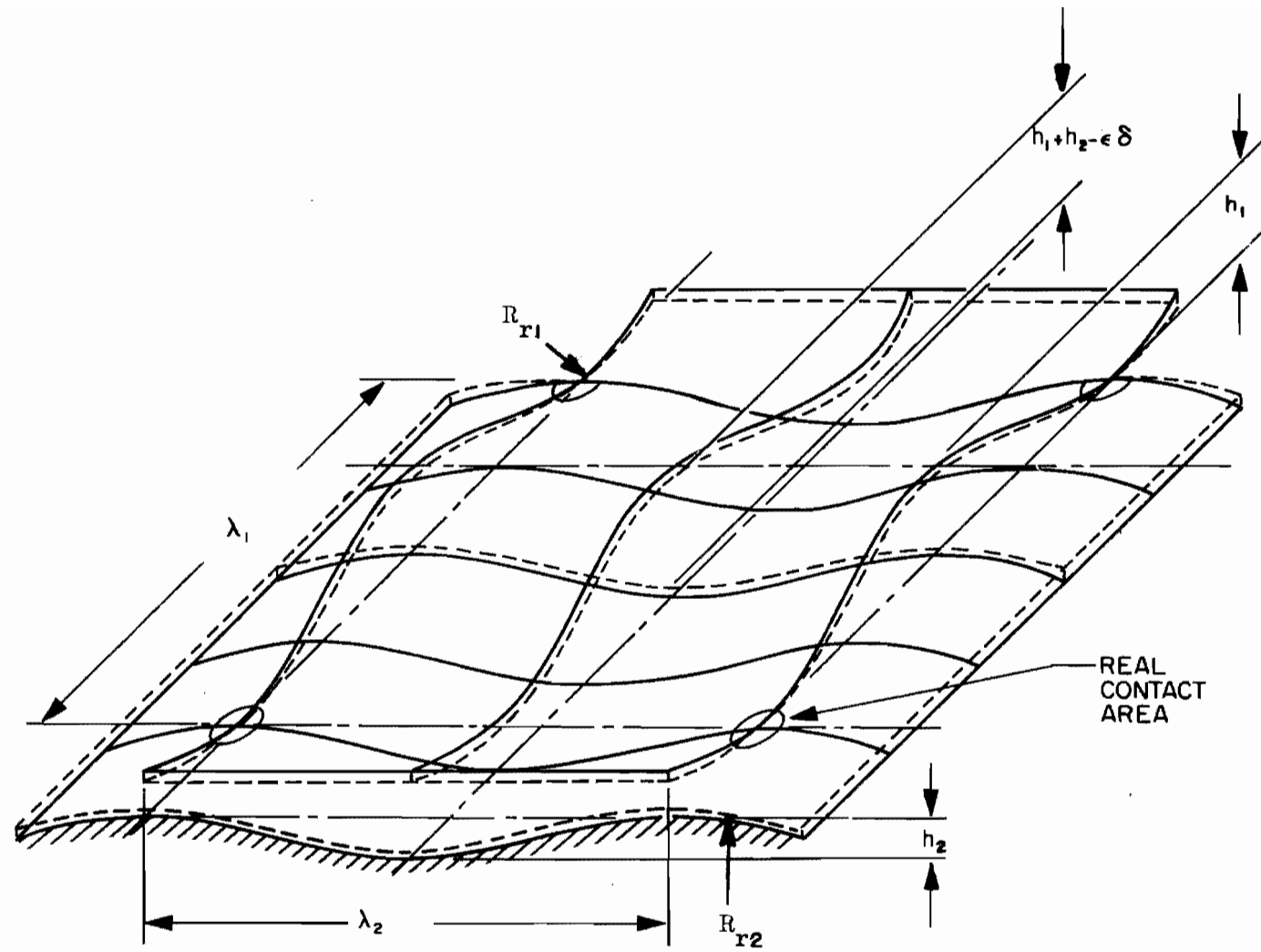
Figure 19. Sinusoidal Model Surfaces
