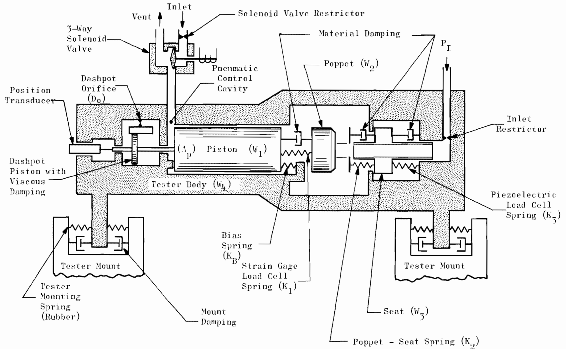
Figure 38. Cycle Tester Schematic
