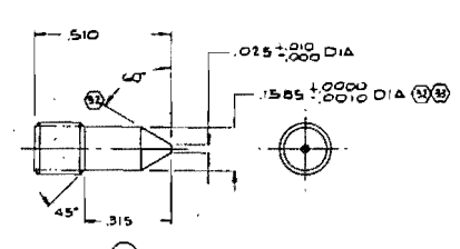
(59) LOCK PIN
