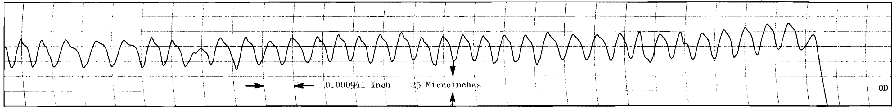
Figure 329. Test Model Q f , Seat Cross Lay Roughness Profile Record, 0.0001-Inch Radius Stylus
