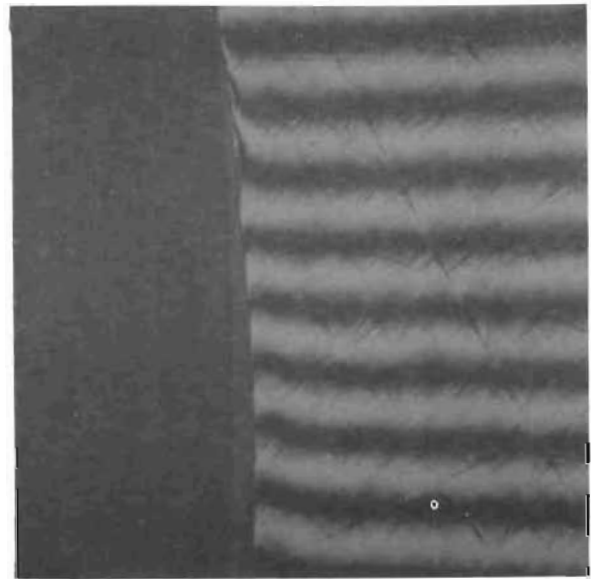
Figure 246. Test Model B S , Seat, 0.033- x 0.033-Inch Interference Photo Normal to ID Showing Handling Damage
