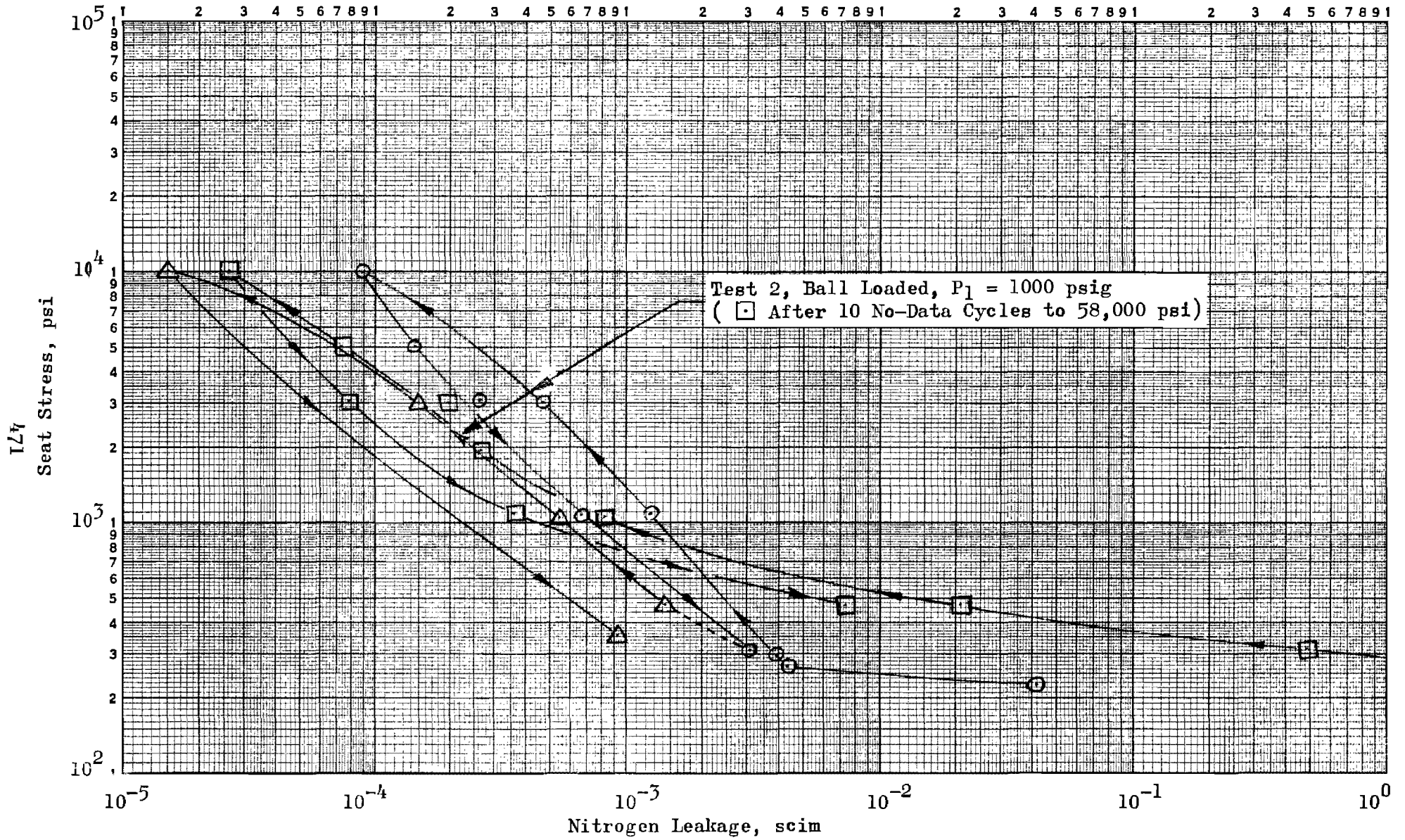
Figure 412. Stress-Leakage Data for Test Model CC f , Test 2
