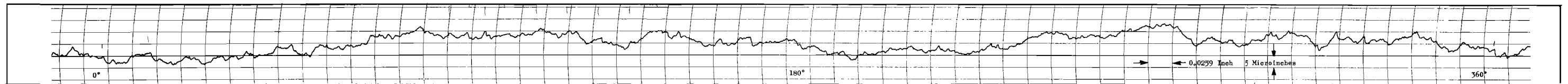
Figure 362. Test Model E c , Seat Circumferential Roundness Profile Record, Midland, 1/16-Inch Ball Stylus
