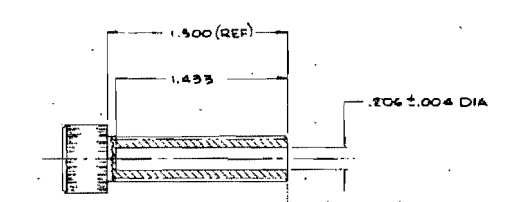
(55) REGULATOR SCREW
