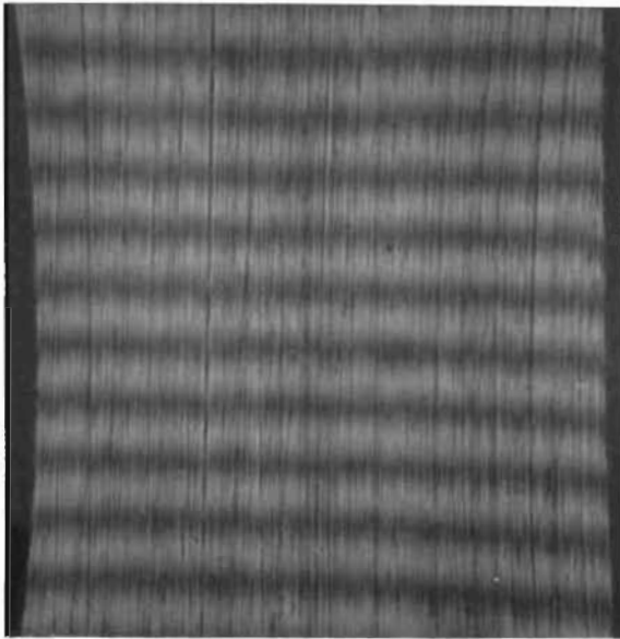
Figure 145. Test Model G_f , Seat, 0.033- x 0.033-Inch Interference Photo
