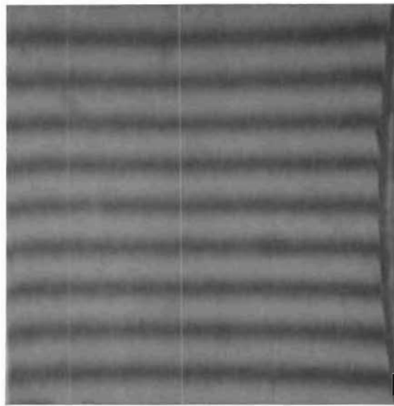
Figure 298. Test Model X_f , Seat, 0.033- x 0.033-Inch Interference Photo
