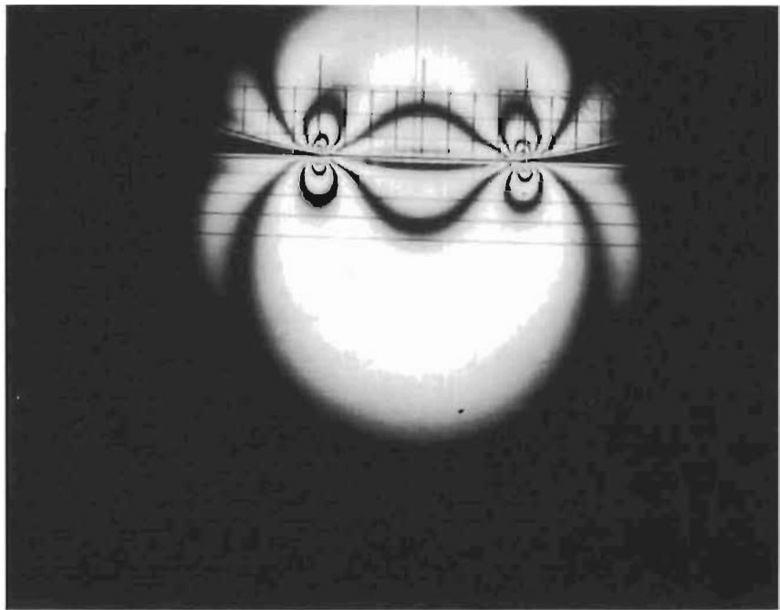
Figure 32. Magnified View of Isochromatics Near Contact Surface
