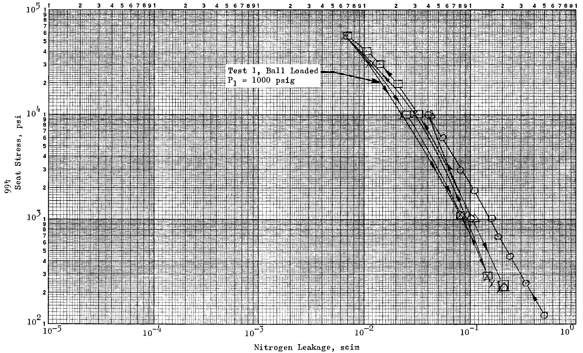
Figure 409. Stress-Leakage Data for Test Model G_f , Test 1
