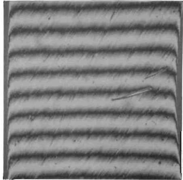
Figure 304. Test Model Y_f , Seat, 0.033- x 0.033-Inch Interference Photo Showing Lapping Scratch
