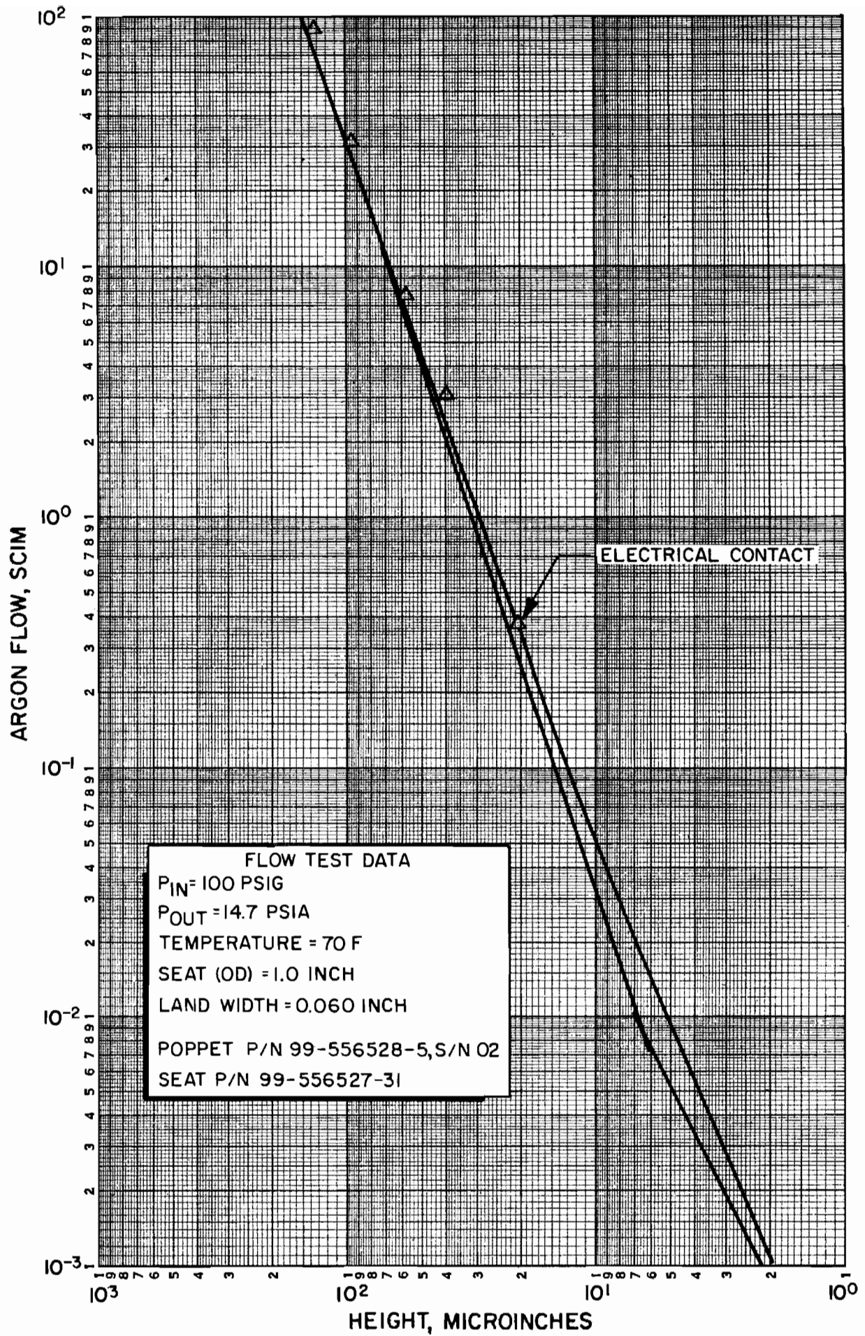
Figure 387. Argon Flow Data, Part 2
