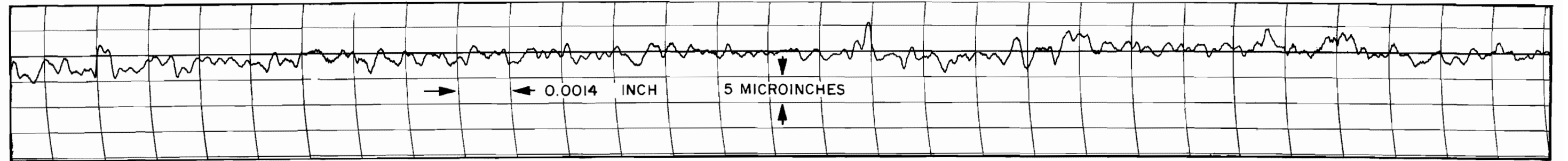
Figure 344. Test Model B, Poppet Roughness Profile Record, 0.0001-Inch Radius Stylus
