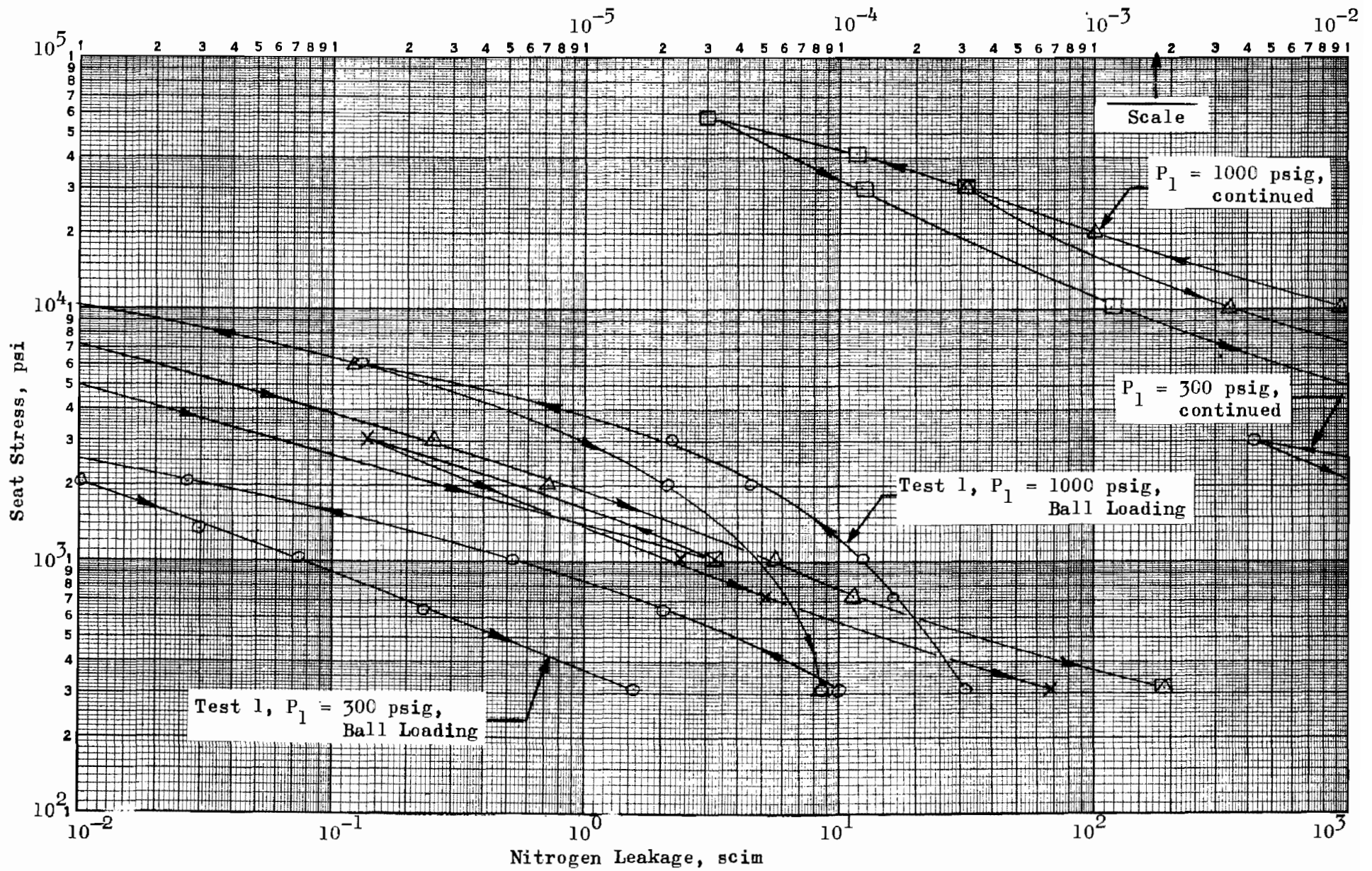
Figure 393. Stress-Leakage Data for Test Model N_f , Test 1
