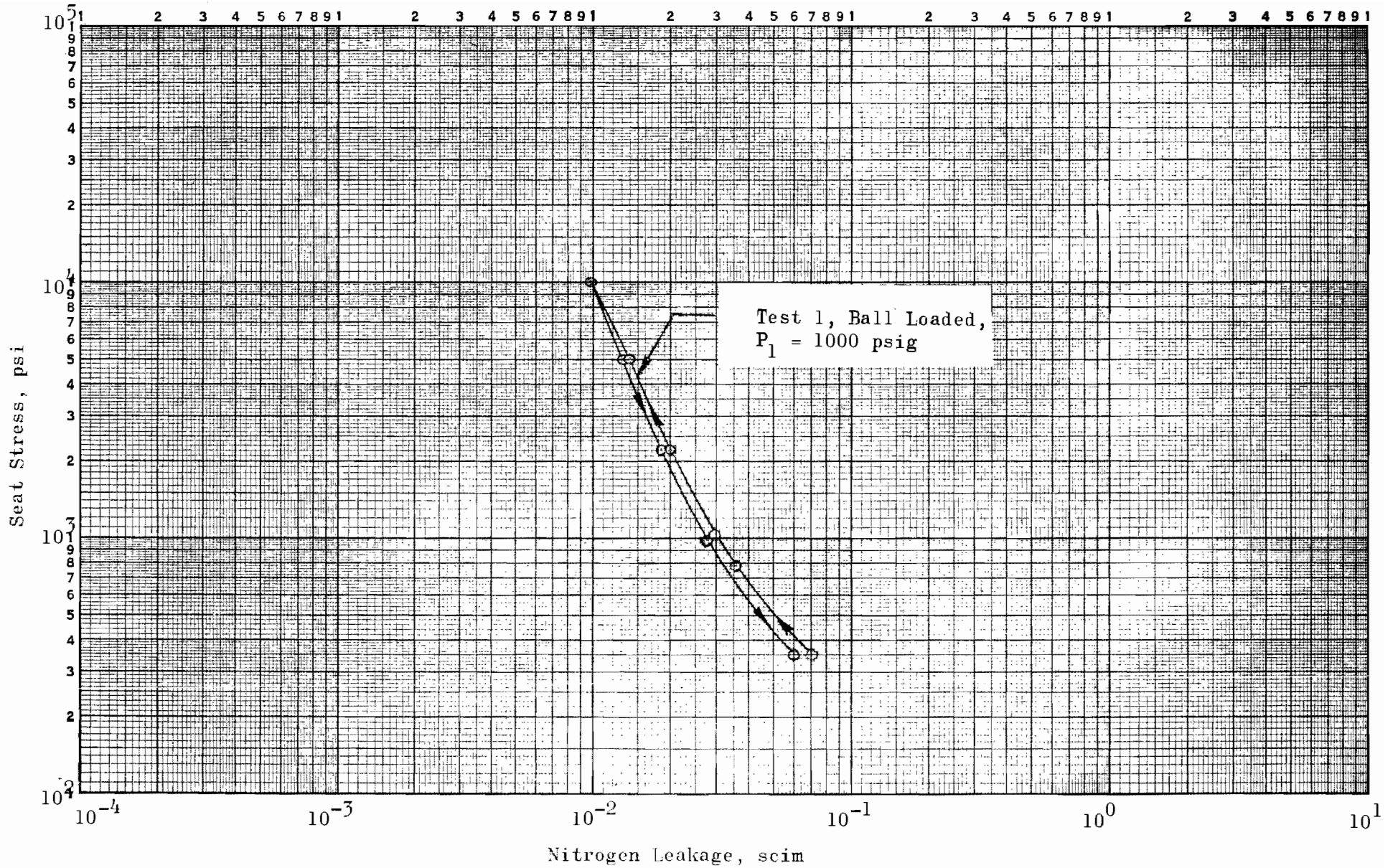
Figure 449. Stress-Leakage Data for Test Model W f , Test 1
