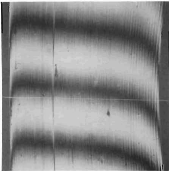
Figure 215. Test Model HH_f , Seat, 0.033- x 0.033-Inch Interference Photo
