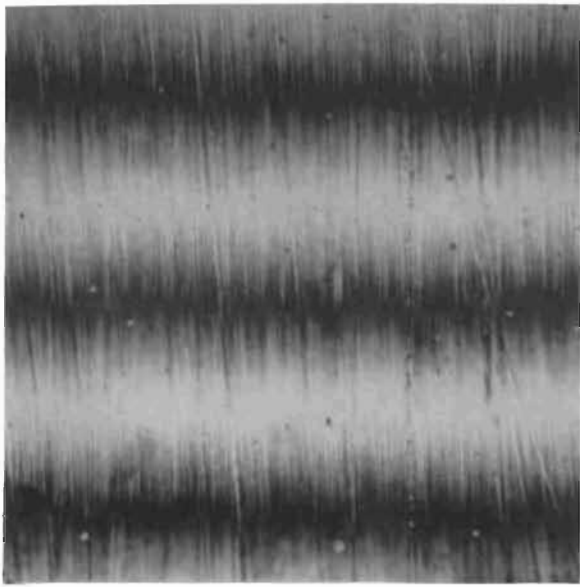
Figure 149. Test Model G f1 , Poppet, 0.0065- x 0.0065-Inch Interference Photo
