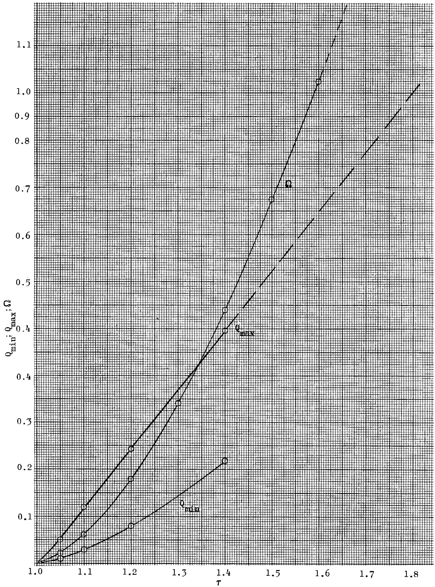
Figure 29. Contact Stress Function for Dubbed Seat
