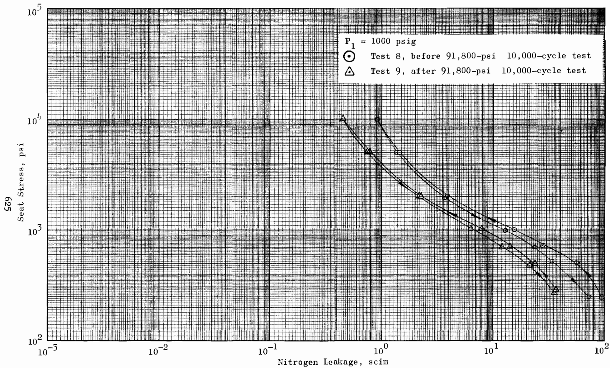
Figure 472. Stress Leakage Data for Cycle Test Model D_f , Tests 8 and 9
