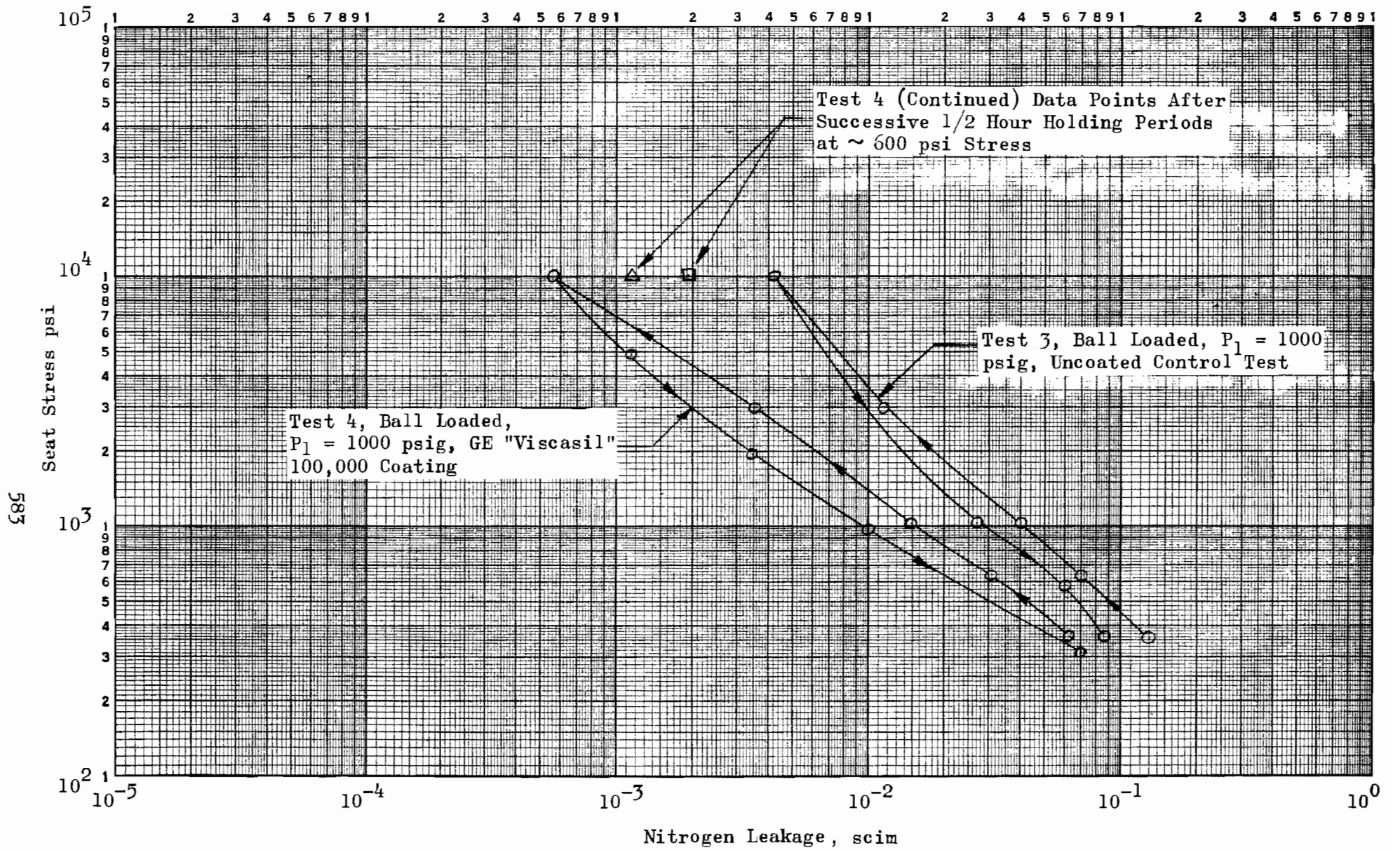
Figure 456. Stress-Leakage Data for Test Model J_{f1} , Tests 3 and 4
