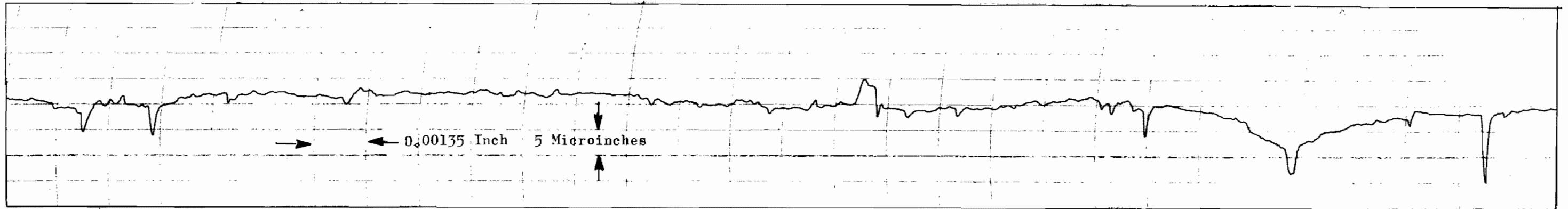
Figure 367. Test Model A s , Poppet Roughness Profile Record, 0.0001-Inch Radius Stylus
