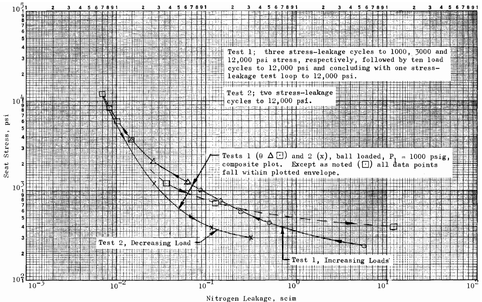
Figure 447. Stress-Leakage Data for Test Model U_f , Tests 1 and 2
