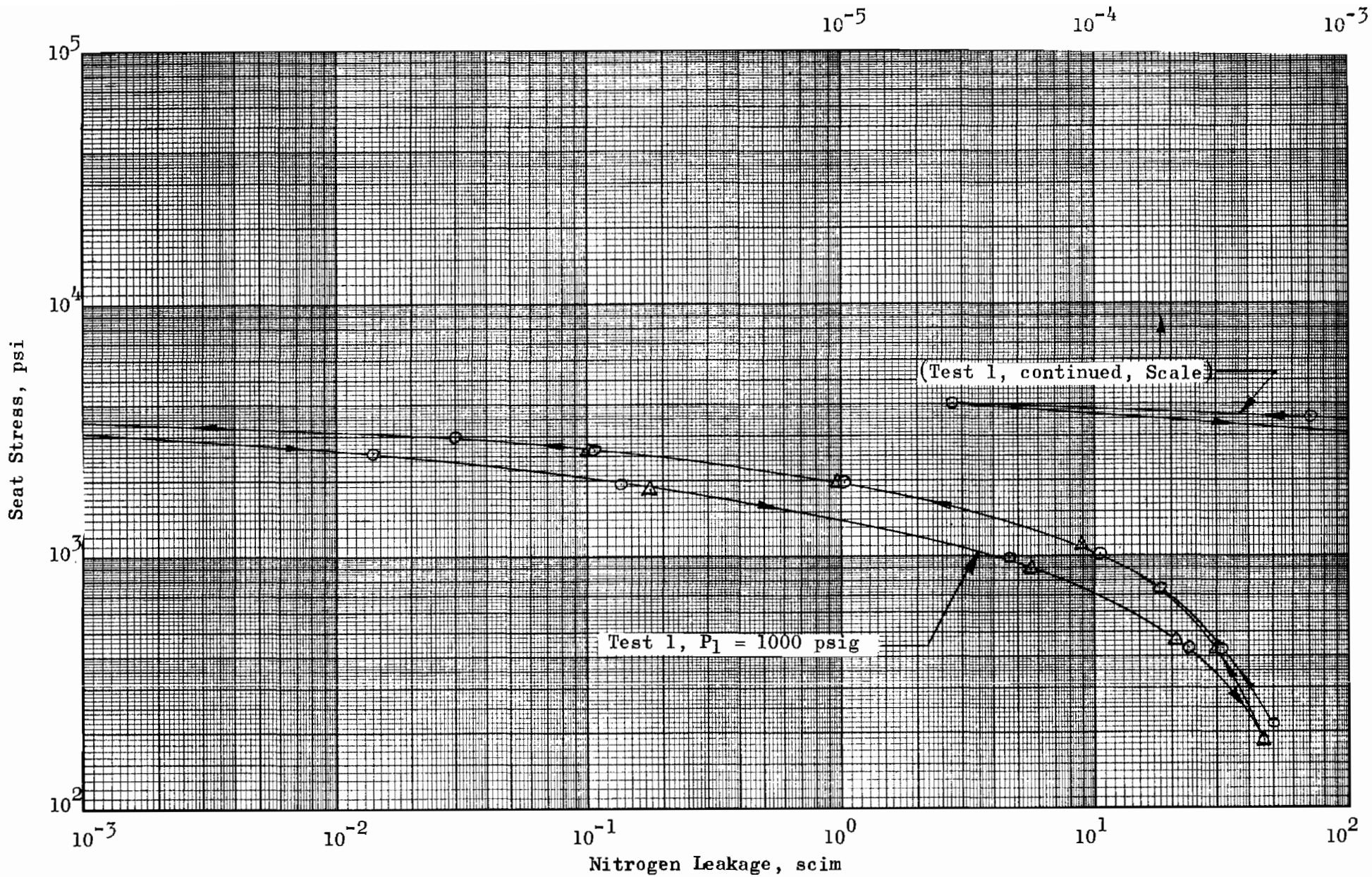
Figure 435. Stress-Leakage Data for Test Model G c , Test 1
