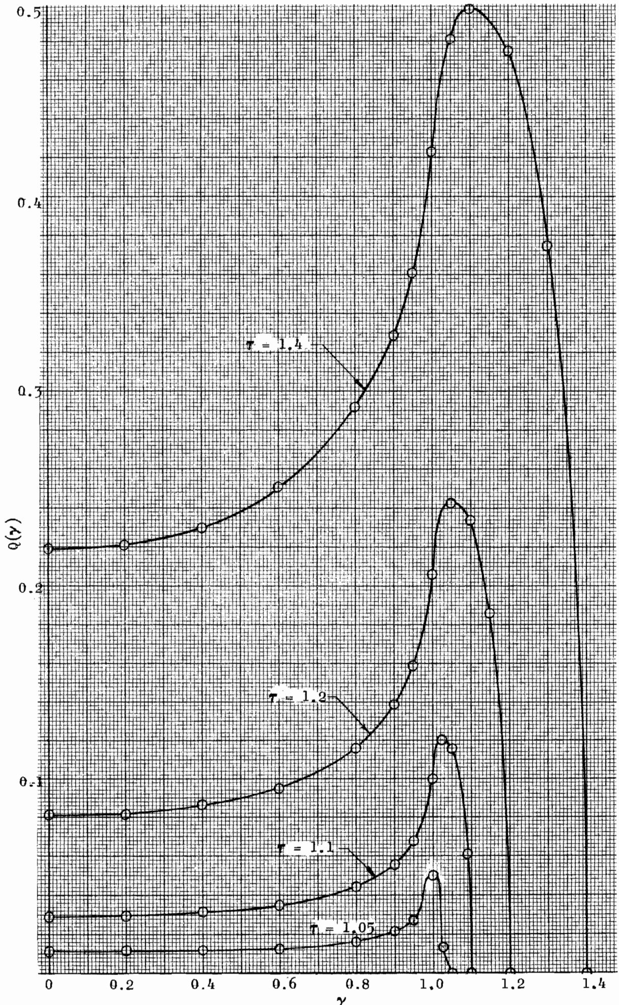
Figure 30. Contact Stress Distribution for Dubbed Seat
