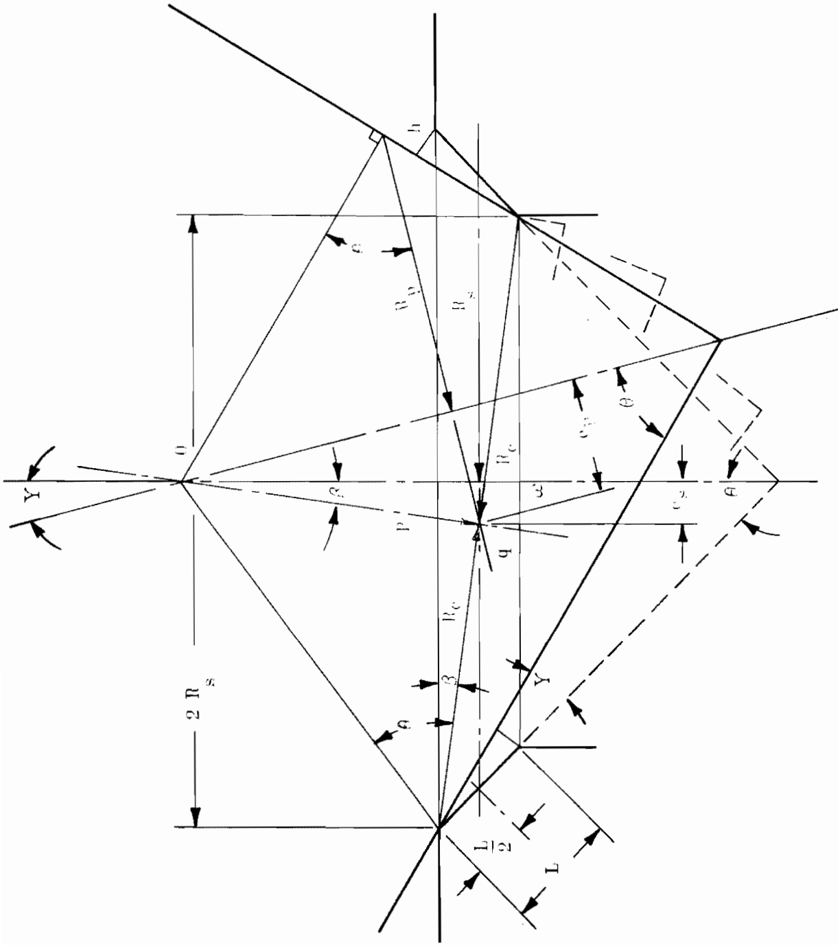
Figure 13. Tilted Conical Poppet Geometry
