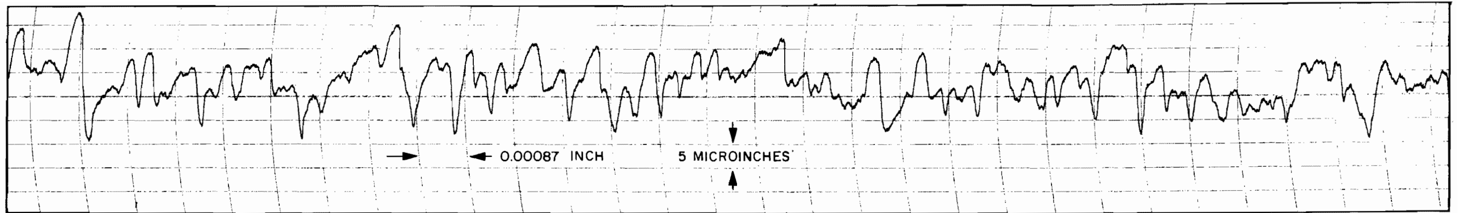
Figure 343. Test Model C, Poppet Roughness Profile Record, 0.0001-Inch Radius Stylus
