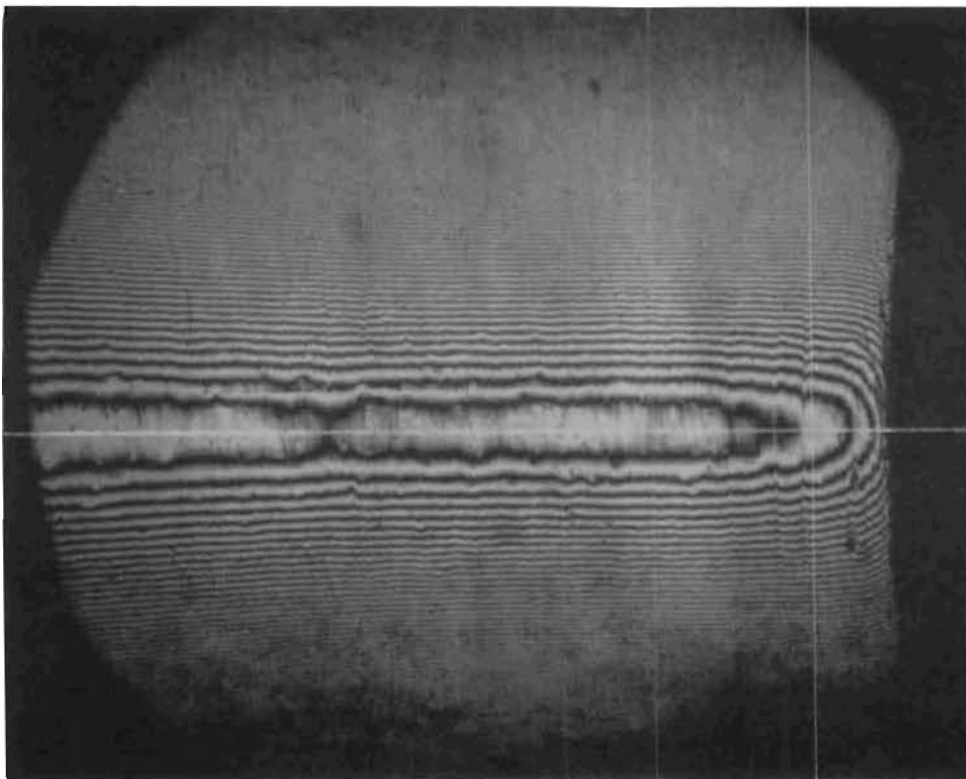
Figure 220. Test Model B c , Poppet, 0.045- x 0.056-Inch Inter- ference Photo, ID at Right
