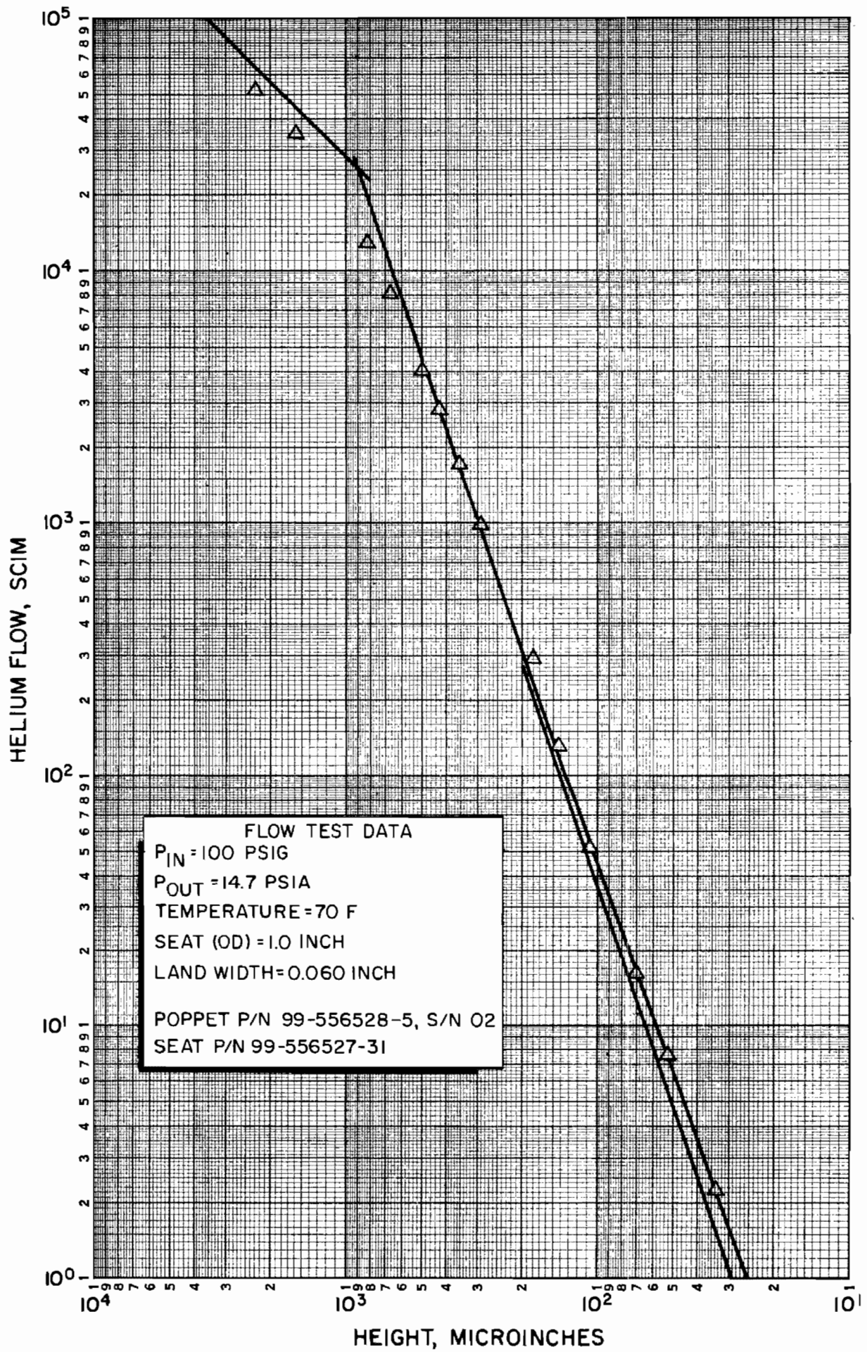
Figure 384. Helium Flow Data, Part 1
