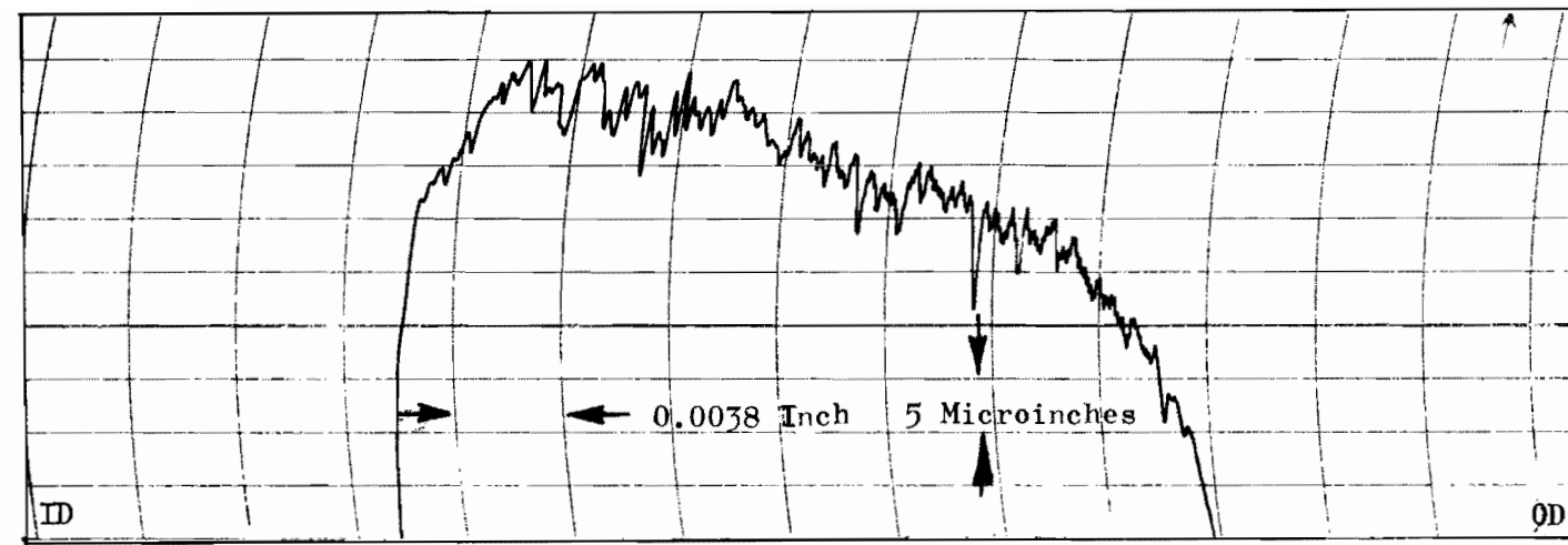
Figure 347. Test Model A c , Seat Cross Land Roughness Profile Record, 0.0005-Inch Radius Stylus
