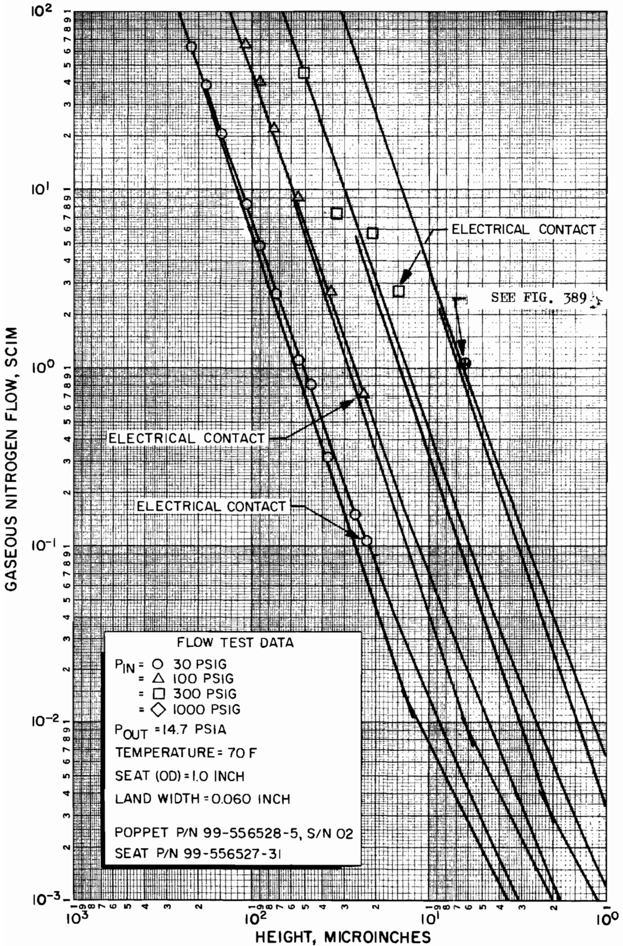
Figure 382. Nitrogen Flow Data, Part 2
