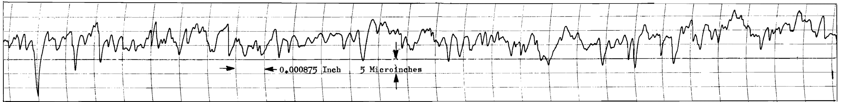
Figure 339. Test Model A f , Poppet Cross Lay Roughness Profile Record, 0.0001-Inch Radius Stylus
