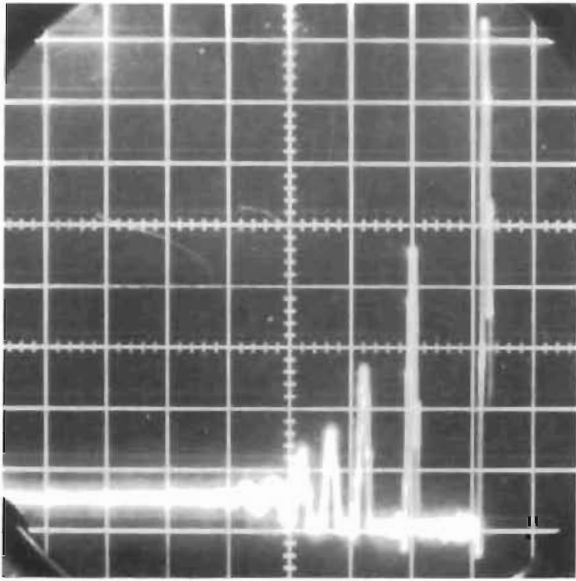
Figure 485. Test Model Y f , Piezo- electric Load Cell, ~ 24 in./sec Impact Velocity, PS = 169 psig (500 lb/div.; 0.001 sec/div.)
