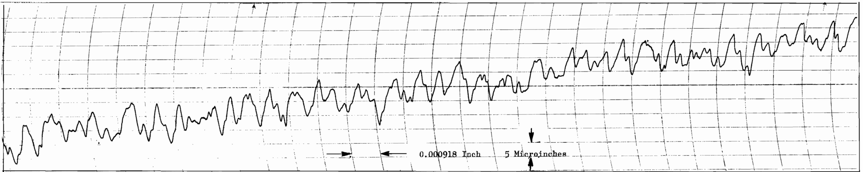
Figure 332. Test Model N_f , Seat Cross Lay Roughness Profile Record, 0.0001-Inch Radius Stylus
