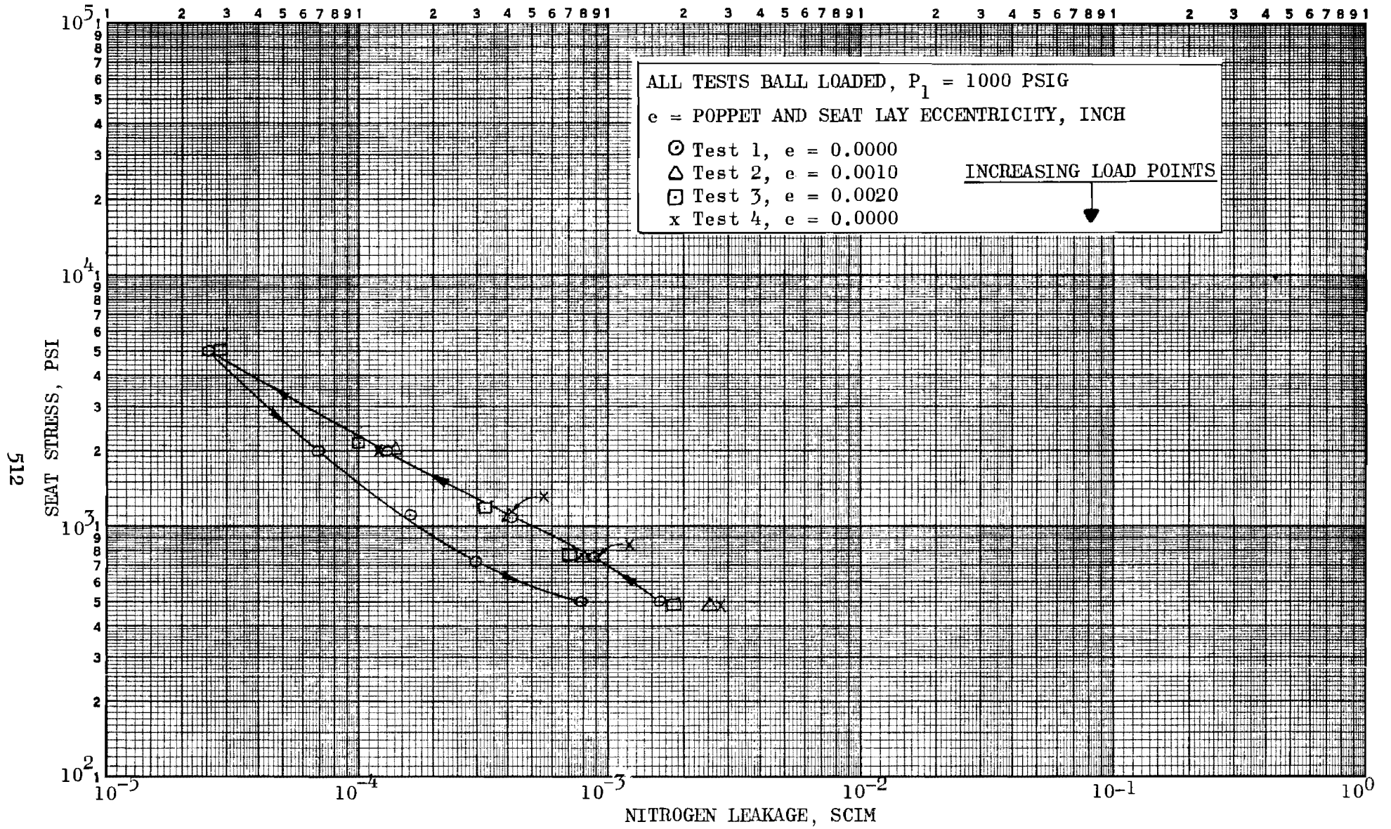
Figure 427. Stress-Leakage Data For Test Model HH f Tests 1 Through 4
