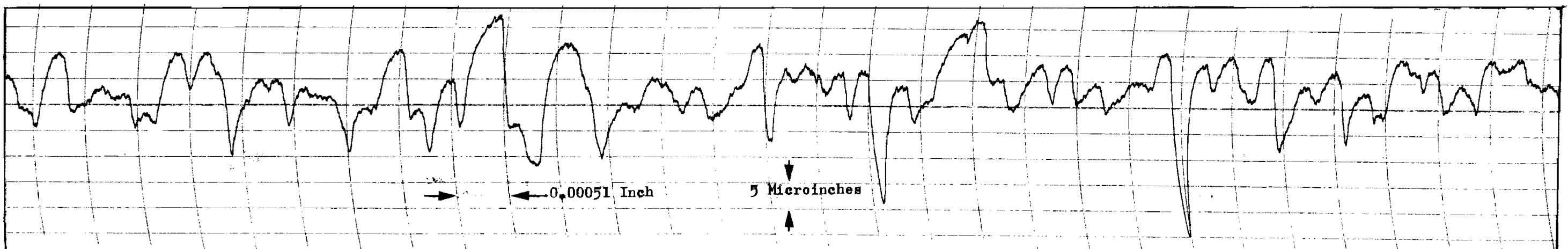
Figure 342. Test Model D, Poppet Roughness Profile Record, 0.0001-Inch Radius Stylus
