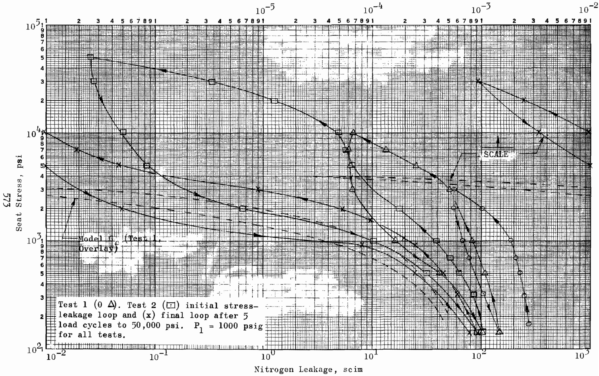
Figure 451. Stress-Leakage Data for Test Model G_{c1} , Tests 1 and 2
