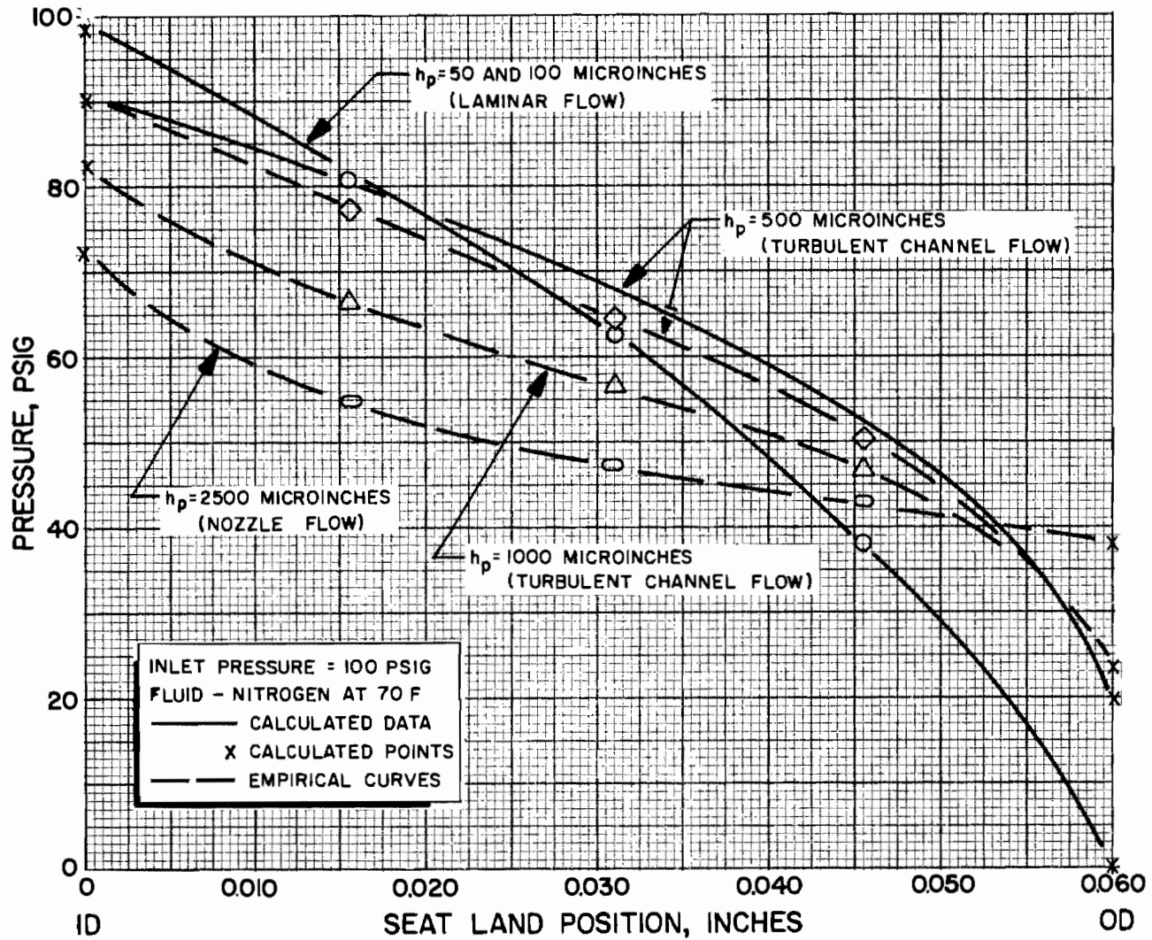
Figure 391. Pressure Distribution at Various Poppet-Seat Heights
