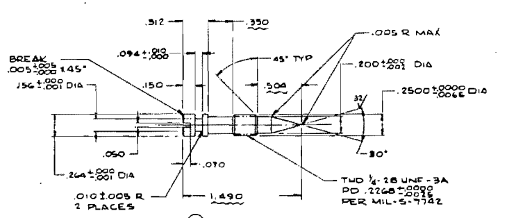
(45) NEEDLE VALVE
