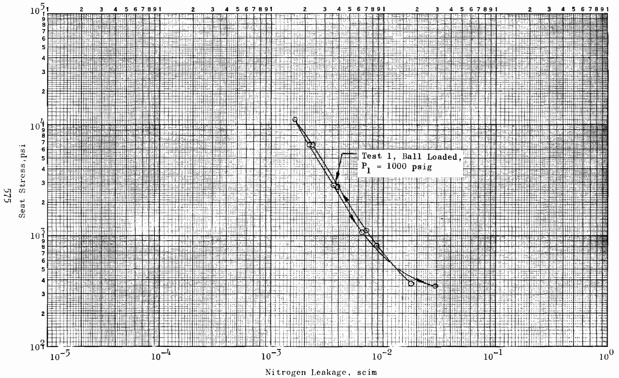
Figure 452. Stress-Leakage Data for Test Model T_f , Test 1
