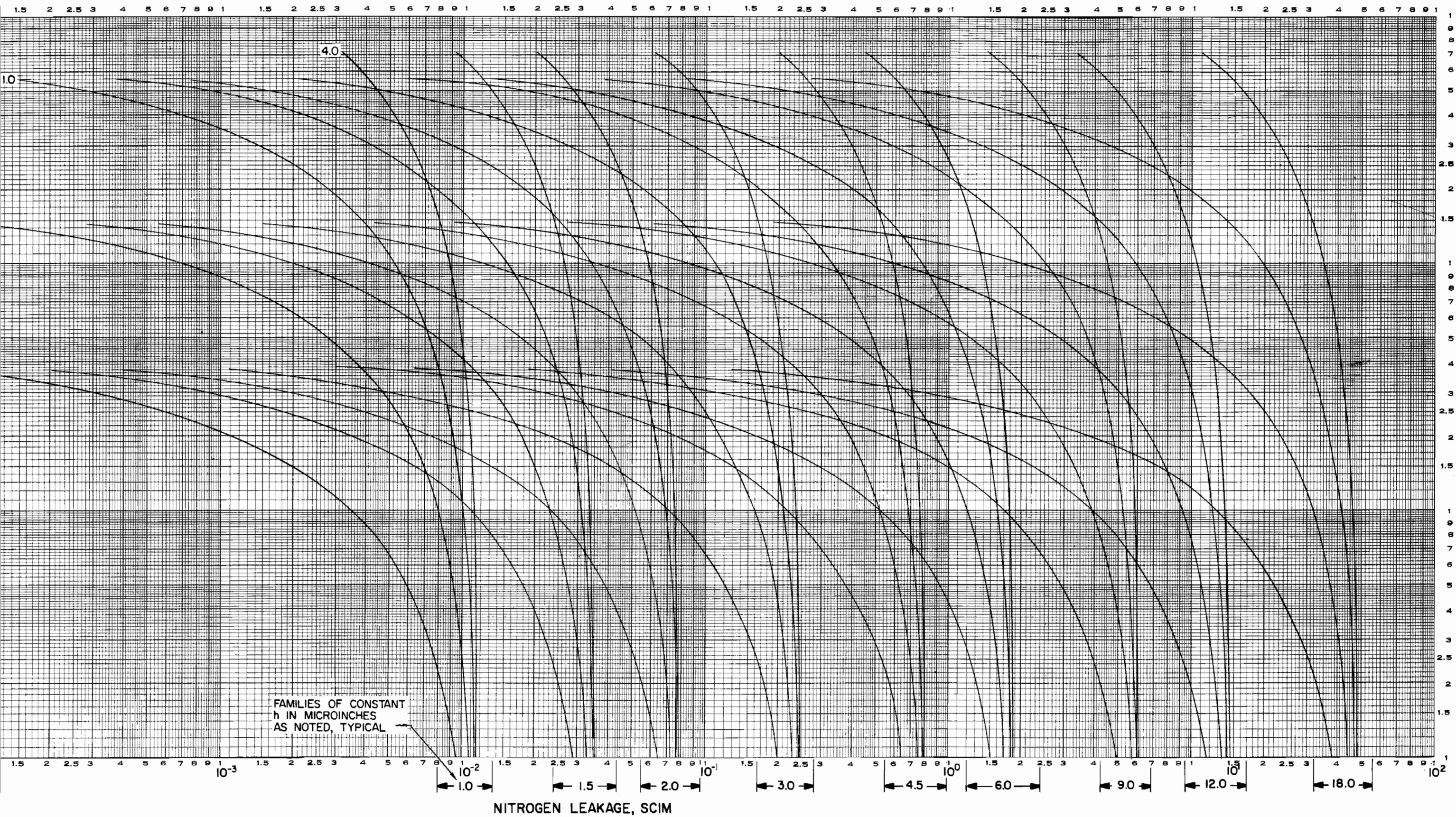
Figure 22. Theoretical Parametric Stress vs Leakage Curves for Steel
