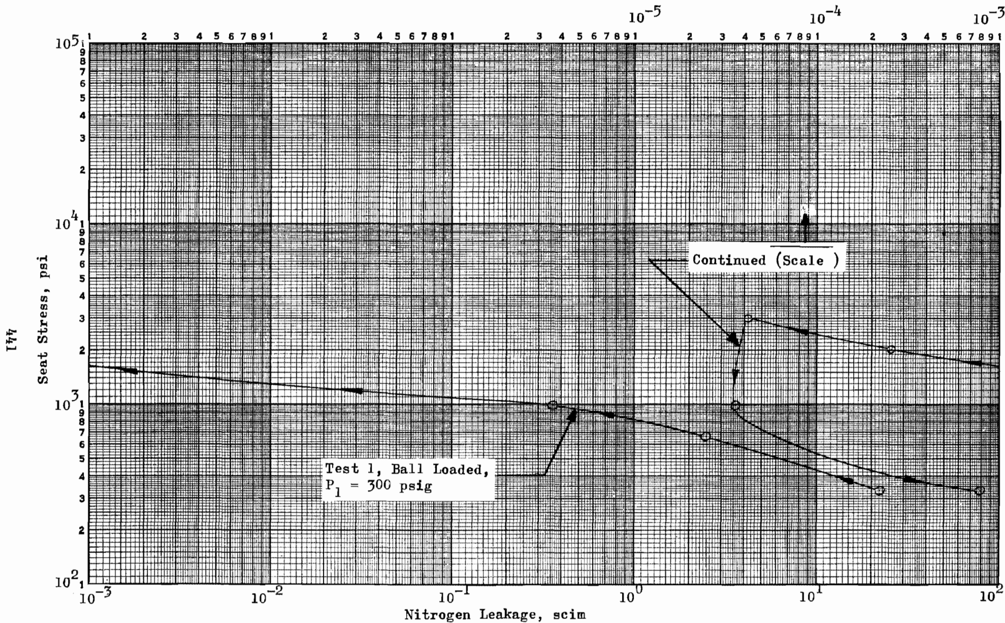
Figure 396. Stress-Leakage Data for Test Model S_f , Test 1
