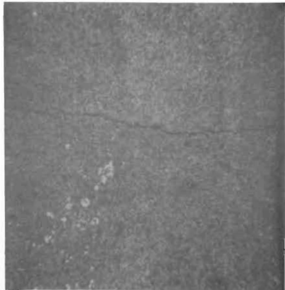
Figure 272. Test Model W_{f1} , Seat, 0.033- x 0.033-Inch Plain Photo Showing Ridged Crack in Plating
