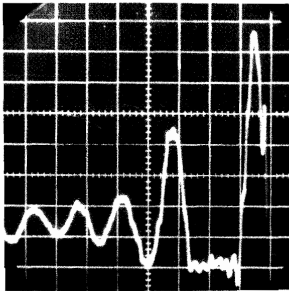
Figure 499. Test Model T_{f1} , Piezo- electric Load Cell, \sim 8.8 in./sec Impact Velocity, PS = 165 psig (175 lb/div.; 0.0002 sec/div.)
