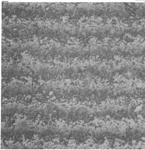
Figure 105. Test Model A, Seat, 0.0065- x 0.0065-Inch Interference Photo
