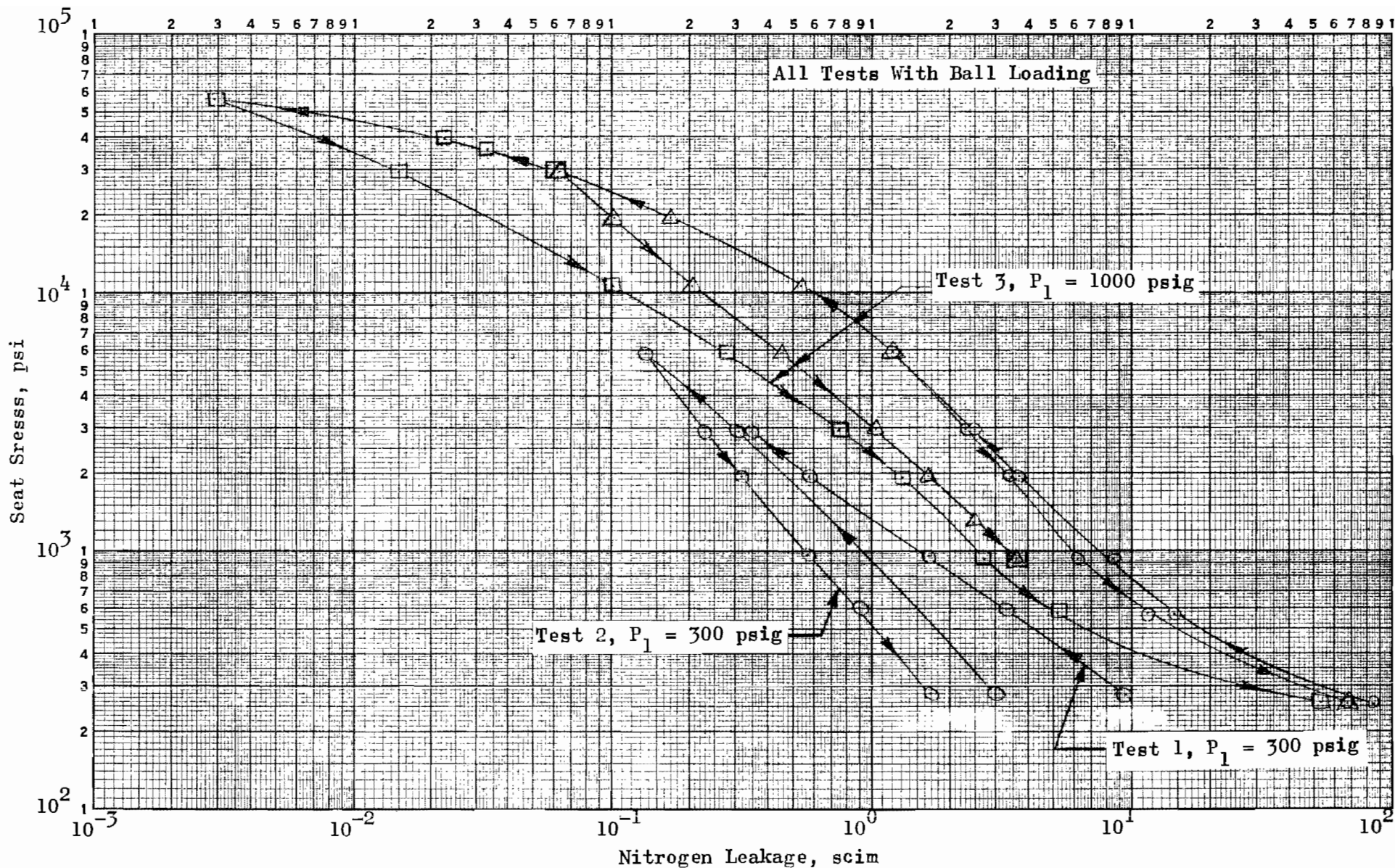
Figure 392. Stress-Leakage Data for Test Model Q_f , Tests 1, 2 and 3
