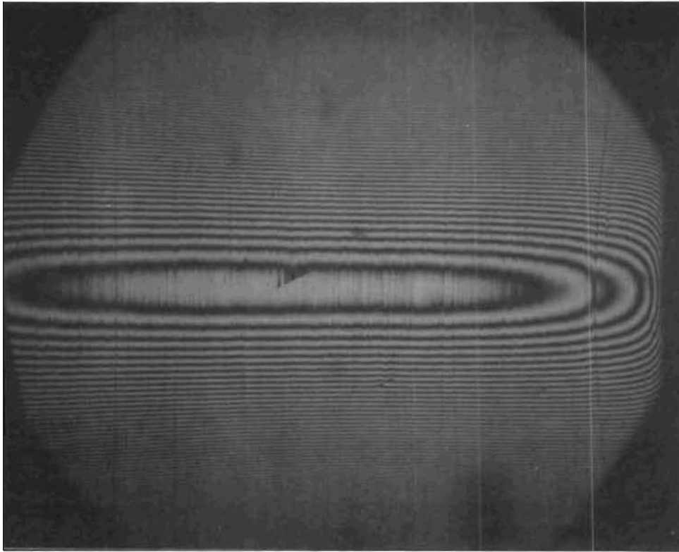
Figure 230. Test Model E_C , Poppet, 0.045- x 0.056-Inch Interference Photo, ID at Right
