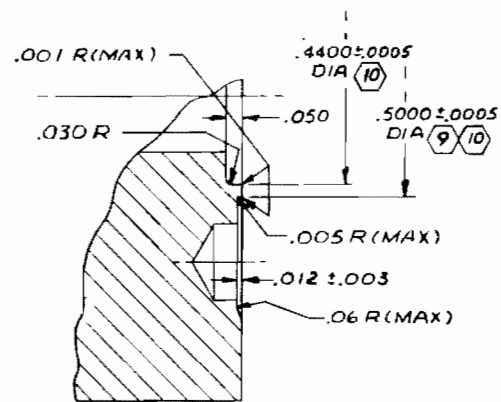
DETAIL "B" 4 TIMES SIZE
