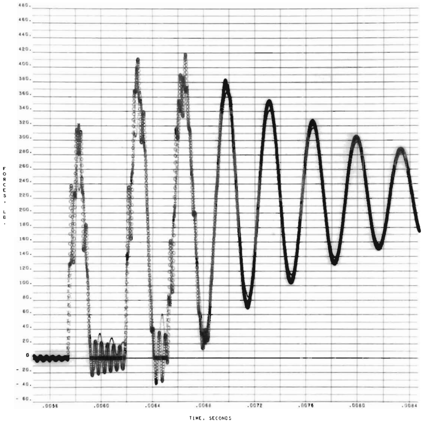
Figure 53. Computed Spring Forces, F_1 ( \cdot ), F_2 ( x ), F_3 ( o ), 1.87 in./sec Impact Velocity, PS = 156 psia, D\phi D = 0.0266 in.
