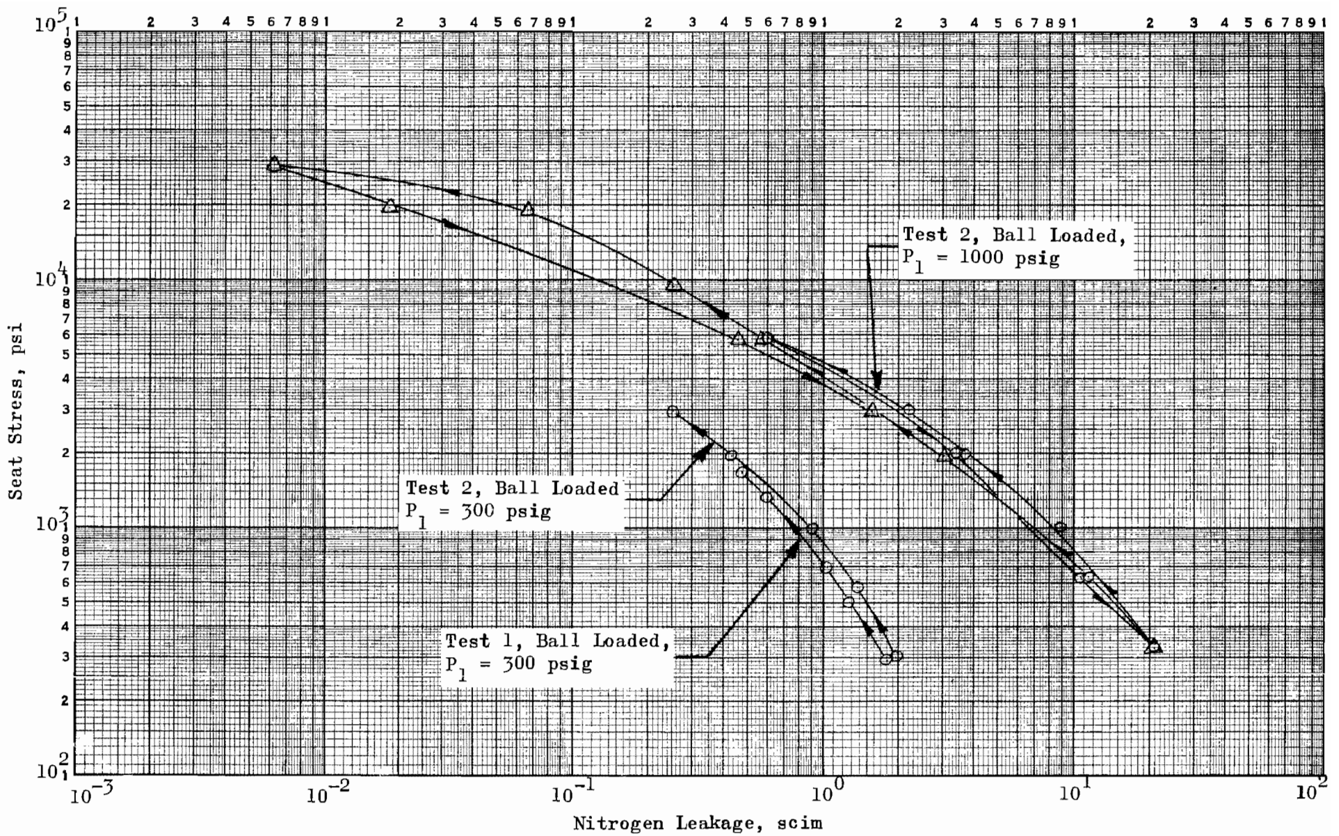
Figure 401. Stress-Leakage Data for Test Model A f , Tests 1 and 2
