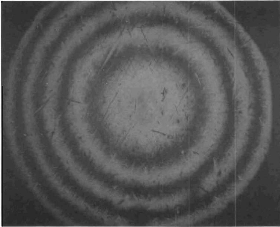
Figure 247. Test Model B s , Poppet, 0.0089- x 0.0110-Inch Interference Photo at \theta = 35 Degrees
