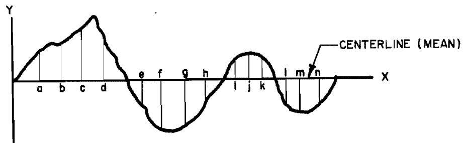
Figure 2. Incremental Division of Theoretical Surface Profile
