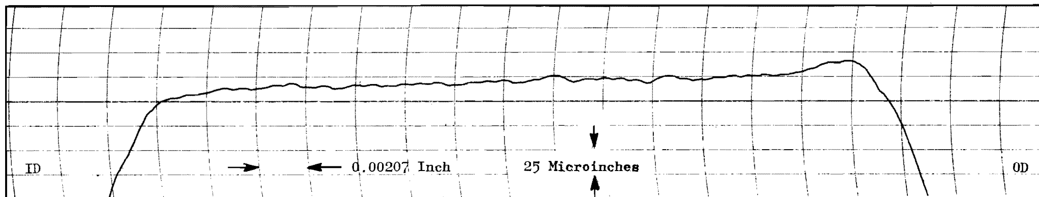
Figure 331. Test Model Q f , Seat Cross Land Profile Record, 1/16-Inch Ball Stylus
