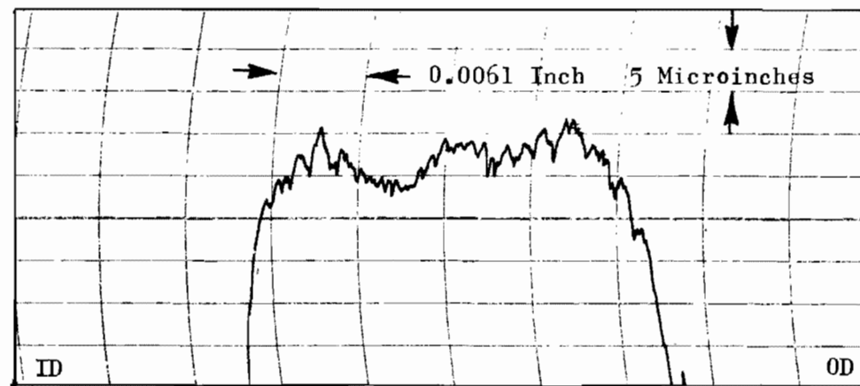
Figure 351. Test Model B c , Seat Cross Land Roughness Profile Record, 0.0005-Inch Radius Stylus
