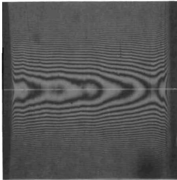
Figure 233. Test Model G_c , Seat, 0.033- x 0.033-Inch Interference Photo
