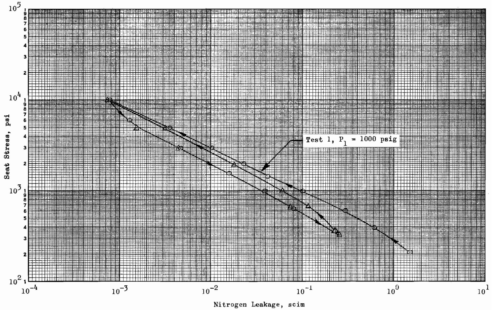
Figure 436. Stress-Leakage Data for Test Model A s , Test 1
