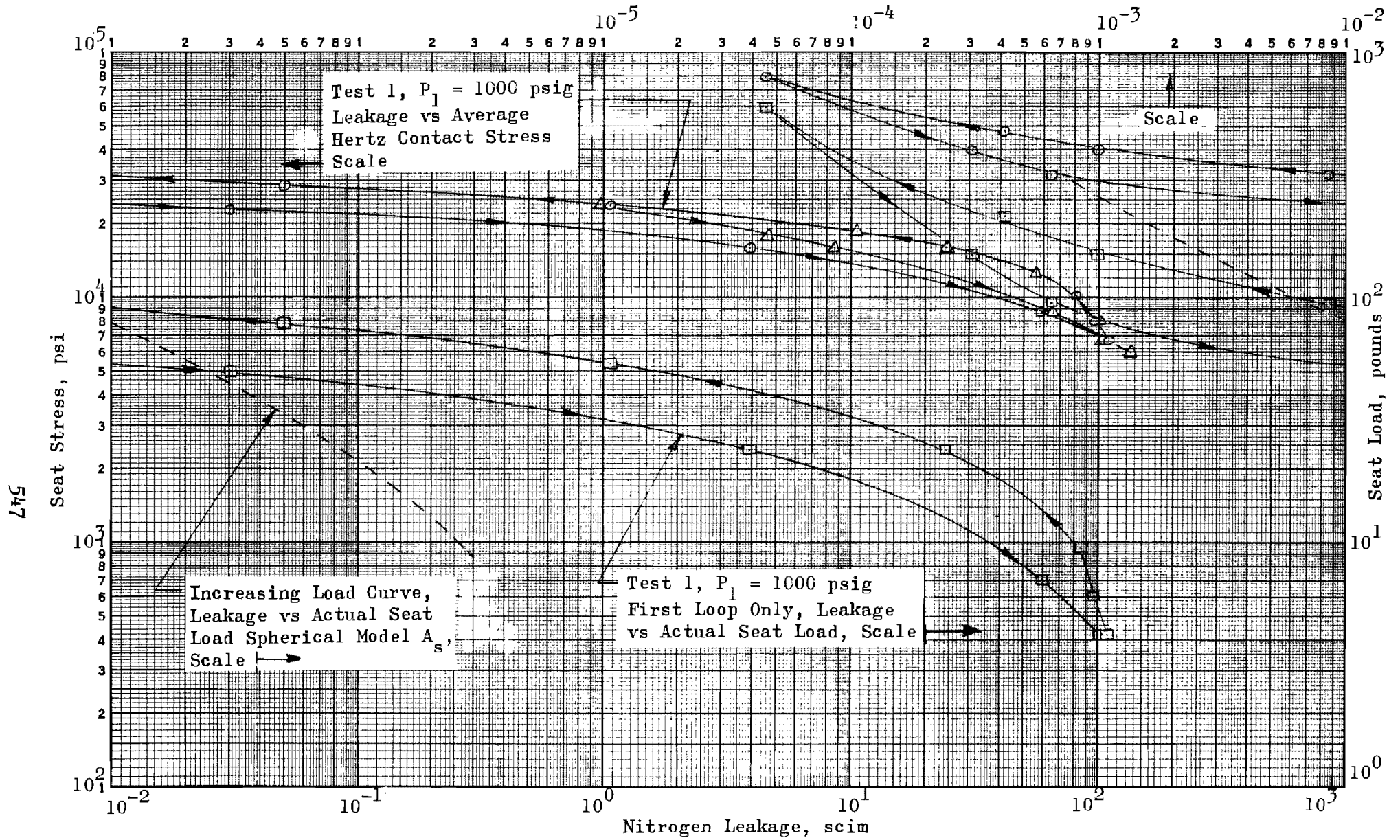
Figure 440. Stress-Leakage Data for Test Model H_{sc} , Test 1
