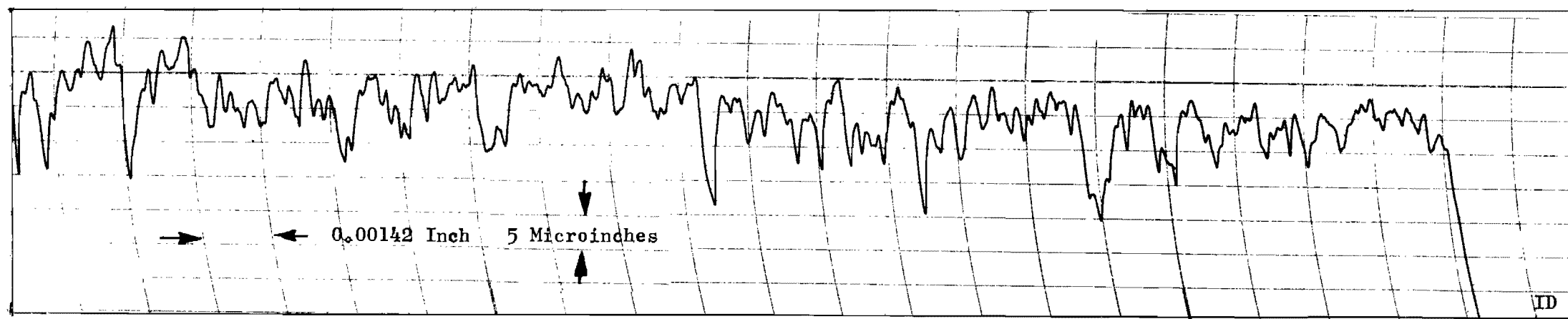
Figure 338. Test Model A f , Seat Cross Lay Roughness Profile Record, 0.0001-Inch Radius Stylus
