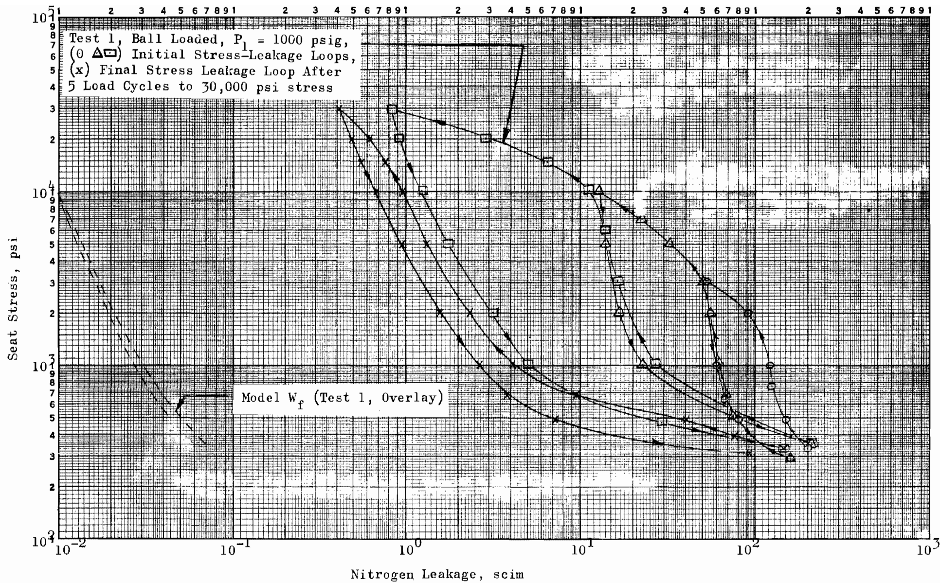
Figure 450. Stress-Leakage Data for Test Model W_{f1} , Test 1
