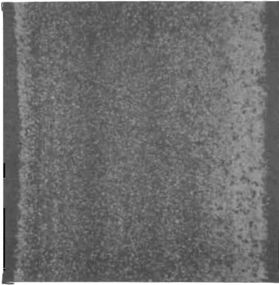
Figure 237. Test Model G_{c1} , Seat, 0.033- x 0.033-Inch Plain Photo Showing Plastic Deformation
