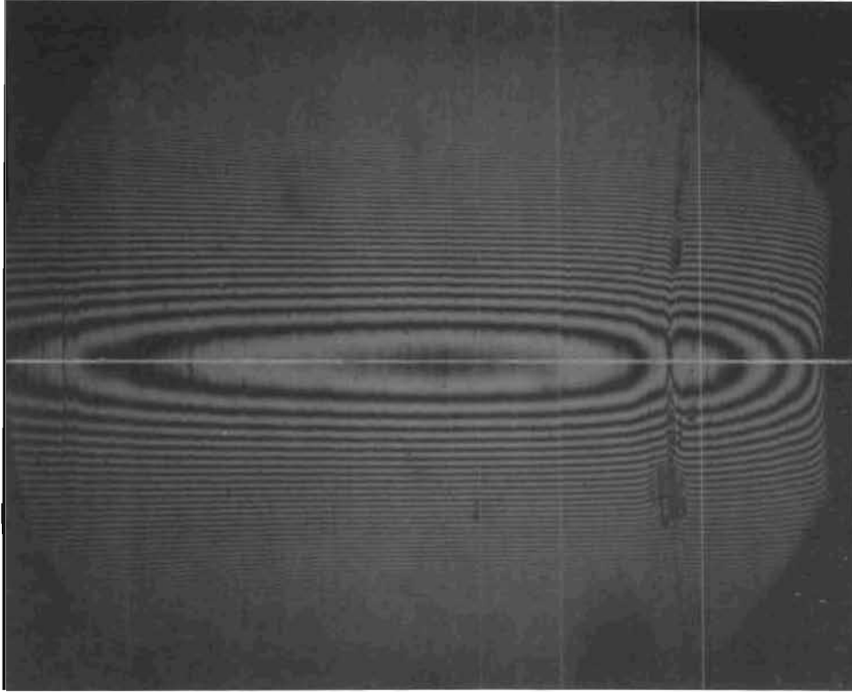
Figure 234. Test Model G_c , Poppet, 0.045- x 0.056-Inch Interference Photo, ID at Right
