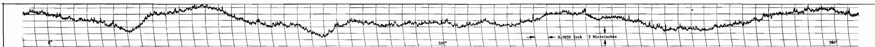
Figure 354. Test Model B c , Poppet Circumferential Roundness Profile Record, Midland, 1/16-Inch Ball Stylus
