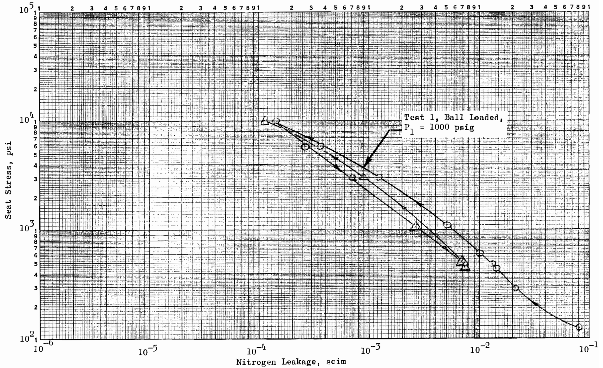
Figure 413. Stress-Leakage Data for Test Model B_f , Test 1
