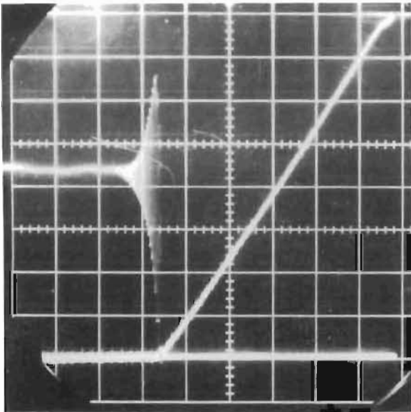
Figure 46. Piezoelectric Load Cell and Position, 1.87 in./sec Impact Velocity, PS = 141 psig (50 lb/div and 0.0125 in./div; 0.01 sec/div)
