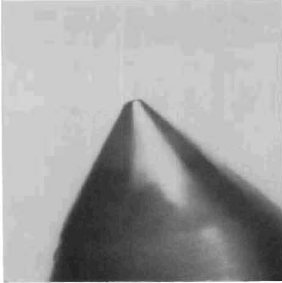
Figure 90. Profilometer Stylus, 0.0005-Inch Radius, 0.016- x 0.016- Inch Plain Photo
