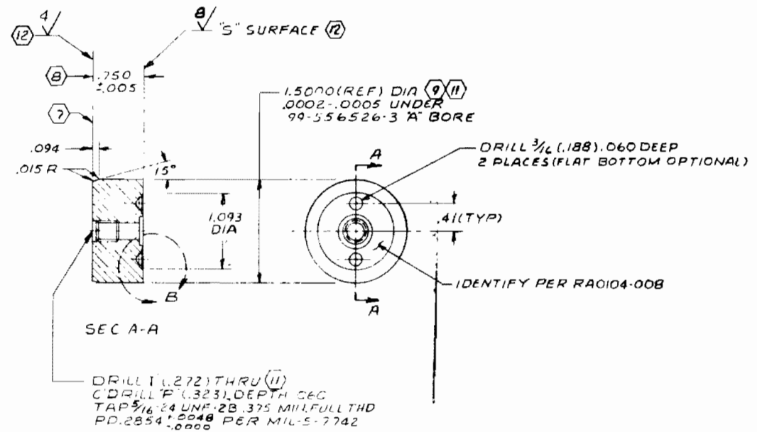
Figure 63. 0.5-Inch Model Seat (Drawing No. 99-556529A)
