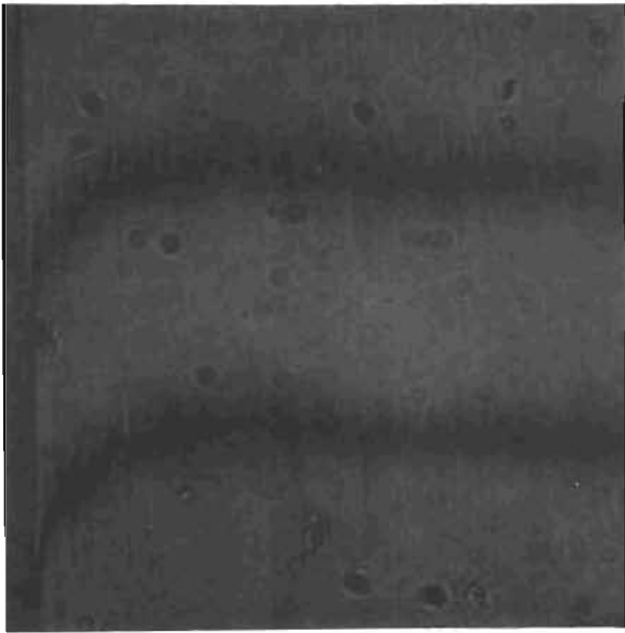
Figure 181. Test Model H f1 , Seat, 0.0065- x 0.0065-Inch Multiple Beam Interference Photo (Spots From Optics Contaminants)
