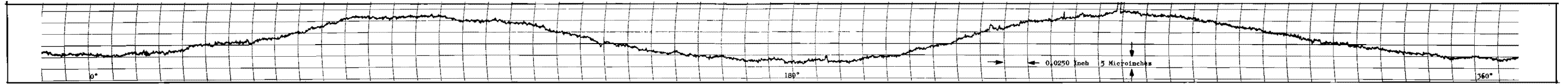
Figure 357. Test Model C c , Seat Circumferential Roundness Profile Record, Midland, 1/16-Inch Ball Stylus
