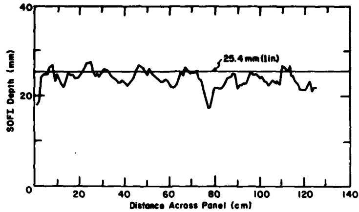
Figure 51. Horizontal profile of SOFI thickness on side B of the panel 4.13 m from the top.
