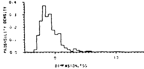
NORM. EXTREME OF SPRINGING STRESS. HALF RANGE BALLAST CONDITIONS
