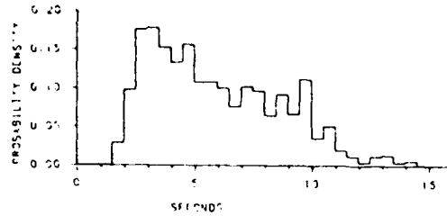
AV. ZERO CROSSING PERIOD, T2 ALL LOADING CONDITIONS
