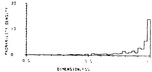
BENDING SHARE SQUARED, XB**2=(1-X**2) FULL LOAD CONDITIONS
