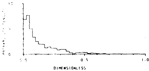
PEAK PERIOD DIVISION RATIO. (T - T_S) / (T_B - T_S) ALL LOADING CONDITIONS
