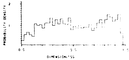
ZERO PERIOD DIVISION RATIO. (T_Z - T_S) / (T_B - T_S) ALL LOADING CONDITIONS
