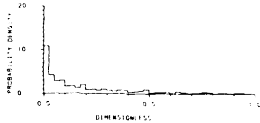
SPRINGING SHARE SQUARED, X**2 ALL LOADING CONDITIONS
