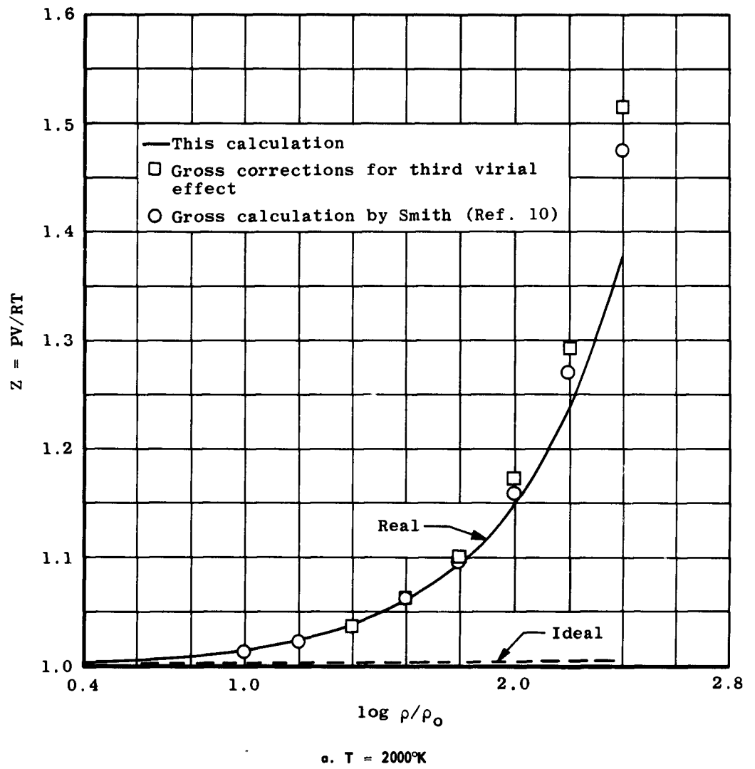
Fig. 2 Corrected and Ideal Compressibility Isotherms for Air
