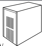
RNS-1008A/ RNS-1009W: W 76.2 D 60 H 69.5 cm RNS-1078C: W 55.8" D 60 H 69.5 cm RNS-1008A/ *489 kg, daily at 70/50° RNS-1009W: *374 kg daily at 90/70° RNS-1078C: *513 kg daily at 70/50° *408 kg daily at 90/70°
