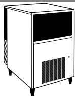
RNS-0385A W 73.8 D 69.0 H 100.4 cm *137 kg daily at 70/50° *112 kg daily at 90/70°
