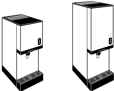
W 41.3 D 61 H 106.7 cm W 41.3 D 61 H 106.7 cm *118 kg daily at 70/50° *85 kg daily at 90/70° *118 kg daily at 70/50° *85 kg daily at 90/70°
