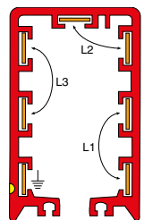
per phase 2 conductors in parallel+earth
