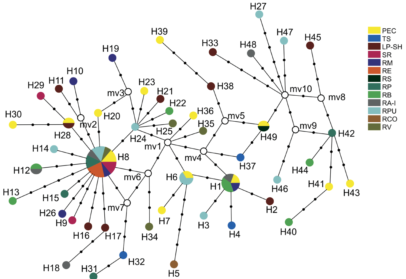
Fig. 7. Median-joining network based on COI haplotypes of Macrobrachium occidentale . Haplotypes derived from 13 basins are represented by colors with node size proportional to number of individuals with that haplotype. Mutational steps are indicated as black dots along network branches and Network software inferred median vectors as white dots. Drainage basins from the peninsula: SR = Santa Rita, LP-SH = Las Pocitas-San Hilario, TS = Todos Santos, and PEC = Plutarco E. Calles. Drainage basins from the mainland: RM = Río Mayo 3; RE = Río Elota; RS = Río Sinaloa 2; RP = Río Presidio 2; RB = Río Baluarte 2; RA-I = Río Ameca Ixtapa B; RPU = Río Purificación; RCO = Río Coyuca 2; RV = Río Verde.
