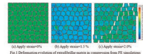
Fig.1 Deformation evolution of extrafibrillar matrix in compression from FE simulations
