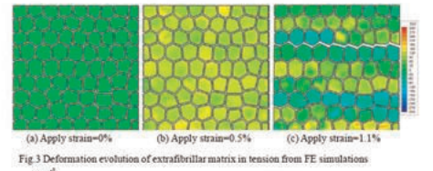
Fig.3 Deformation evolution of extrafibrillar matrix in tension from FE simulations
