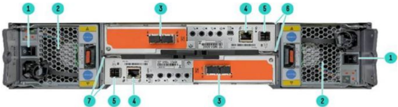
HPE MSA 1060 Storage-Rear View
