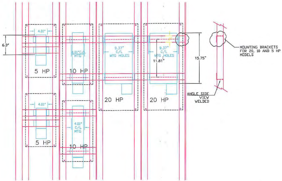
VIEW FROM REAR OF VFD MOUNTING RACK
