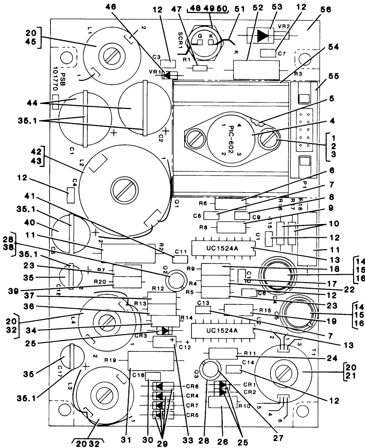
Figure 54. Circuit Card Assembly (Power Supply)
