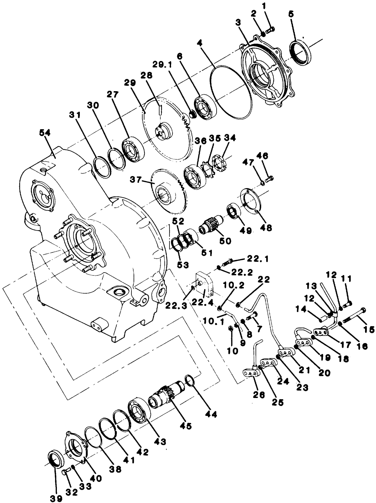
Figure 45. Gas Turbine Engine (Gearbox)
