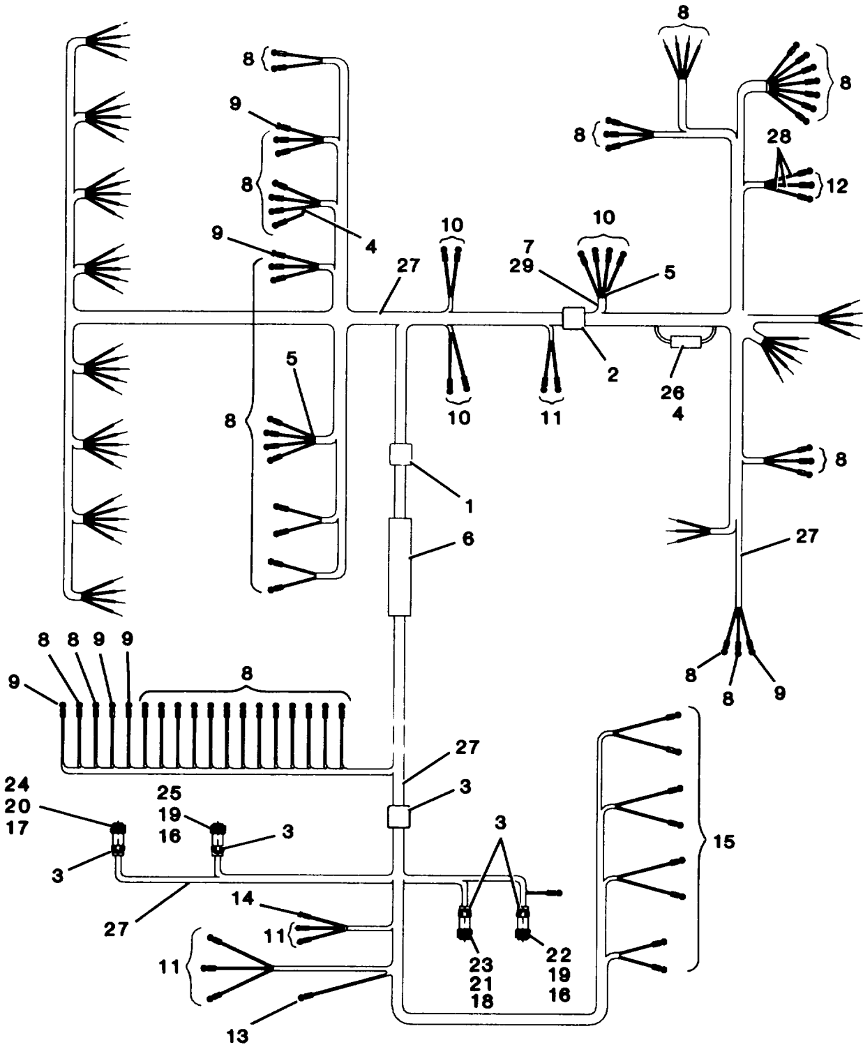
Figure 50. Wiring Harness Assembly (Control Panel)
