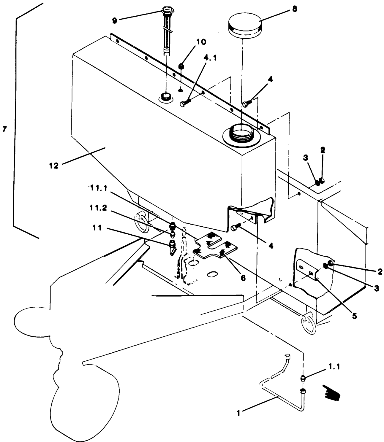
Figure 25. Engine Fuel Tank
