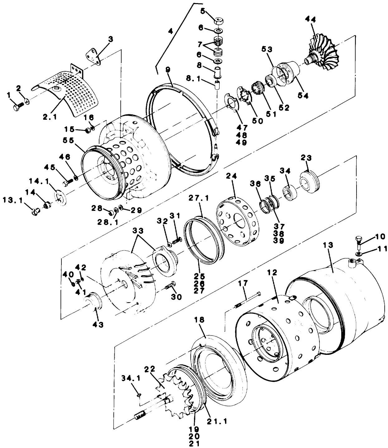
Figure 43. Gas Turbine Engine (Power Section)
