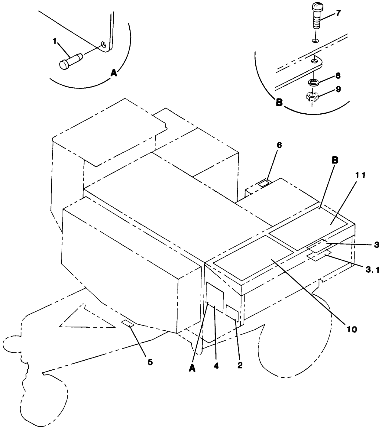
Figure 1. Identification and Instruction Plates
