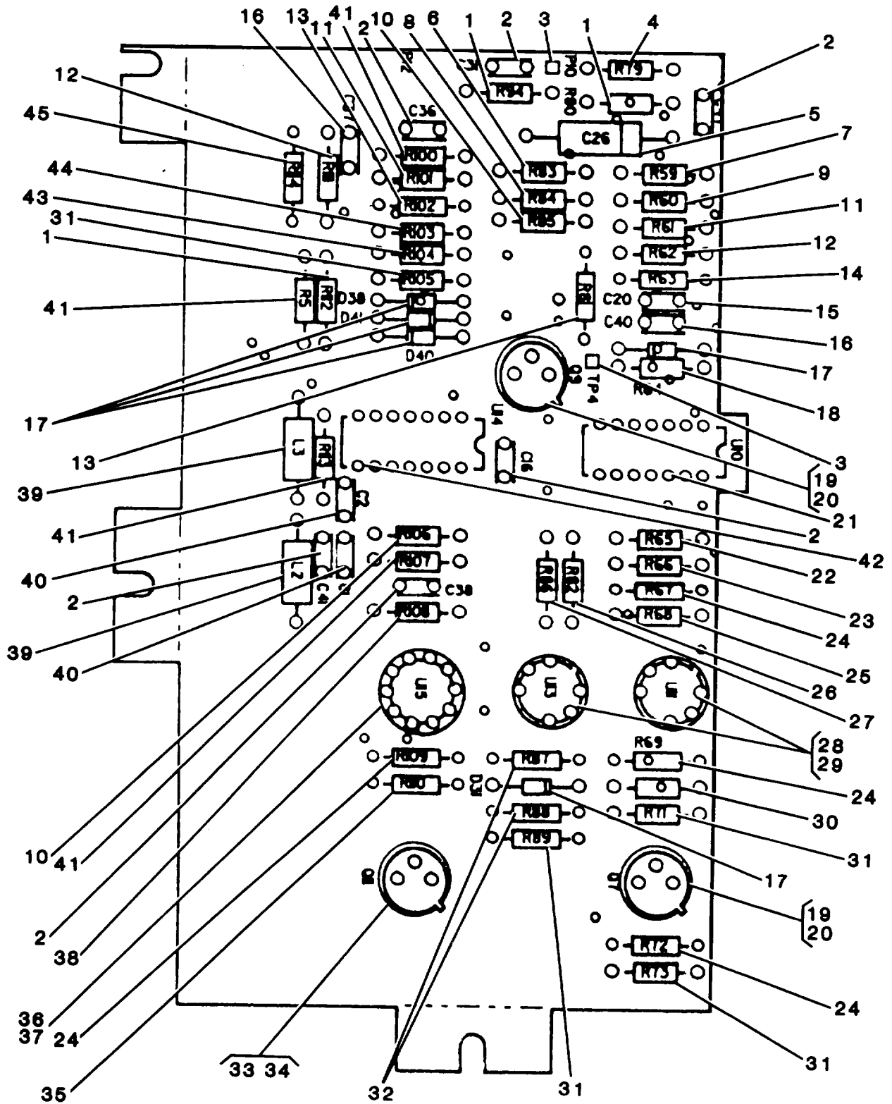
Figure 17D. GECM Circuit Card Assembly (Section D)
