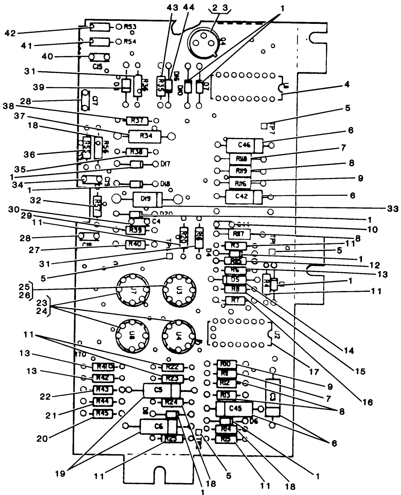
Figure 17C. GEOM Circuit Card Assembly (Section C)
