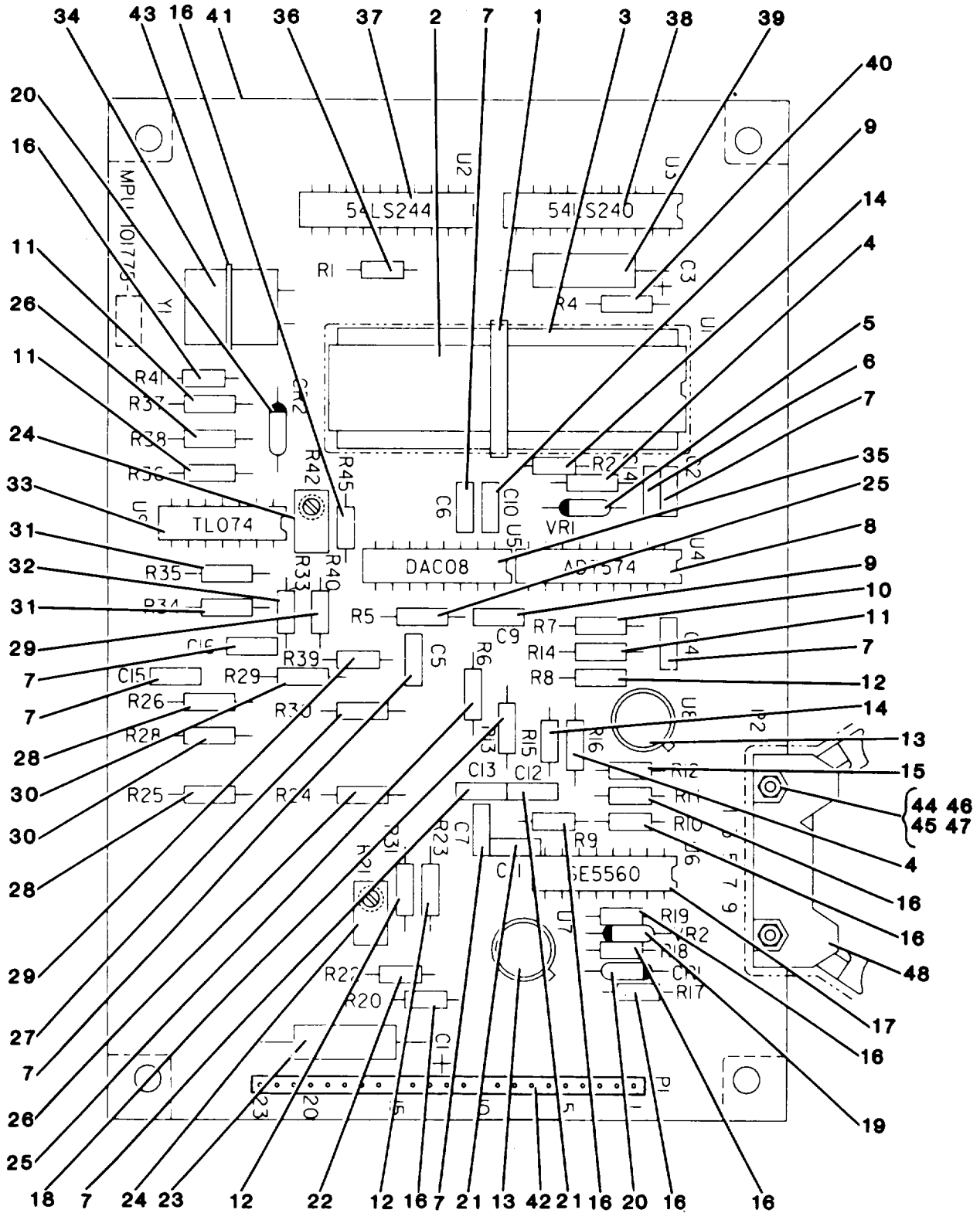
Figure 52. Circuit Card Assembly (MPU)
