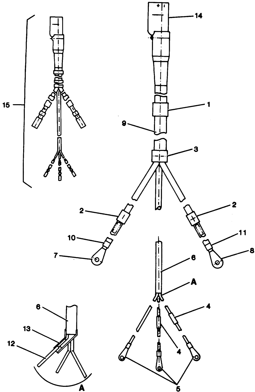
Figure 57. Power Cable Assembly
