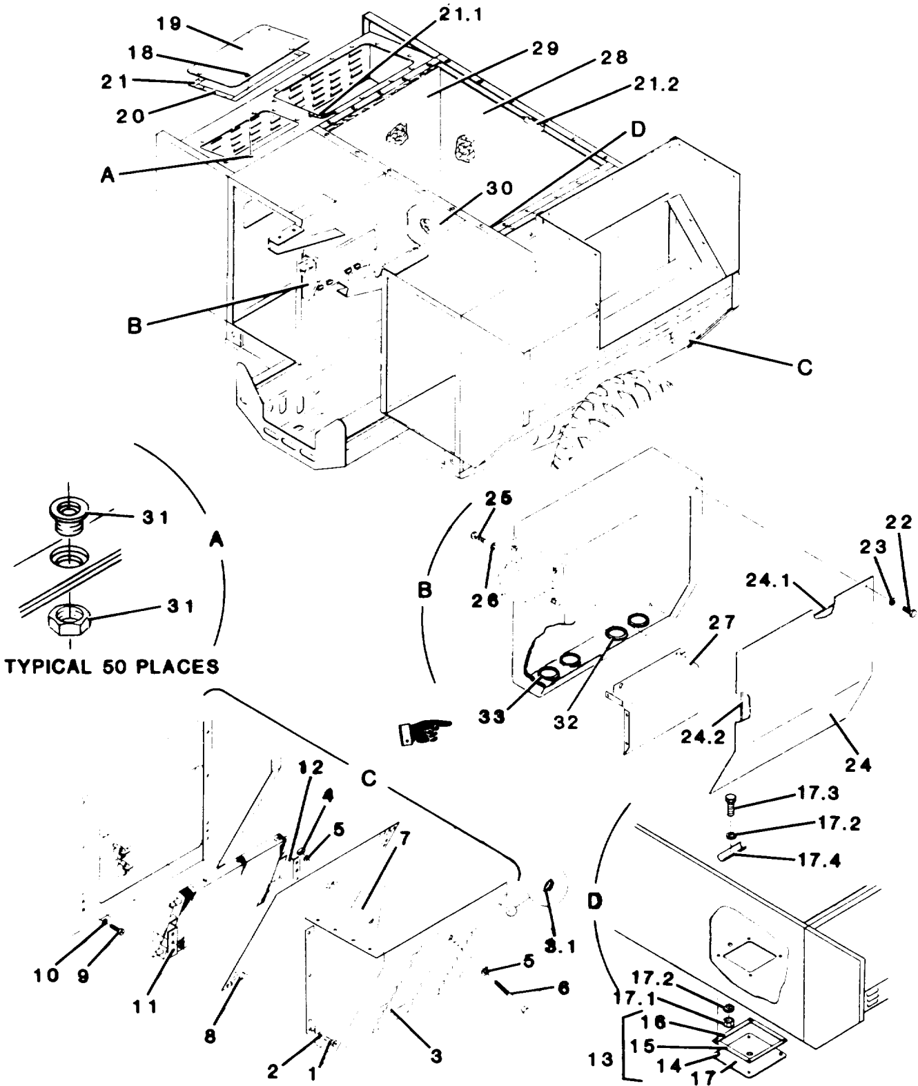
Figure 8. Trailer Body (Covers and Insulation)
