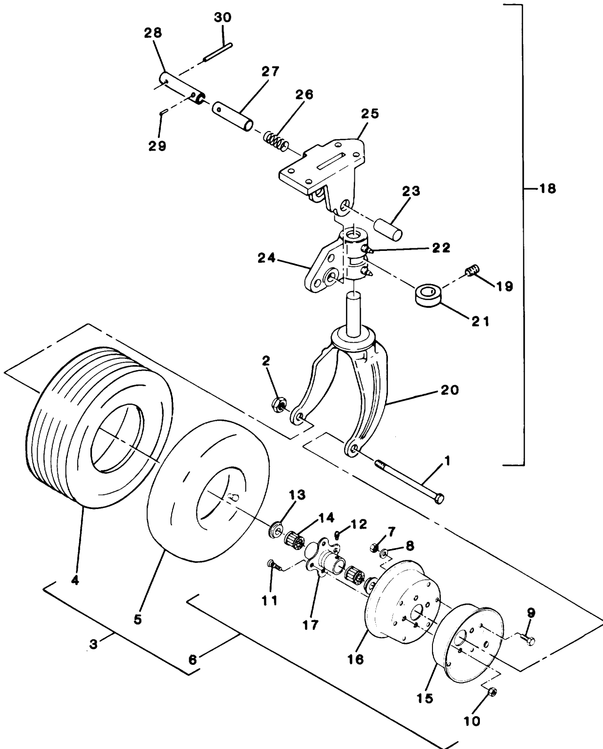
Figure 62. Swivel Caster and Wheel Assembly
