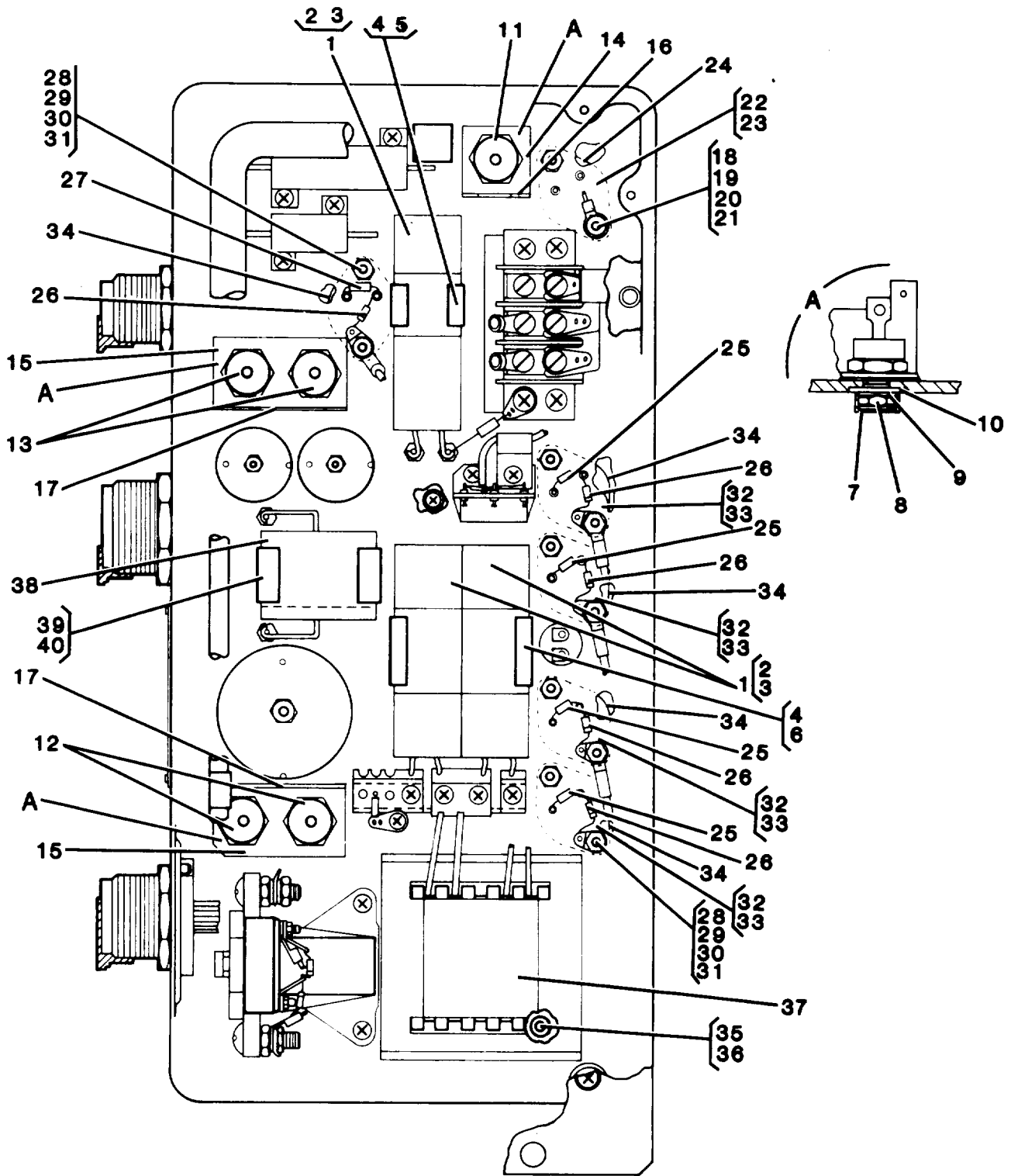
Figure 19. GECM Components (Capacitors, Diodes, etc.)
