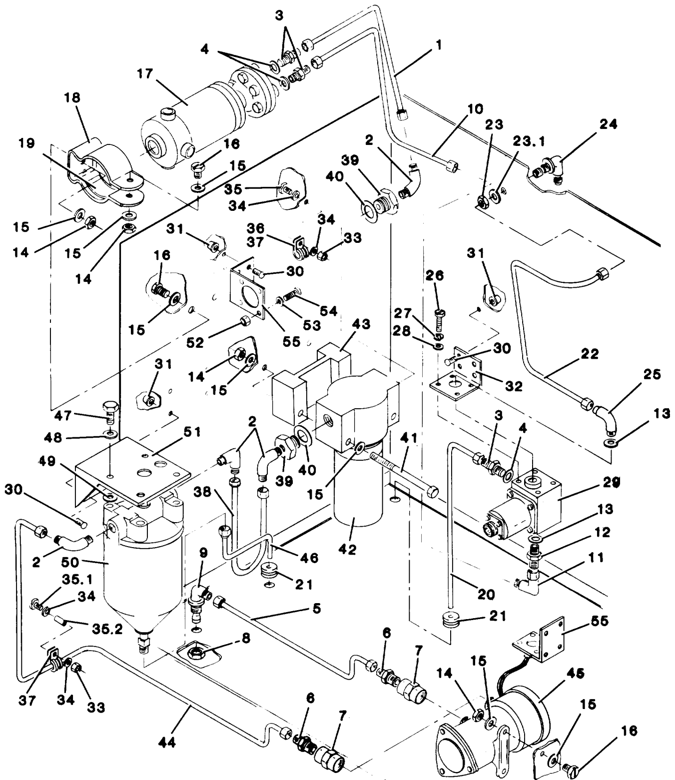
Figure 28. Fuel Housing Components
