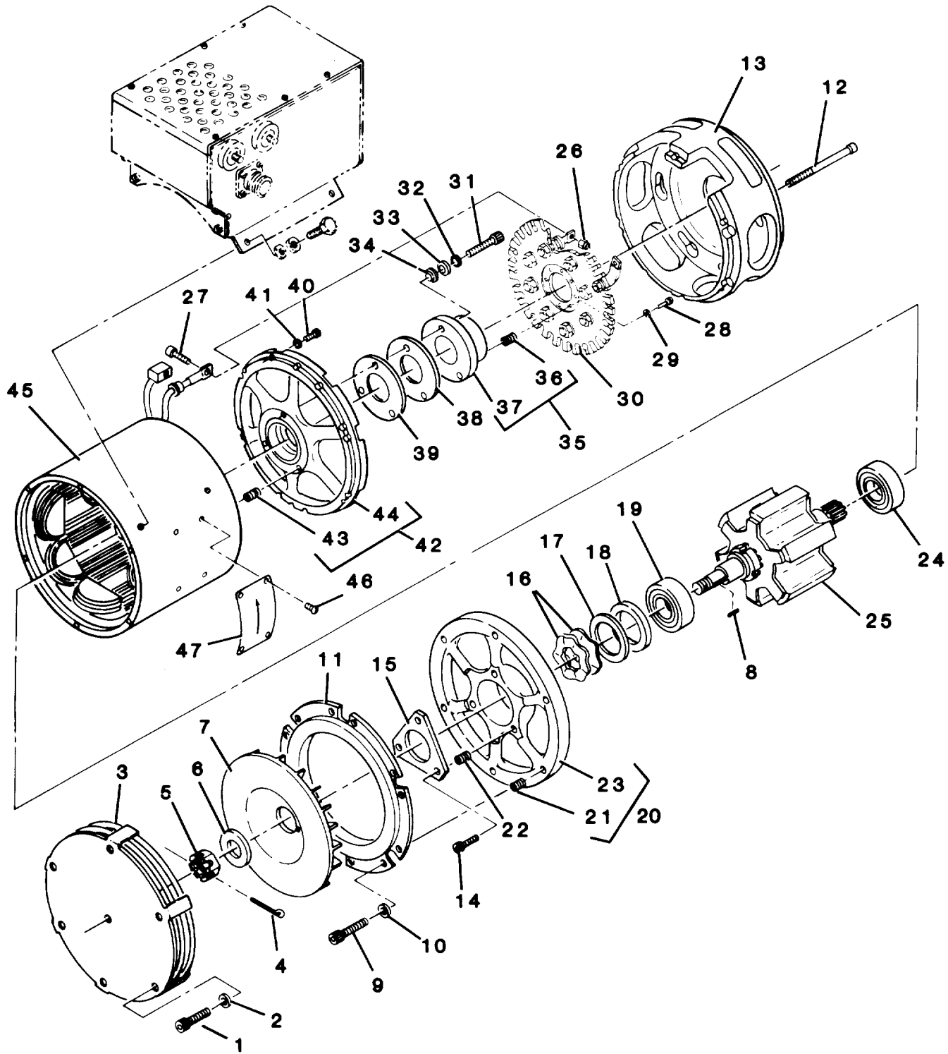
Figure 23. 10KW Generator Assembly
