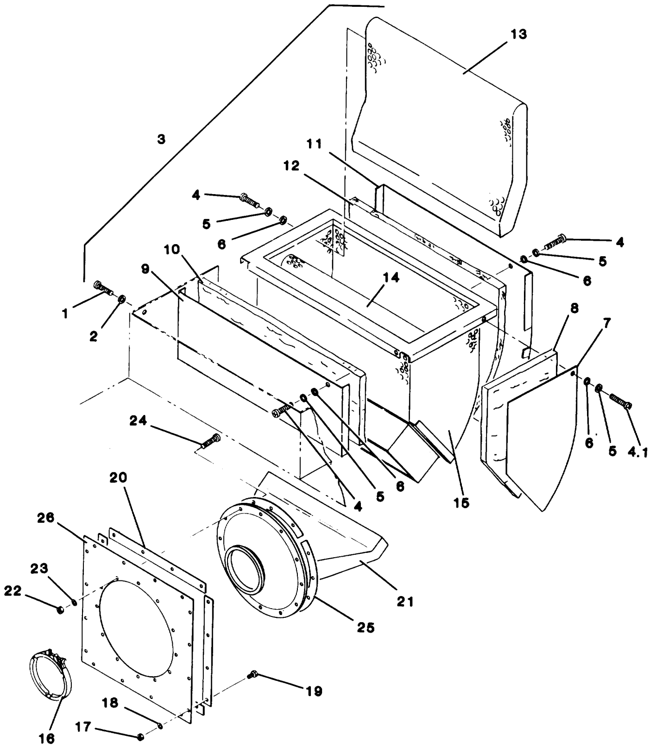
Figure 46. Exhaust Duct
