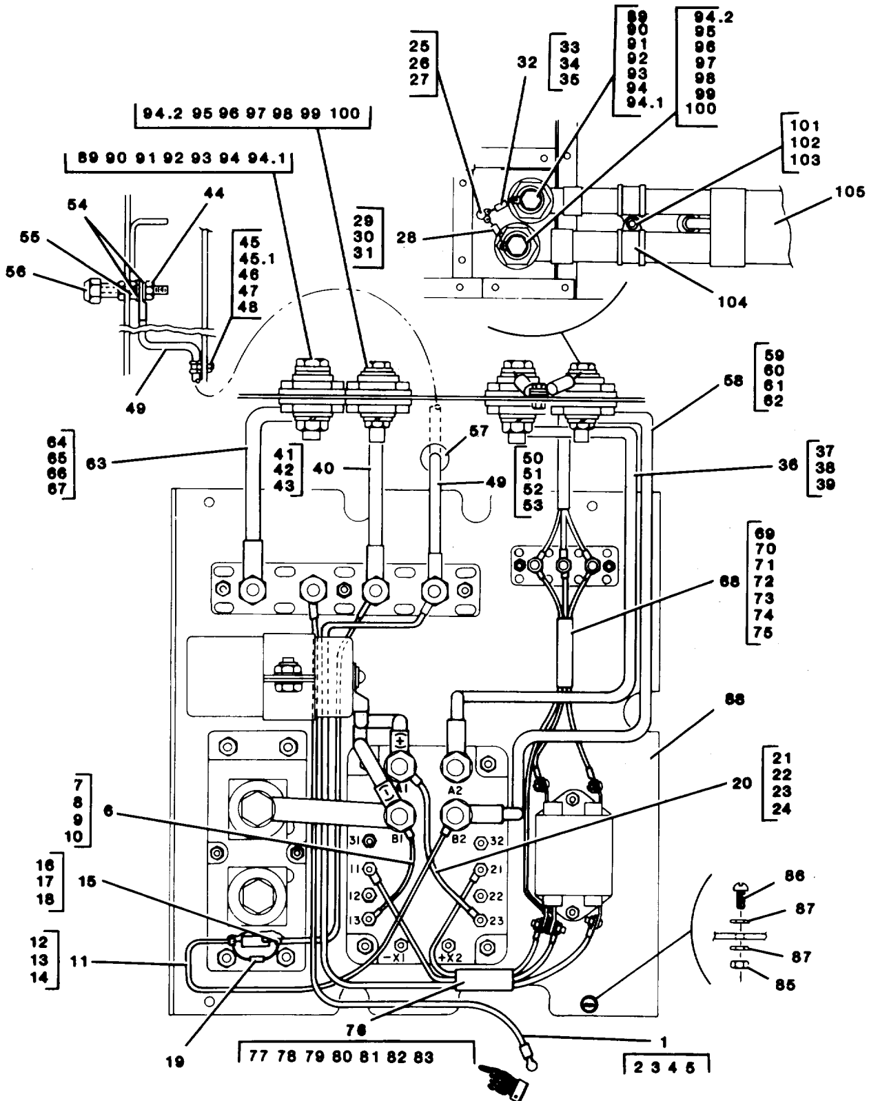
Figure 56. Load Connection Component Wiring
