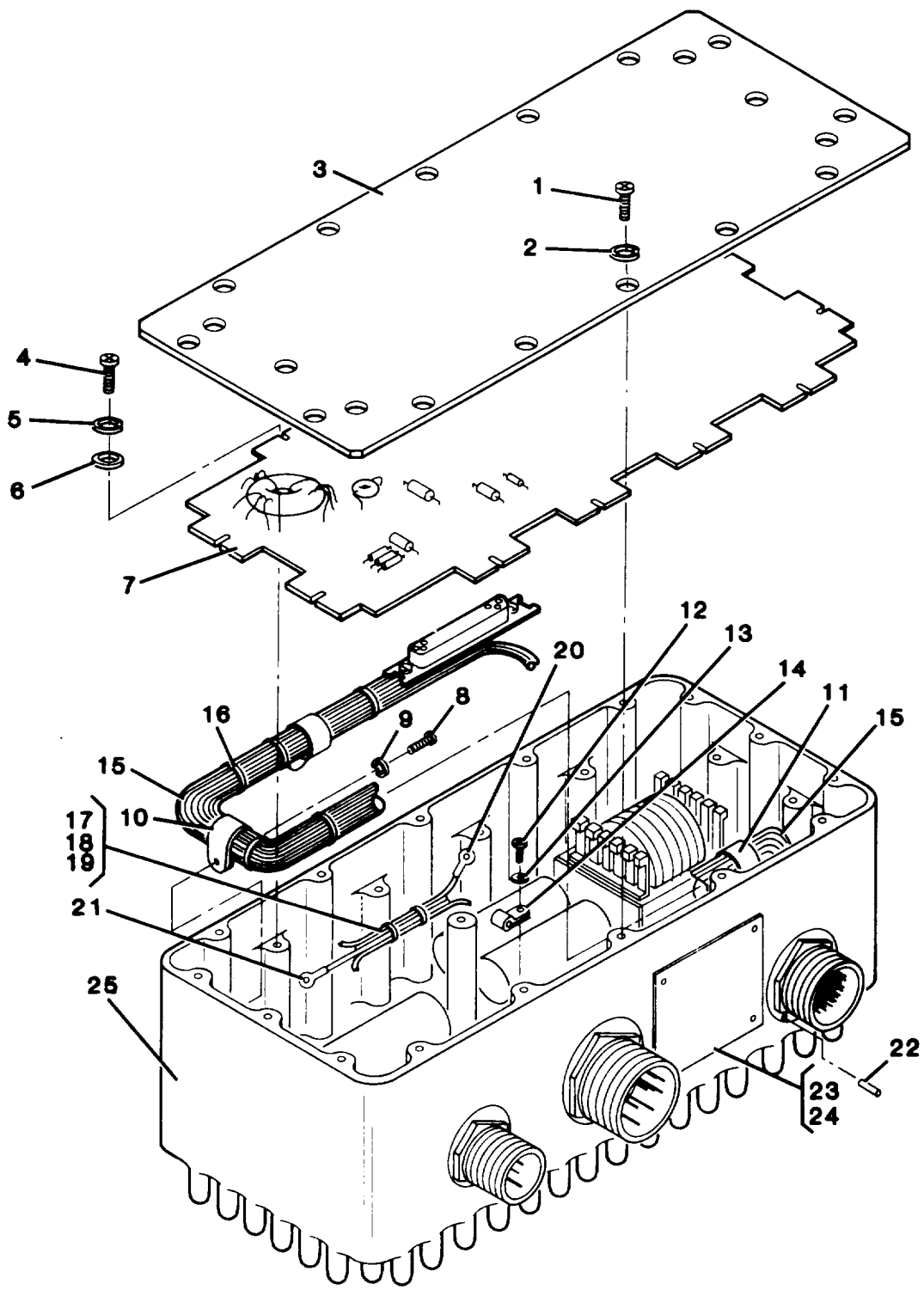
Figure 16. Generator Electronic Control Module (GECM) Assembly
