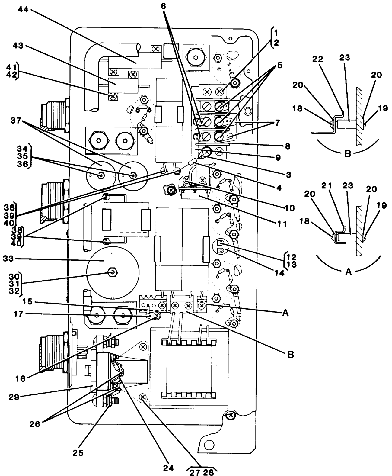
Figure 19A. GECM Components (Terminal Board, Transformer, etc.)
