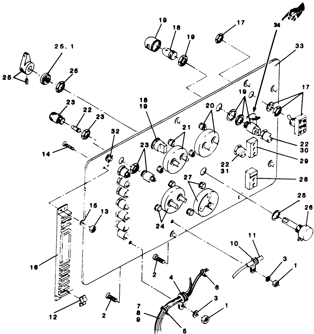
Figure 49. Control Panel Assembly
