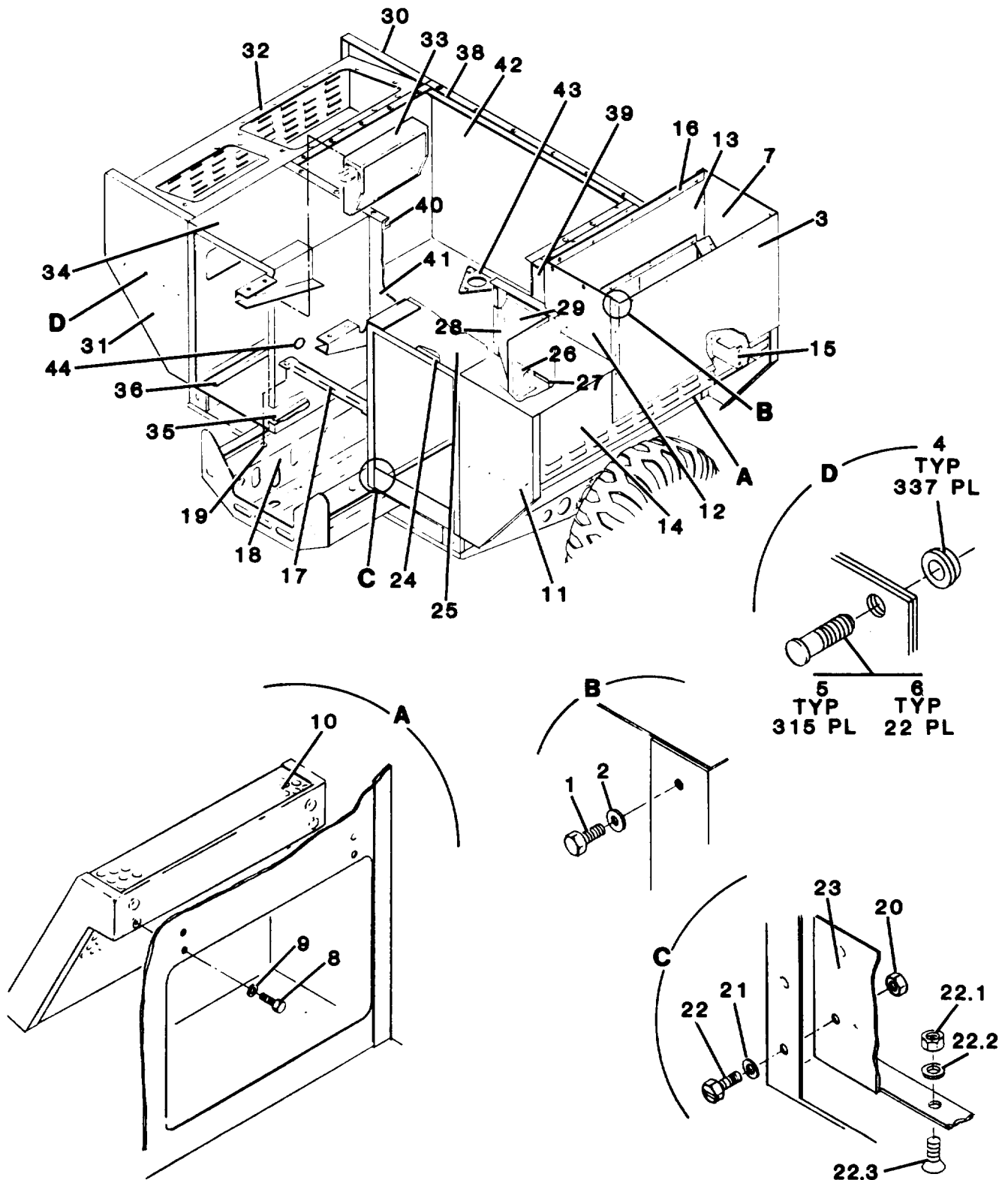
Figure 12. Trailer Body Assembly
