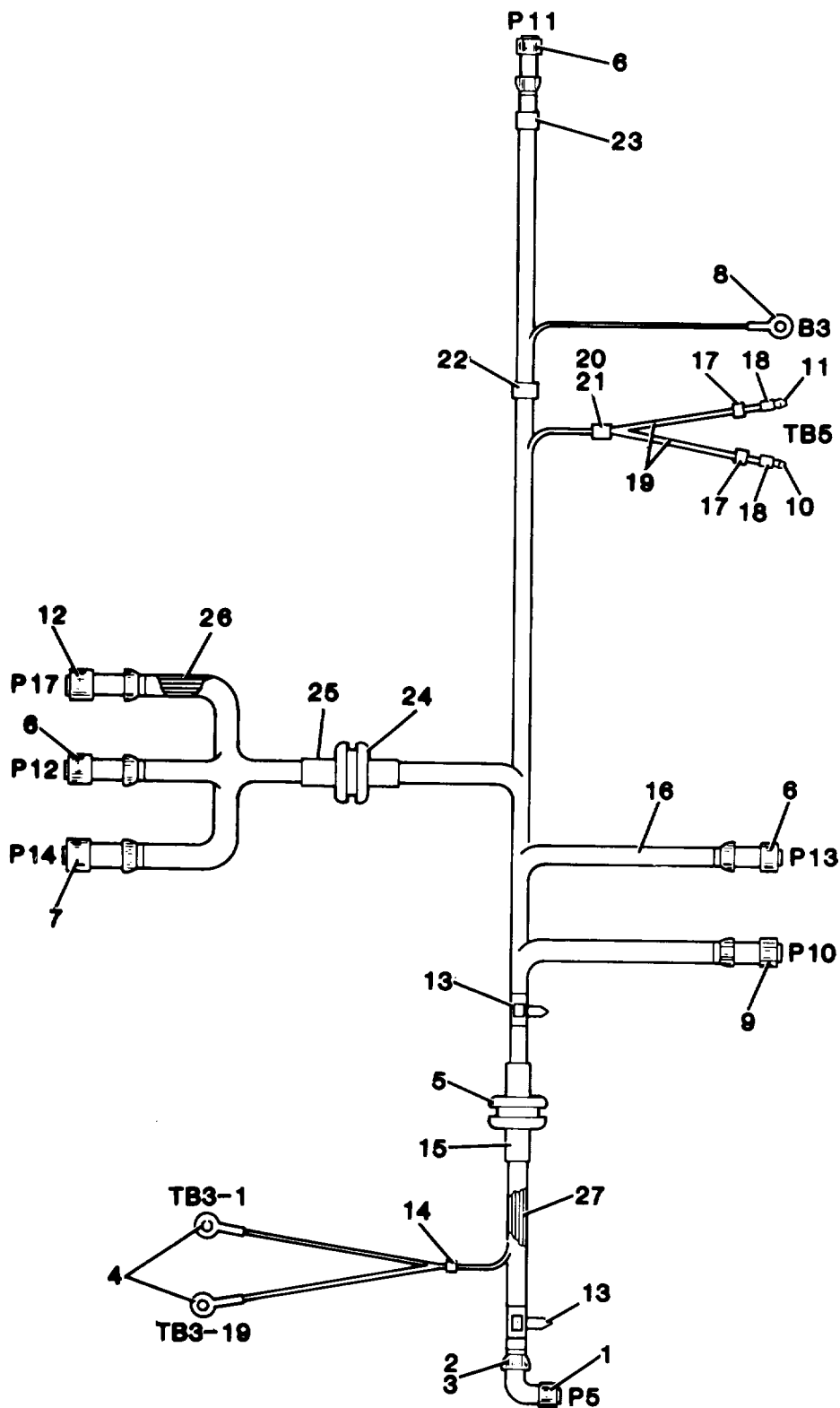
Figure 48. Wiring Harness Assembly (Engine)
