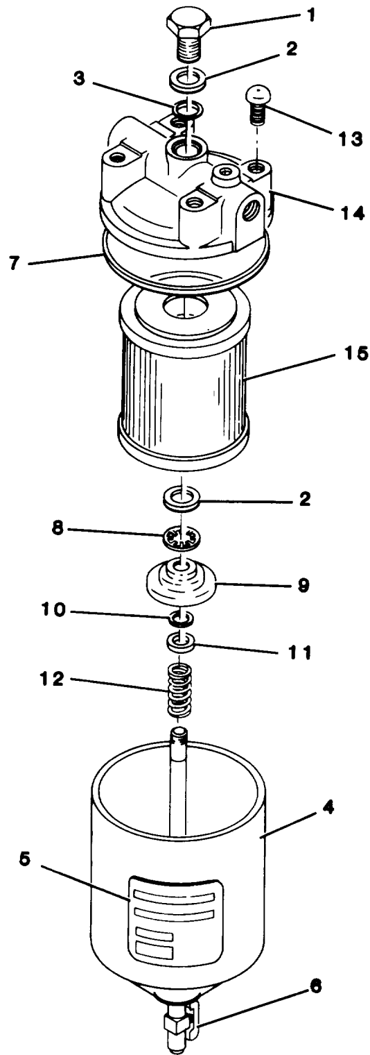
Figure 36. Primary Fuel (Fluid) Filter Assembly
