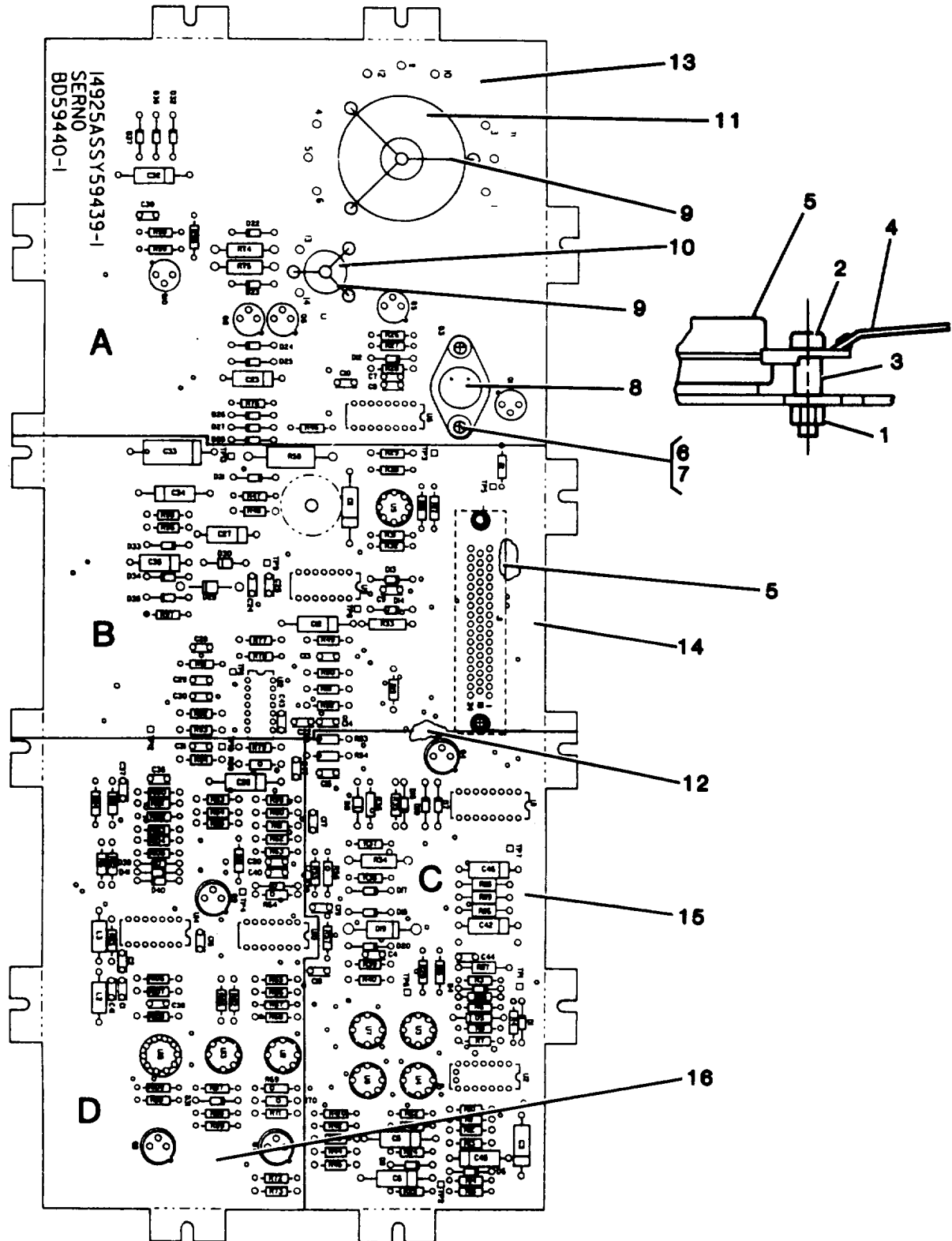
Figure 17. Circuit Card Assembly (GECM)
