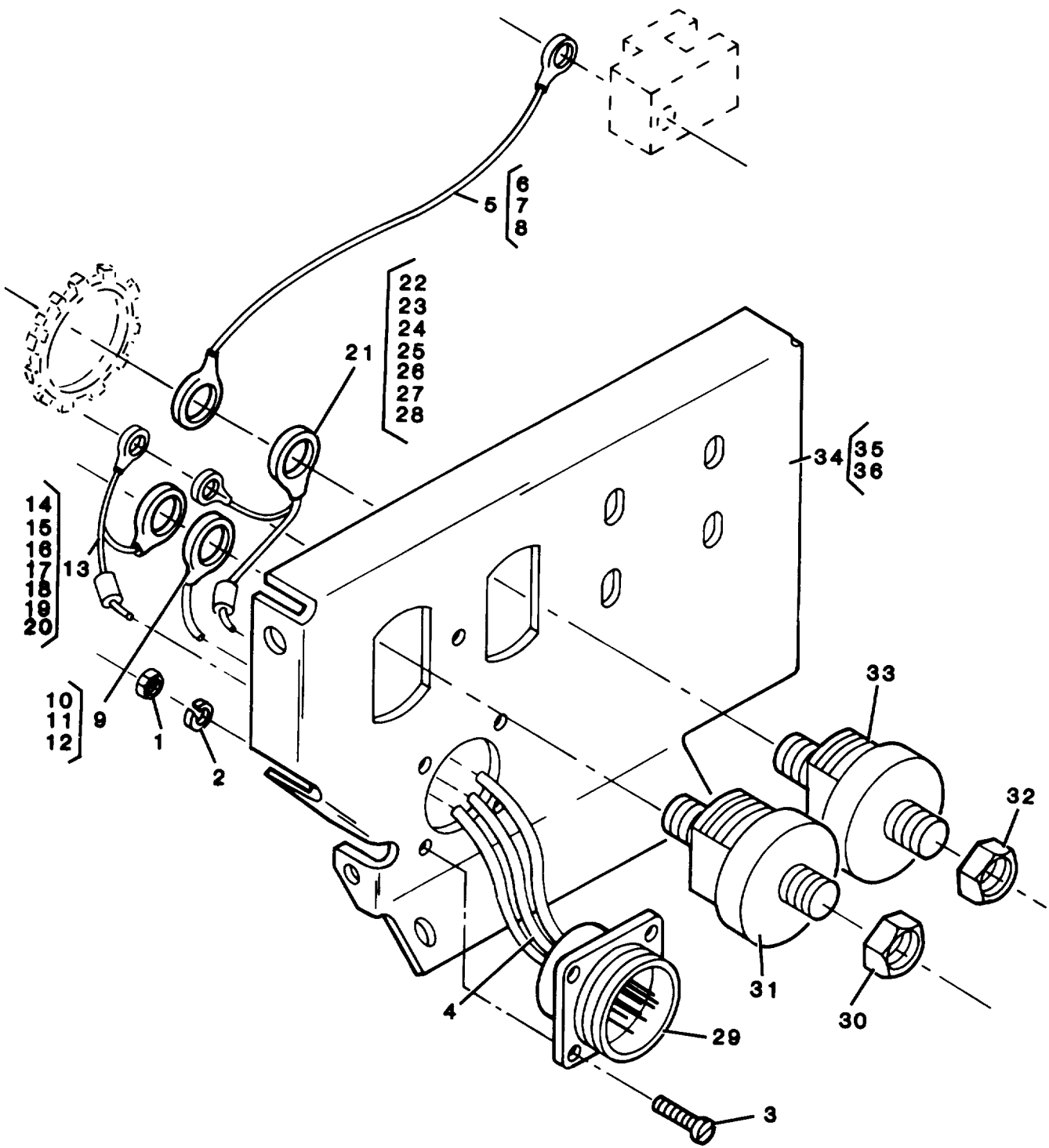
Figure 24A. Generator Filter Left Side Assembly
