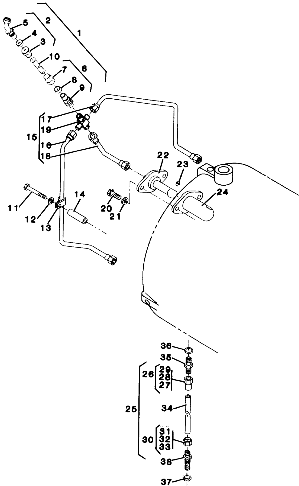
Figure 27. Fuel Manifold and Fuel Injection Nozzles
