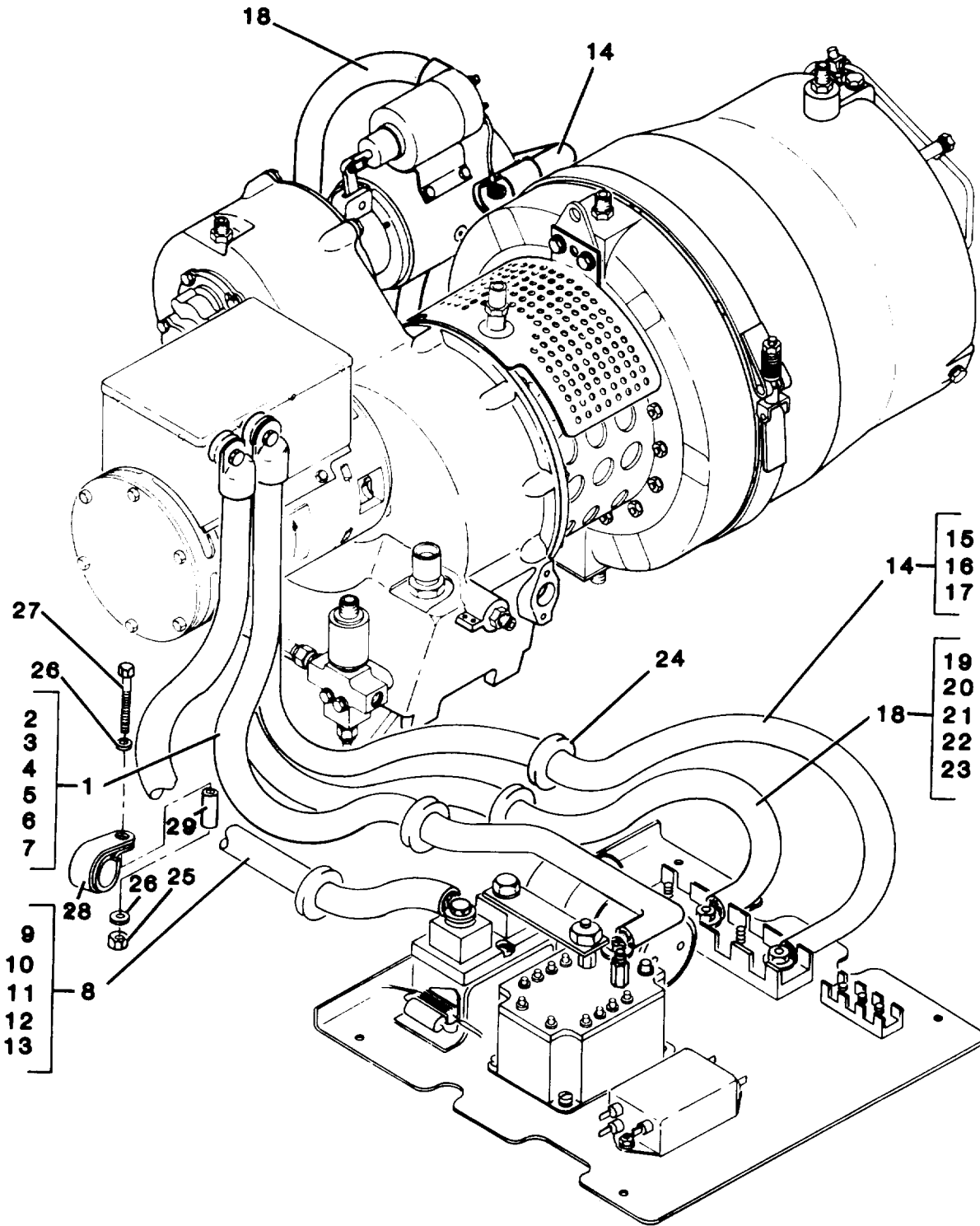
Figure 55. Load Connection (Wiring)
