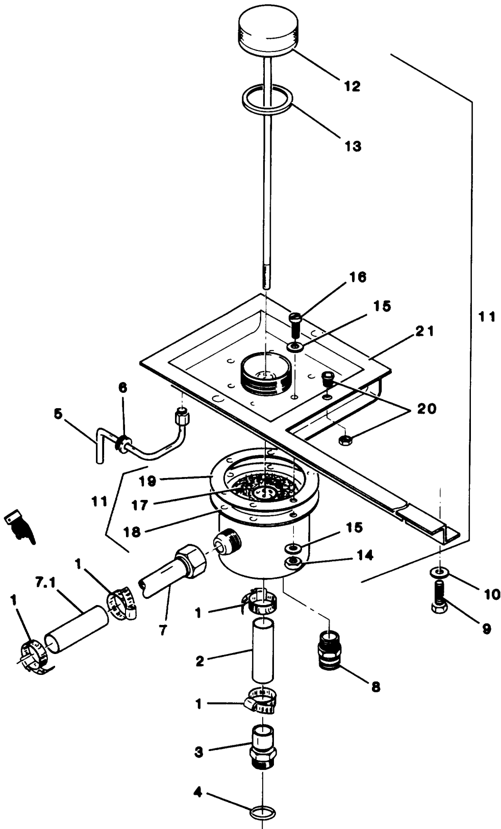
Figure 38. Oil Filler/Breather Assembly
