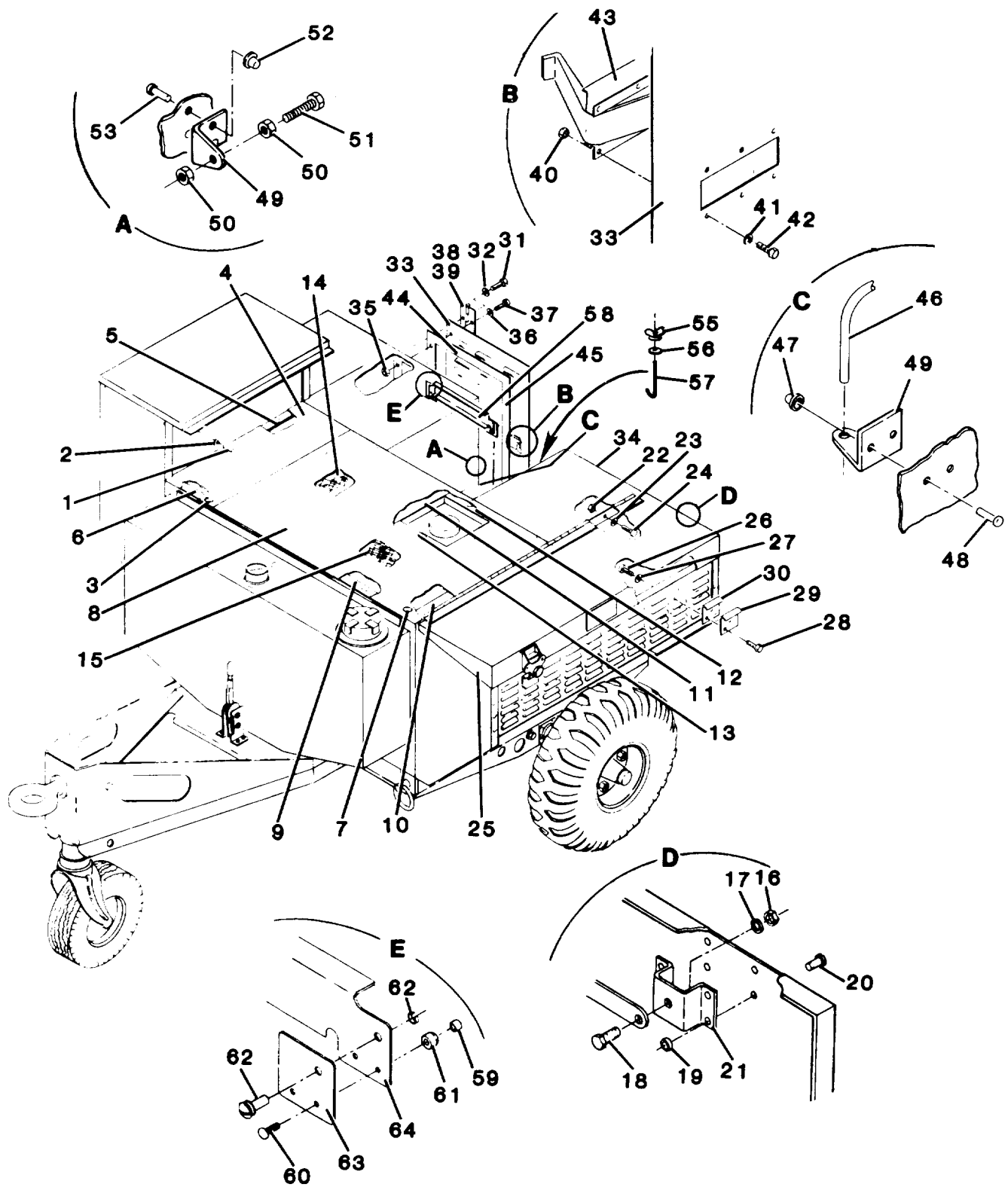
Figure 2. Access Covers and Doors
