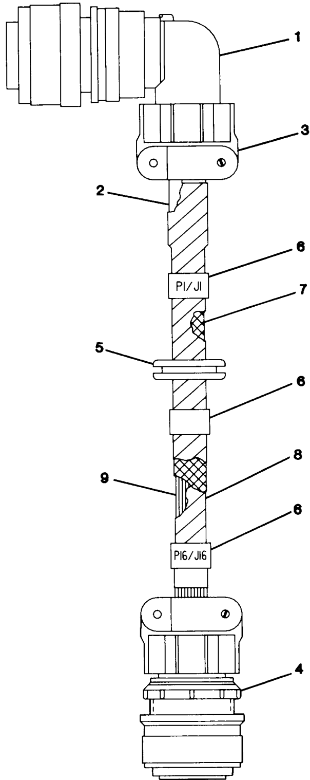
Figure 15. Wiring Harness Assembly (Generator to GEKM)
