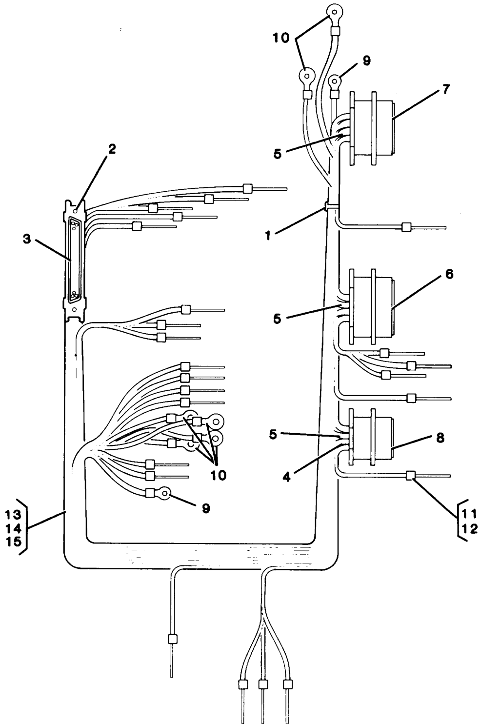
Figure 18. Branched Wiring Harness Assembly (Internal to GECM)
