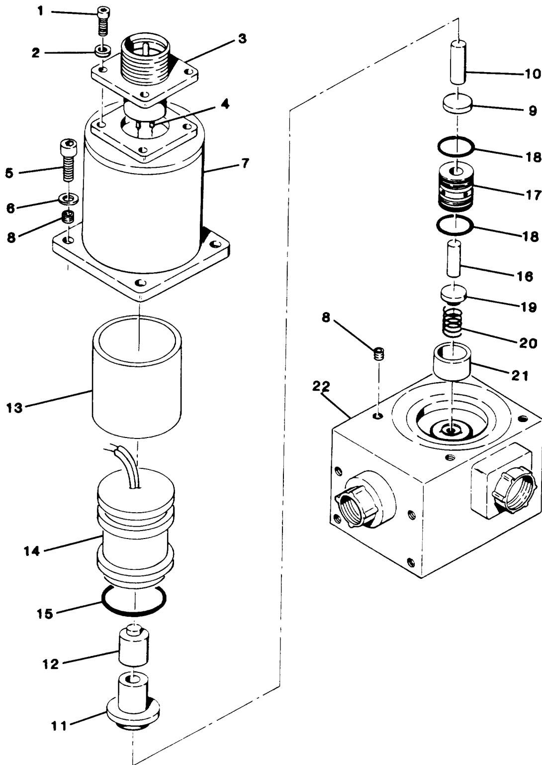
Figure 30. Solenoid Valve Assembly
