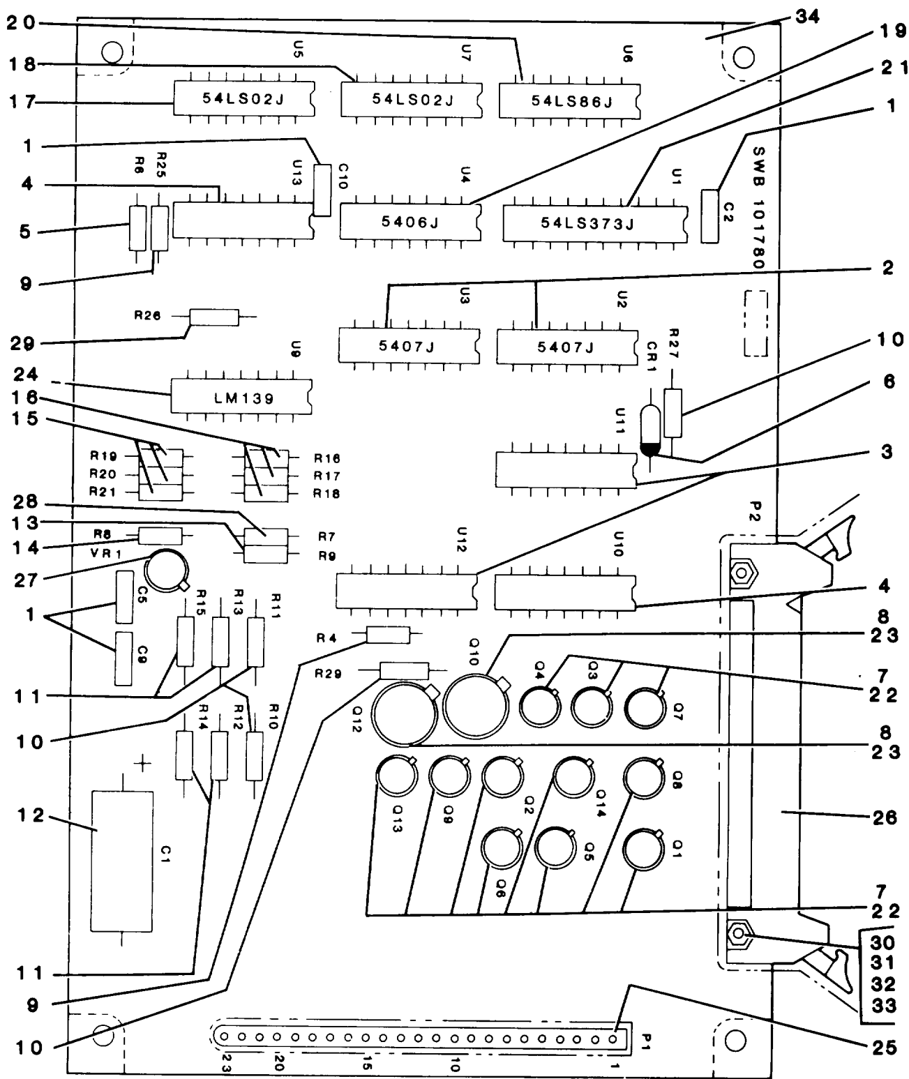
Figure 53. Circuit Card Assembly (Switch)
