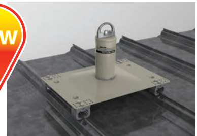
Standing Seam
