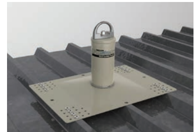
Metal Sheathing
