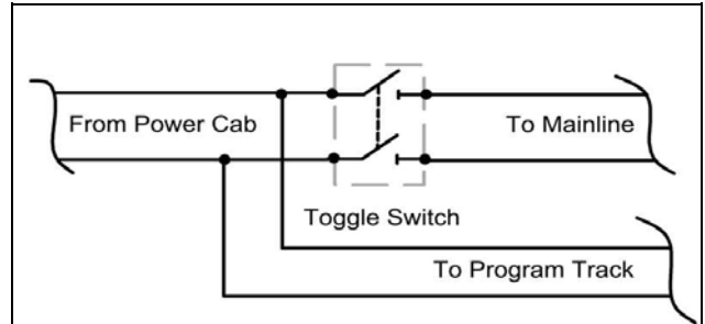
Wiring for Program Track with the Power Cab
