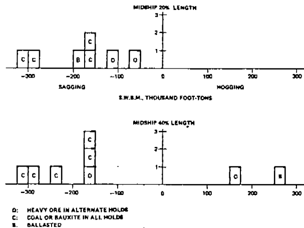
Figure 2-3 Typical Still Water Bending Moments, Ore Carrier FOTINI L. Each box represents one voyage
