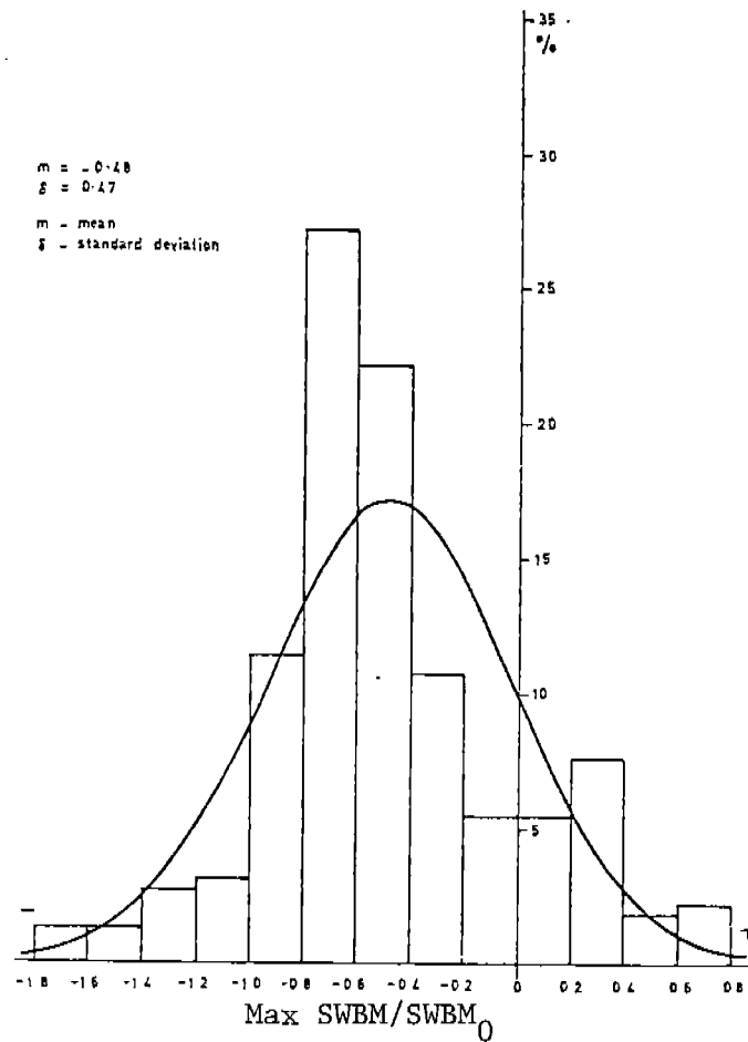
Figure 2-4 Frequency Distribution and Histogram of Max SWBM/SWBM 0 for a General Cargo Ship and Two Bulk Carriers (from Reference 4)
