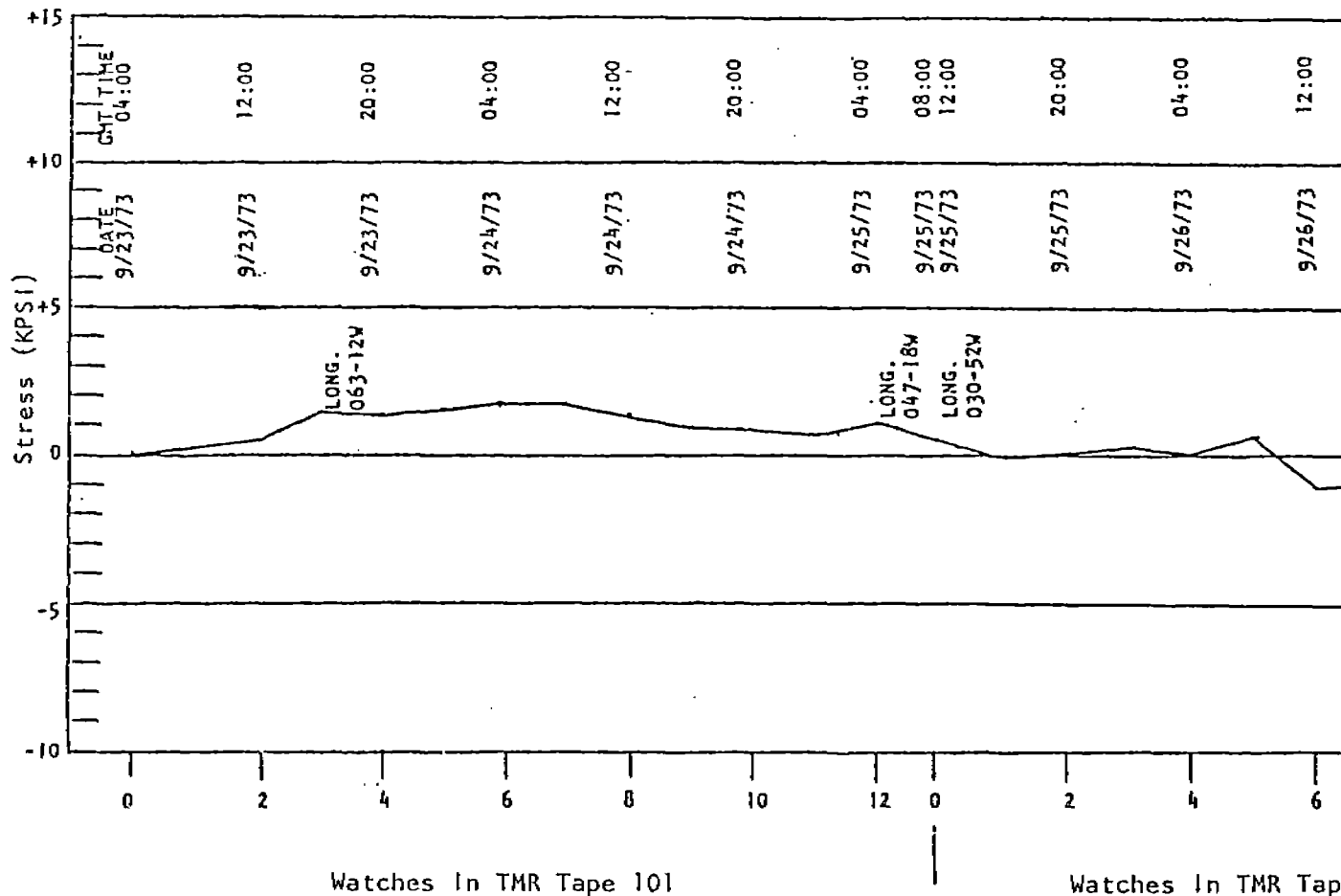
Figure 2-5 SL-7 - Typical Voyage Variation Of The Relative Still Water (from Reference 2)
