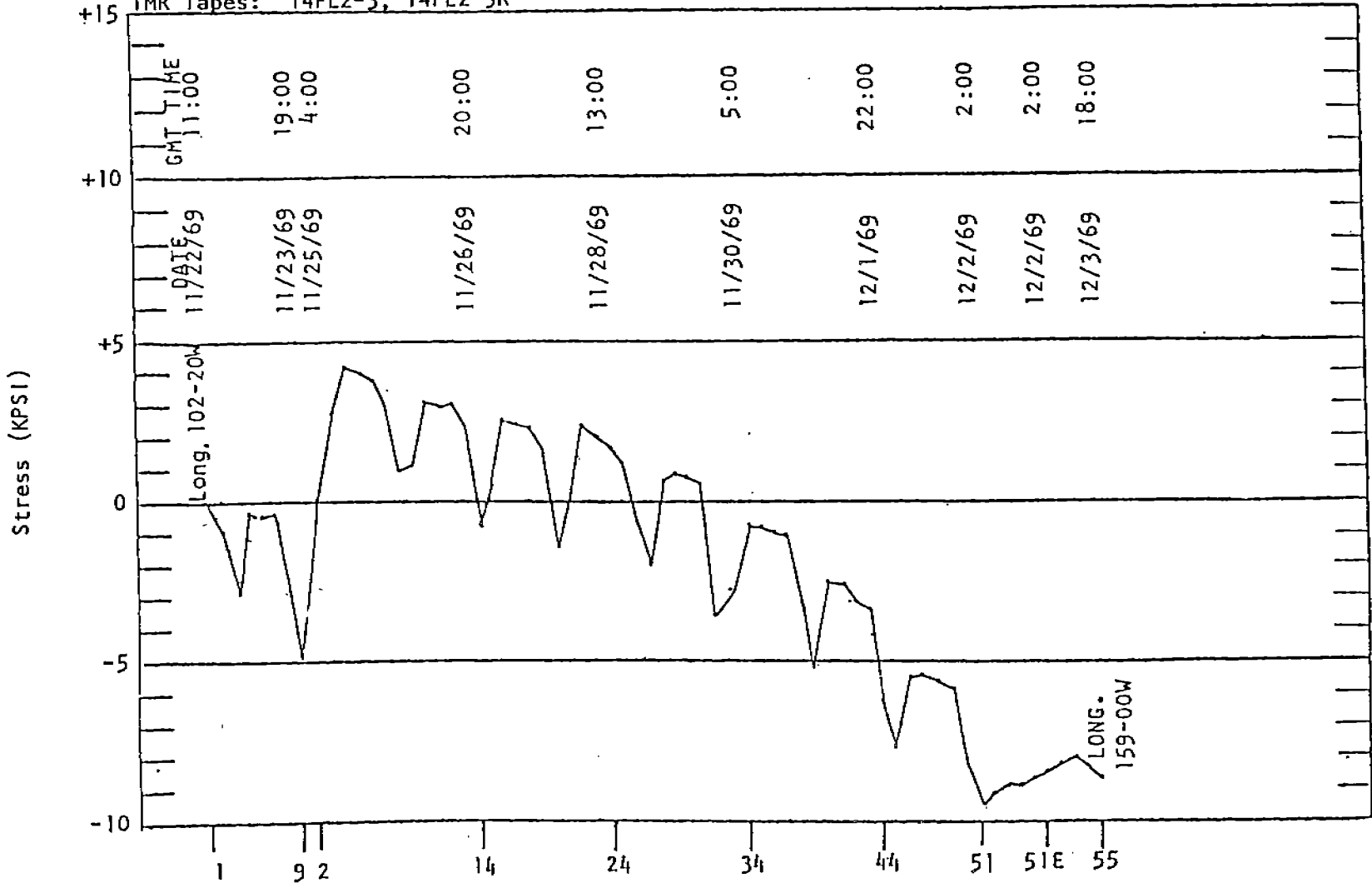
Figure 2-6 FOTINI L - Typical Voyage Variation Of The Relative Still Water Stresses
