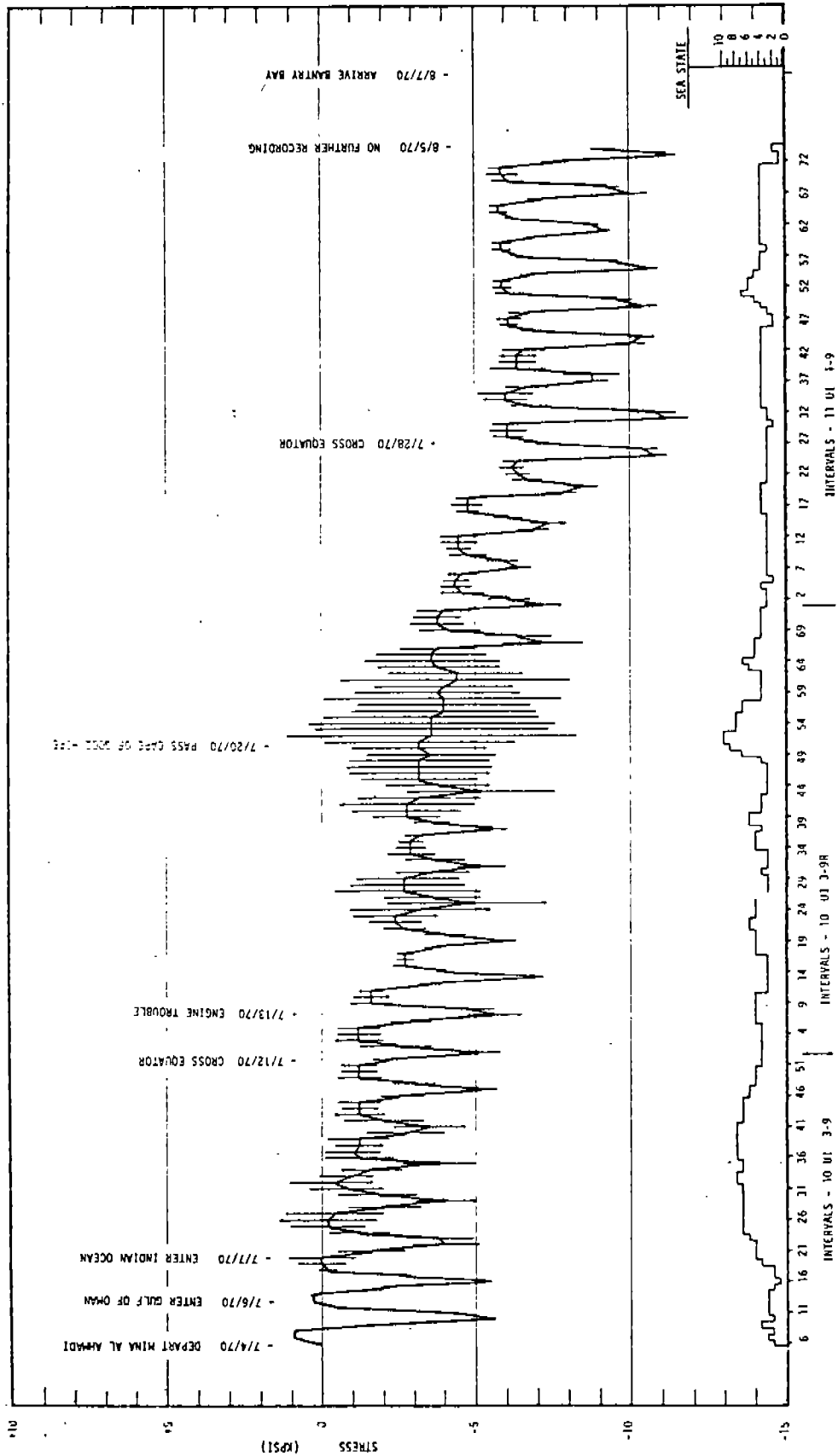
Figure 3-6 Midship Vertical Bending Stress Variations for Loaded Condition of Voyage 10 of UNIVERSE IRELAND
