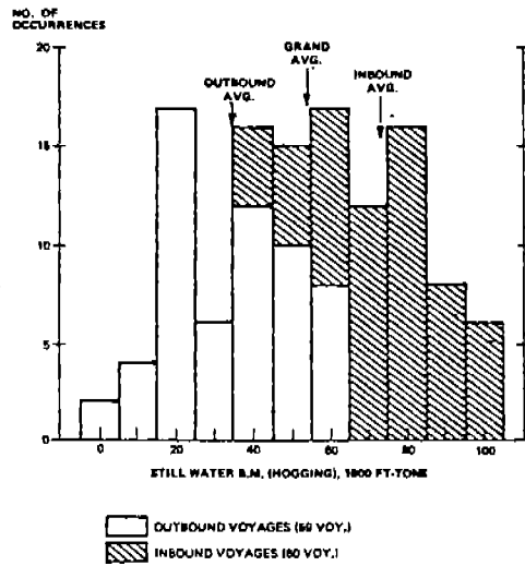
Figure 2-1 Histogram of Still Water Bending Moments, Container-ship NEW ORLEANS
