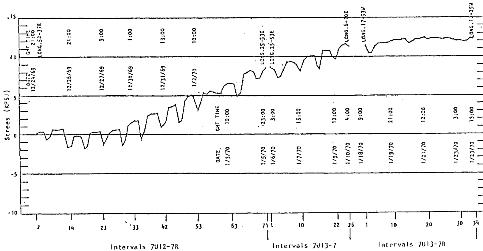
Figure 2-7 UNIVERSE IRELAND - Typical Voyage Variation Of The Relative Still Water Stresses
