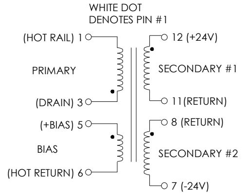
FIGURE 1: SCHEMATIC DIAGRAM
