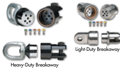
Heavy-Duty Breakaway
