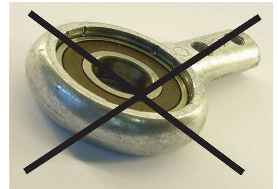
Picture 3: Do not use pressed in bearing holders. The geared hub would slip under load in high gear mode!
