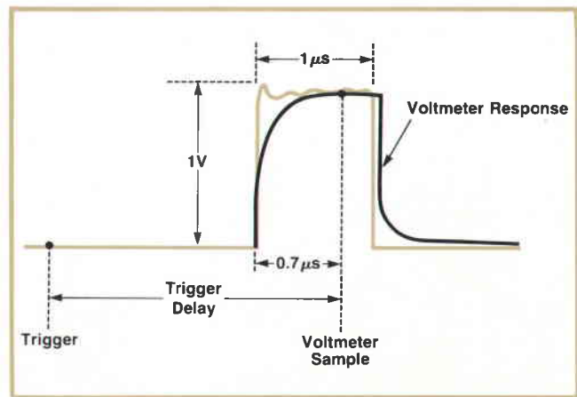
Fig. 4. Model 3437A Systems Voltmeter can be programmed to sample and read the amplitude of a pulse at a point in time precisely related to a trigger by the voltmeter's programmable delay. Uncertainty (jitter) in the location of the sample is less than 10 ns. The voltmeter will be accurate to at least 2% within 0.7 \mu\text{s} after the pulse leading edge.
