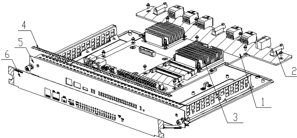
Figure 1 disassembly process
