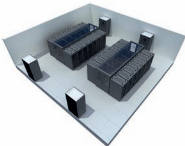
Raised floor data center with perimeter precision cooling (Liebert HPM)
