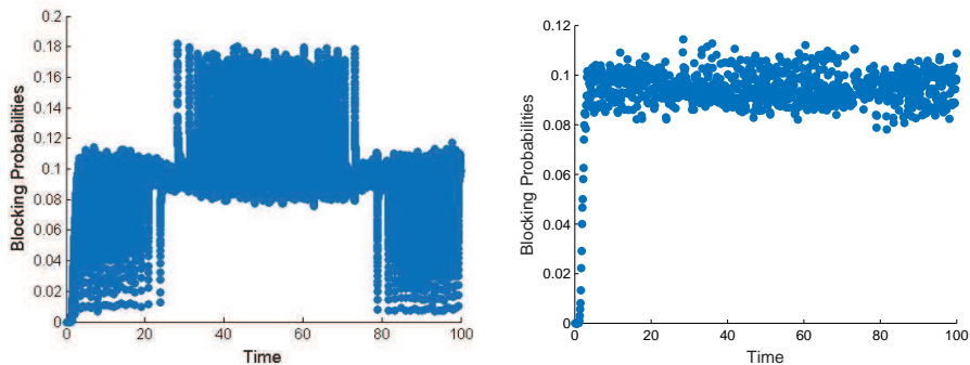
Figure 4: Simulation estimates of the blocking probabilities in the nonstationary M_t/M/s_t/0 model for the sinusoidal arrival rate in (4.19) with blocking probability target B = 0.1 and parameter triple (\bar{\lambda}, \beta, T) = (100, 25, 100) with the MOL staffing algorithm without any averaging, (left) and with randomization (right).
