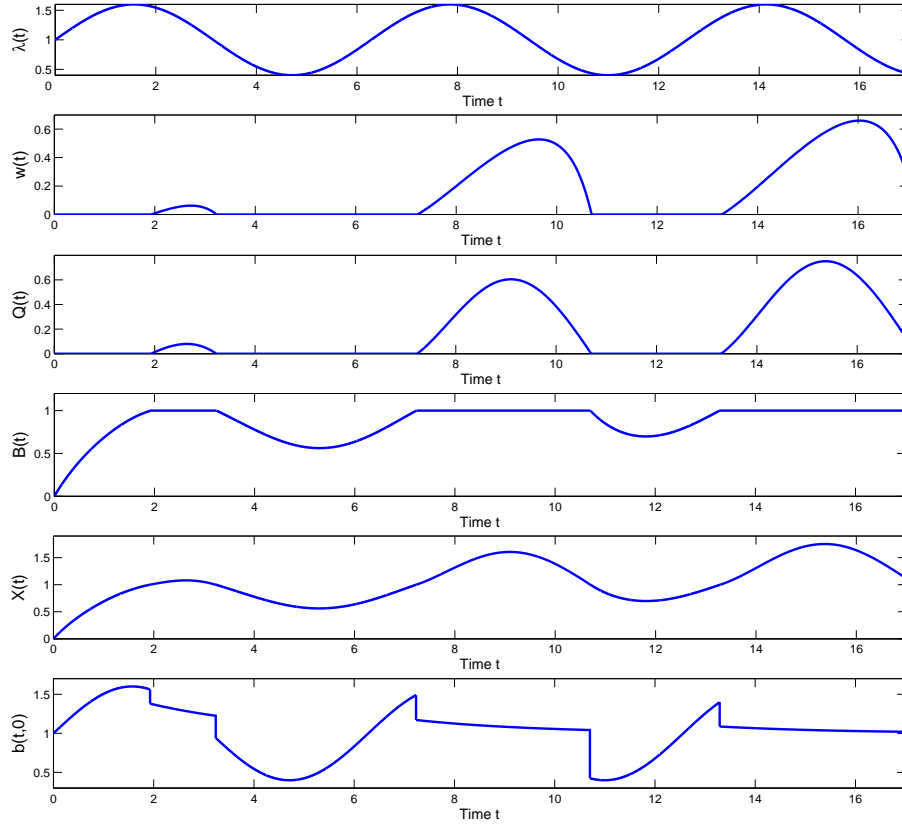
Figure 2: Six performance functions for the G_t/H_2/s + E_2 fluid model with sinusoidal arrival-rate function \lambda(t) = 1 + 0.6 \sin(t) for service capacity s and mean service and patience times equal to 1: (i) arrival rate \lambda(t) ; (ii) head-of-line waiting time w(t) ; (iii) fluid waiting in queue Q(t) ; (iv) fluid in service B(t) ; (v) total fluid in system X(t) ; (vi) rate into service b(t, 0) .
