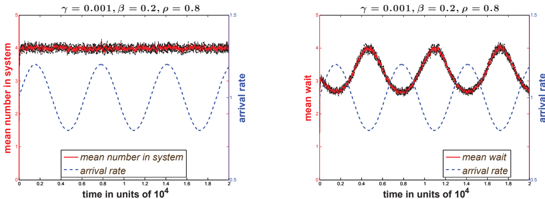
Figure 8: Simulation estimates of the time-varying mean number in the system (left) and the mean virtual waiting time (right), for the M_t/M_t/1 model with sinusoidal arrival rate function \lambda(t) \equiv 1 + \beta \sin \gamma t with \beta = 0.2 and \gamma = 0.001 with the rate-matching control in (7.51) for traffic intensity \rho = 0.8 .
