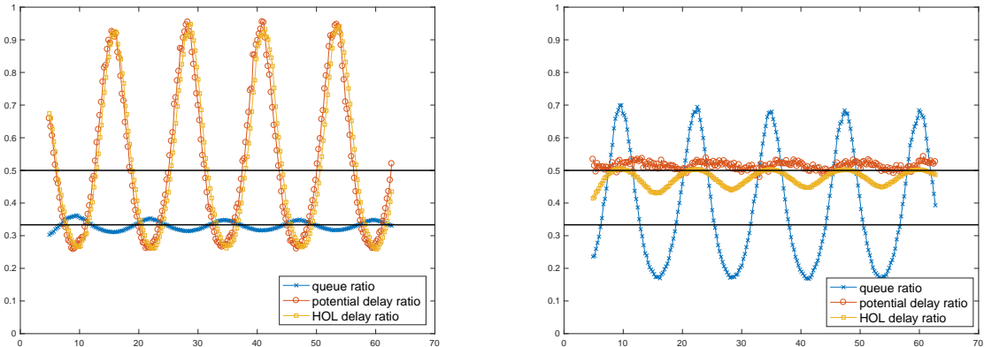
Figure 6: Queue and delay ratios obtained from the FQR rule (left) and HLDR rule (right) for a two-class M_t/M/s_t queue with arrival rate functions \lambda_1(t) = 60 - 20 \sin(t/2) , \lambda_2 = 90 + 30 \sin(t/2) , common service rate \mu = 1 , without abandonment ( \theta_1 = \theta_2 = 0 ) and the QoS parameter \gamma = 0.25
