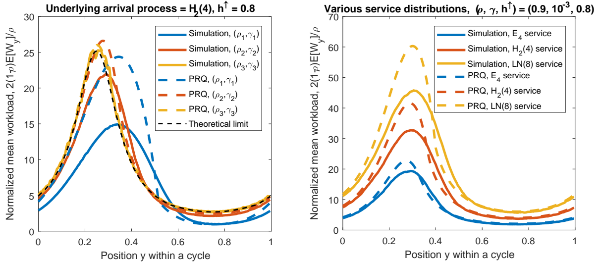
Figure 7: A comparison of the solution to the PRQ problem in (7.43) as a function of the position y within a cycle to simulation estimations and the HT limit in Theorem 5 of Whitt and You (2017a) for the normalized mean workload 2(1 - \rho)E[W_{\gamma,\rho,y}]/\rho for W_{\gamma,\rho,y} in (7.42) in the underloaded (H_2(4)_t/LN(1)/1) model with arrival-rate function in (7.47) for (\gamma, \rho) \in \{(0.7, 10^{-2}), (0.9, 10^{-3}), (0.95, 10^{-4})\} (left) and for three different service-time distributions (right).
