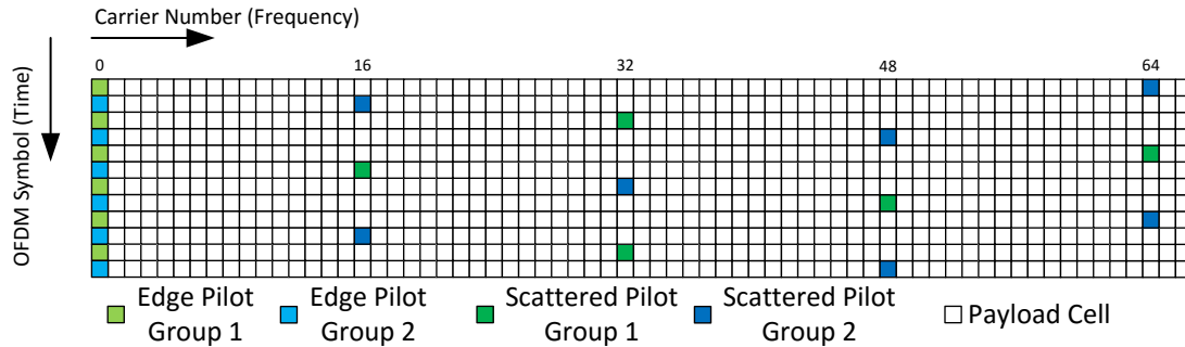
Figure L.11.24 MIMO pilot scheme MP16_4 for null pilot encoding.
