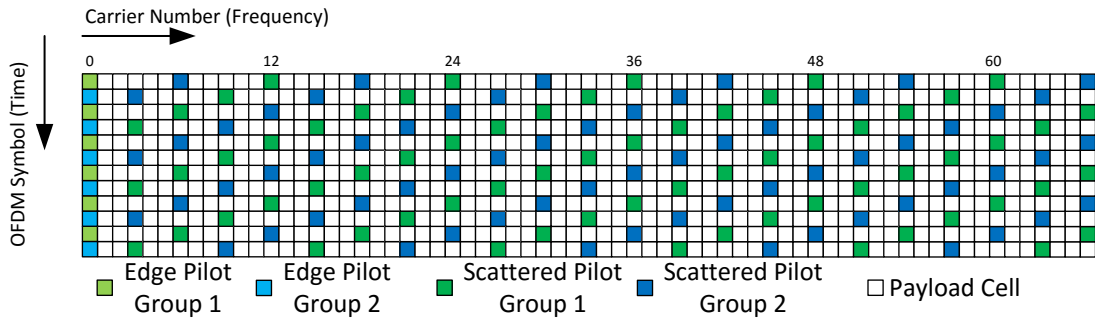
Figure L.11.13 MIMO pilot scheme MP3_2 for null pilot encoding.
