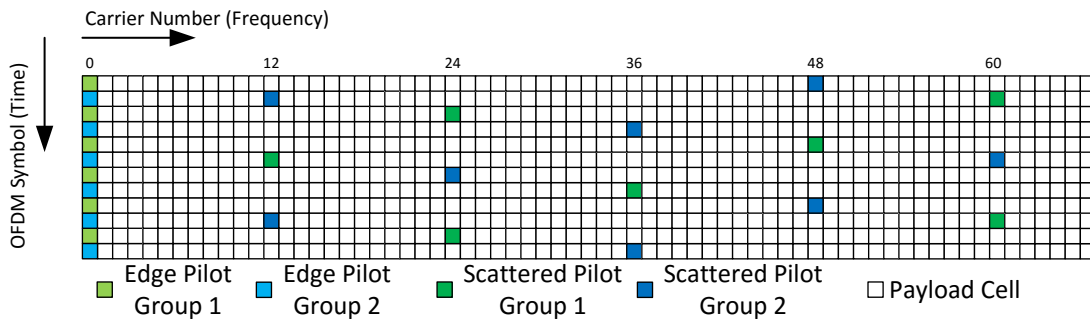
Figure L.11.22 MIMO pilot scheme MP12_4 for null pilot encoding.
