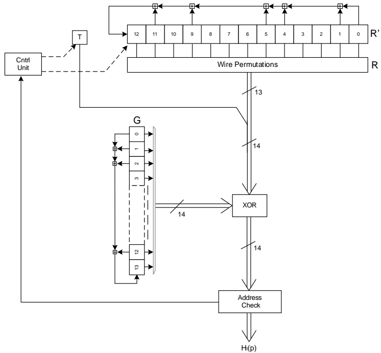
Figure 7.28 FI address generation scheme for the 16K FFT size.
