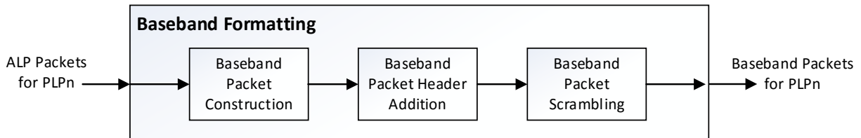
Figure 5.2 Block diagram of baseband formatting.
