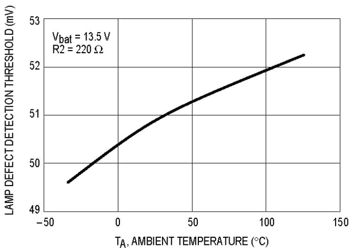
Figure 7. Defect Lamp Detection Versus Temperature
