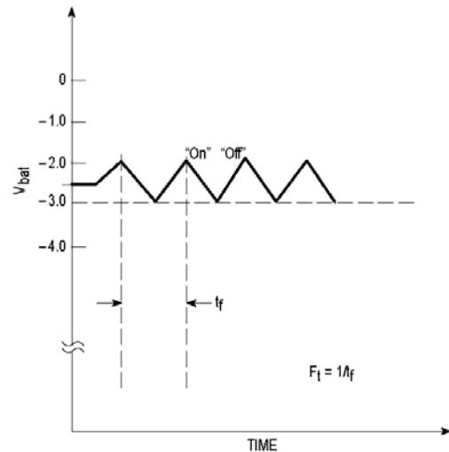
Figure 2. One Defective Lamp Oscillator Timing Diagram
