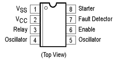
P SUFFIX PLASTIC PACKAGE CAS 626
