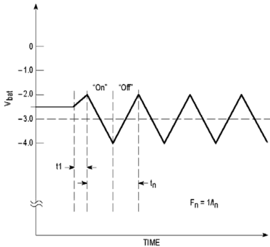
Figure 1. Normal Operation Oscillator Timing Diagram
