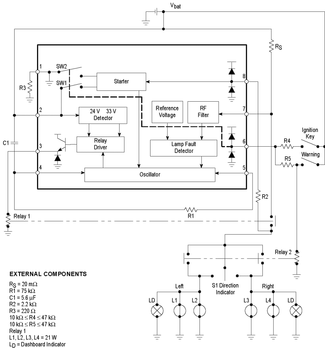
Figure 10. Typical MC33193 Application
