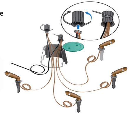
12/2 Low voltage cable wire 20AMP rated, 240W, 12V for landscape lighting
