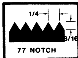
FOR CERAMIC, ALUMINUM AND OTHER METAL TILE.
