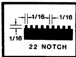
FOR LINOLEUM, LINOLEUM TILE AND ASPHALT TILE.
