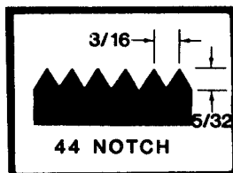
FOR PLASTIC WALL TILE, CERAMIC AND METAL TILE.
