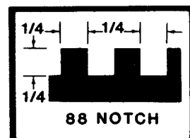
FOR CERAMIC TILE INSTALLED WITH THIN SET MORTAR.
