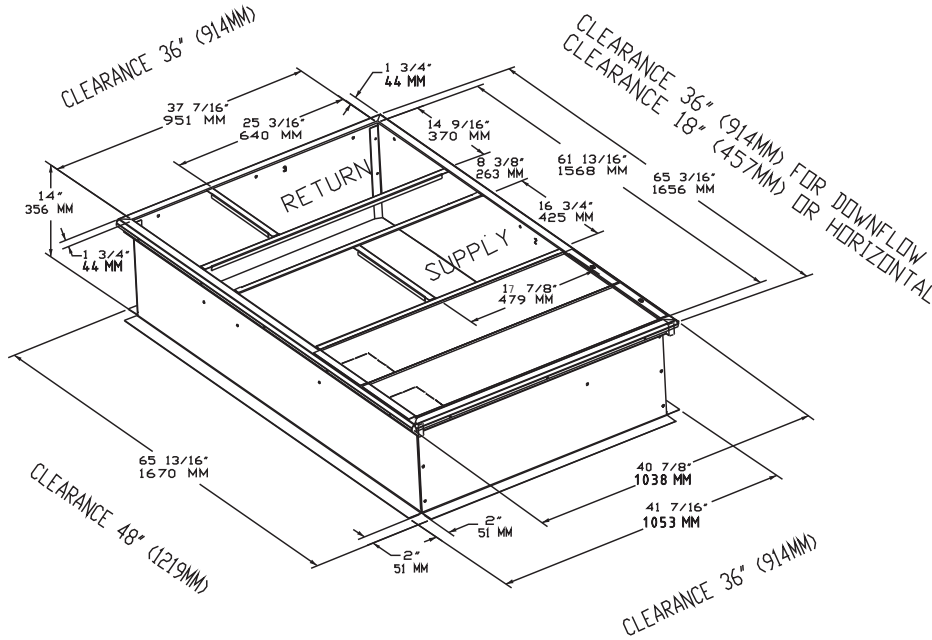
Figure 8. Cooling and gas/electric - 3-5 tons standard efficiency; 3 tons high efficiency downflow duct connections - field fabricated
