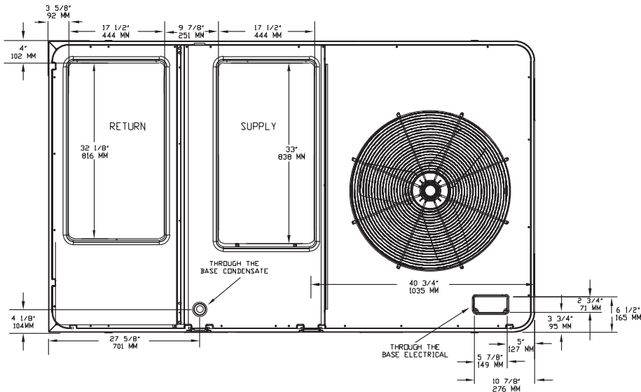
Figure 22. Cooling and gas/electric - 7½ tons (dual compressor standard efficiency) - 10 tons standard efficiency, 6 tons high efficiency, 7½ tons (microchannel) high efficiency; downflow airflow supply/return through the base utilities
