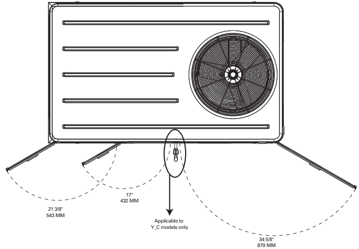
Figure 28. Cooling and gas/electric - 7½ tons (dual compressor standard efficiency), 10 tons standard efficiency, 6 tons high efficiency, 7½ tons (microchannel) high efficiency; swing diameter for hinged door(s) option
