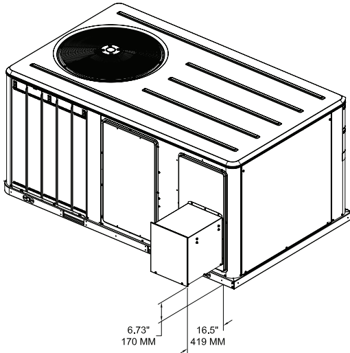
Figure 27. Cooling and gas/electric - 7½ tons (dual compressor standard efficiency), 10 tons standard efficiency, 6 tons high efficiency, 7½ tons (microchannel) high efficiency; power exhaust
