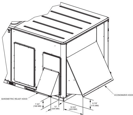
Figure 39. Cooling and gas/electric - 7½ tons (dehumidification) high efficiency, 8½-10 tons high efficiency - economizer, manual or motorized fresh air damper
