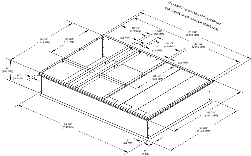
Figure 36. Cooling and gas/electric - 7½ tons (dehumidification) high efficiency, 8½-10 tons high efficiency; duct connections field fabricated
