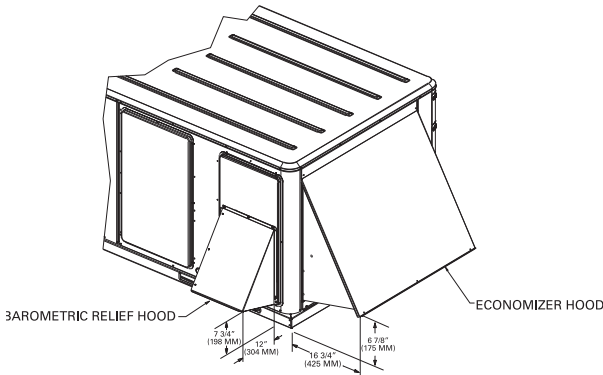
Figure 29. Cooling and gas/electric - 6-10 tons standard efficiency, 4-6 tons high efficiency, 7½ tons (microchannel) high efficiency; economizer, manual or motorized fresh air damper
