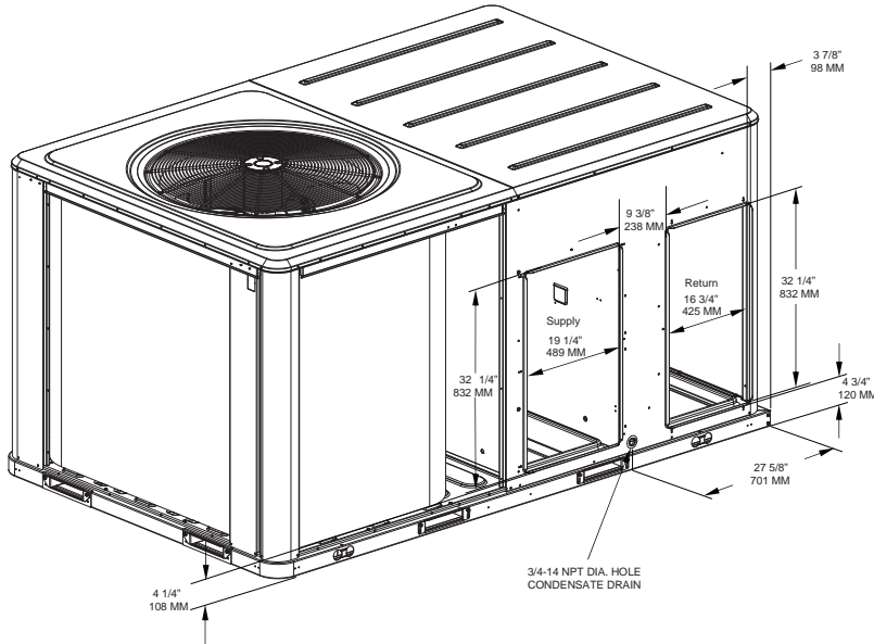
Figure 34. Cooling and gas/electric - 7½ tons (dehumidification) high efficiency, 8½-10 tons high efficiency; unit clearance and roof opening
