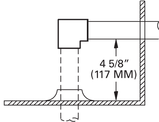
Figure 30. Gas/electric - 6-10 tons standard efficiency, 4-6 tons high efficiency, 7½ tons (microchannel) high efficiency; height of gas pipe required from inside base of unit to gas shut off assembly (factory provided) - Y_C models only
