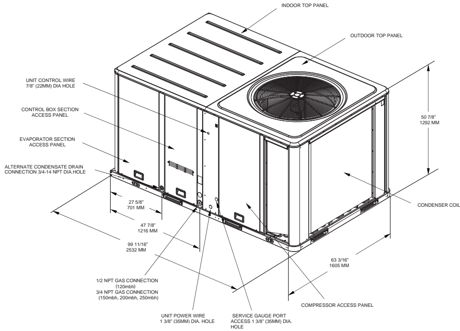
Figure 32. Cooling and gas/electric - 7½ tons (dehumidification) high efficiency, 8½-10 tons high efficiency; downflow airflow supply/return, through the base utilities
