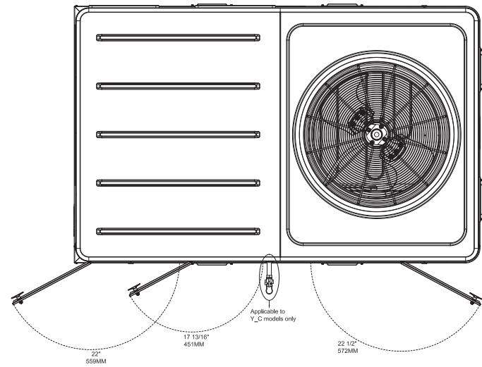
Figure 38. Cooling and gas/electric - 7½ tons (dehumidification) high efficiency, 8½-10 tons high efficiency; swing diameter for hinged door(s) option
