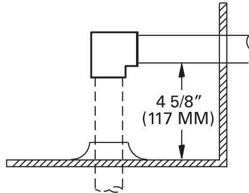
Figure 40. Gas/electric - 7½ tons (dehumidification) high efficiency, 8½-10 tons high efficiency - height of gas pipe required from inside base of unit to gas shut off assembly (factory provided) - Y_C models only
