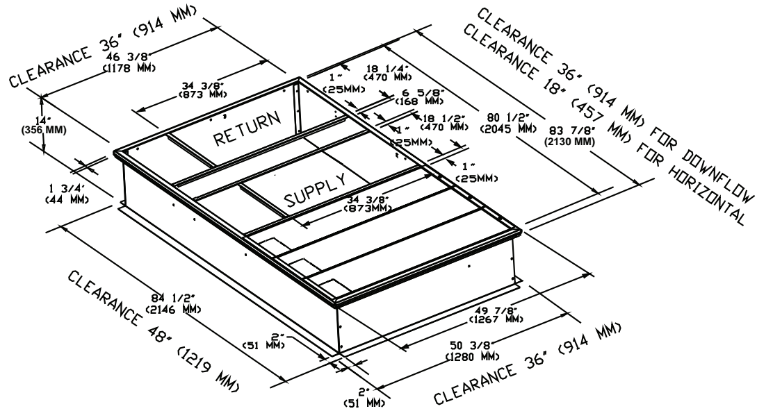
Figure 26. Cooling and gas/electric - 7½ tons (dual compressor standard efficiency), 10 tons standard efficiency downflow, 6 tons high efficiency, 7½ tons (microchannel) high efficiency; duct connections field fabricated
