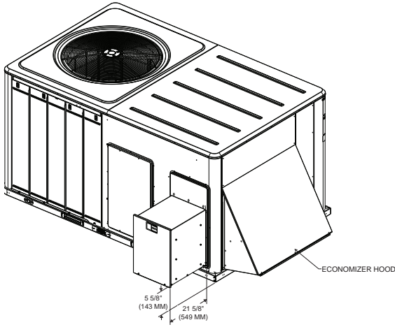
Figure 37. Cooling and gas/electric - 7½ tons (dehumidification) high efficiency, 8½-10 tons high efficiency - power exhaust
