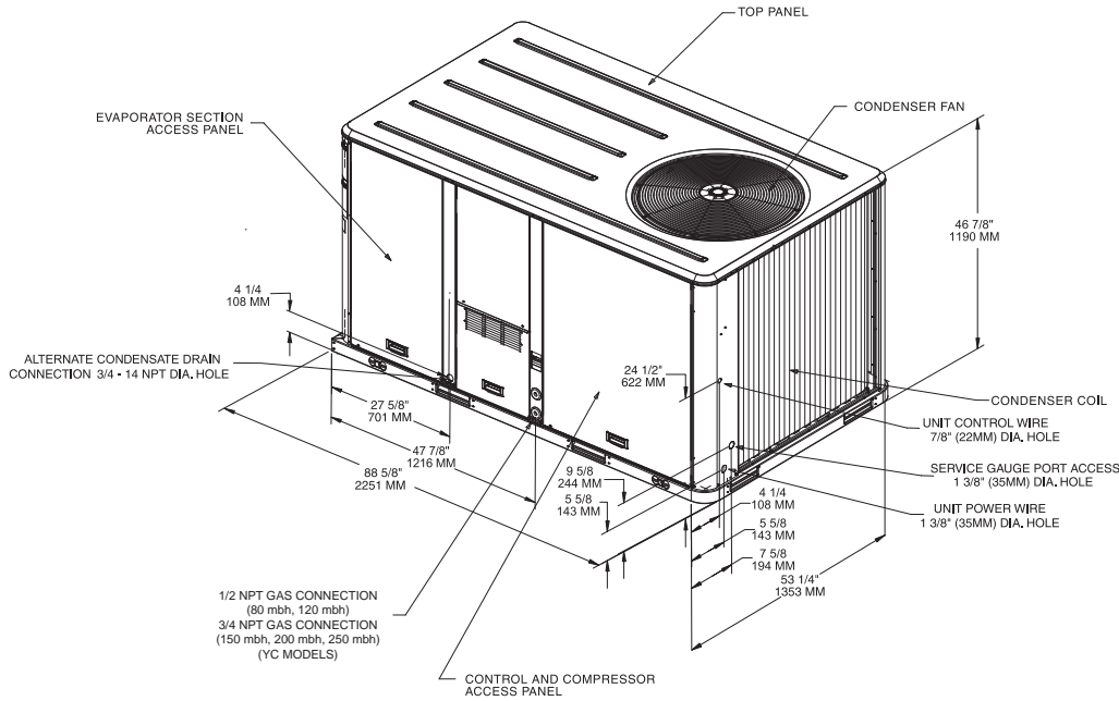
Figure 22. Cooling and gas/electric - 7½ tons (dual compressor standard efficiency) - 10 tons standard efficiency, 6 tons high efficiency, 7½ tons (microchannel) high efficiency; downflow airflow supply/return through the base utilities
