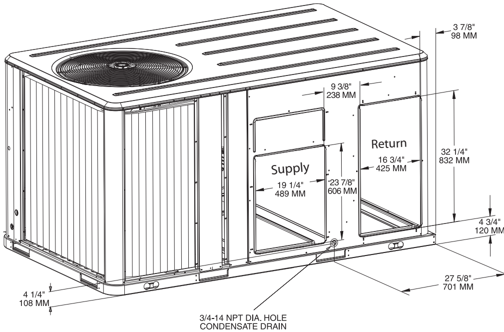
Figure 24. Cooling and gas/electric - 7½ tons (dual compressor standard efficiency), 10 tons standard efficiency, 6 tons high efficiency, 7½ tons (microchannel) high efficiency; unit clearance and roof opening
