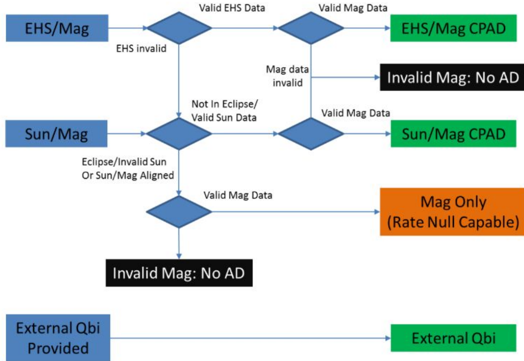
Figure 15. Attitude Determination Operational Flow
