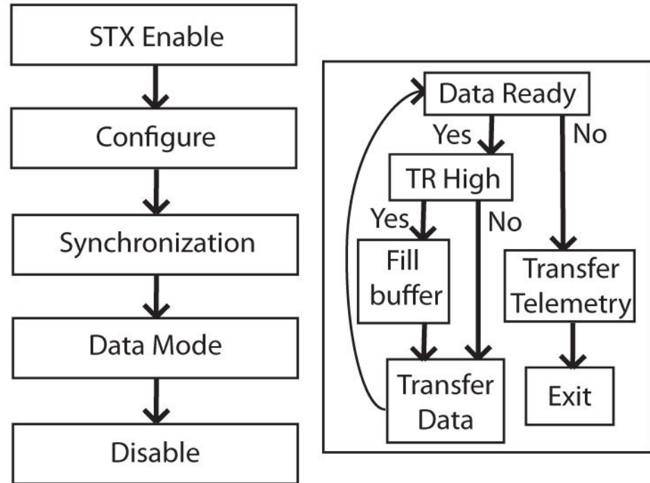
S-Band Control
