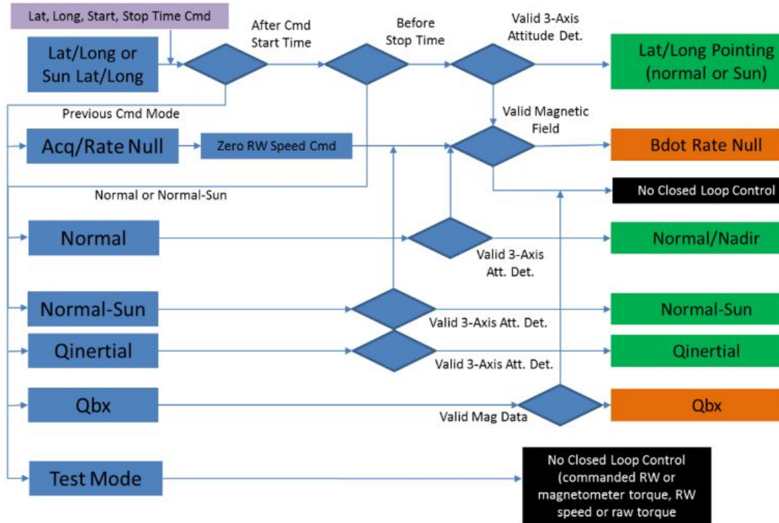
Figure 14. Attitude Control Operational Mode Logic Flow
