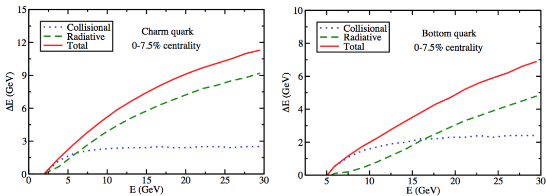
FIGURE 2.11: Comparison of radiative and collisional energy losses for charm (left) and for bottom (right) quarks as a function of the quark energy from calculations in [124].
