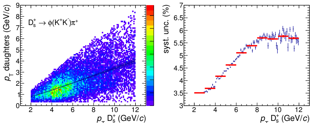
FIGURE 4.25: Left: scatter plot of daughter p_T versus D_s -meson p_T . Right: final systematic uncertainties propagated at D_s -meson level, after weighting for daughter kinematics, as a function of p_T .
