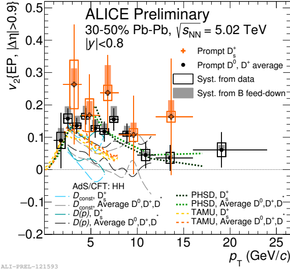
FIGURE 5.35: v_2 of D_s mesons for Pb-Pb collisions at \sqrt{s_{\text{NN}}} = 5.02 TeV in the 30-50% centrality class [41] compared with the PHSD [245] and TAMU [170] model calculations.
