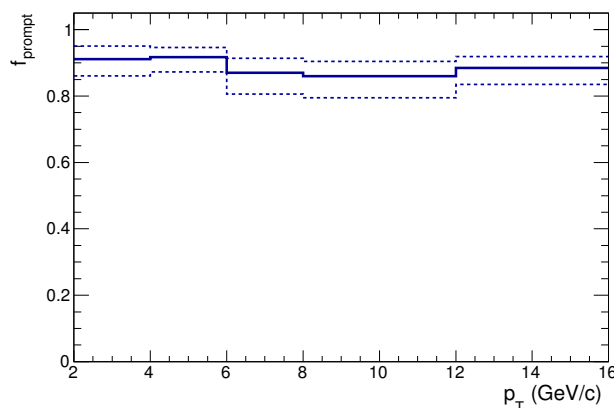
FIGURE 6.11: Fraction of prompt D_s in the p_T intervals considered for the analysis.
