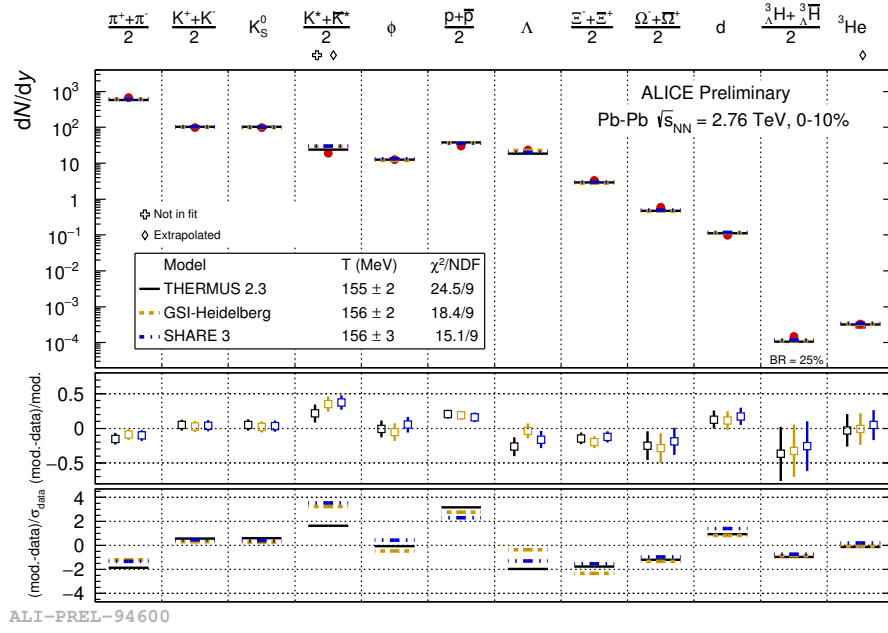
FIGURE 1.8: Grand Canonical thermal fit to ALICE 0-10% Pb-Pb data at \sqrt{s_{NN}} = 2.76 TeV [152], with \mu_B , \gamma_s , \gamma_c fixed to 1, 0 and 20 respectively.
