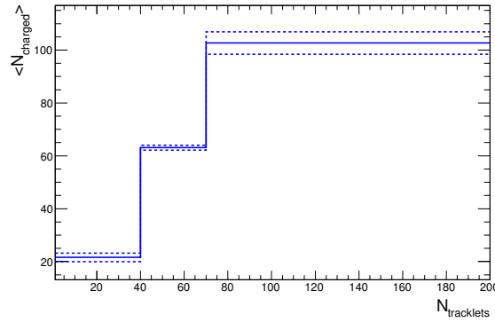
FIGURE 6.18: Average N_{\text{ch}} values in |\eta| < 1 for the considered multiplicity classes. The lower and higher dashed lines represent the systematic uncertainties.
