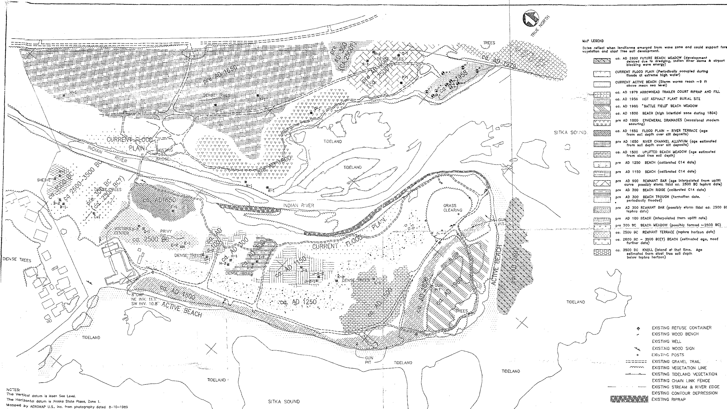
MAP 1 LANDFORM CHRONOLOGY SITKA NATIONAL HISTORICAL PARK
